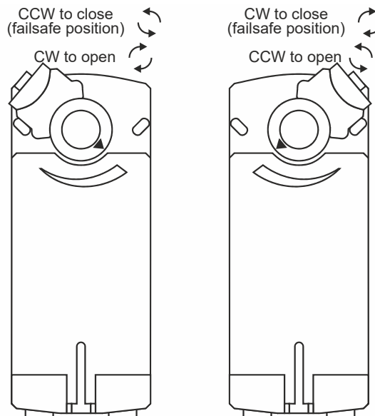
Fig. 2. Mounting orientation
