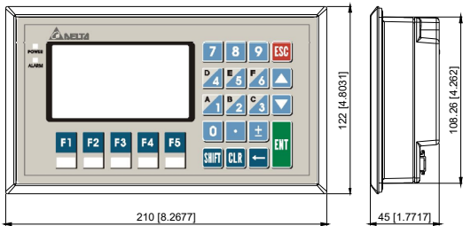
Front Panel and Right Side Diagram
