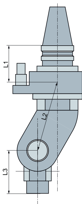
Gambar 12-17 Adaptor kepala crossover
