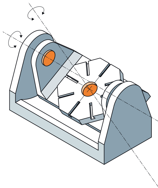
Meja putar 90^{\circ}/90^{\circ}
