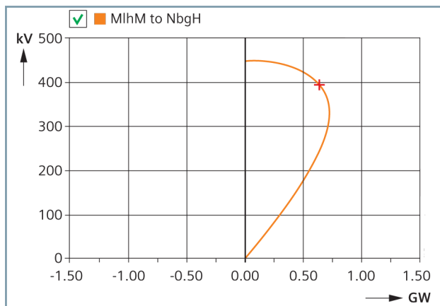
Figure 6.3/3 Voltage Stability Curve
