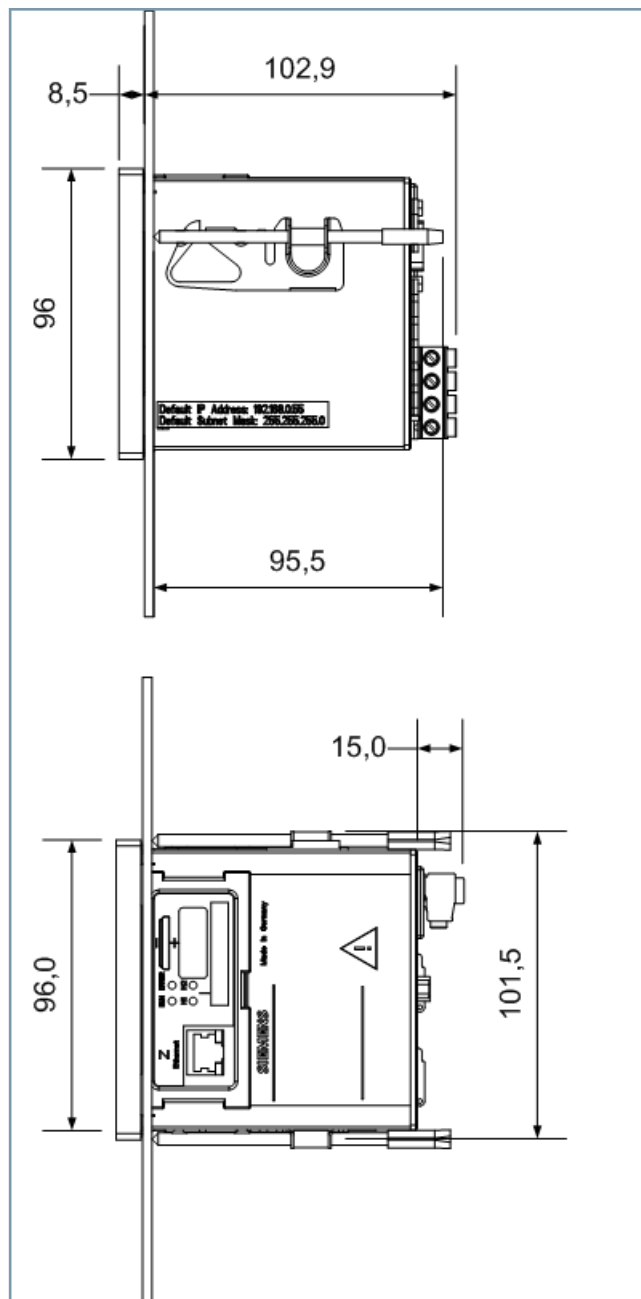
Figure 3.1/17 Dimensional Drawing of the SICAM P850/P855 with Display
