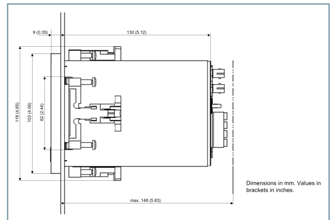
Figure 2.2/16 Side View SICAM Q200
