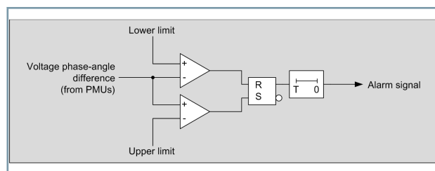
Figure 6.3/9 Deriving a Signal From Voltage-Angle Differences
