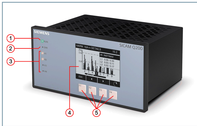
Figure 2.2/14 Layout of SICAM Q200 – Front Side
