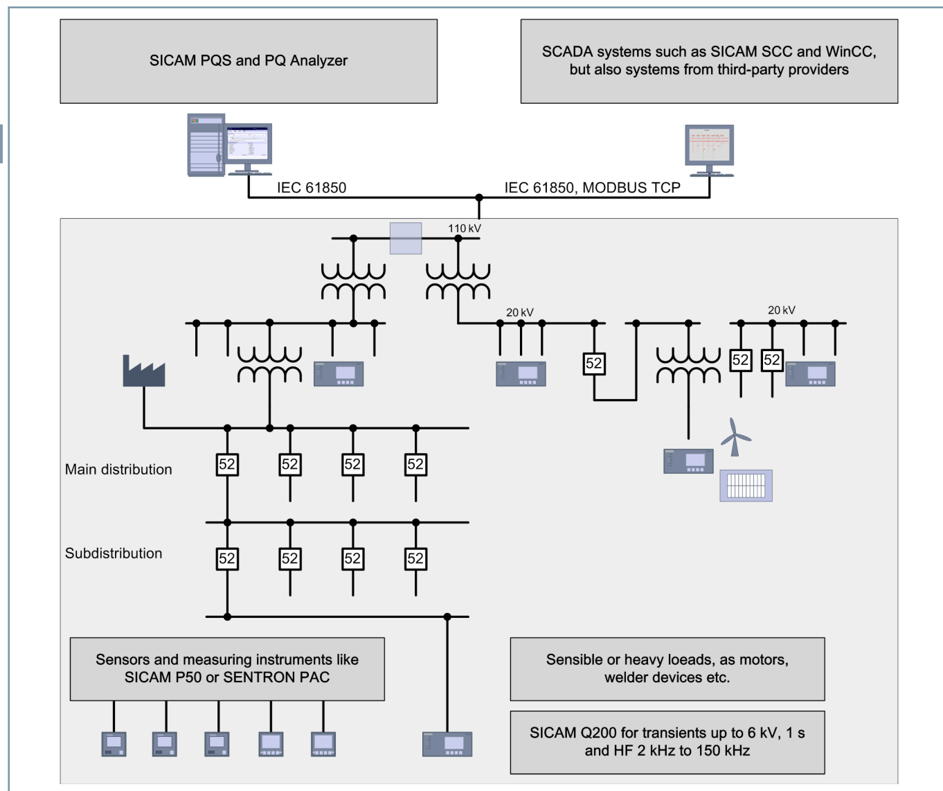
Figure 2.2/8 Power Distribution System Overview in Different Environments
