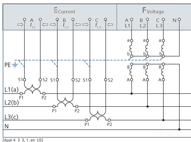
Figure 3.2/13 4-Wire Network, 3 Voltage and 3 Current Transformers, Any Load
