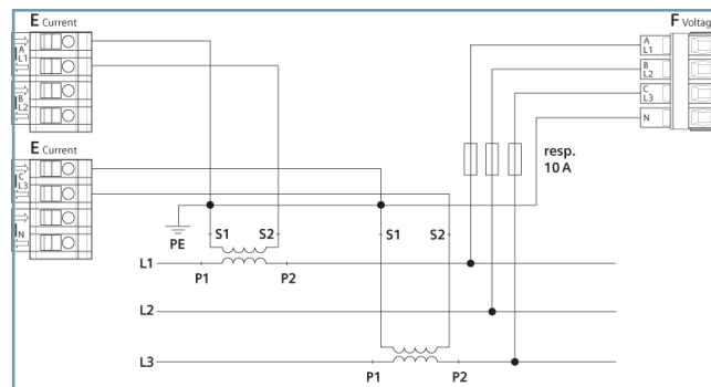
Figure 2.3/10 Connection Example 3-Wire Network, 2 Current Transformers, Any Load
