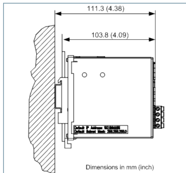
Figure 3.2/14 Dimensional Drawing of the SICAM MMU
