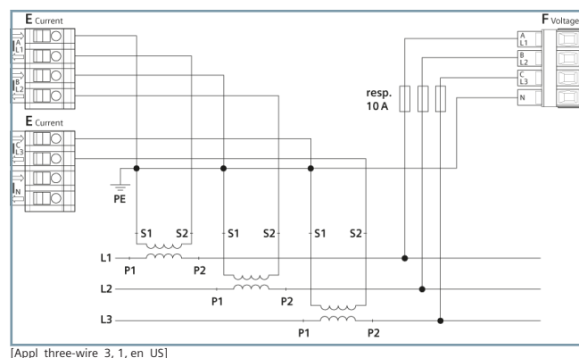
Figure 2.3/8 Connection Example 3-Wire Network, 3 Current Transformers, Any Load
