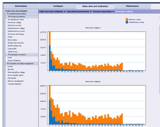
Figure 3.1/4 Graphical Representation of the Harmonics
