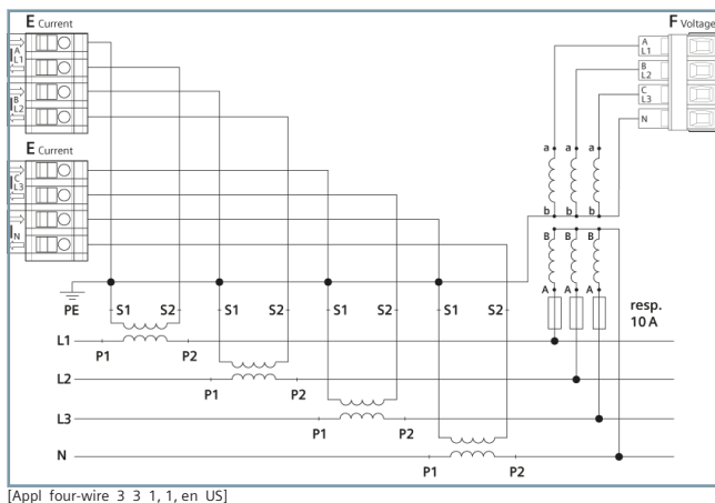
Figure 2.3/15 Connection Example 4-Wire Network, 3 Voltage Transformers and 3 Current Transformers, Any Load, 1 Current Transformer on the Neutral Phase
