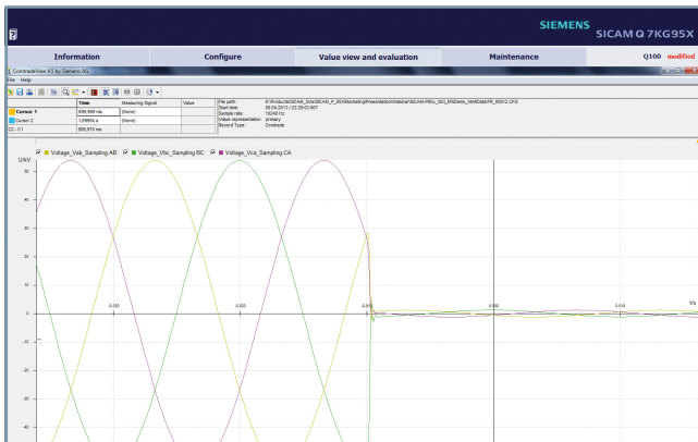
Figure 2.3/3 Sine Recording in COMTRADE View with COMTRADE Viewer Software and SIGRA Plug-In
