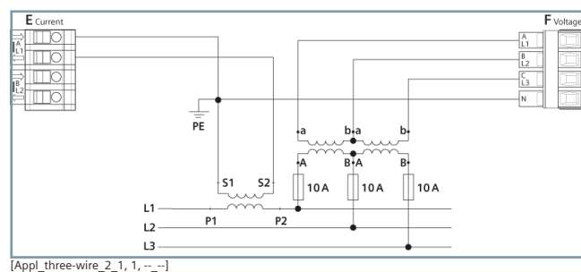
Figure 2.3/9 Connection Example 3-Wire Network, 2 Voltage Transformers and 1 Current Transformer, Same Load
