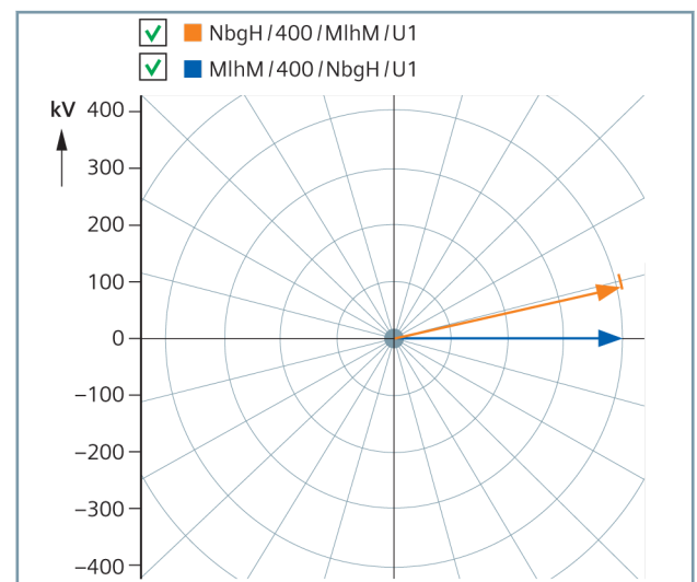
Figure 6.3/1 Voltage Phasors of 2 Measuring Points in the Power System
