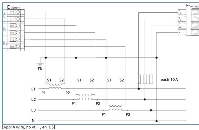
Figure 3.1/14 Connection Example 4-Wire Network, No Voltage Transformer and 3 Current Transformers, Any Load
