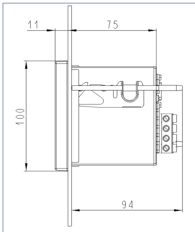
Figure 3.3/20 SICAM P 7KG7750, Variant IP 65
