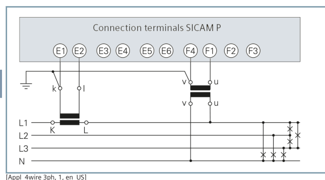
Figure 3.3/15 4 Conductors, 3 Phases, Uniform Load
