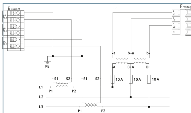
Figure 2.4/11 Connection Example 3-Wire Network, 2 Voltage and 2 Current Transformers, Any Load
