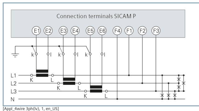
Figure 3.3/18 4 Conductors, 3 Phases (Low-Voltage System) 1,2
