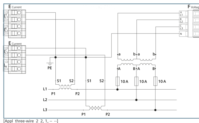
Figure 2.3/11 Connection Example 3-Wire Network, 2 Voltage Transformers and 2 Current Transformers, Any Load
