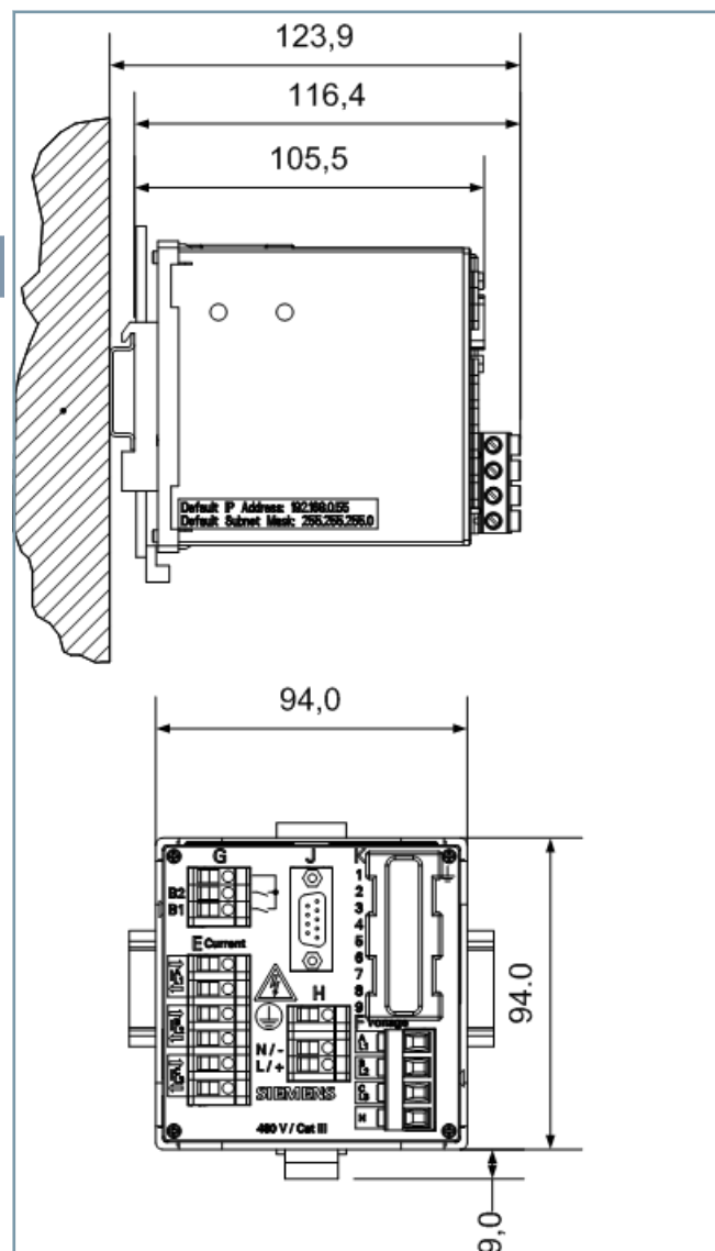
Figure 3.1/16 Dimensional Drawing of the SICAM P850/P855, DIN-Rail Device
