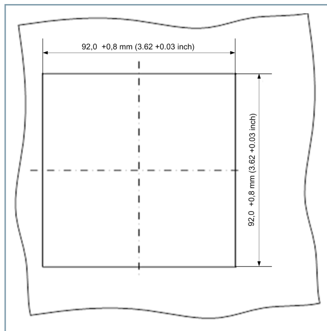
Figure 2.3/19 Cut-Out in Switch Panel
