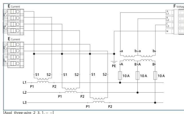
Figure 2.3/12 Connection Example 3-Wire Network, 2 Voltage Transformers and 3 Current Transformers, Any Load
