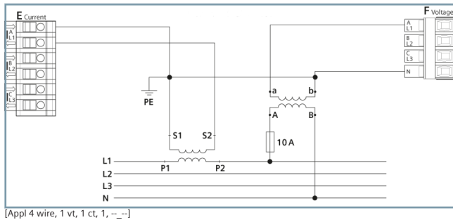
Figure 3.1/13 Connection Example 3-Wire Network, 1 Voltage and 1 Current Transformer, Any Load
