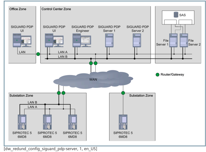
Figure 6.3/14 Redundant Configuration of the SIGUARD PDP Servers
