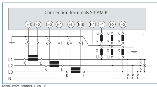
Figure 3.3/19 4 Conductors, 3 Phases (High-Voltage System)
