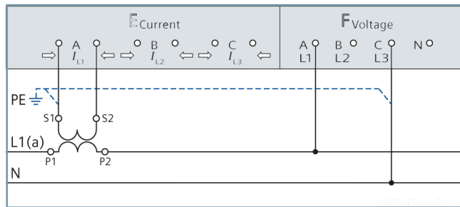
Figure 4.1/9 1-Phase System
