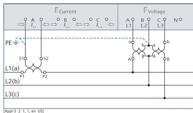
Figure 3.2/9 3-Wire Network, 2 Voltage and 1 Current Transformers, Same Load*
