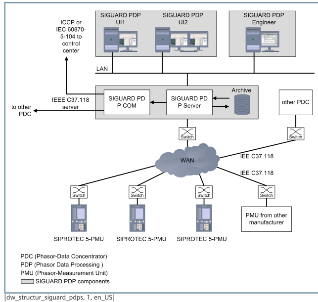
Figure 6.3/13 Structure of the SIGUARD Phasor Data Processing System
