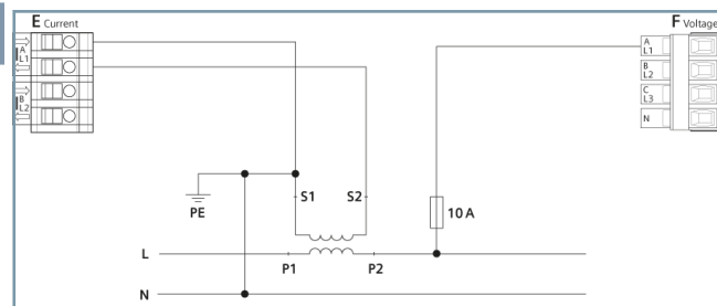
Figure 2.3/7 Connection Example 1-Phase System, 1 Current Transformer
