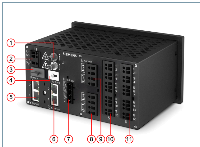
Figure 2.2/15 Layout of SICAM Q200 – Rear Side
