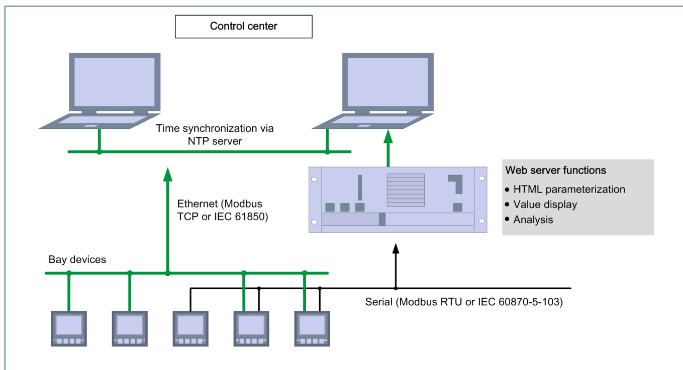
Figure 3.1/2 Application Example
