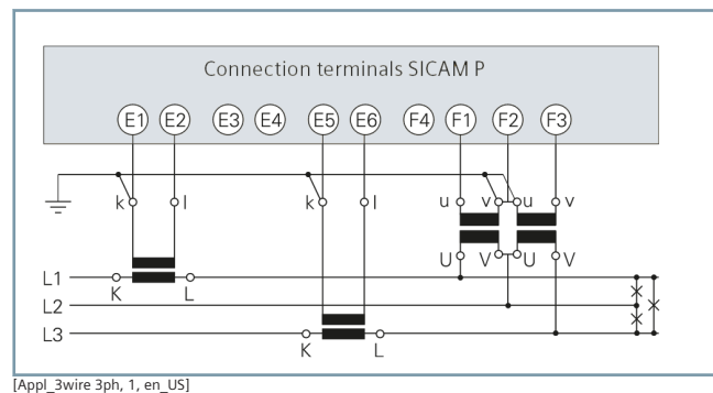
Figure 3.3/17 3 Conductors, 3 Phases
