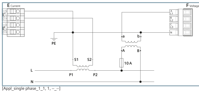
Figure 2.3/14 Connection Example 1-Phase System, 1 Voltage Transformer and 1 Current Transformer, Same Load
