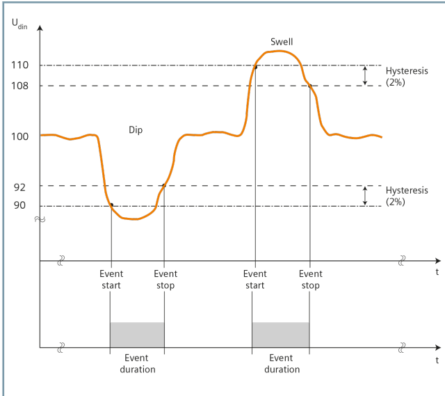
Figure 2.3/2 Recording of the Event Recorder: Overvoltage and Under-voltage
