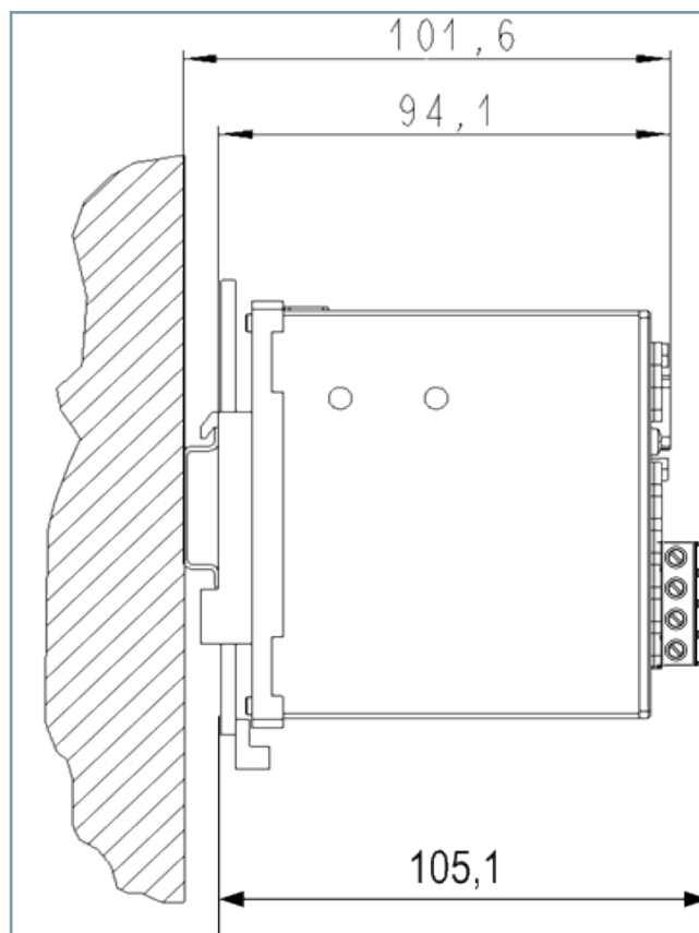
Figure 3.3/22 Sicam P 7KG7755 for DIN-Rail Installation
