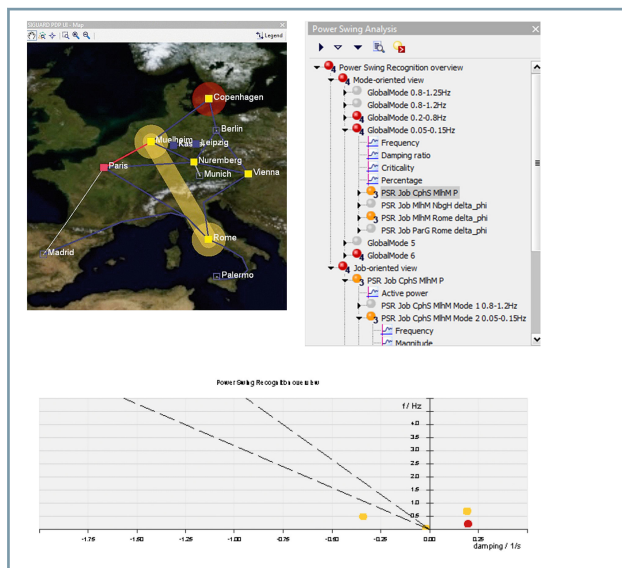
Figure 6.3/2 Overview Diagram of the "Power-Swing Recognition" Application
