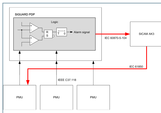
Figure 6.3/10 Closing the Control Loop via IEC 60870-5-104 and RTU
