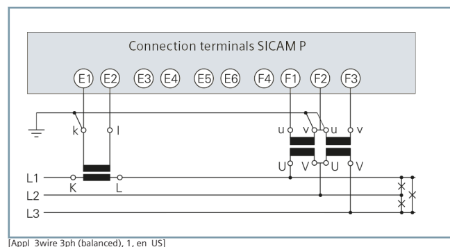
Figure 3.3/16 3 Conductors, 3 Phases, Uniform Load
