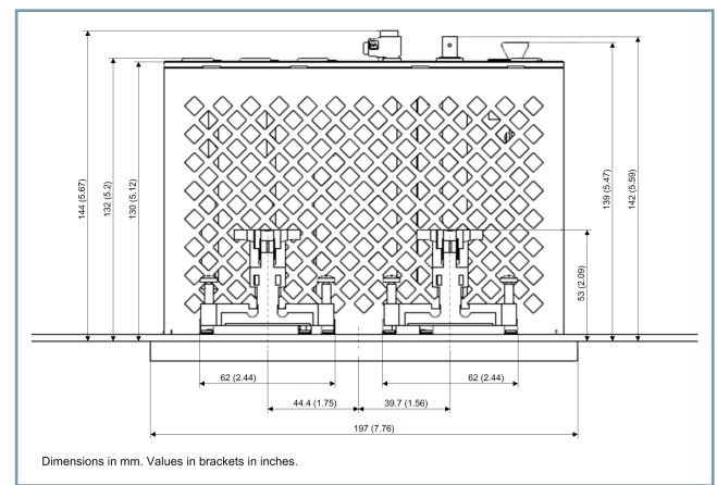
Figure 2.2/17 Top View SICAM Q200, Variant 1
