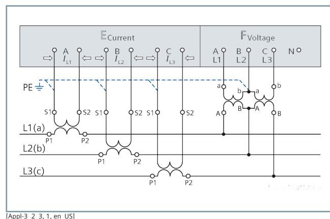
Figure 3.2/10 3-Wire Network, 2 Voltage and 3 Current Transformers, Any Load*
