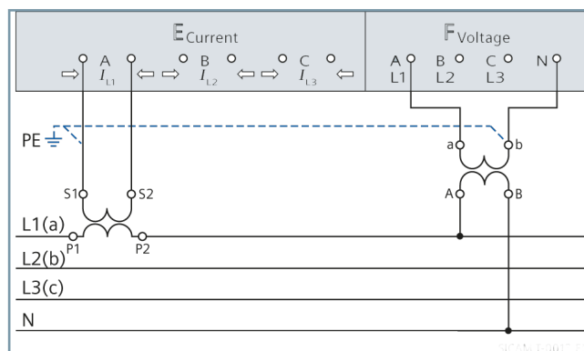
Figure 3.2/11 4-Wire Network, 1 Voltage and 1 Current Transformer, Same Load
