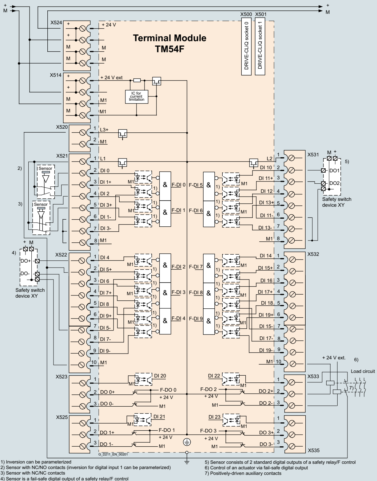
Connection example of TM54F Terminal Module
