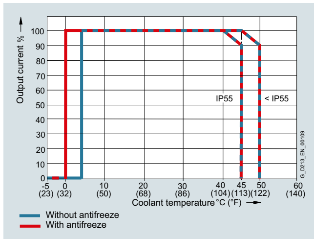
Current derating as a function of the temperature of the cooling liquid in the converter-side deionized water circuit 1)
