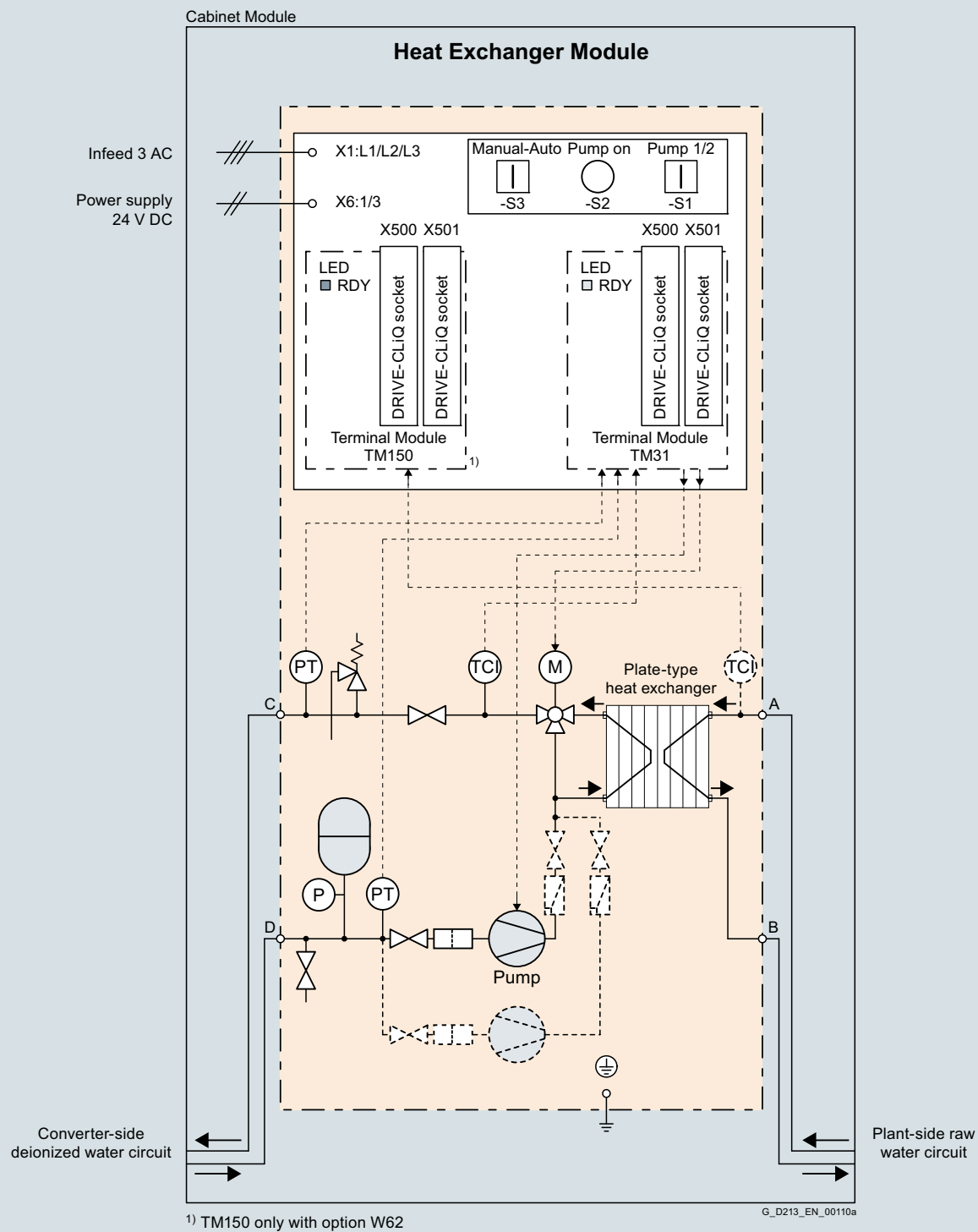
Connection example: Heat Exchanger Module, liquid-cooled
