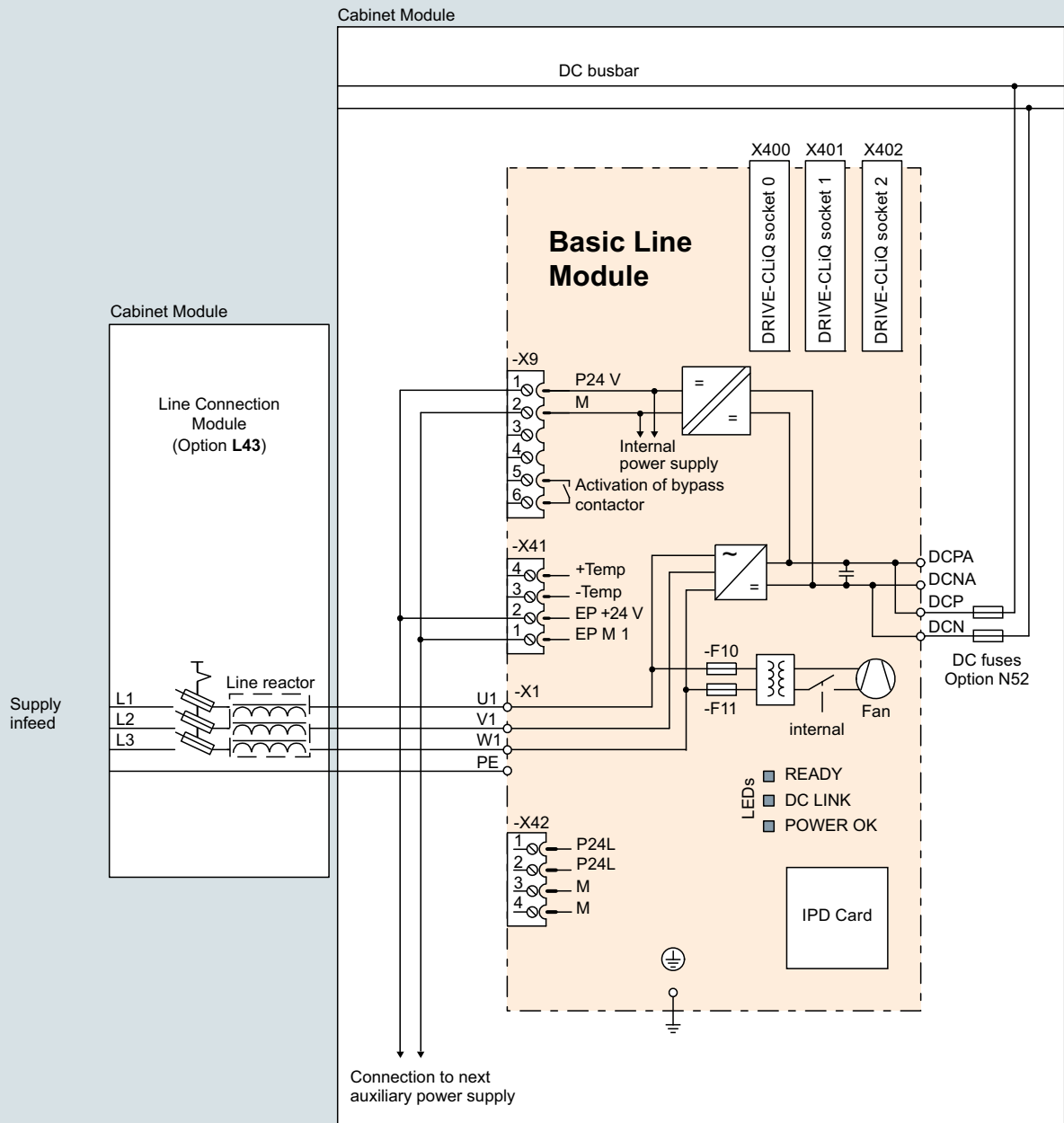
Connection example: Basic Line Module
