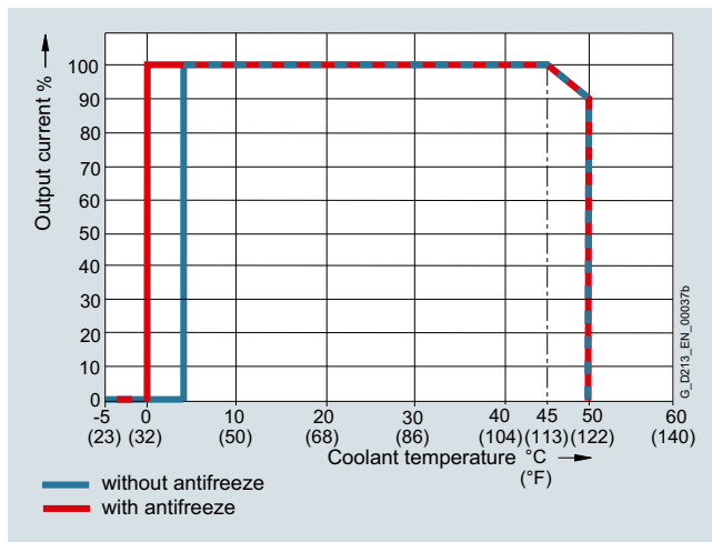
Current derating as a function of the temperature of the cooling liquid 1) (stainless steel heat exchanger)
