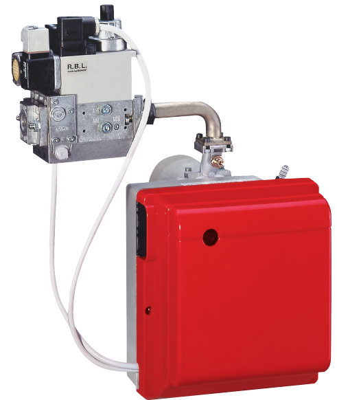
Gas train installed on the burner
