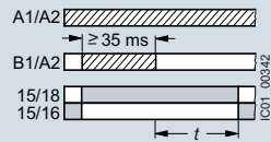
B OFF-delay with control signal
