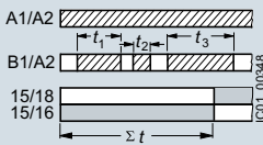
I Additive ON-delay, with control signal
