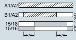
C ON-delay/OFF-delay with control signal
