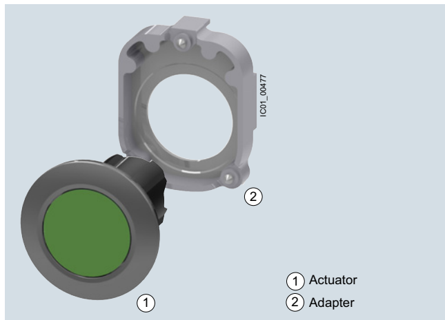
Actuators and indicators, flat, 30 mm, metal, matte, including adapter (adapter included in the scope of supply)
