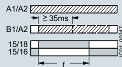
G Passing make contact with control signal, not retriggerable (pulse-forming with control signal)
