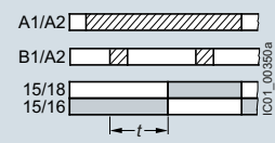
L Pulse-delayed with control signal (fixed pulse (at 1 s) and settable pulse delay)
