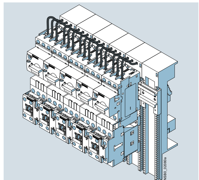
SIRIUS load feeders with busbar adapters snapped onto busbars
