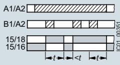
M Retriggerable interval relay with activated control signal (watchdog)
