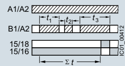
H Additive ON-delay, instantaneous OFF with control signal
