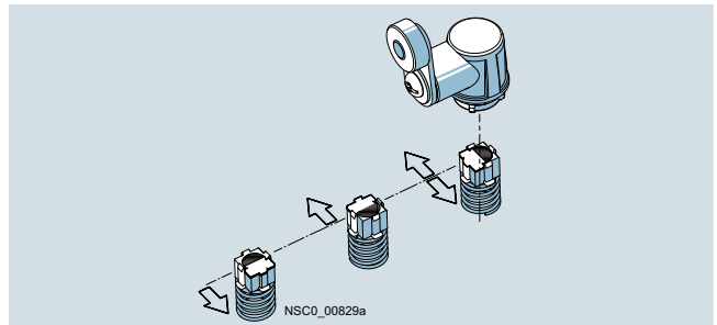
Twist actuators for twist levers and rod levers, with setting of switching direction to right, left, or right/left (standard for all twist lever actuators except fork levers)
