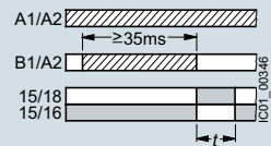
F Retriggerable interval relay with deactivated control signal (passing break contact with control signal)
