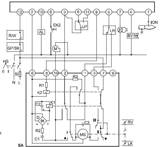
SQL90.220xx / 2-stage modulating control
