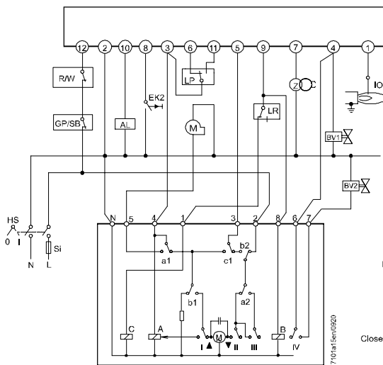
SQL7x.454xx / 2-stage control 1-wire control
