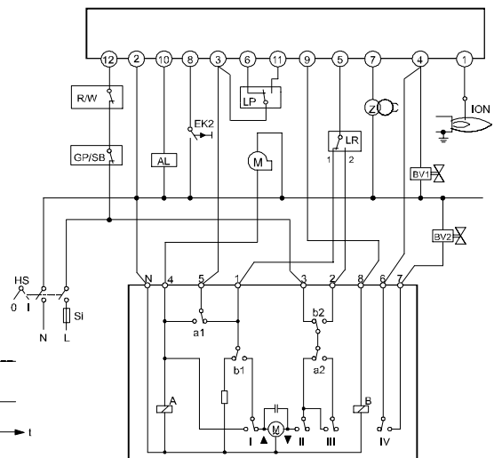
SQL7x.424xx / 2-stage control 2-wire control
