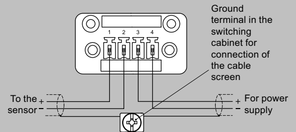
SITRANS RD150 connections
