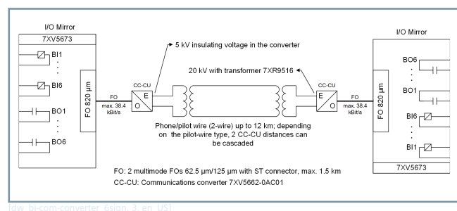
Figure 8.1/8 Binary Signal Exchange of 6 Signals via a Pilot Wire Connection
