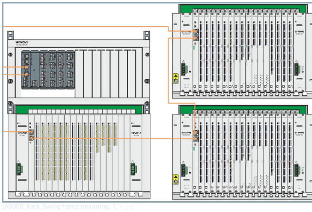
Figure 2.3/2 SICAM A8000 Rack – Swing-Frame Mounting
