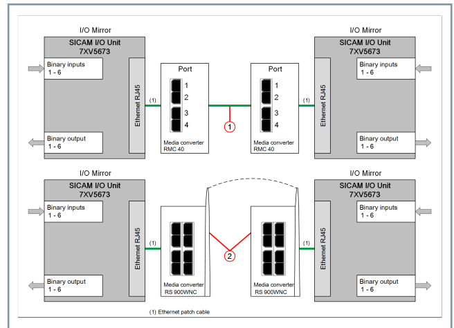
Figure 8.1/12 Binary Signal Transmission via Optical Fiber or Wireless Connection; Connection via the Integrated Ethernet Interface to External Transmission Devices
