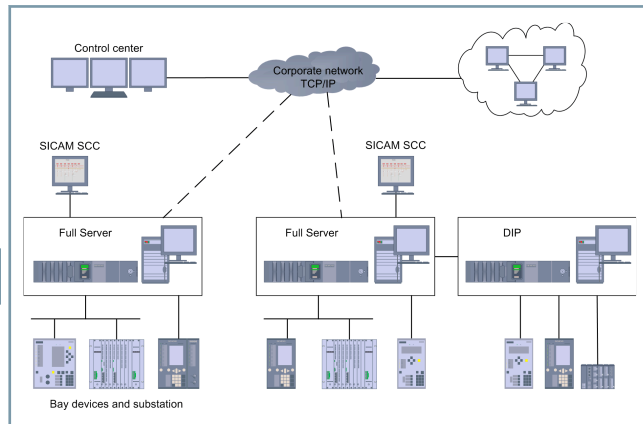
Figure 2.1/2 Sample Configuration with 2 SICAM PAS Systems
