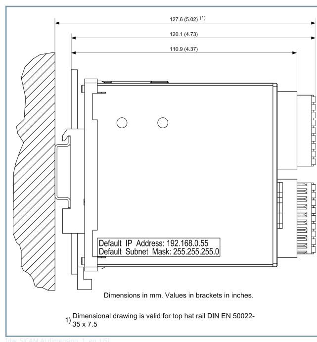
Figure 8.2/3 Dimensions of the SICAM AI-Unit 7XV5674
