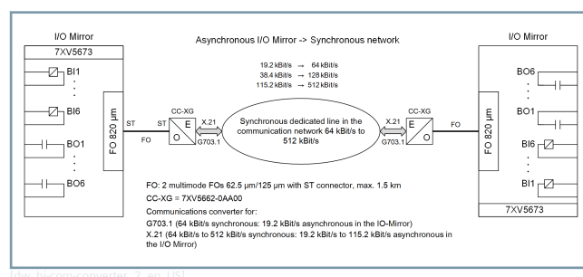
Figure 8.1/10 Binary Signal Exchange via a Communication Converter with a G.703.1-/X.21 Interface via a Communication Network
