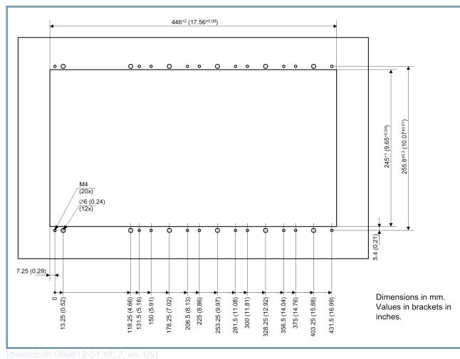
Figure 5.2/3 Cut-Out Widths and Drilling Pattern
