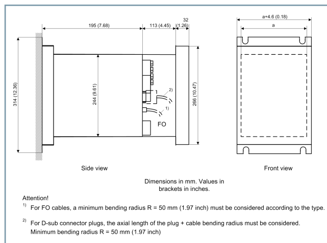
Figure 5.2/6 1/3 Surface Mounting Device with Integrated On-site Operation Panel; Dimensions in the Side and Front Views
