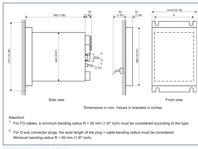
Figure 5.2/5 Surface Mounting Device with Detached On-site Operation Panel; Dimensions in the Side and Front Views
