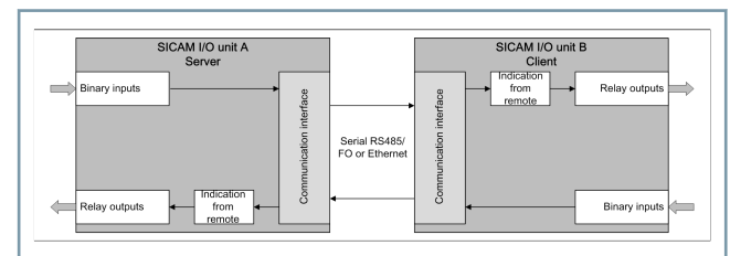
[diw_10-Mirror_Bidirect-trans-2-device, 1, en_US]
