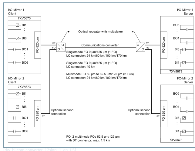
Figure 8.1/9 Binary Signal Exchange of Up to 12 Signals via Long Optical Fiber Connections
