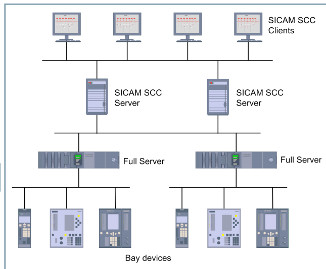
Figure 2.1/10 Redundant SICAM SCC with Redundant Full Server
