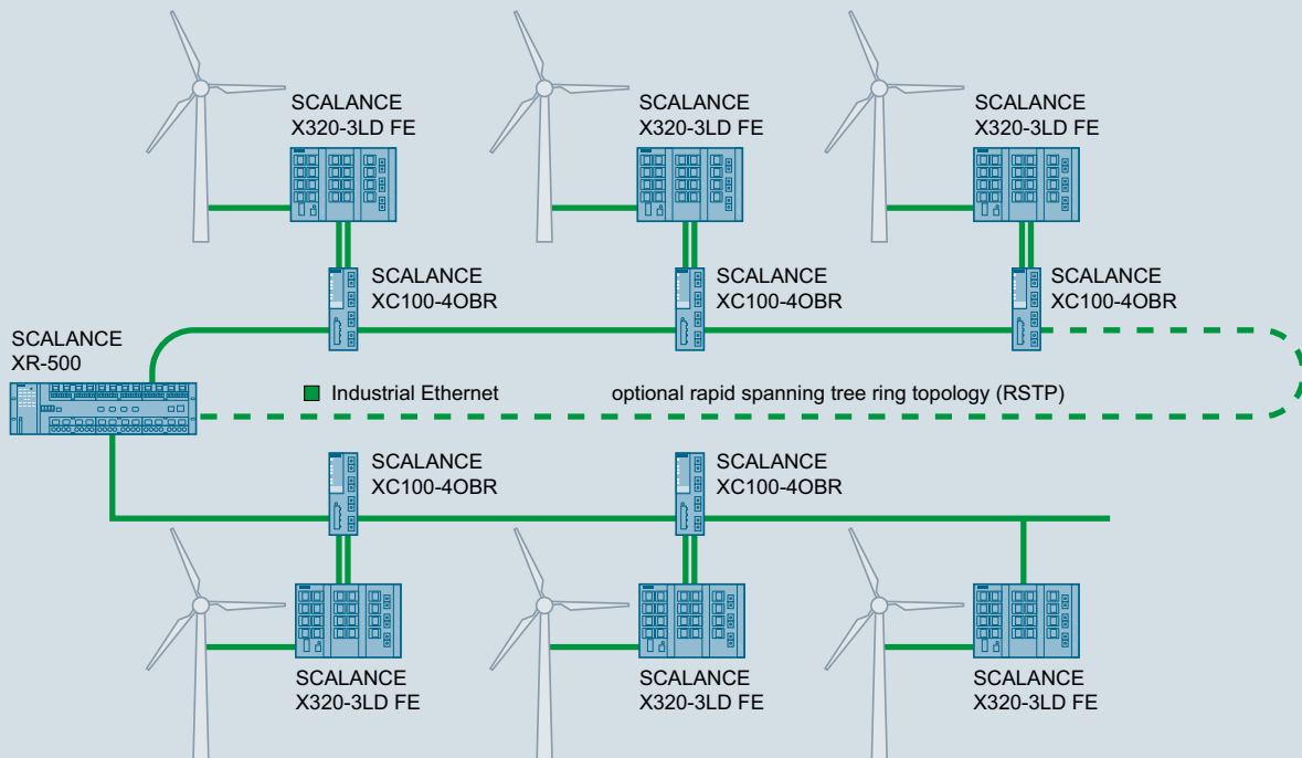
Redundant network with SCALANCE XC100-4OBR
