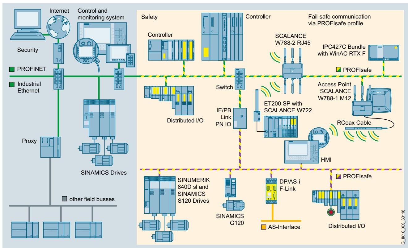
Fail-safe wireless communication with PROFIsafe
