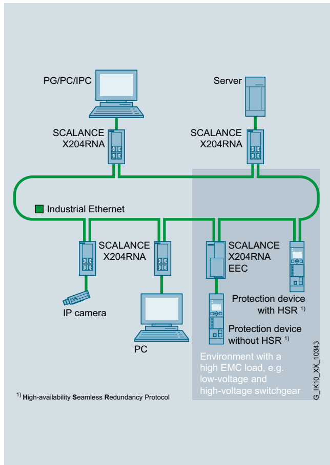
Ring-shaped HSR network structure with SCALANCE X-204RNA
