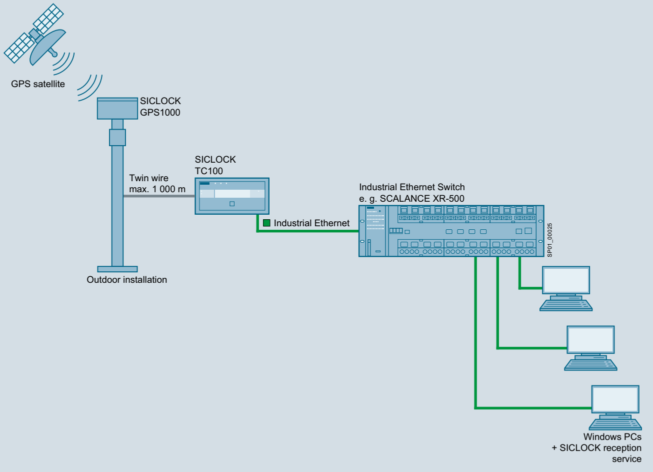
SICLOCK TC100 central plant clock with SICLOCK GPS1000 wireless receiver: Synchronization of IT systems (with failure protection)
