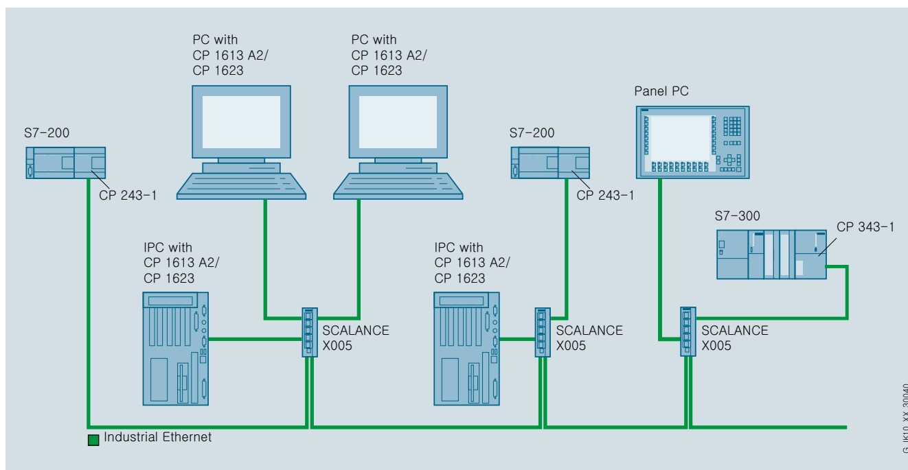
Electrical line topology with SCALANCE X005
