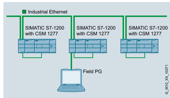
Linear topology with CSM 1277
