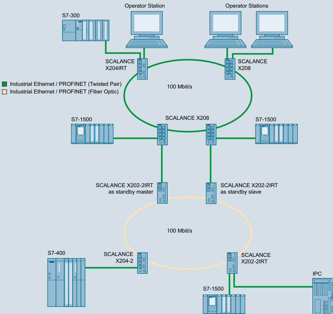
Redundant coupling of two subnetworks with SCALANCE X-200IRT
