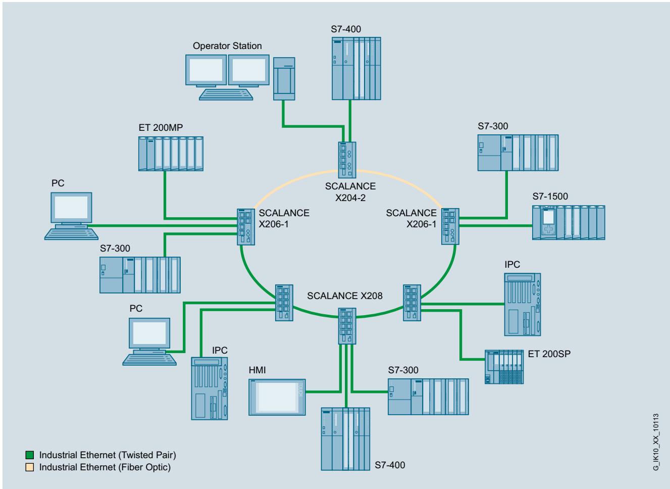
High-speed redundancy in mixed ring with fiber-optic and twisted-pair cables
