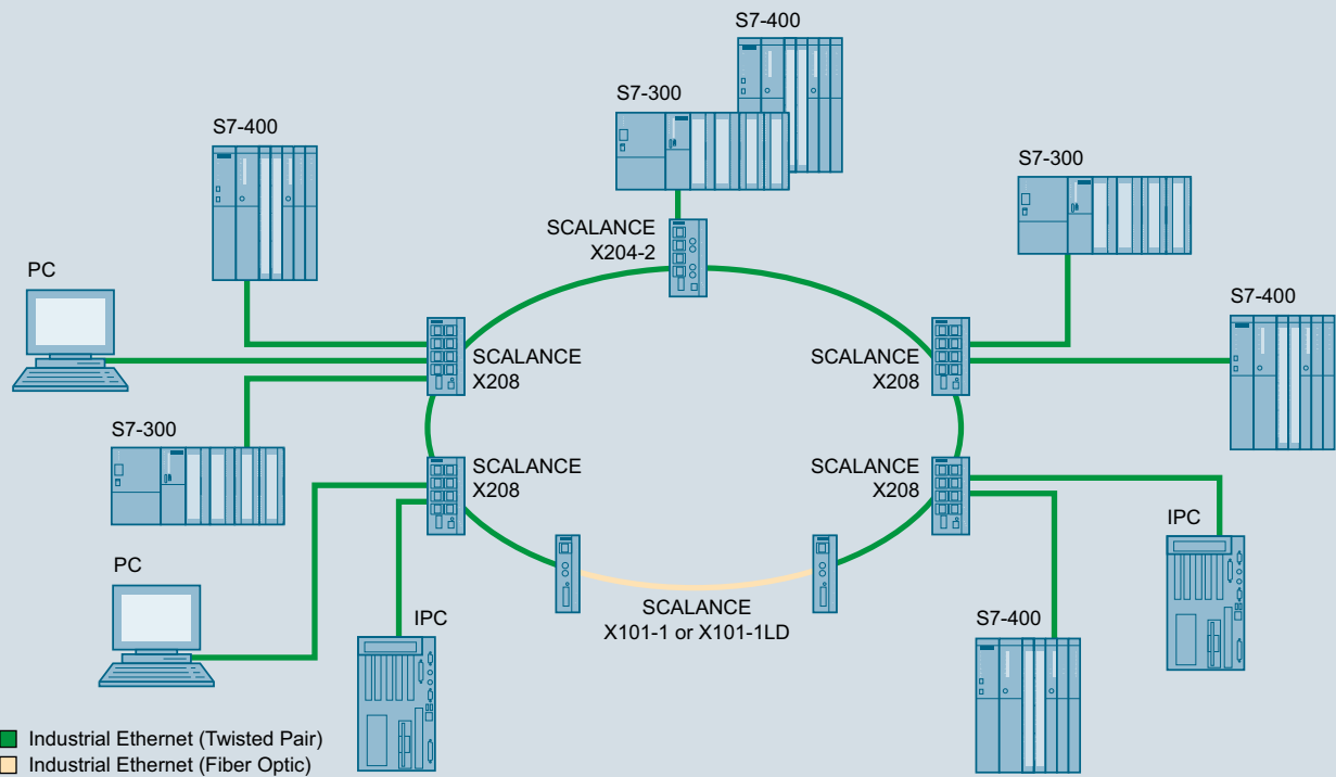
Electrical/optical ring topology with SCALANCE X101-1/X101-1LD
