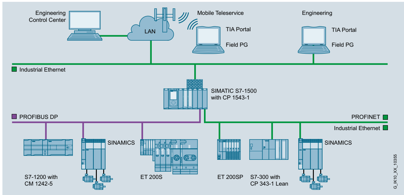
Connection to a higher-level network with network separation and access protection (firewall function)
