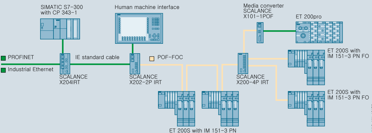
Mixed network topology with plastic fiber-optic cables and twisted-pair cables
