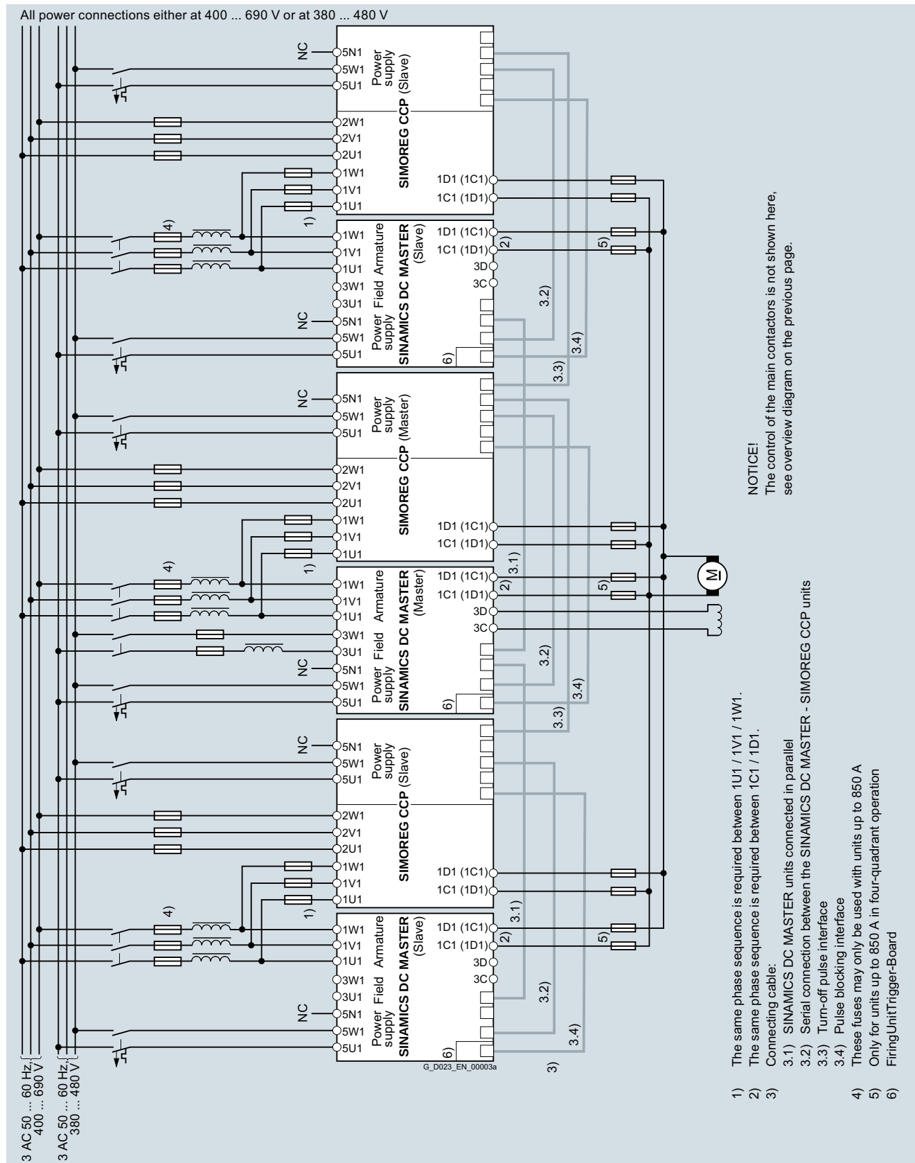
Block diagram for parallel connection
