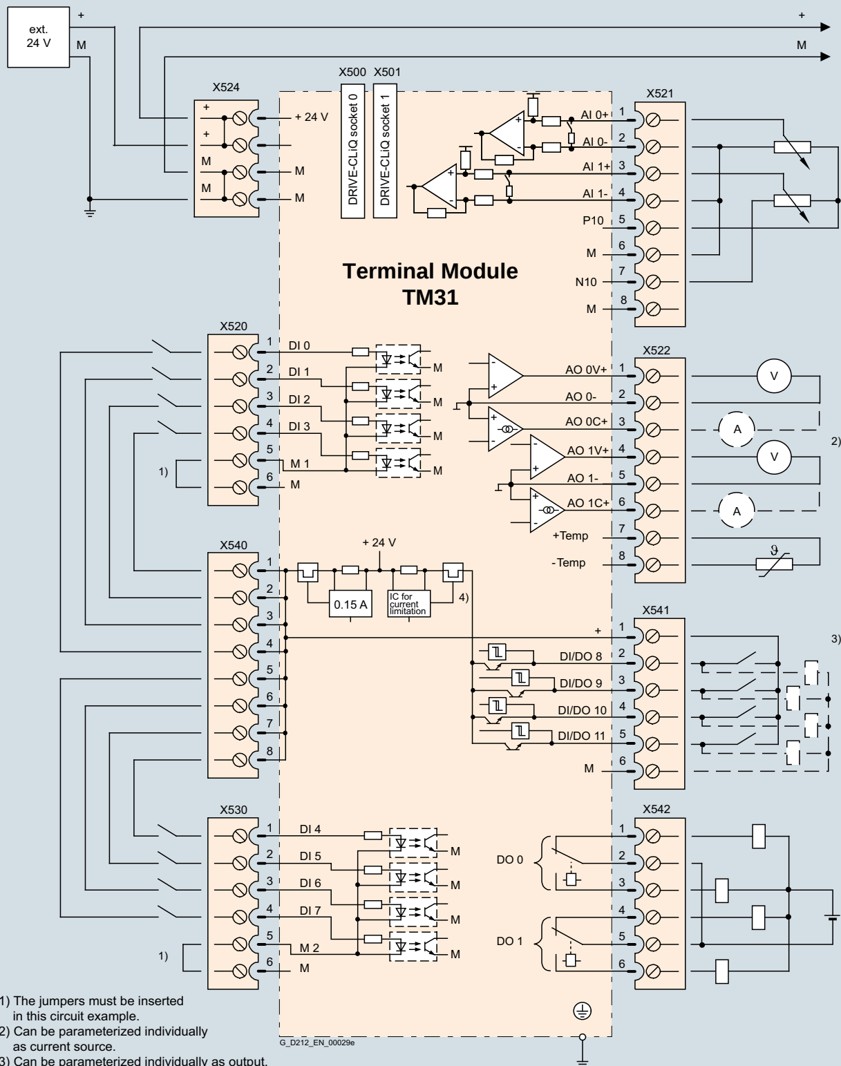
Connection example of a TM31 Terminal Module
