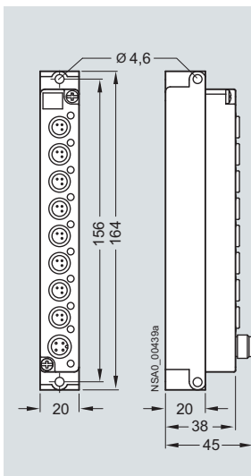
IO-Link K20 I/O module, 8 digital inputs, M8 (3RK5 010-0CA00-0AA0)
