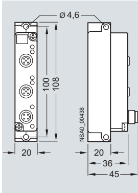
IO-Link K20 I/O module, 4 digital inputs, M12 (3RK5 010-0BA10-0AA0)
