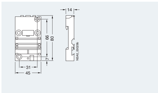
3RK1 901-2DA00 Mounting plate for standard rail mounting Arrangement and drilled holes identical to that of the user module
