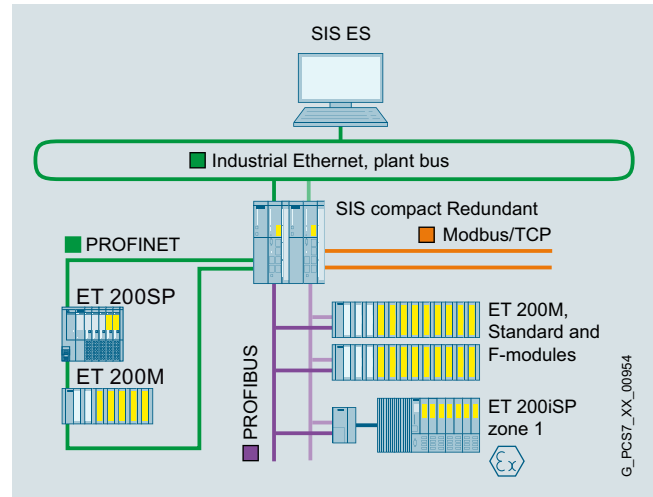
Configuration example: SIMATIC SIS compact Basic Package Redundancy
