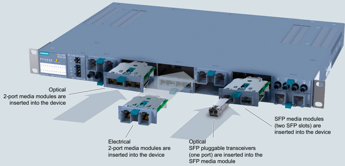
Insertion of 2-port media modules in media module slot
