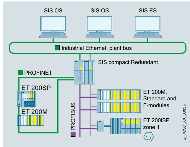
Configuration example: SIMATIC SIS compact Extended Package Redundancy
