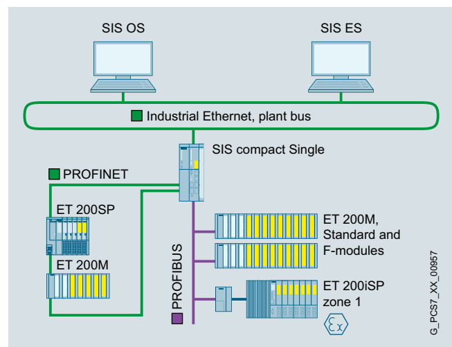
Configuration example: SIMATIC SIS compact Extended Package Single
