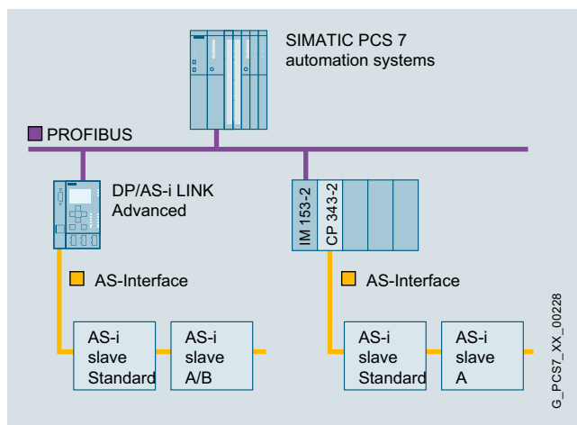
AS-i integration in SIMATIC PCS 7 via PROFIBUS DP
