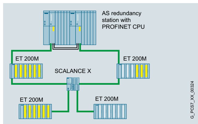
Safety-related PROFINET IO communication with system redundancy
