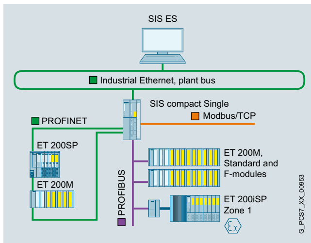
Configuration example: SIMATIC SIS compact Basic Package Single
