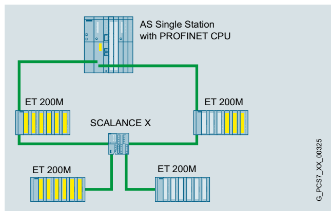
Safety-related PROFINET IO communication with media redundancy
