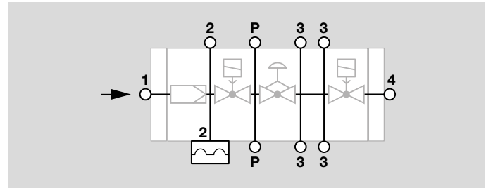
Pressure tap points for large body size models
