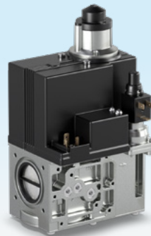
V1 is fast opening/closing, V2 is slow opening/fast closing
