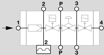
Pressure tap points for small body size models
