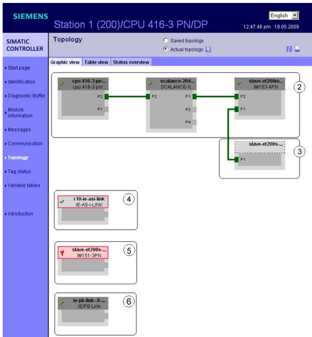
Figure 4-17 Topology - Graphical view
