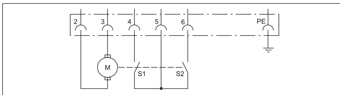
Figure 5-6 Circuit diagram
