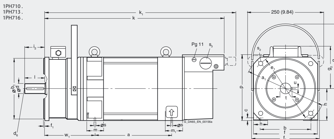
Figure 4-16 1PH7, type of construction IM B35, forced ventilation, with braking module
