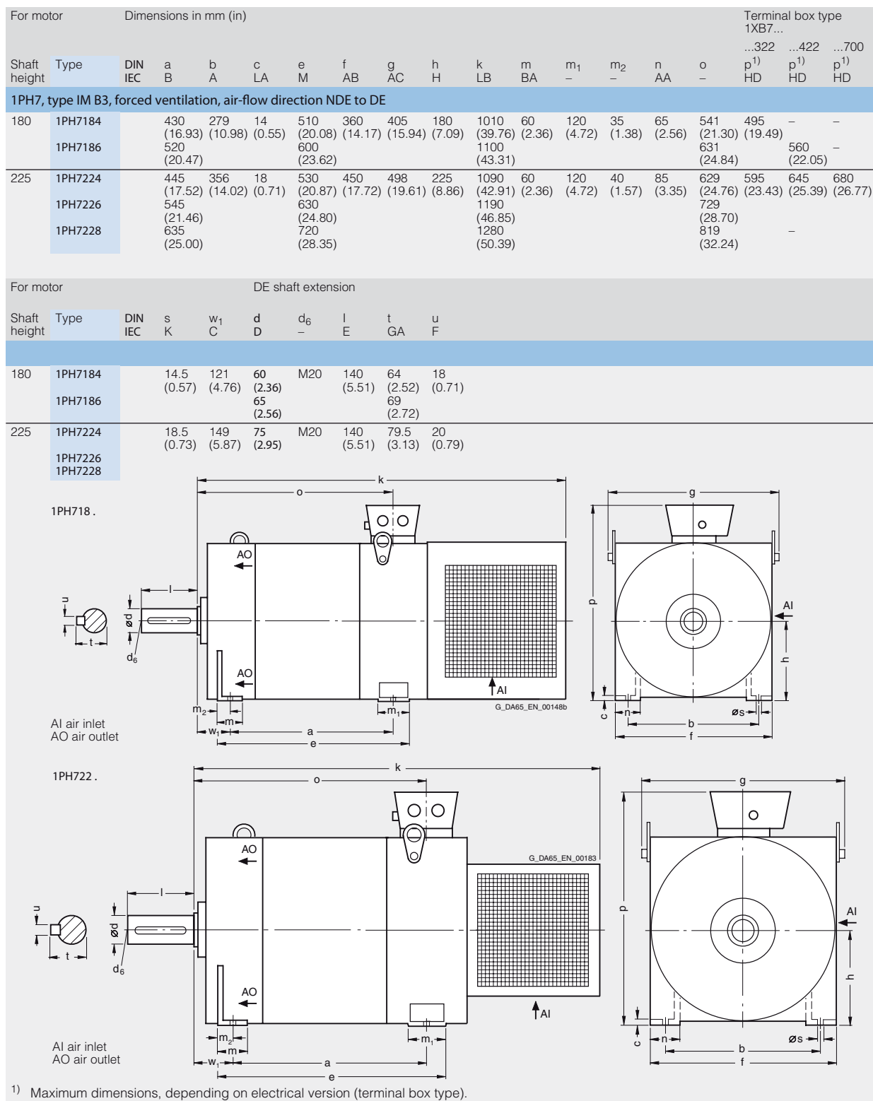
Figure 4-5 1PH7, type of construction IM B3, forced ventilation, direction of air flow DE-NDE
