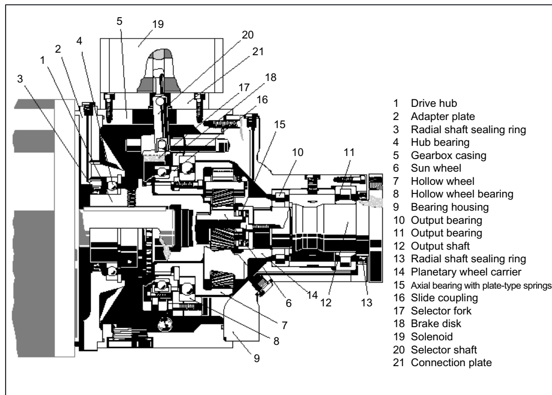
Figure 5-4 Gearbox design for 1PH7, SH 100 to 160
