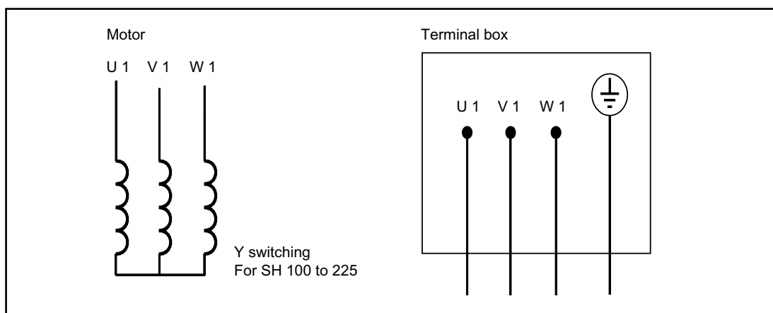
Figure 6-3 Circuit diagram
