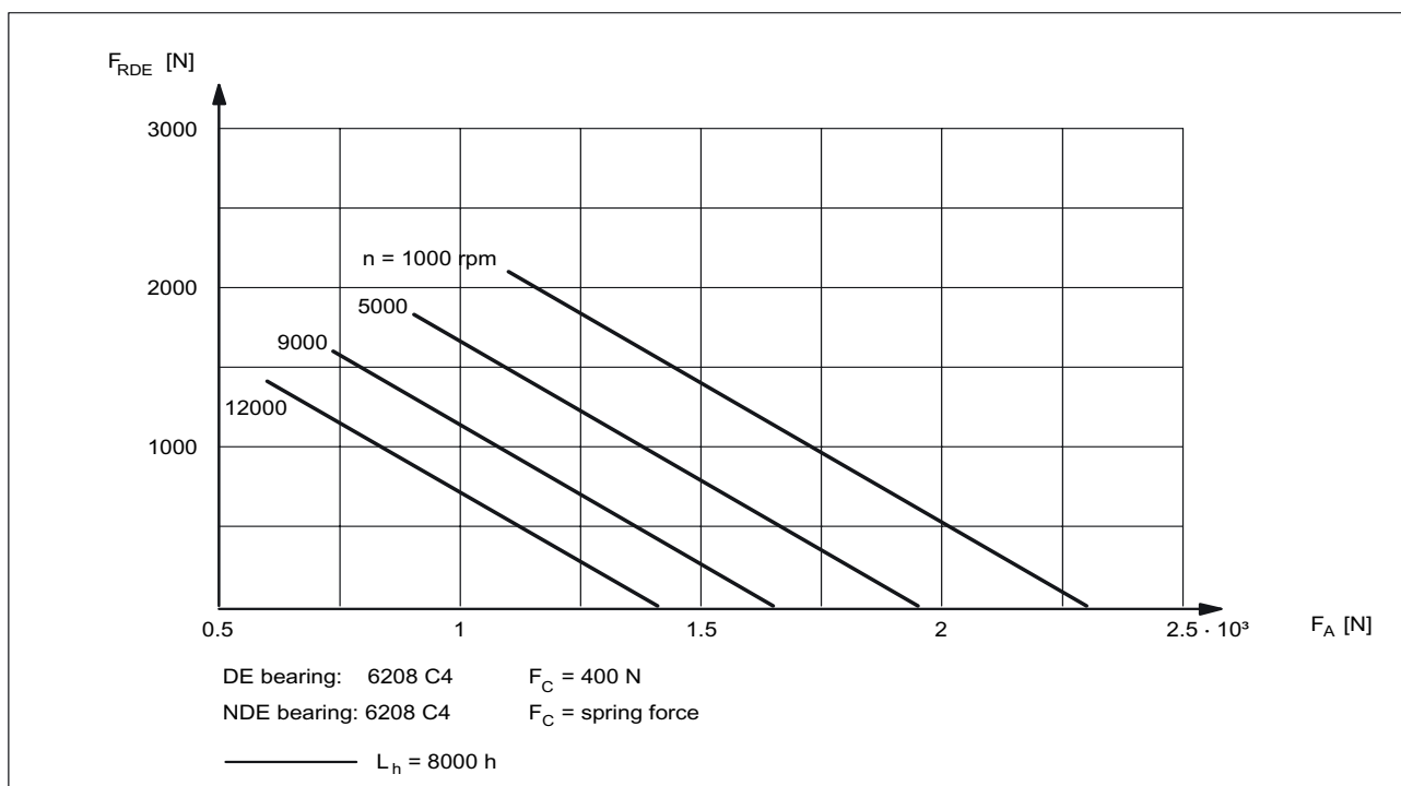
Figure 3-16 Cantilever force diagram, SH 100 (increased max. speed)
