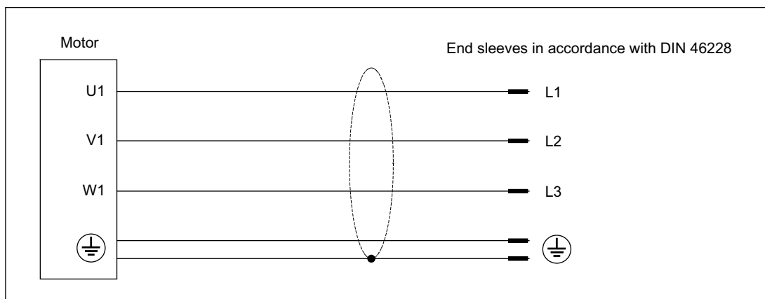
Figure 6-2 Power cable
