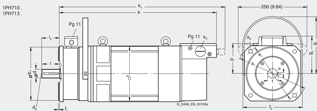
Figure 4-11 1PH7, type of construction IM B5, forced ventilation, with braking module
