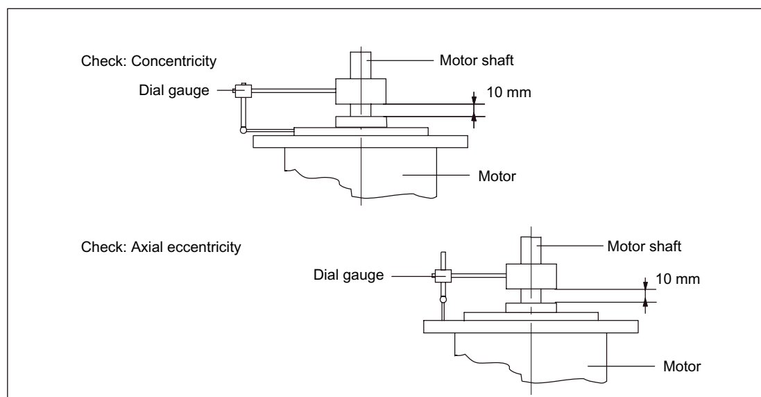
Figure 3-20 Checking the concentricity and axial eccentricity
