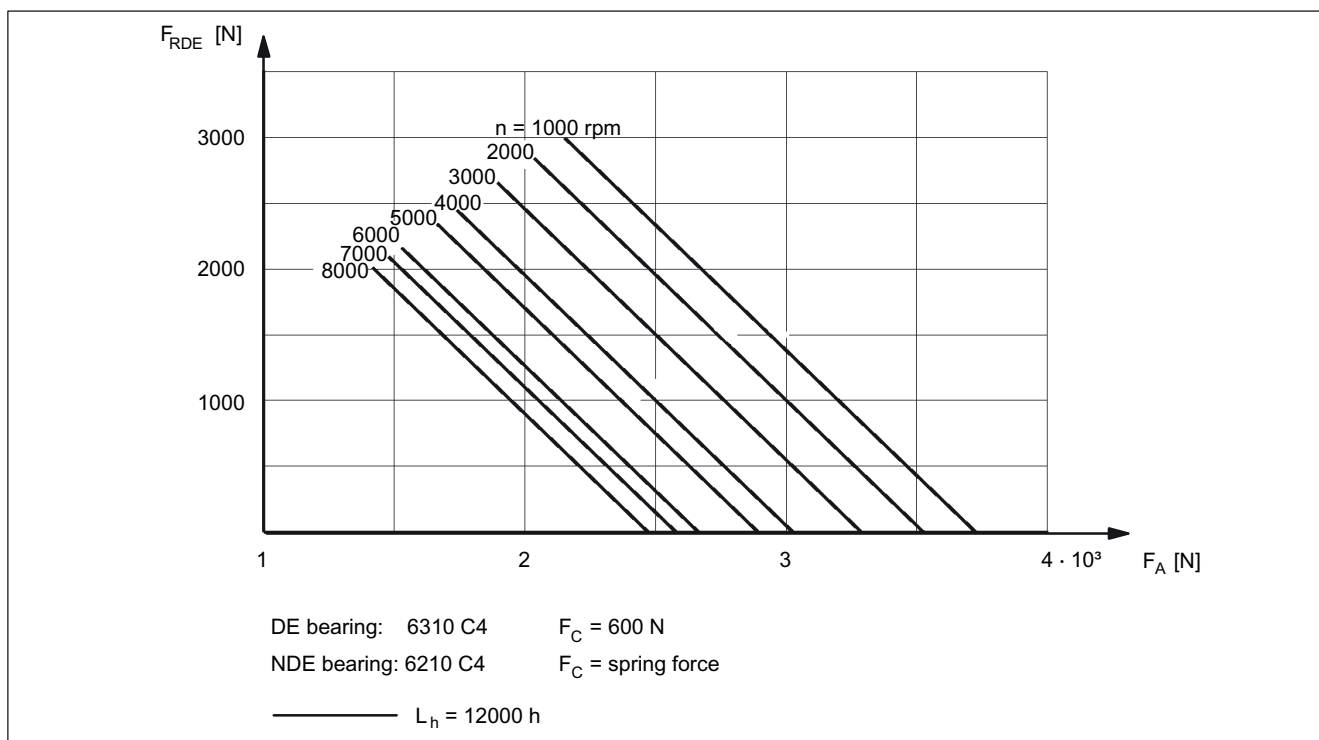
Figure 3-14 Axial force diagram, SH 132
