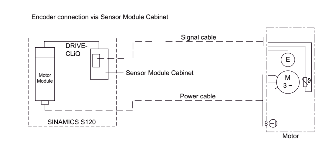
Figure 6-7 Encoder connection for motors without DRIVE-CLiQ
