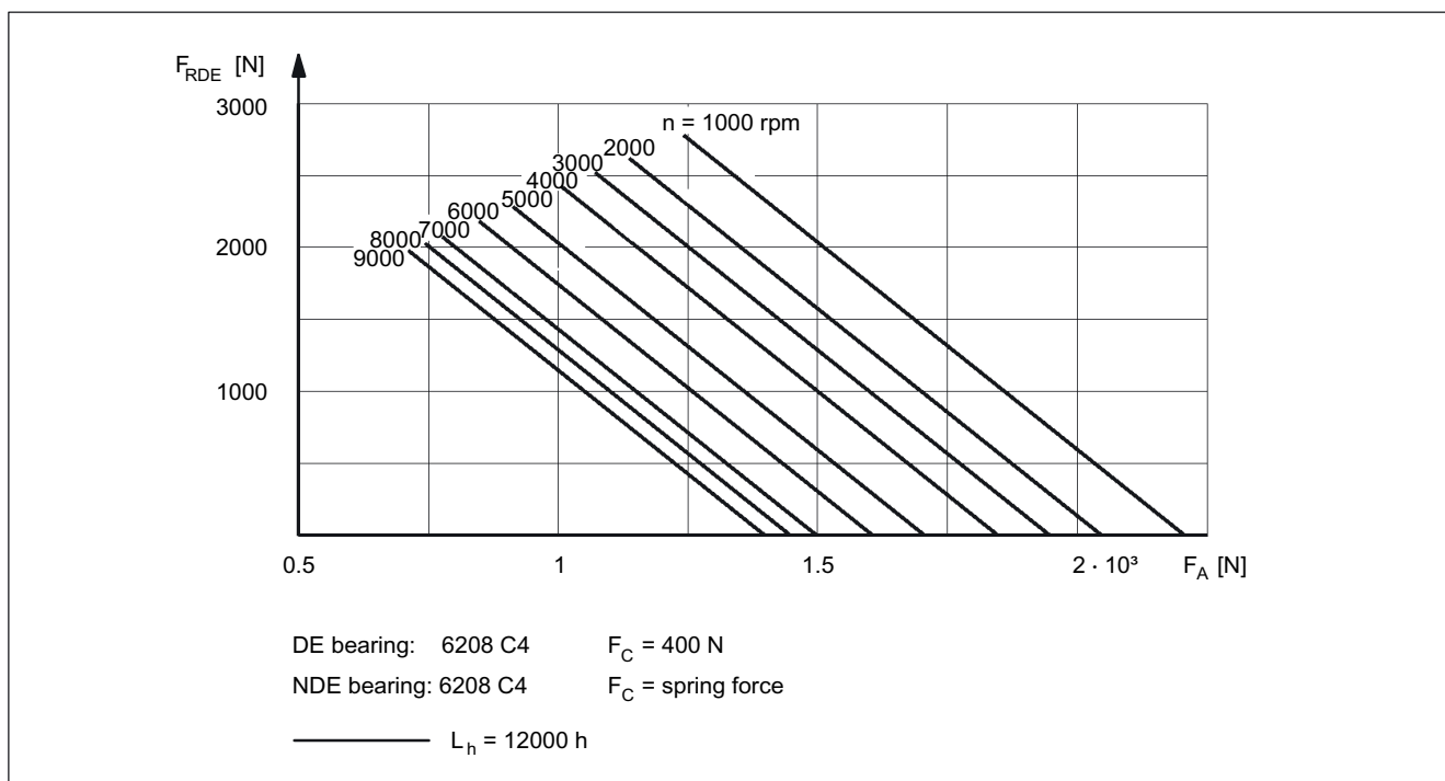
Figure 3-13 Axial force diagram, SH 100
