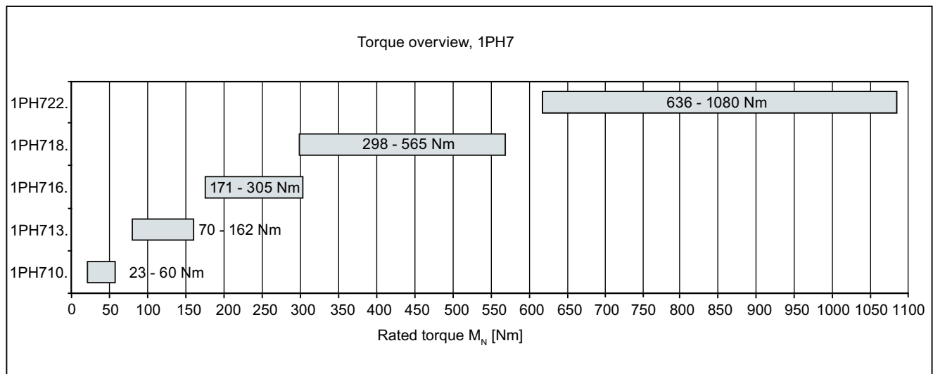
Figure 1-1 Torque overview
