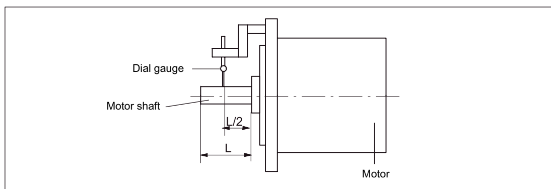
Figure 3-19 Checking the radial eccentricity
