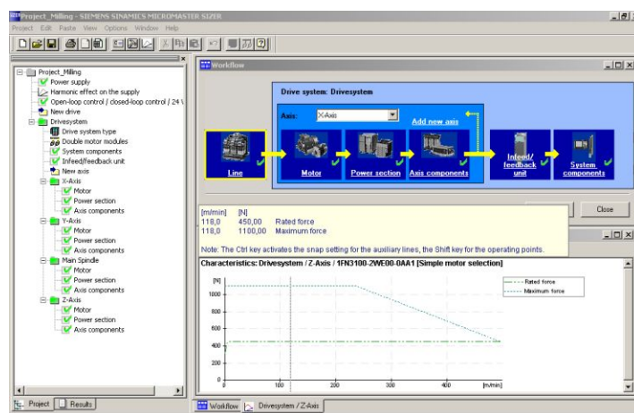
Figure 2-1 SIZER
