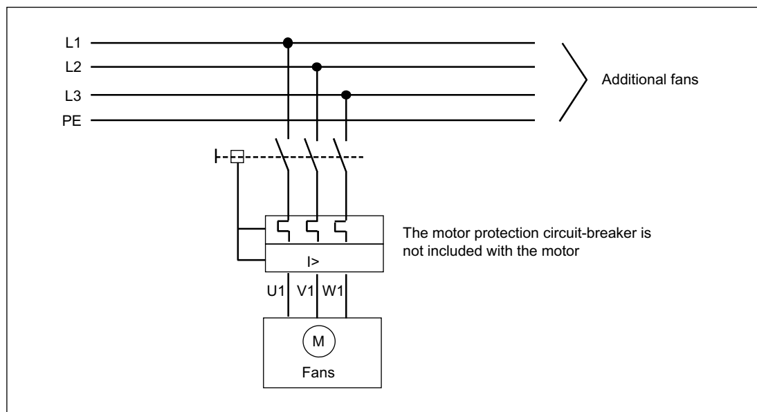
Figure 6-5 Recommended connection
