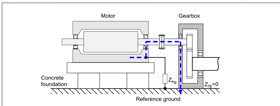
Figure 7-3 Bearing current due to the grounding situation (= rotor ground current)
