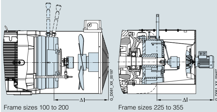
Fig. 7 Brake, rotary pulse encoder (under cover) and separately driven fan, order codes F01/F04 + F70 + G04/G05/G06/G11/G12 [optionally with manual release, order code F50 ]
