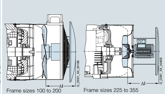
Fig. 8 Protective cover for separately driven fan, order code H00
