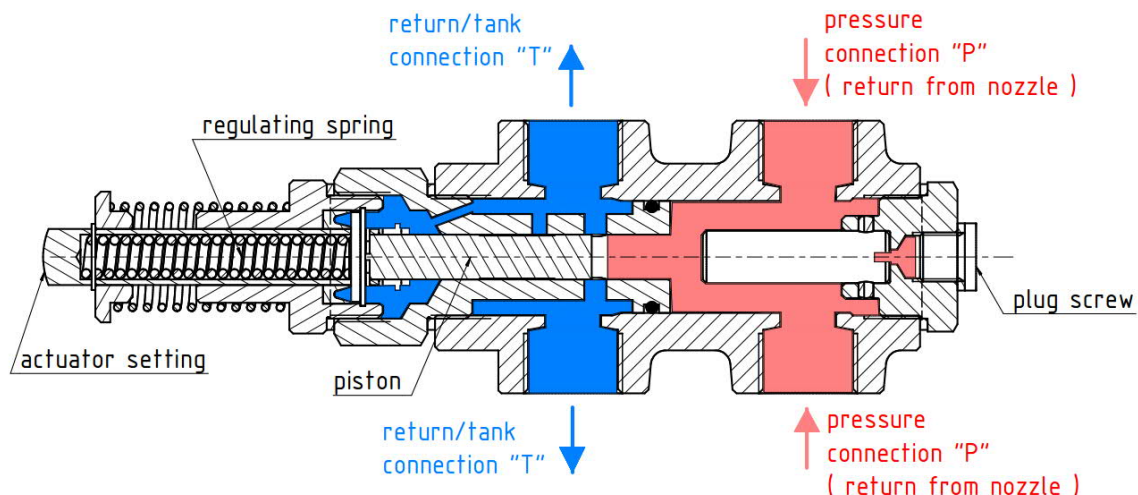
Fig.1 Operating principle
