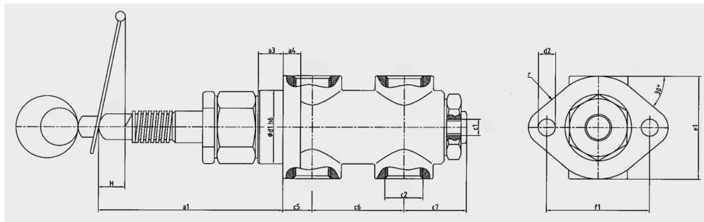
Fig.2 Dimensions
