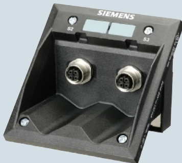
Control cabinet bushing with two M12 sockets
