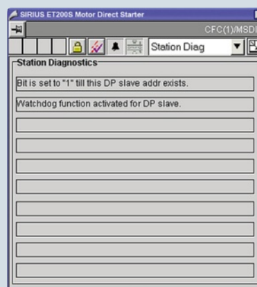
Faceplate for diagnostics
