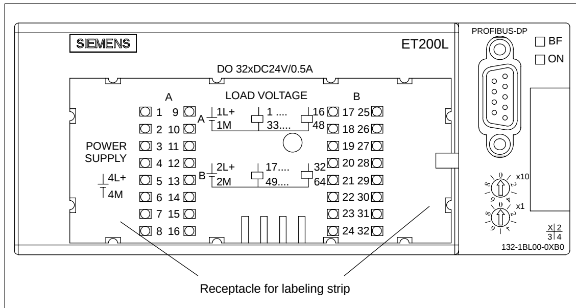
Figure 8-7 View of the L 32 DO Electronics Block DC 24 V/0.5 A
