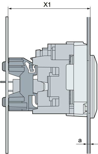
30.5 mm devices with modules, PCB assembly
