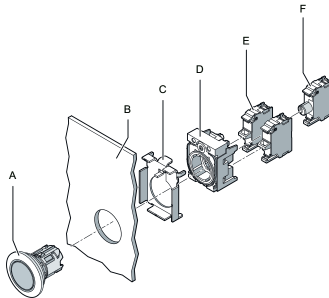
Mounting with actuator 30.5 mm
