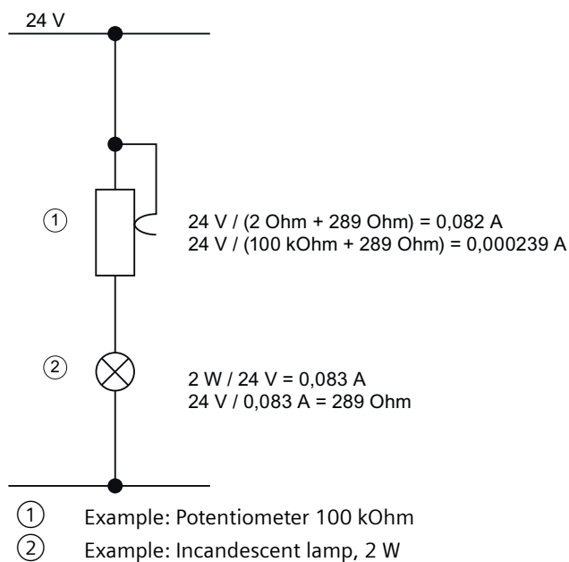
Connection diagram for potentiometer
