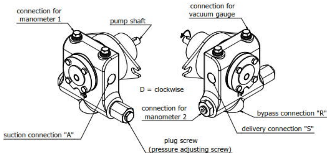
Fig. 2. Direction of rotation – clockwise “D”
