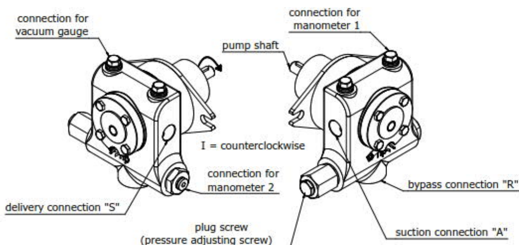
Fig. 1. Direction of rotation – counterclockwise "I"
