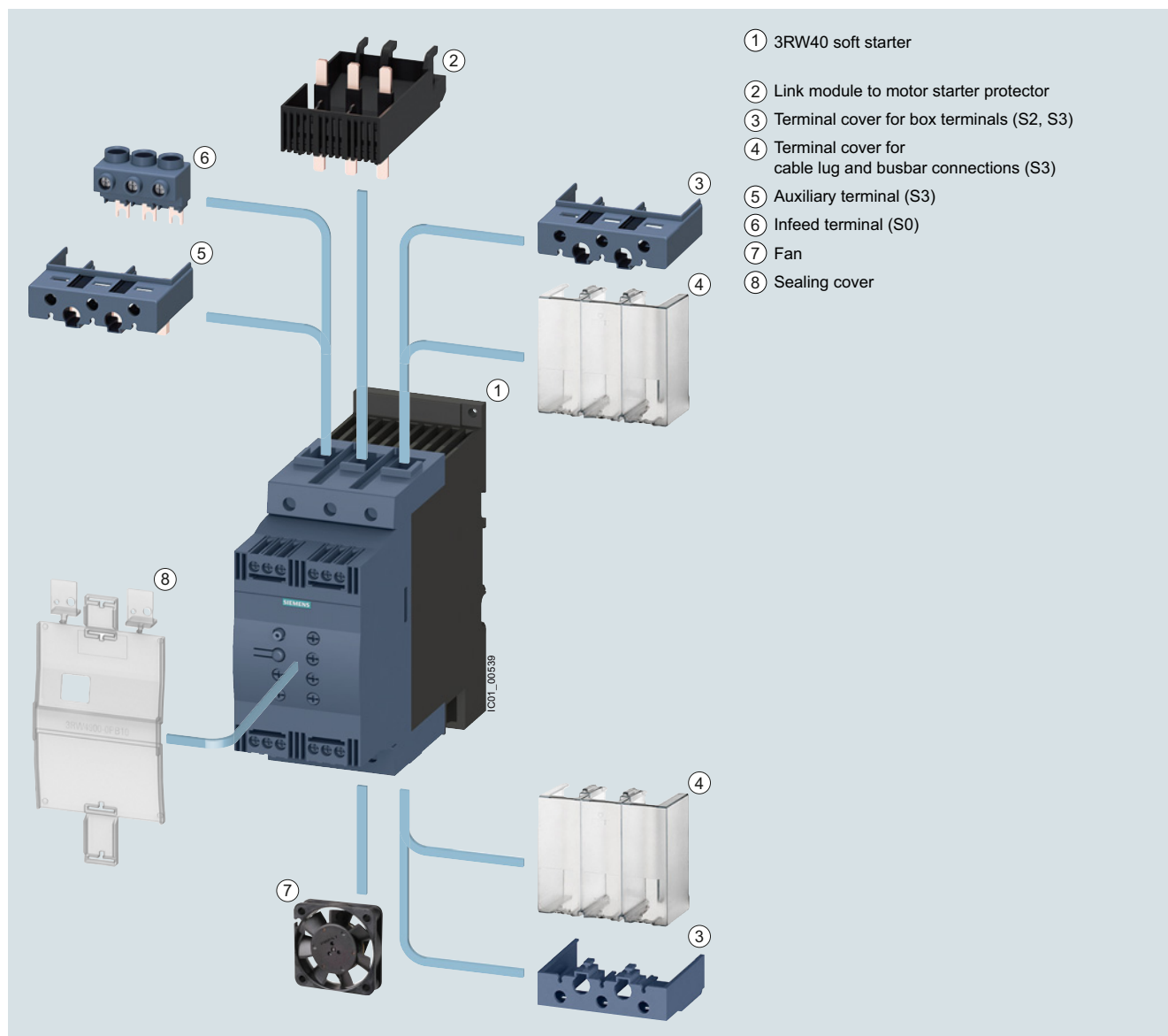
SIRIUS 3RW40 Basic Performance soft starter with accessories (see page 6/94)
