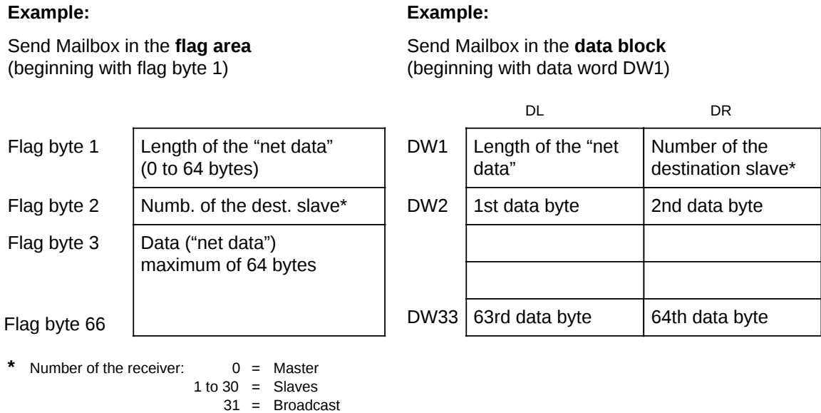
Figure 13-4. Structure of the Send Mailbox
