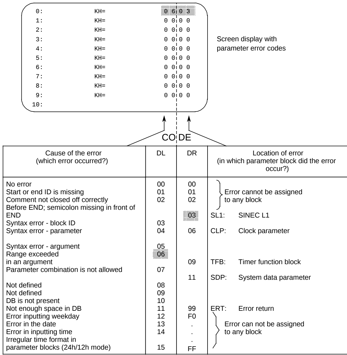
Figure 9-3. Parameter Error Codes and Their Meaning
