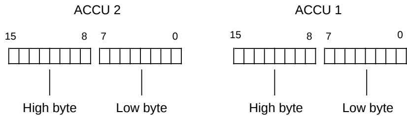
Figure 8-1. Accumulator Structure
