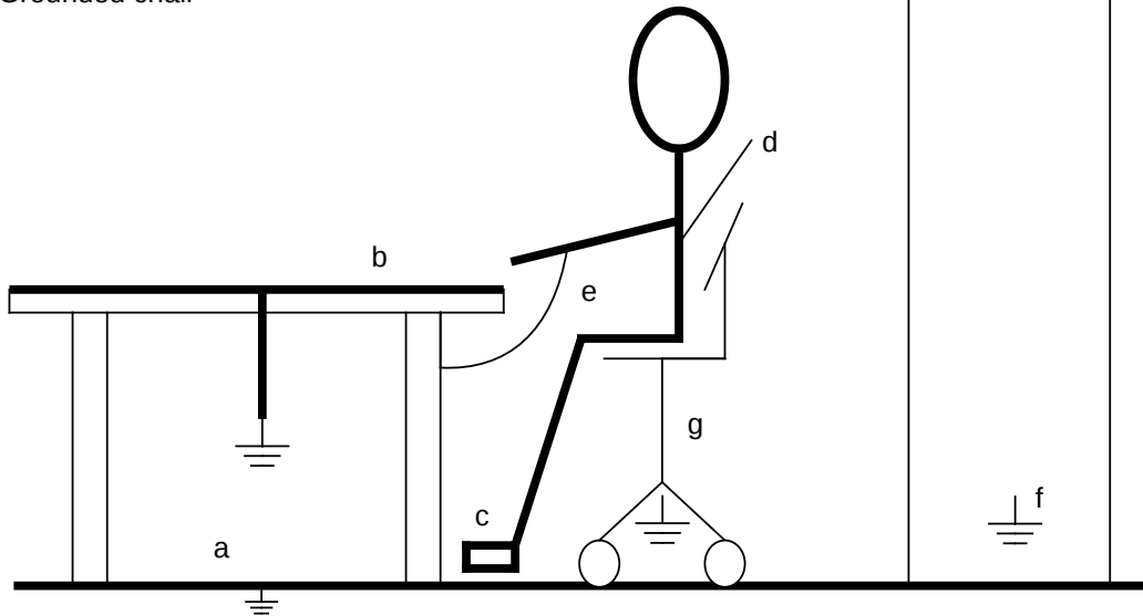
Figure C-1. ESD Measures
