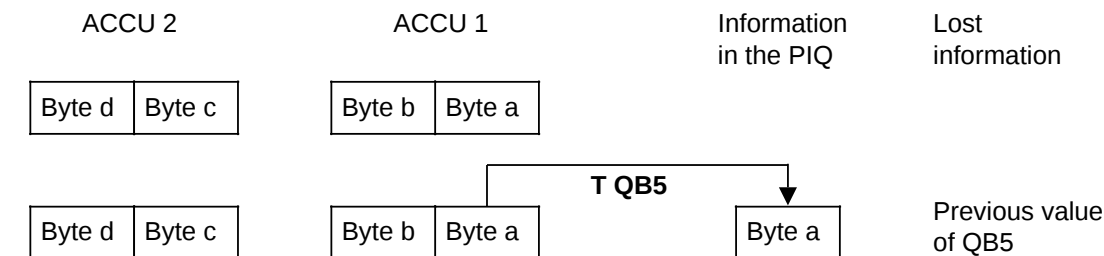
Figure 8-3. Transferring a Byte
