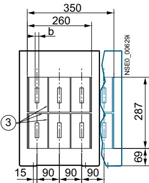
Vertical connection
