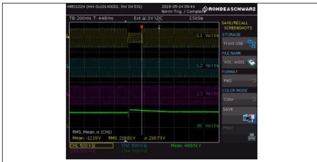
Input voltages phases L1 – L3, DC Link Voltage
