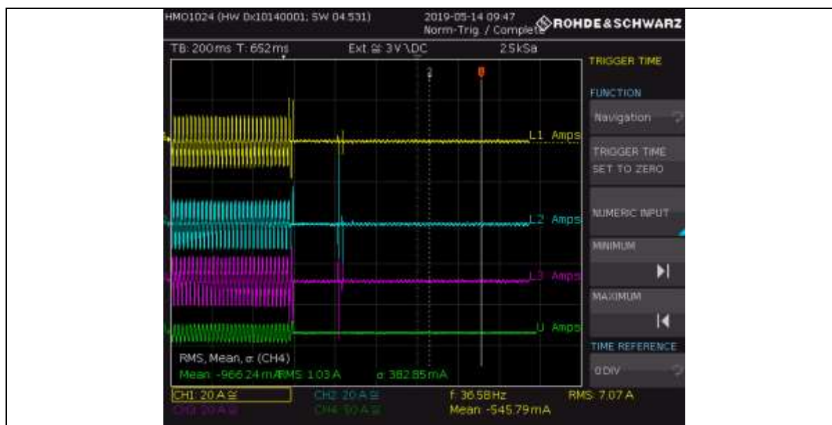
Input currents phases L1 – L3, Output current U
