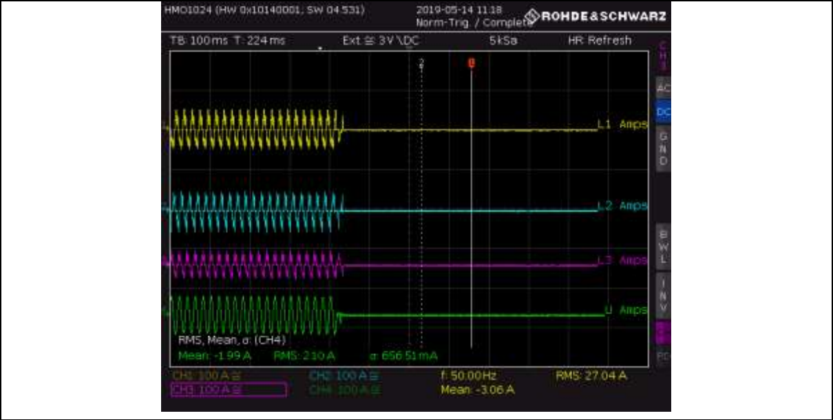
Input currents phases L1 – L3, Output current U
