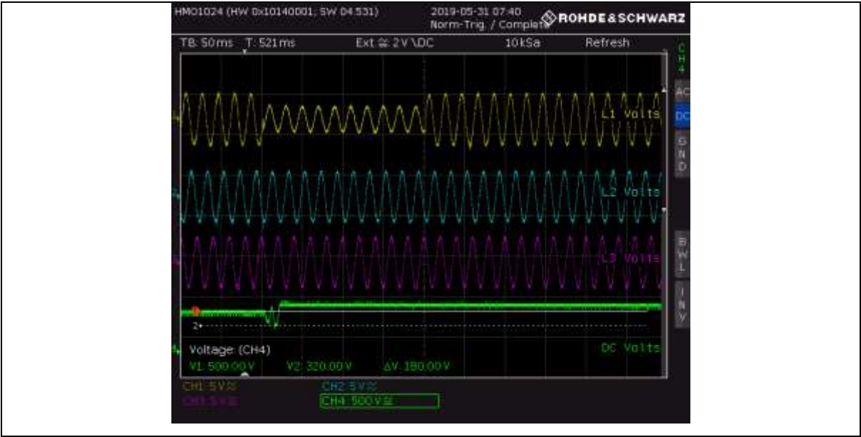
Input voltages phases L1 – L3, DC Link Voltage
