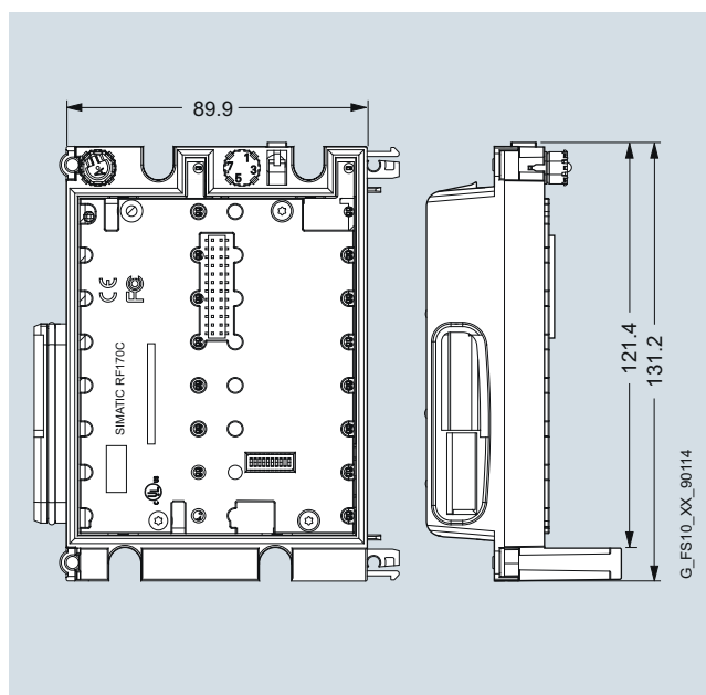
SIMATIC RF170C communications module
