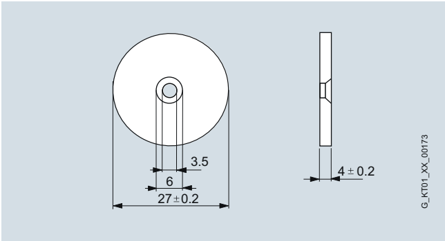
MDS D424 transponder
