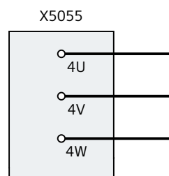
Figure 3-4 Connection of motor phases
