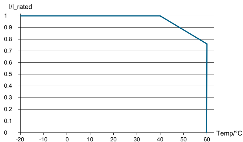
Figure 5-2 Derating for PDC1000 as a function of the ambient temperature
