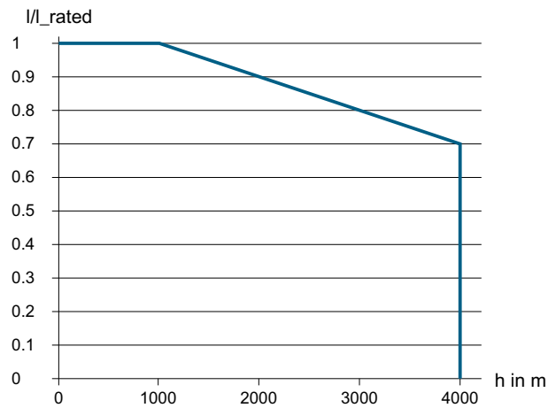
Figure 5-1 Derating for PDC1000 as a function of the installation altitude
