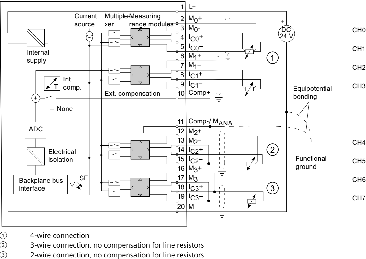
Figure 6-15 Block diagram and wiring diagram
