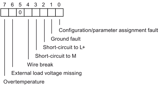
Figure B-6 Diagnostic byte for a digital output channel of the SM 322; DO DC 8 x 24 V/0.5 A
