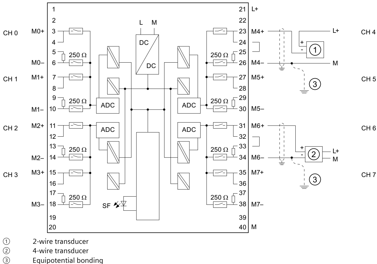
Figure 6-4 Wiring and block diagram
