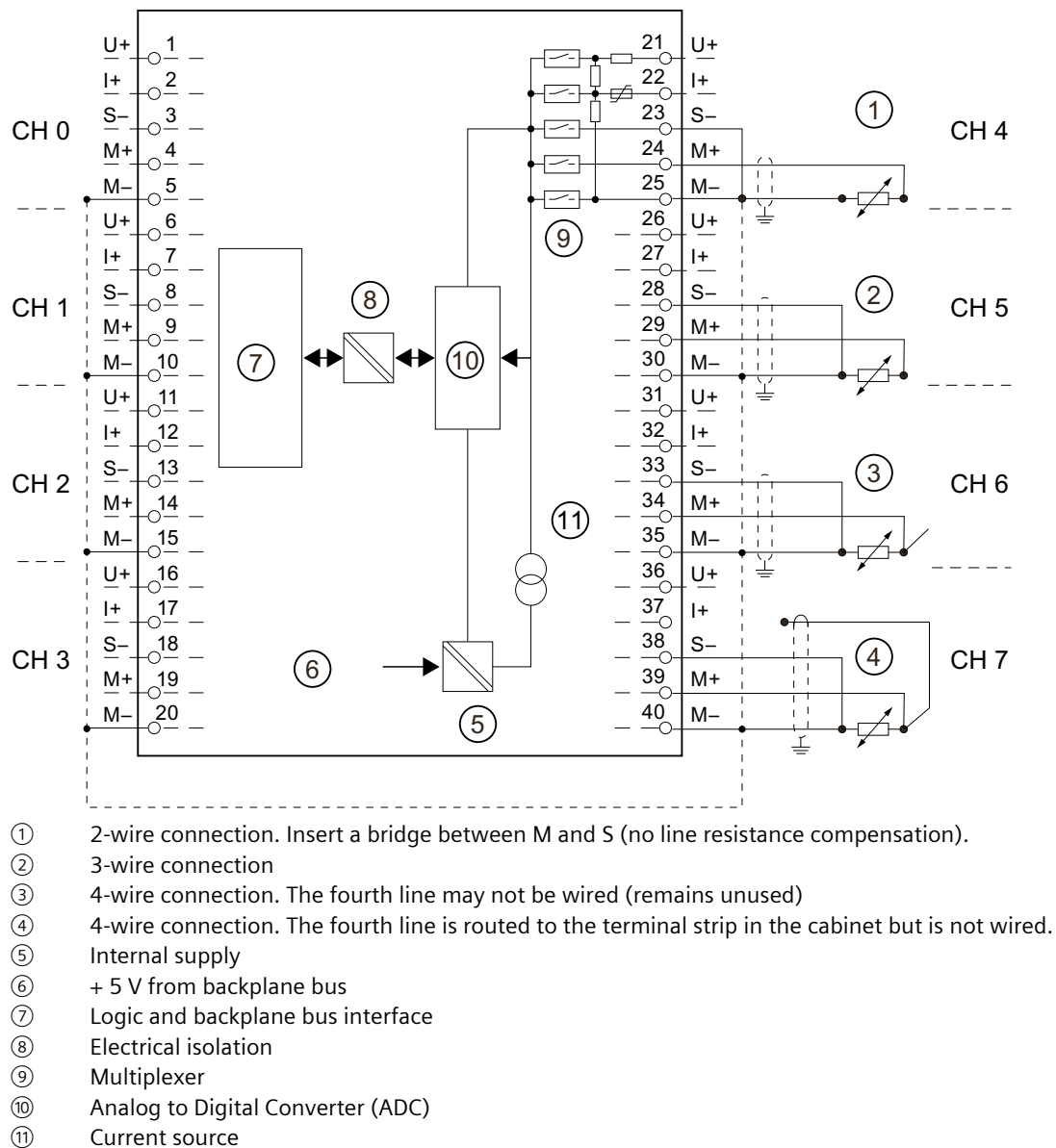
Figure 6-12 Block diagram and terminal diagram
