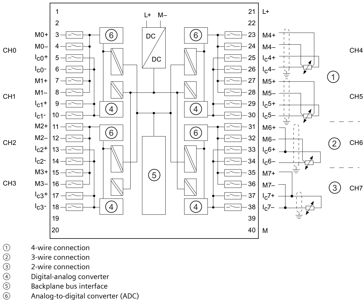
Figure 6-21 Wiring and block diagram
