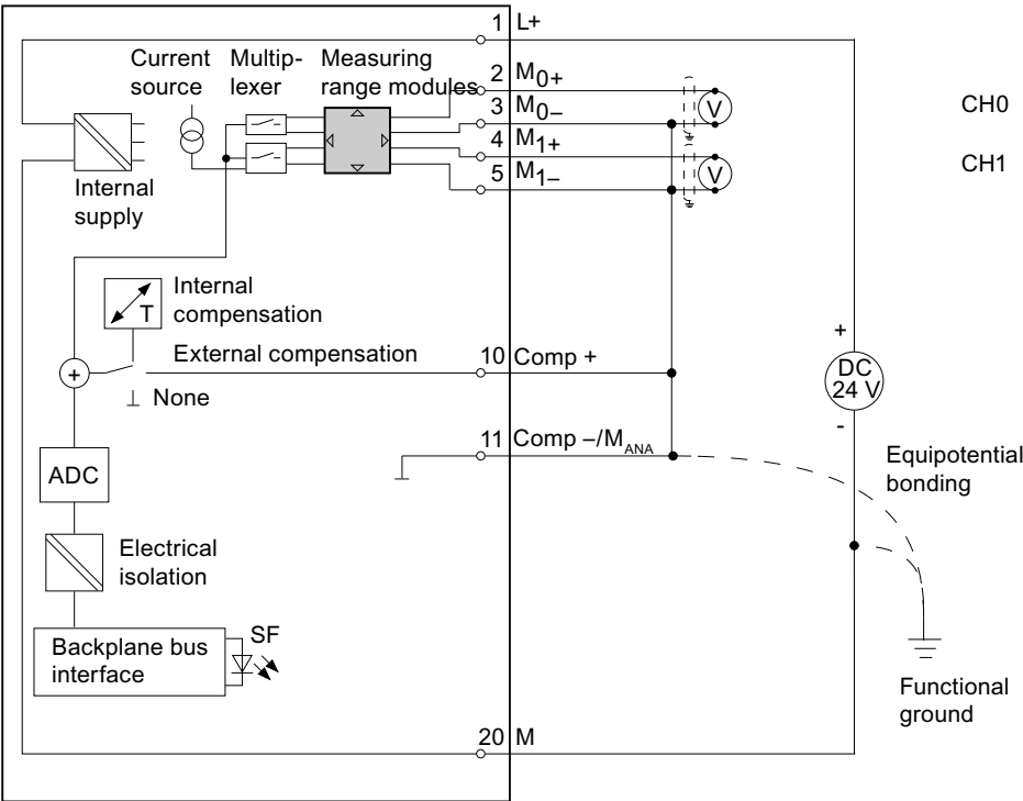
Figure 6-17 Wiring and block diagram
