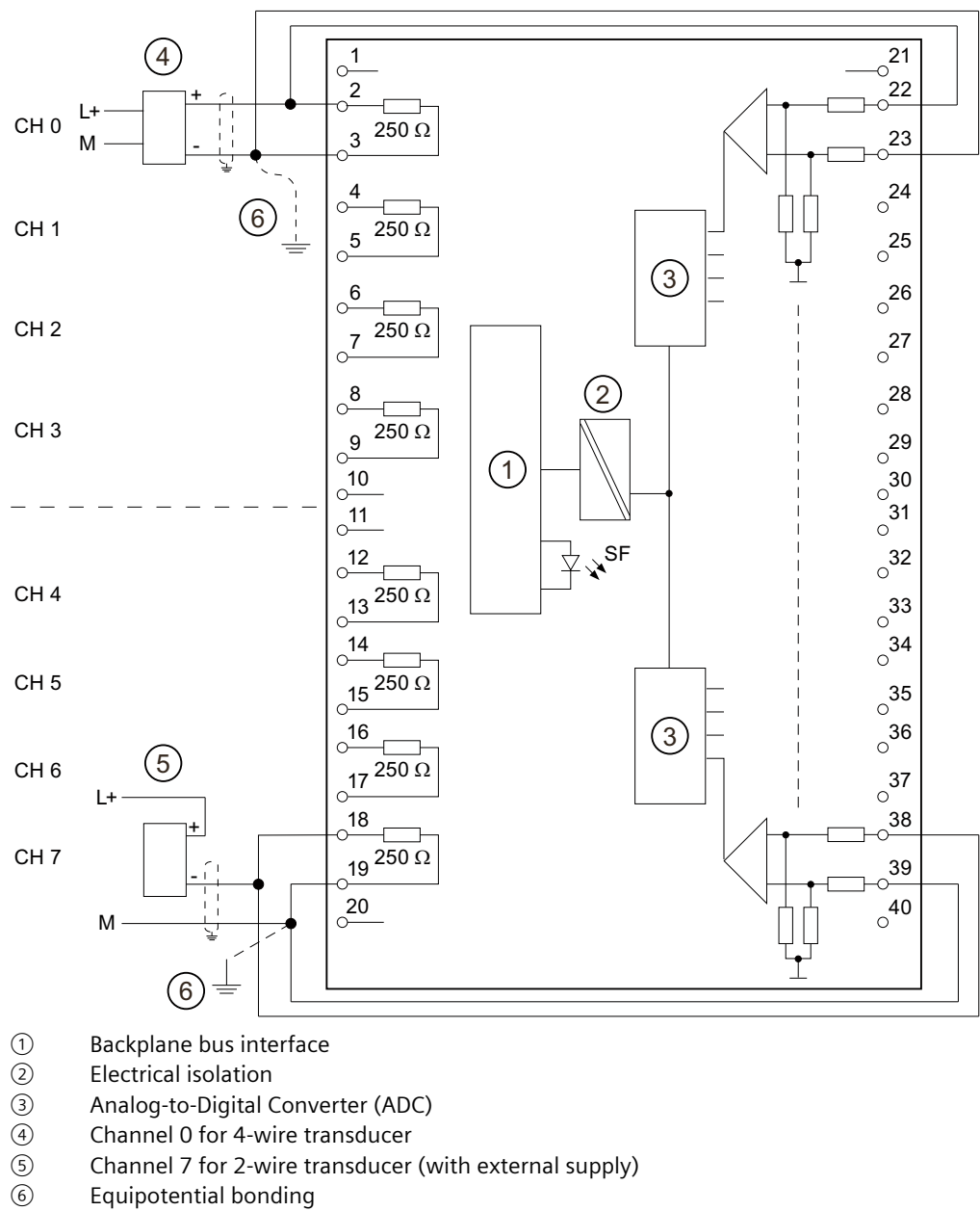
Figure 6-2 Wiring and block diagram
