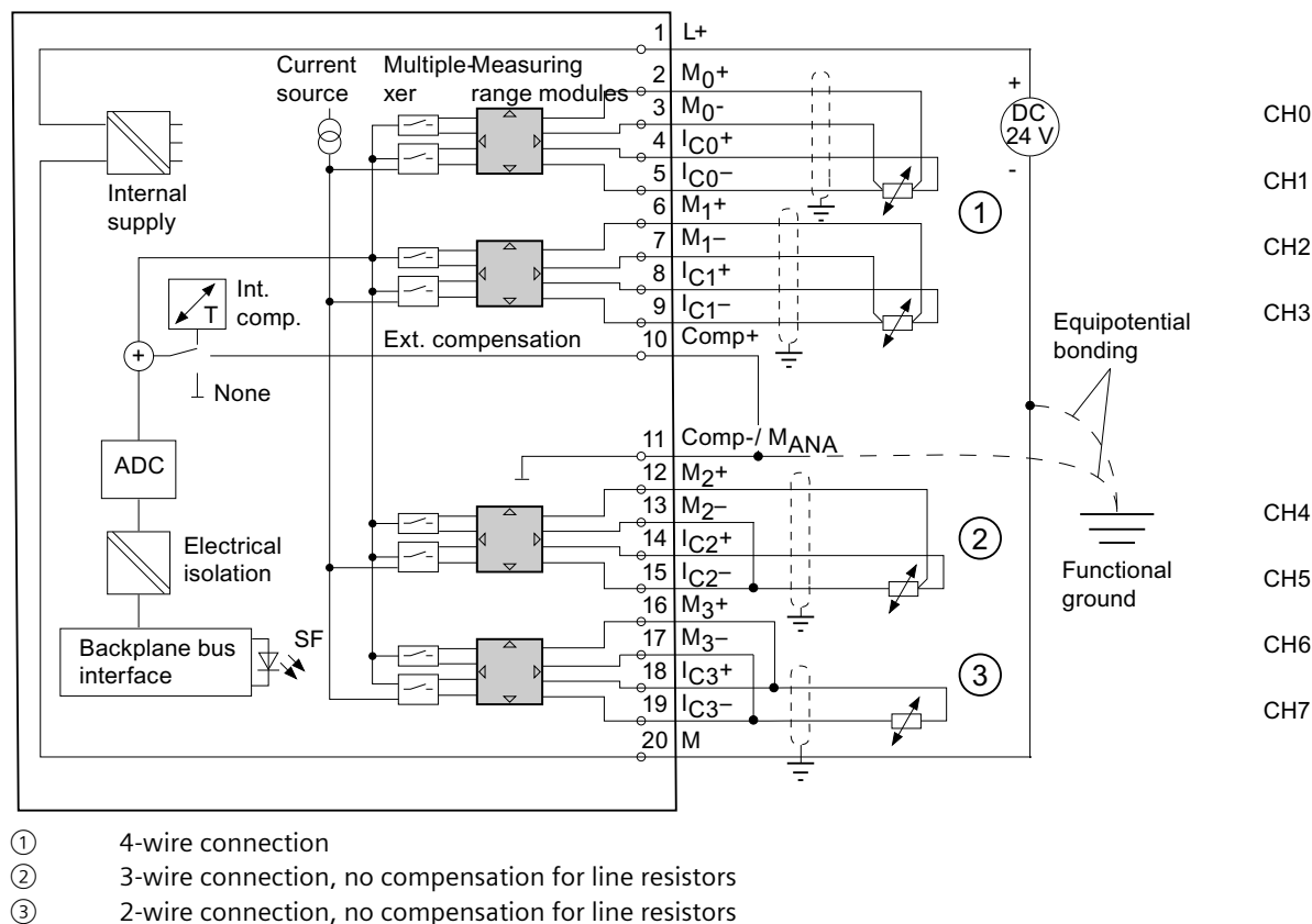
Figure 6-15 Block diagram and wiring diagram
