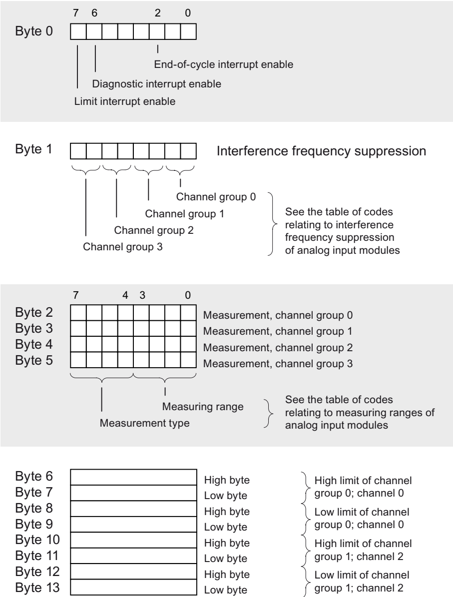
Figure A-5 Data record 1 for the parameters of analog input modules
