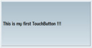
图 9-28 TextAlignment - 左
