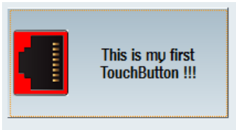
图 9-27 ShowFocusRect
