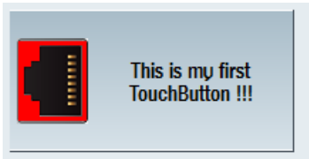
图 9-25 Unchecked
