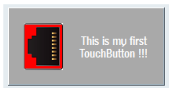
图 9-35 setMargins(20, 20, 20, 20, 20)
