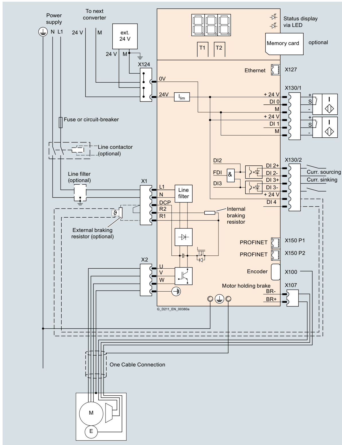
Connection example SINAMICS S210 servo converter, 1 AC series
