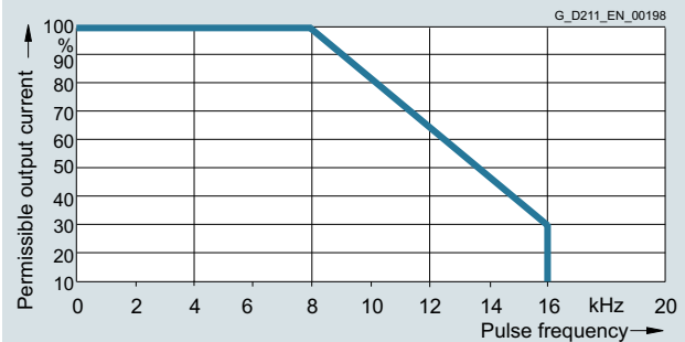
Output current as a function of pulse frequency
