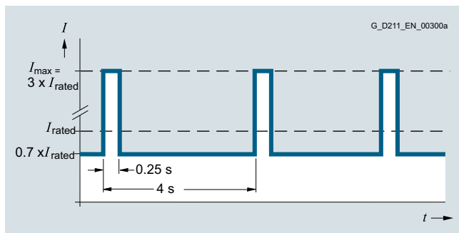
Peak current duty cycle with previous load (300 % overload)
