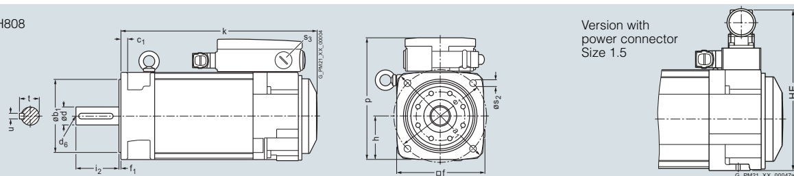
Hollow shaft 1PH808
