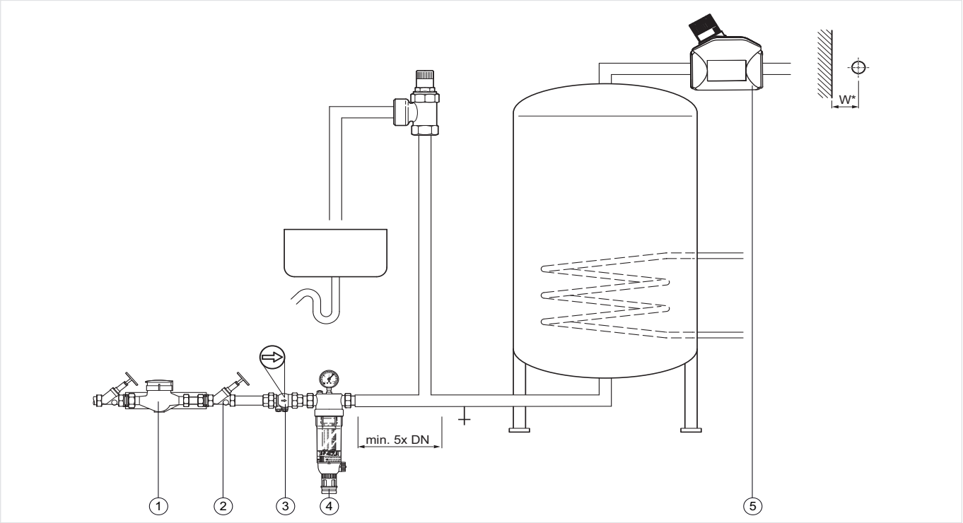
Fig. 1 Standard installation example for the pressure reducing valve
