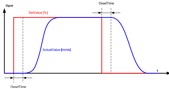
Figure 3-3 Dead time between the setpoint output and the movement of the hydraulic axis
