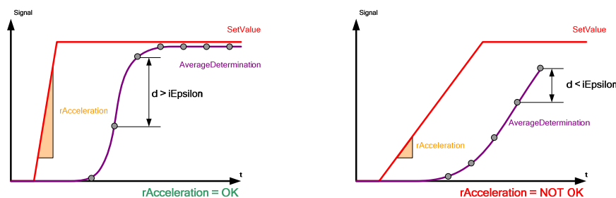
Figure 8-7 Expert parameter – acceleration “rAcceleration”
