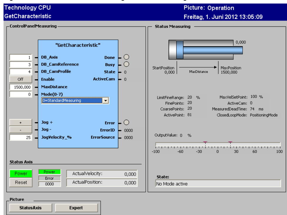
Figure 2-1 HMI user interface for usage as commissioning tool
