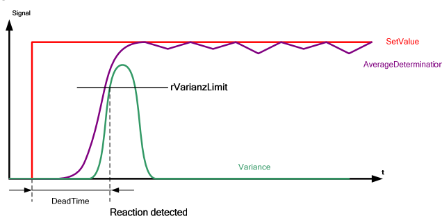
Figure 8-5 Expert parameter - decision threshold “rVarianzLimit”
