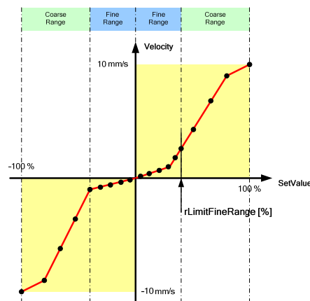
Figure 8-6 Expert parameter – limit coarse/fine range “rLimitFineRange”
