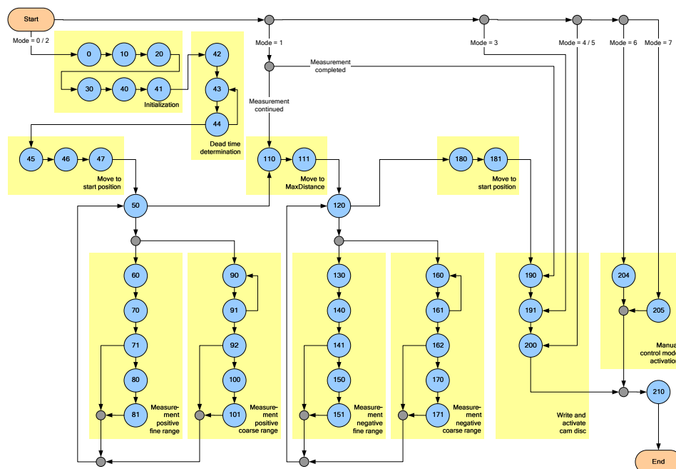
Figure 8-1 Finite state machine of the FB 520 “GetCharacteristics” block
