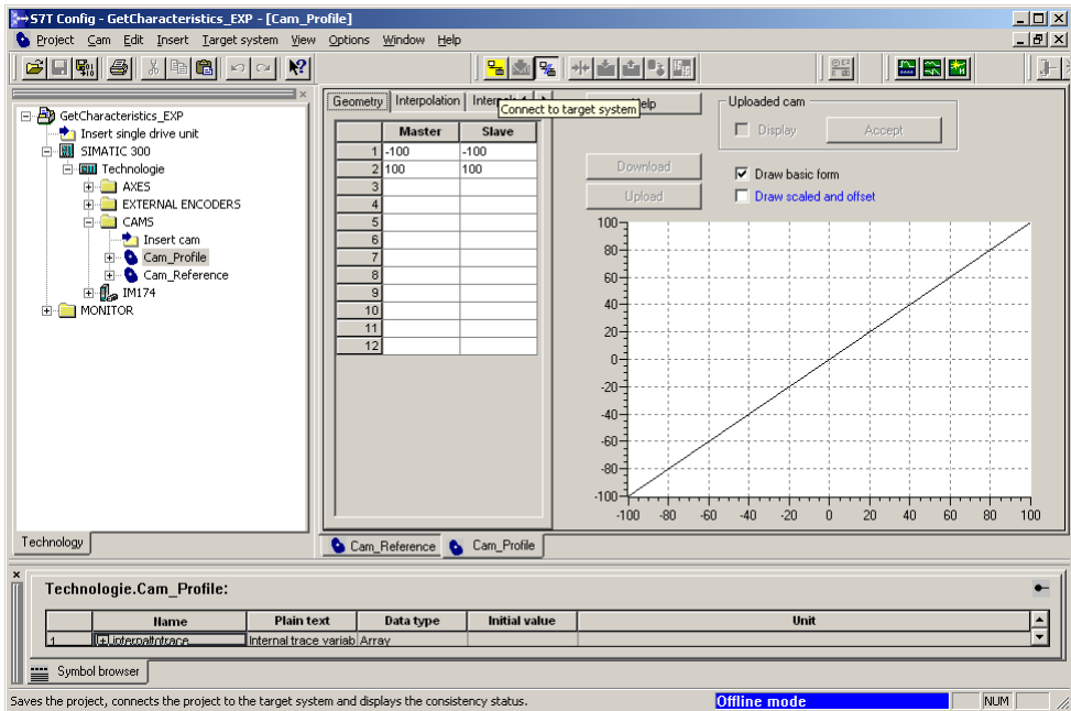
Figure 4-1 Creating the required cam disks as interpolation point table
