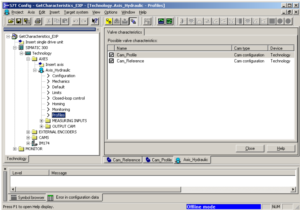
Figure 4-2 Defining the cam disks as compensation characteristic
