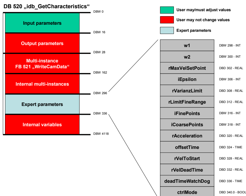
Figure 6-2 Structure of the instance data block
