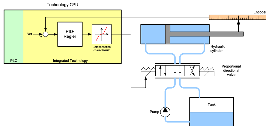
Figure 1-1 Control of a hydraulic axis
