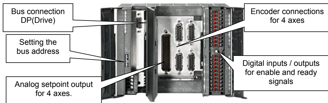
Figure 2-3 Interfaces of IM174 for the activation of the hydraulic axes
