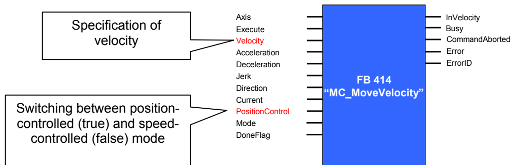
Figure 9-1 Selection of open-loop mode via FB 414 "MC_MoveVelocity"
