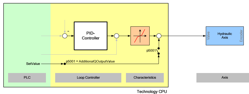
Figure 9-3 Direct output of a voltage value
