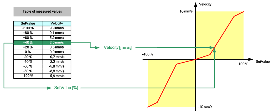
Figure 3-2 Creating the compensation characteristic
