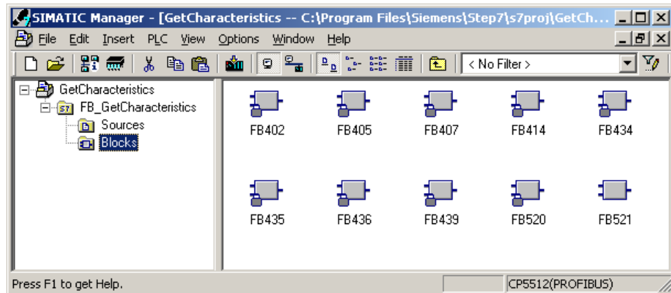
Figure 5-1 Blocks of the technology template
