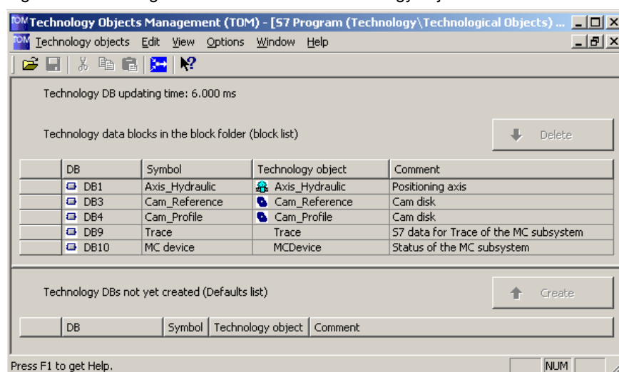
Figure 4-4 Creating the data blocks of the technology objects
