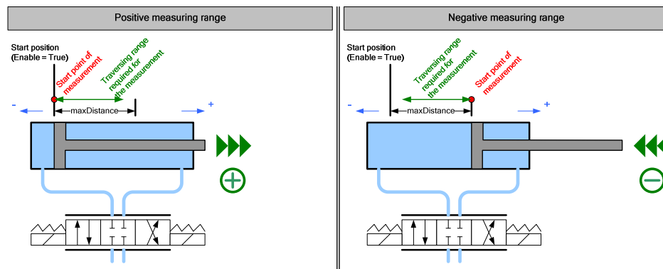
Figure 6-3 Selection of the start position and setting of the “maxDistance” parameter
