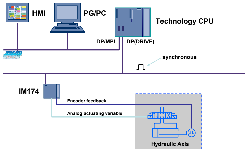
Figure 2-2 Typical structure for controlling a hydraulic axis
