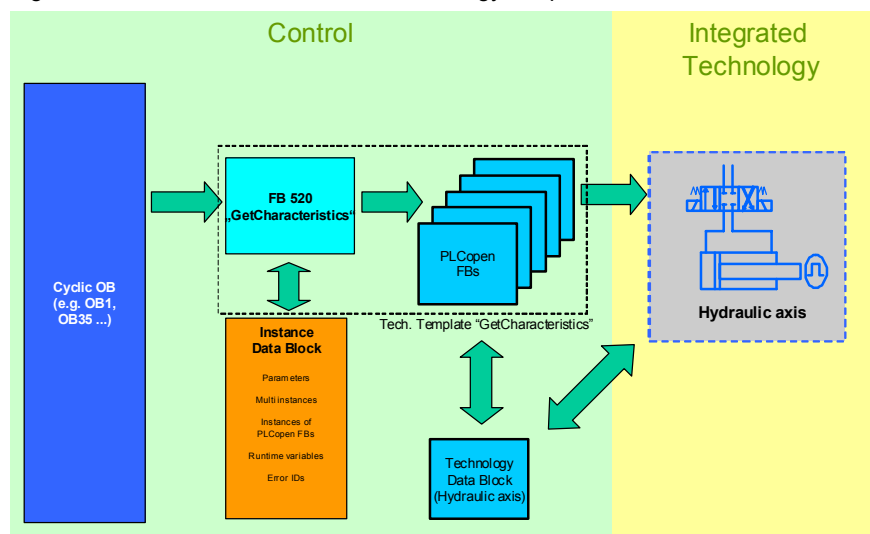
Figure 6-1 Call environment of the technology template
