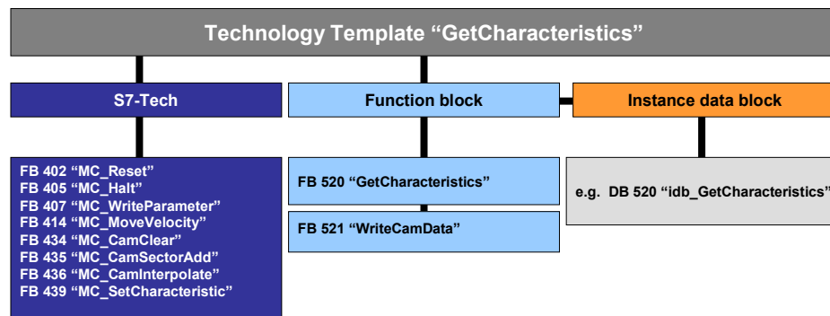
Figure 1-3 Components contained in the technology template
