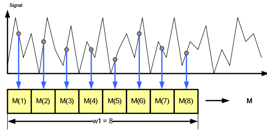
Figure 8-2 Expert parameter – window length “w1”
