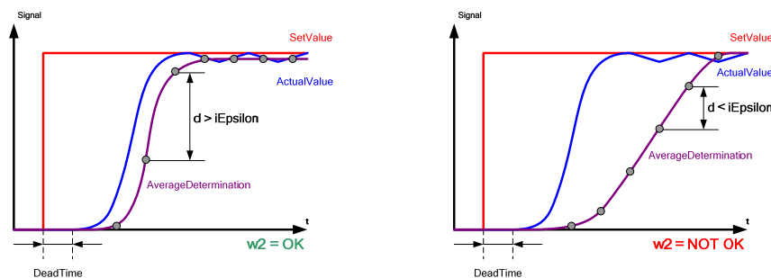
Figure 8-3 Expert parameter - window length “w2”
