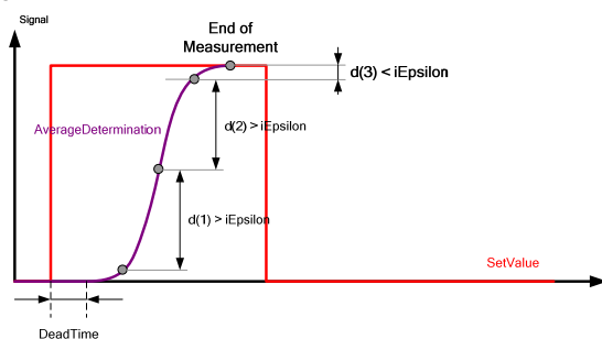
Figure 8-4 Expert parameter - decision threshold “iEpsilon”
