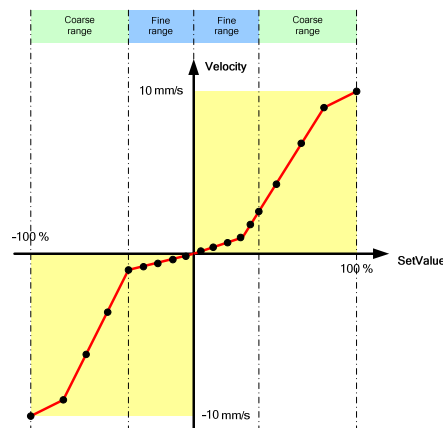
Figure 3-4 Increasing the accuracy of the compensation characteristic
