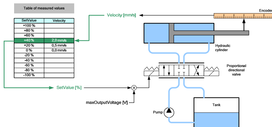
Figure 3-1 Measuring principle
