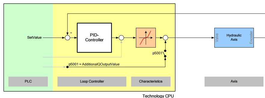
Figure 3-5 Integration of the compensation characteristic into the control loop
