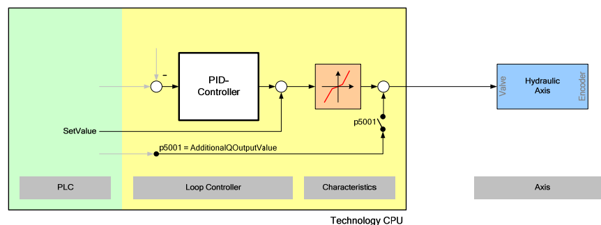
Figure 9-2 Modification of the control loop in open-loop mode
