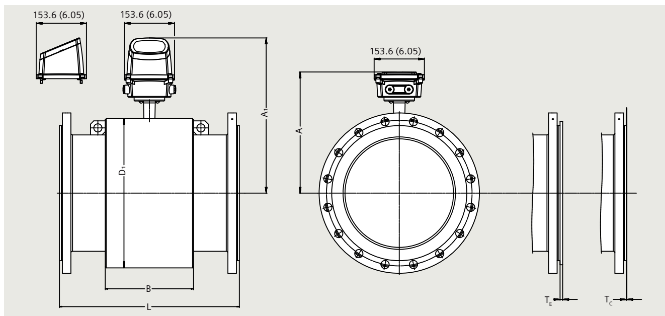
SITRANS FMS300 sensor in compact (integral-mount transmitter) and remote design. Dimensions in mm (inch)
