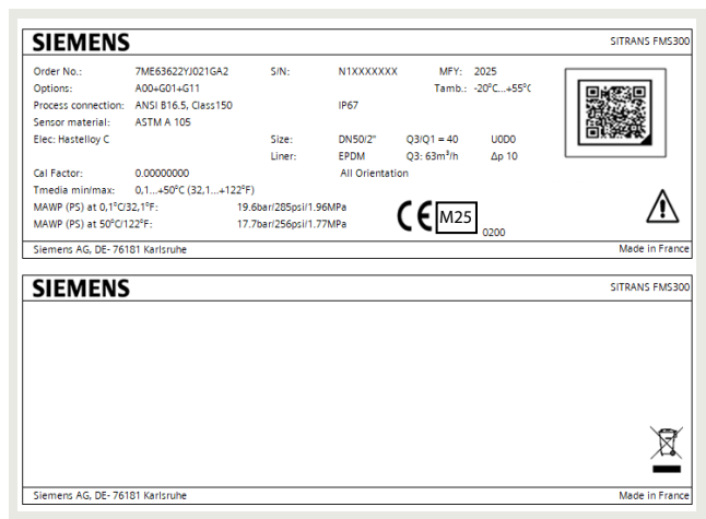
Sensor label
