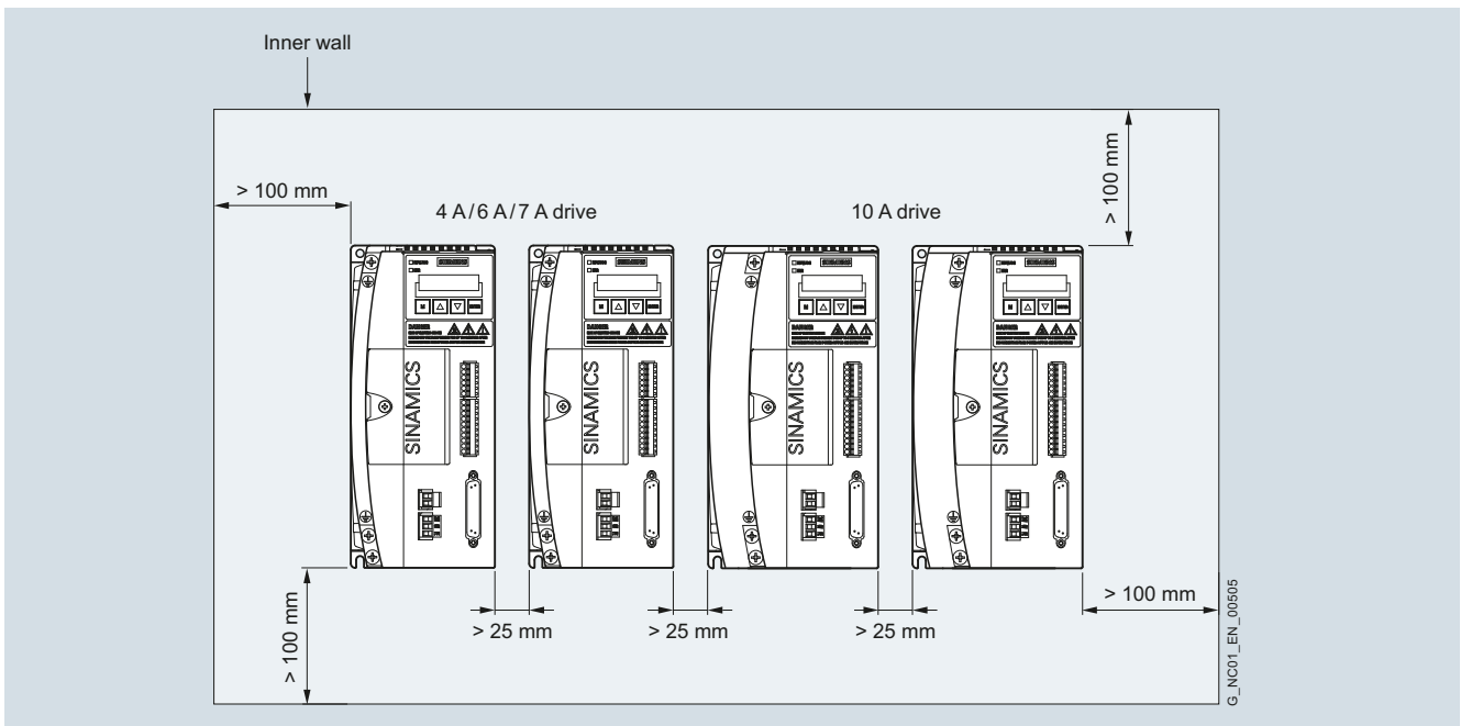
Mounting clearance
