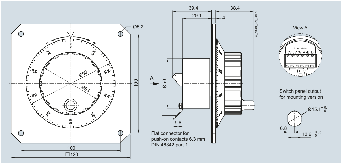
Electronic handwheel with front panel 120 mm × 120 mm
