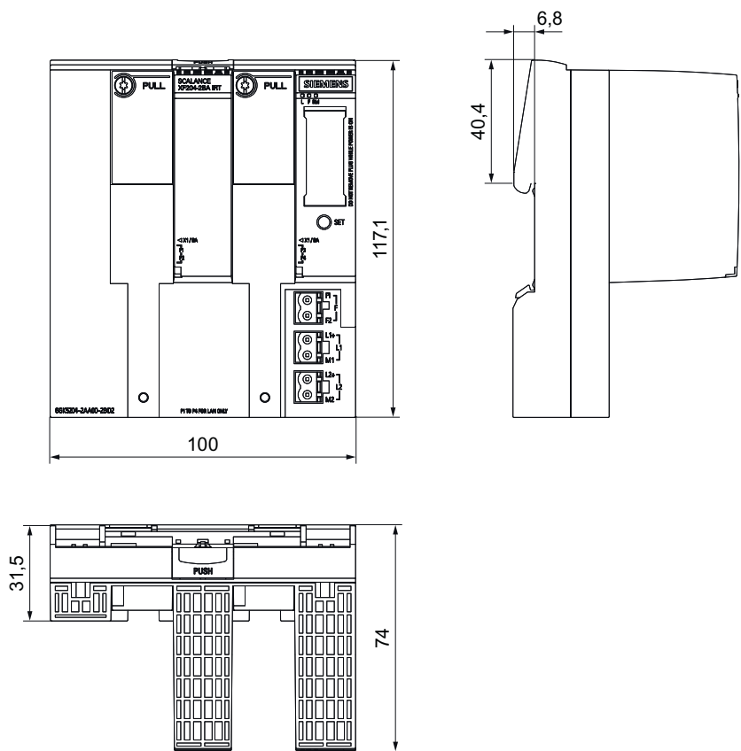
Figure A-9 Dimension drawing SCALANCE XF204-2BA IRT
