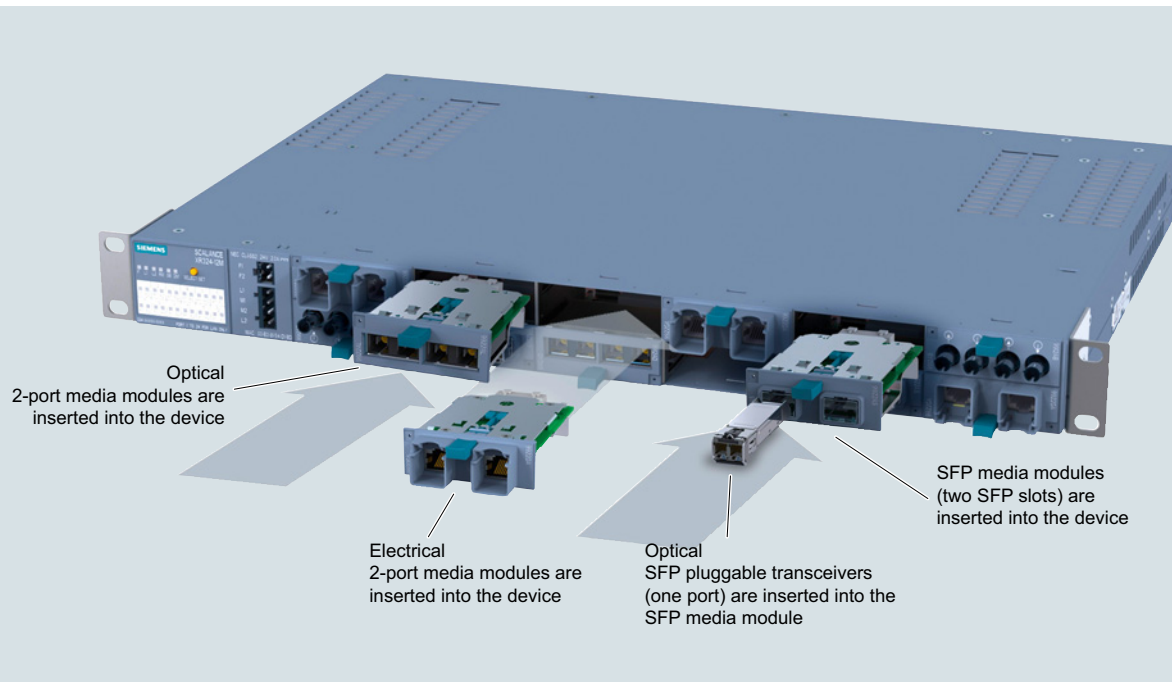
Insertion of 2-port media modules in media module slot
