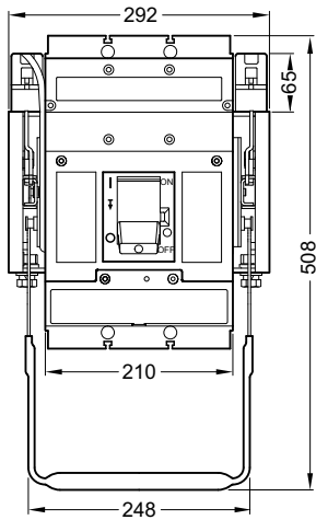
Withdrawable version
