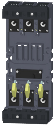
Locking plug-in base against inserting the circuit breaker/disconnector
