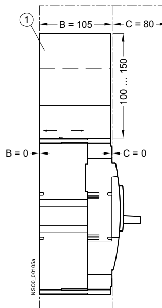
① 3VT9200-8CB30
