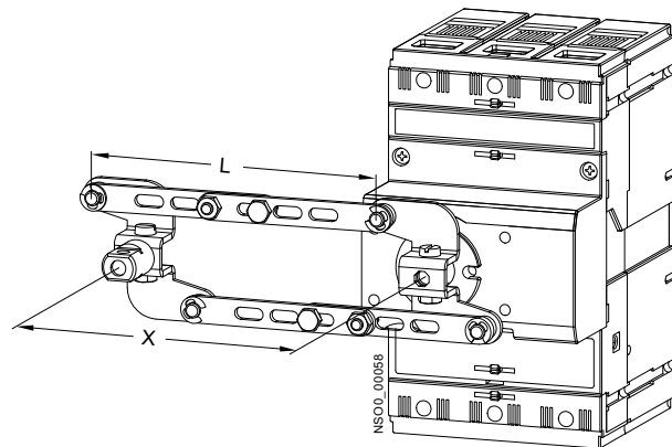
Arrangement of circuit breakers/switch disconnectors with 3VT9100-8LB00 mechanical interlocking for parallel switching
