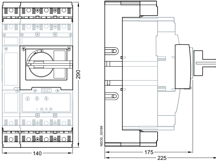
Plug-in version, rotary operating mechanism
