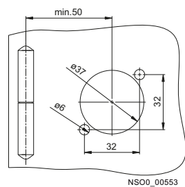
Dimensions of door cut-out
