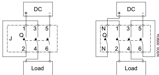
Connection of 3P circuit breaker in DC circuit up to 250 V DC
