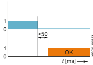
Reaction time of the shunt trip
