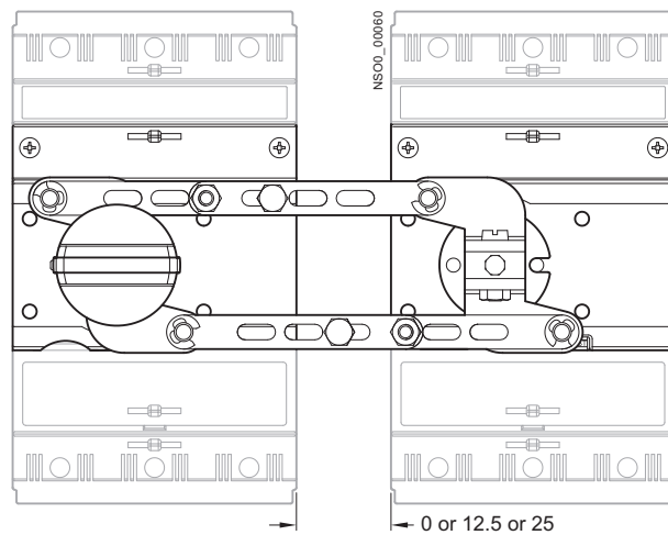
Arrangement of circuit breakers/switch disconnectors with 3VT9100-8LB00 mechanical interlocking for parallel switching
