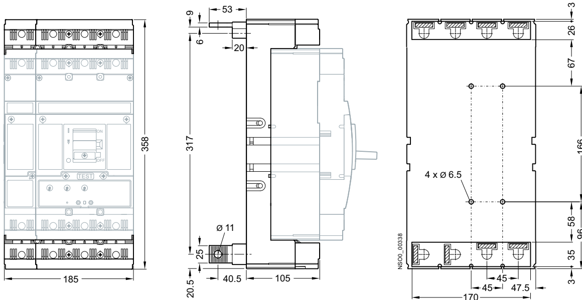
Drilling pattern
