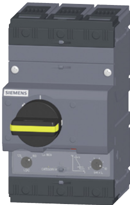
Fig. 1: Rotary operating mechanism with knob
