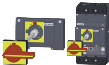
Fig. 2: Rotary operating mechanism with extension shaft, coupling driver and knob
