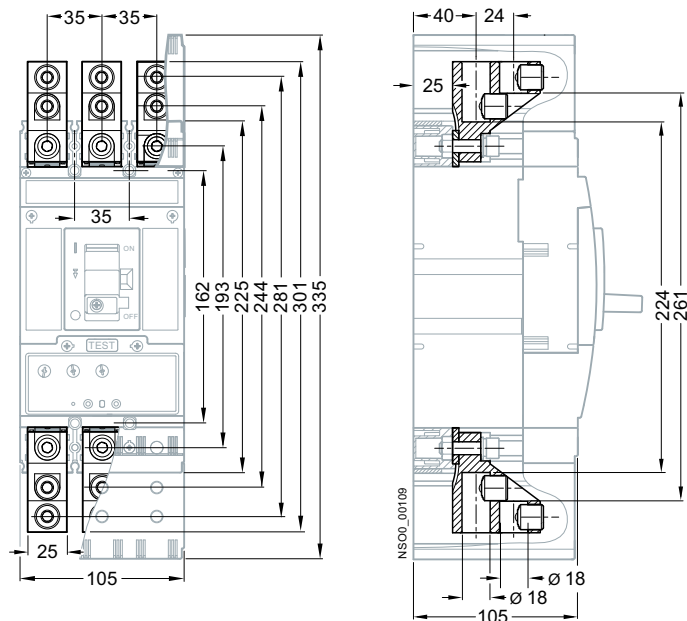
Fixed-mounted version, front connection (3VT9215-4TF30 connecting set)
