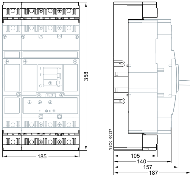
Plug-in version, rear connection with 3VT9300-4RC30 + 3VT9300-4RC00 connecting set
