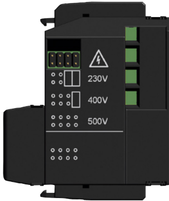
Location of accessory compartments 10 in 3VT2 circuit breakers
