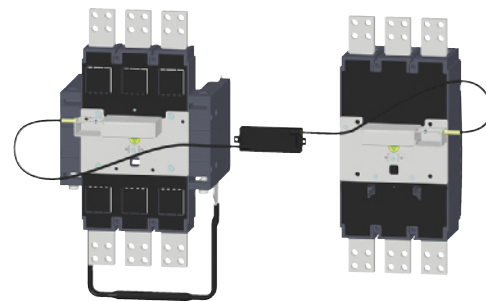
Mechanical interlocking by Bowden between fixed-mounted and withdrawable 3VT5 circuit breakers
