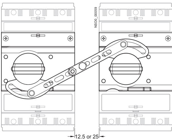
Arrangement of circuit breakers/switch disconnectors with 3VT9100-8LA00 mechanical interlocking
