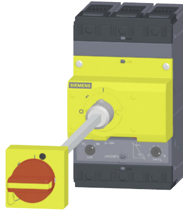
Fig. 2: Rotary operating mechanism with extension shaft, coupling driver and knob
