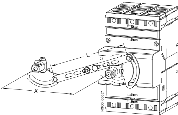
Arrangement of circuit breakers/switch disconnectors with 3VT9100-8LA00 mechanical interlocking
