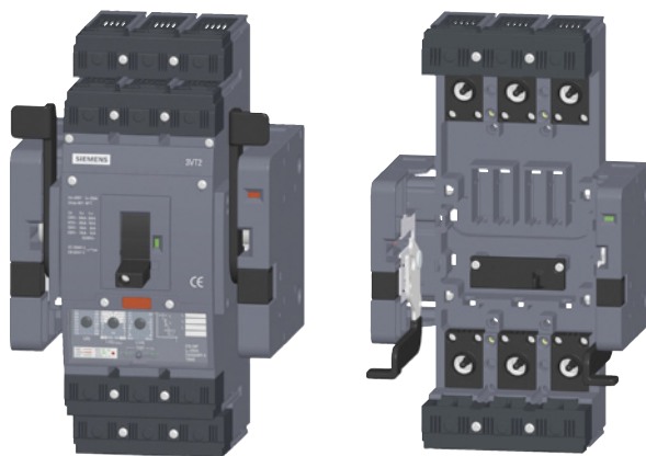
Circuit breaker installed in withdrawable version base
