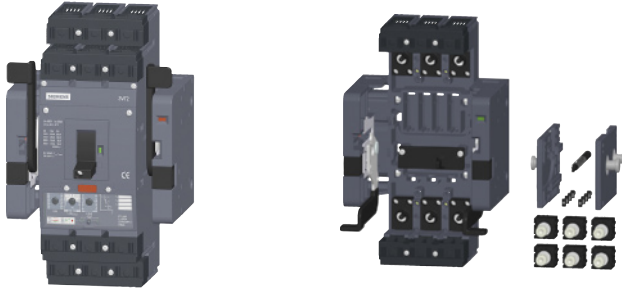
Circuit breaker installed in withdrawable version base
