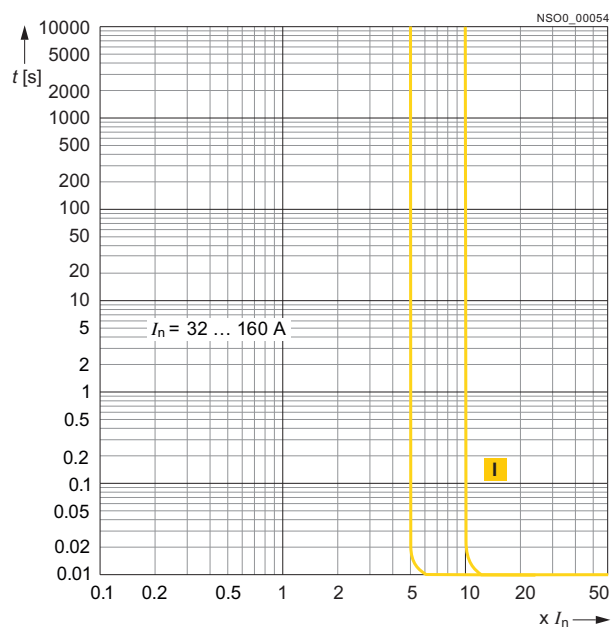
Characteristic "N", I_n = 32, 40, 50, 63, 80, 100, 125, 160 \text{ A}
