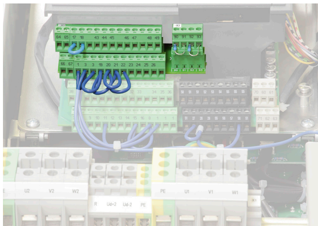
G04 Peripheral board 3 in the compact unit
