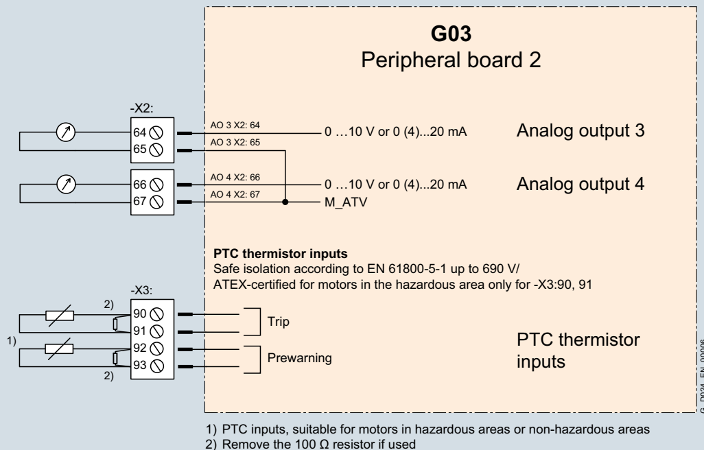
G03 Circuit diagram for peripheral board 2
