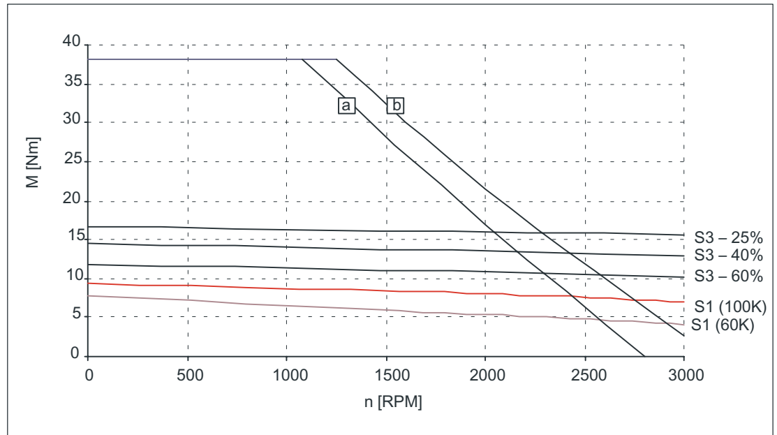
Figure 3-17 Speed-torque diagram 1FT6064-6AC7□
