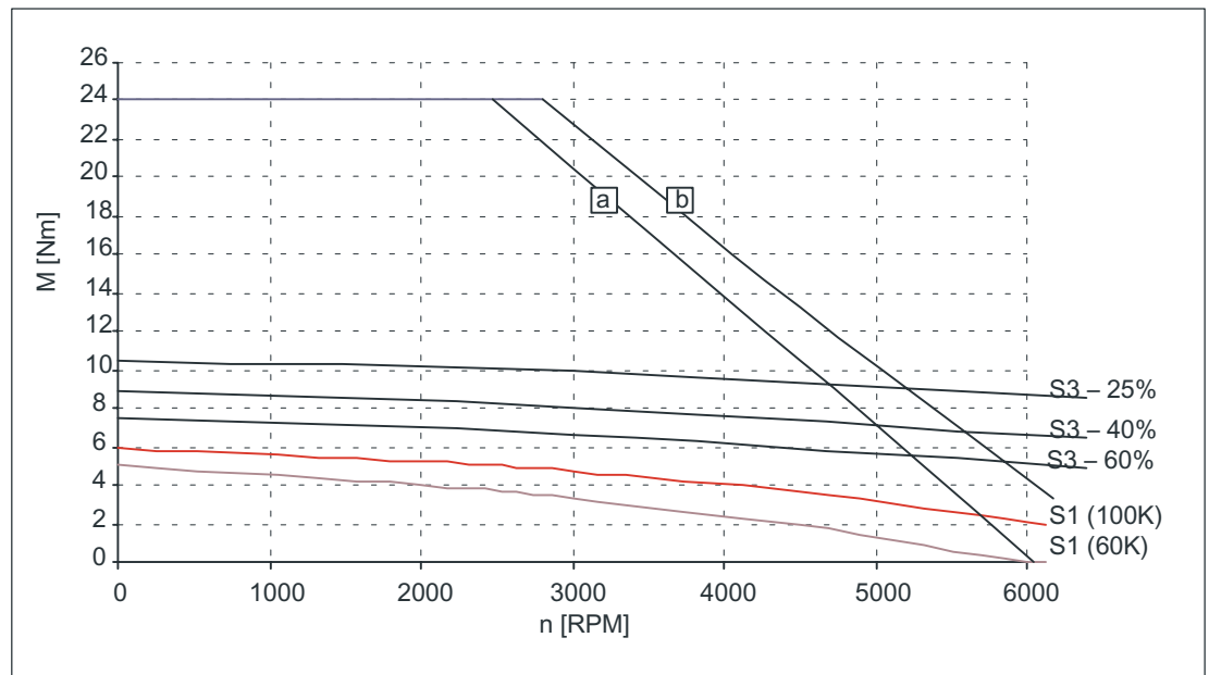
Figure 3-15 Speed-torque diagram 1FT6062-6AH7□
