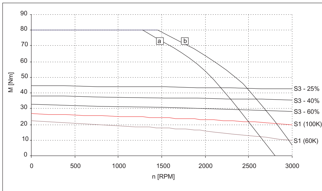
Figure 3-37 Speed-torque diagram 1FT6102-8AC7□
