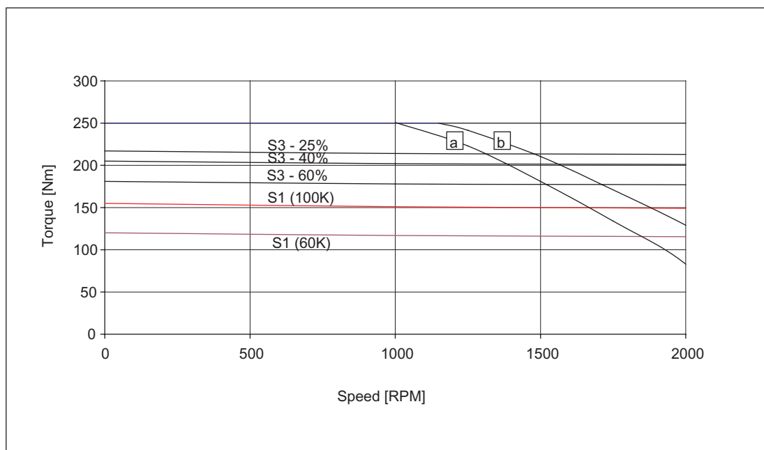
Figure 3-95 Speed-torque diagram 1FT6132-6WB7□
