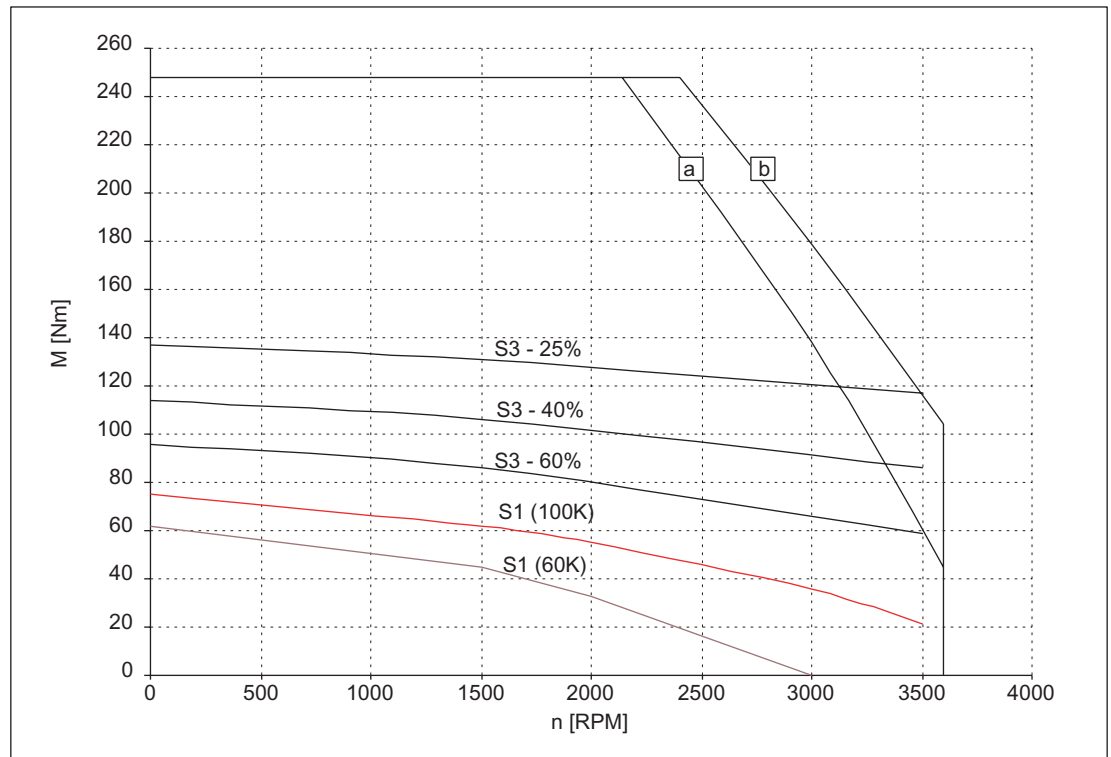
Figure 3-48 Speed-torque diagram 1FT6132-6AF71
