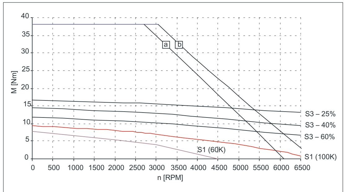
Figure 3-19 Speed-torque diagram 1FT6064-6AH7□
