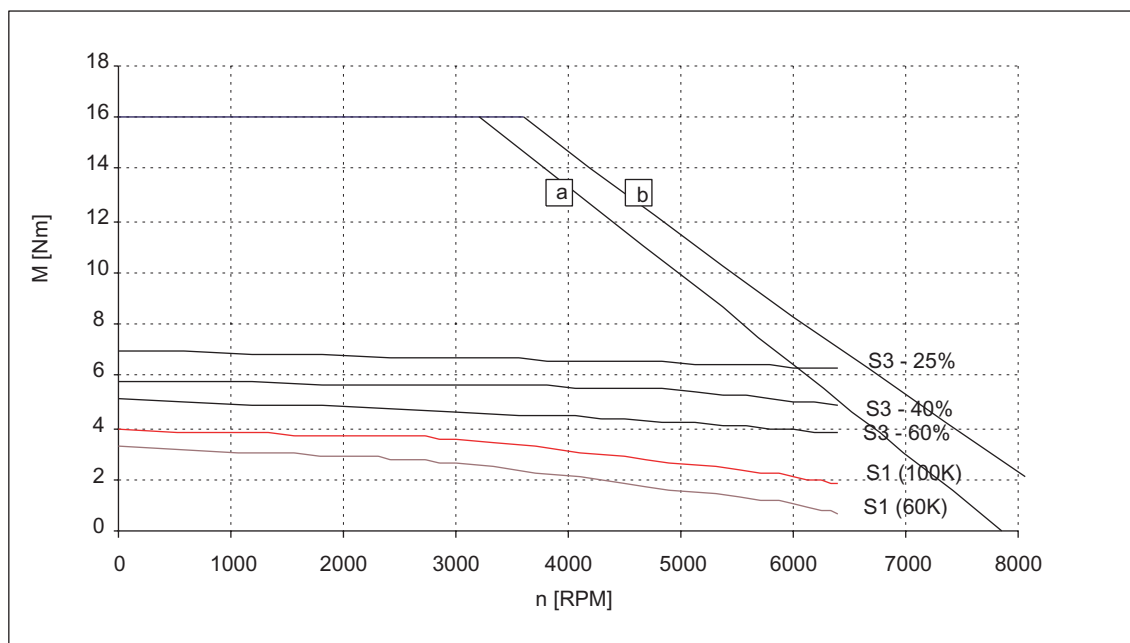
Figure 3-12 Speed-torque diagram 1FT6061-6AK7
