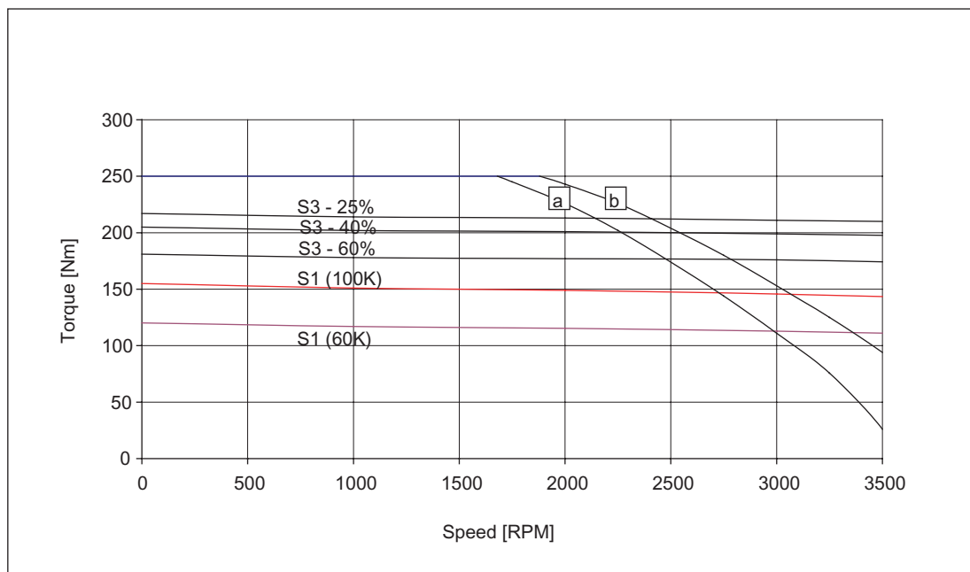
Figure 3-96 Speed-torque diagram 1FT6132-6WD7□
