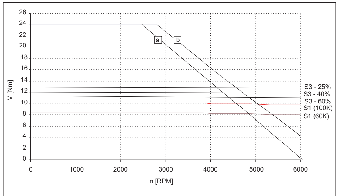
Figure 3-79 Speed-torque diagram 1FT6062-6WH7
