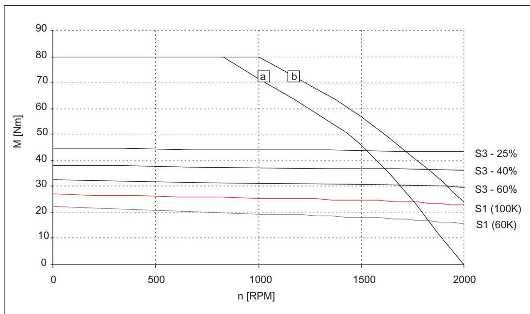
Figure 3-36 Speed-torque diagram 1FT6102-8AB7□
