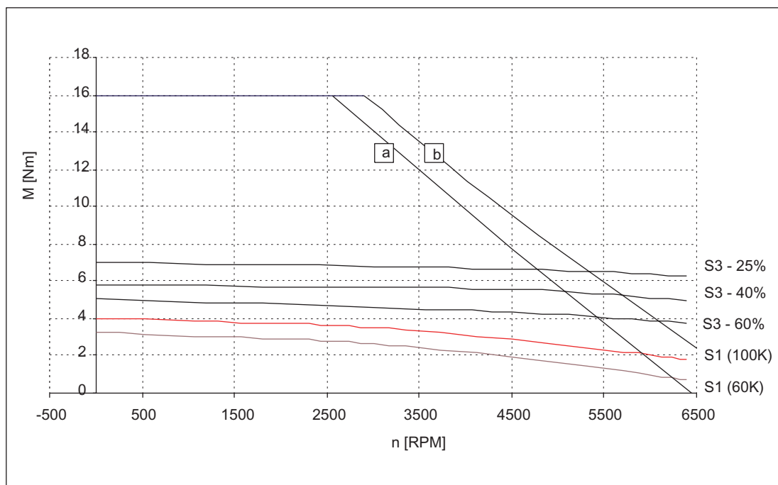
Figure 3-11 Speed-torque diagram 1FT6061-6AH7
