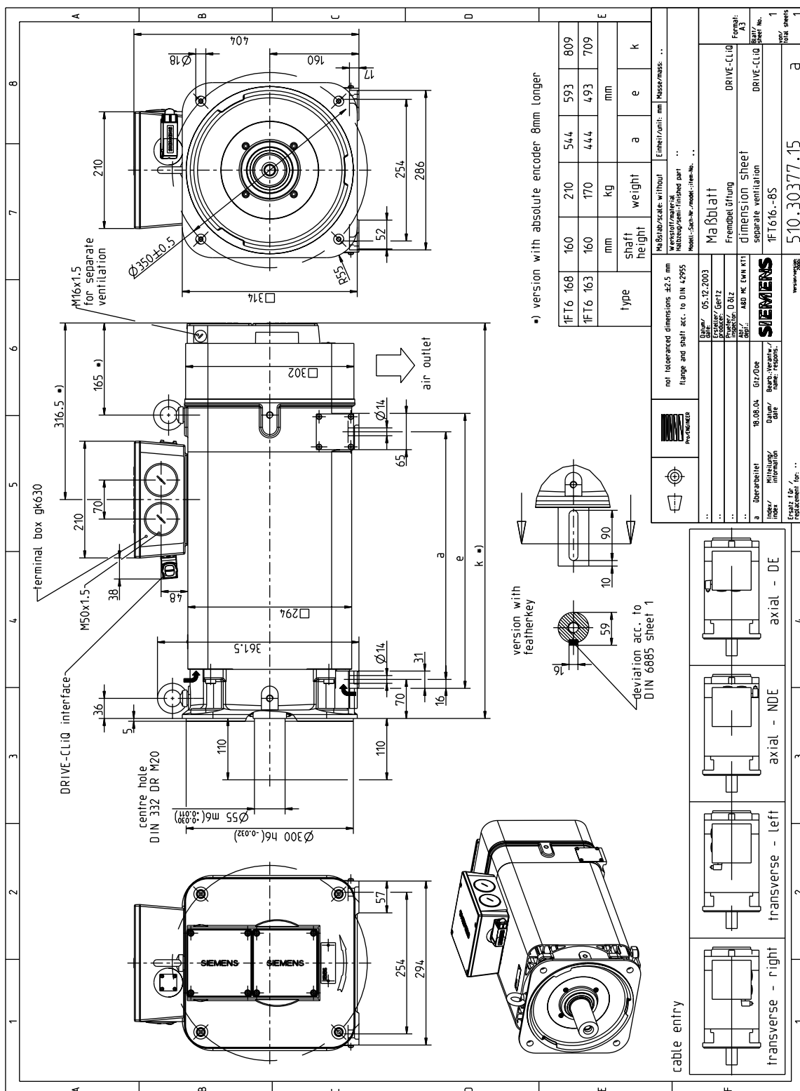
Figure 5-8 1FT616x-8Sx76-5xxx_DQ
