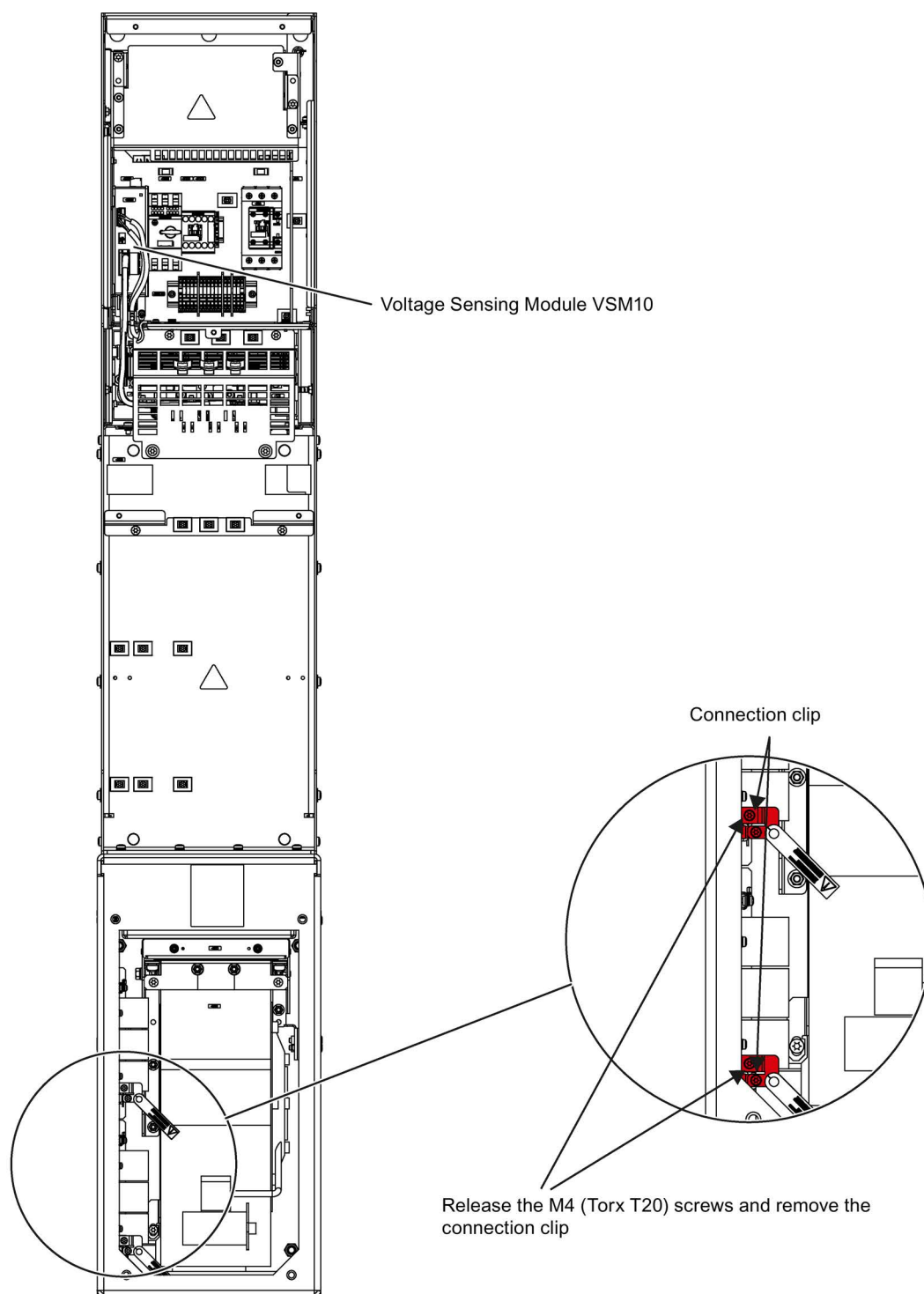
Figure 4-12 Removing the connection clip of the basic interference suppression module to ground for frame size HI
