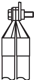
Figure A-2 2 cable lugs per connection
