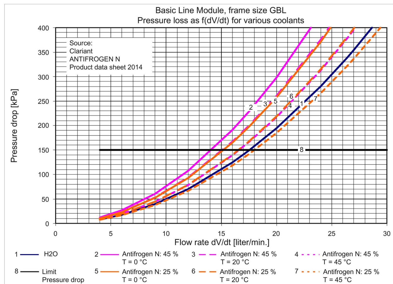
Figure 10-6 Pressure drop as a function of volumetric flow for Basic Line Module, frame size GBL
