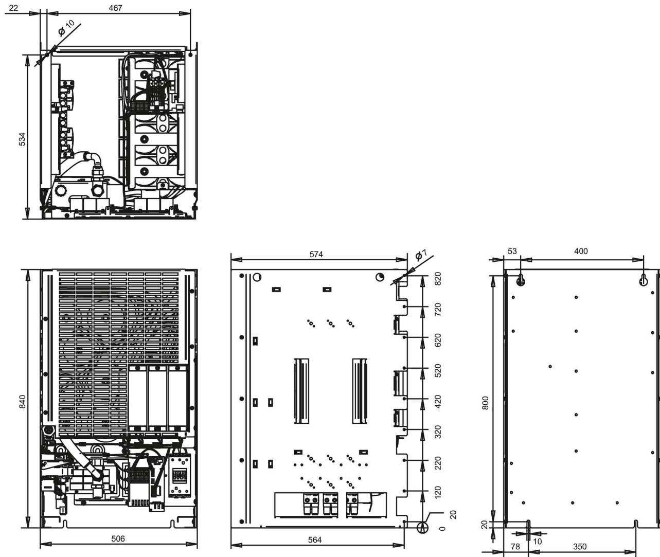
Figure 4-19 Dimension drawing, filter module, frame size J1L
