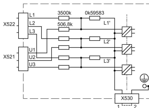
Figure 4-7 Internal circuit of the VSM10 Voltage Sensing Module
