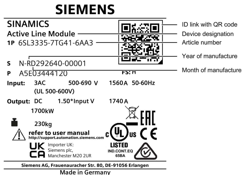
Figure 11-24 Nameplate using an Active Line Module as example
