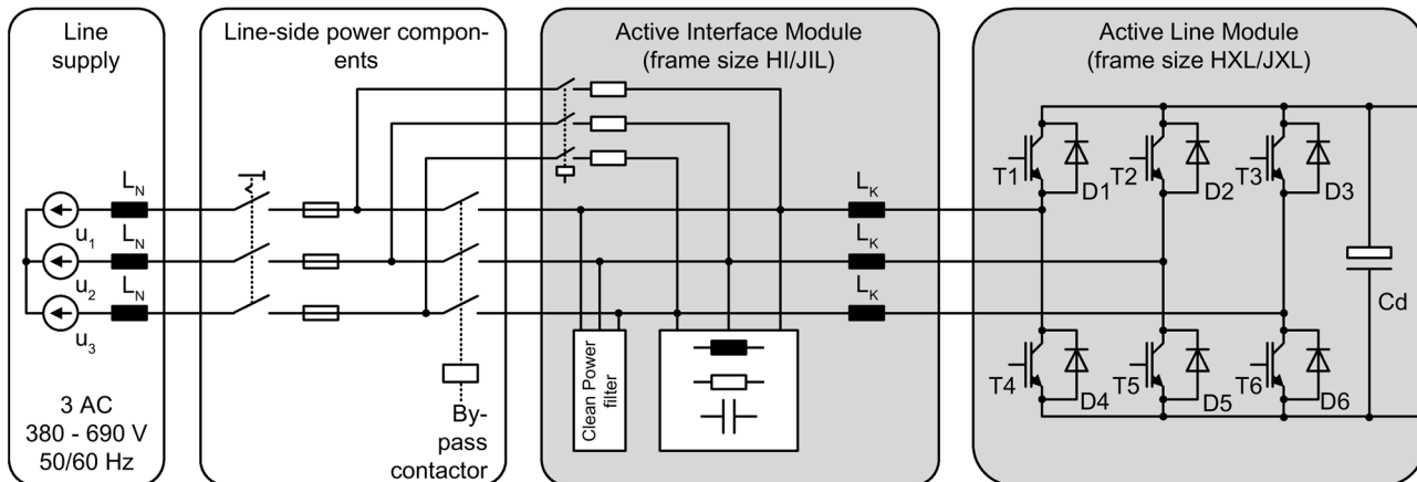
Figure 6-11 Overview of Active Infeeds, frame sizes HI/HXL and JI/JXL
