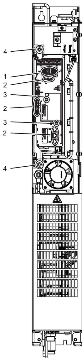
Figure 11-11 Replacing the Control Interface Module, Basic Line Module, frame size FBL
