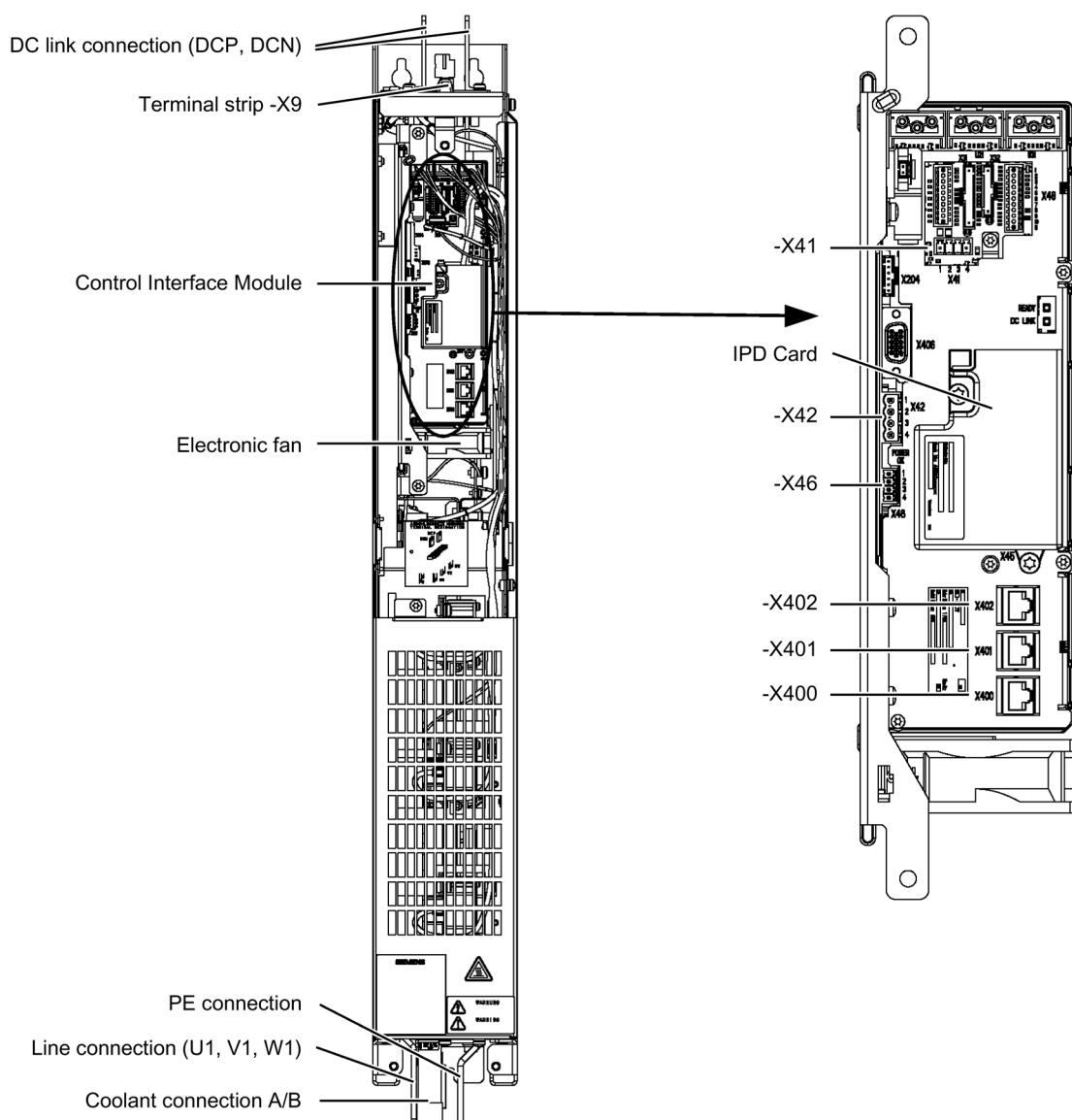
Figure 6-12 Active Line Module, frame size GXL
