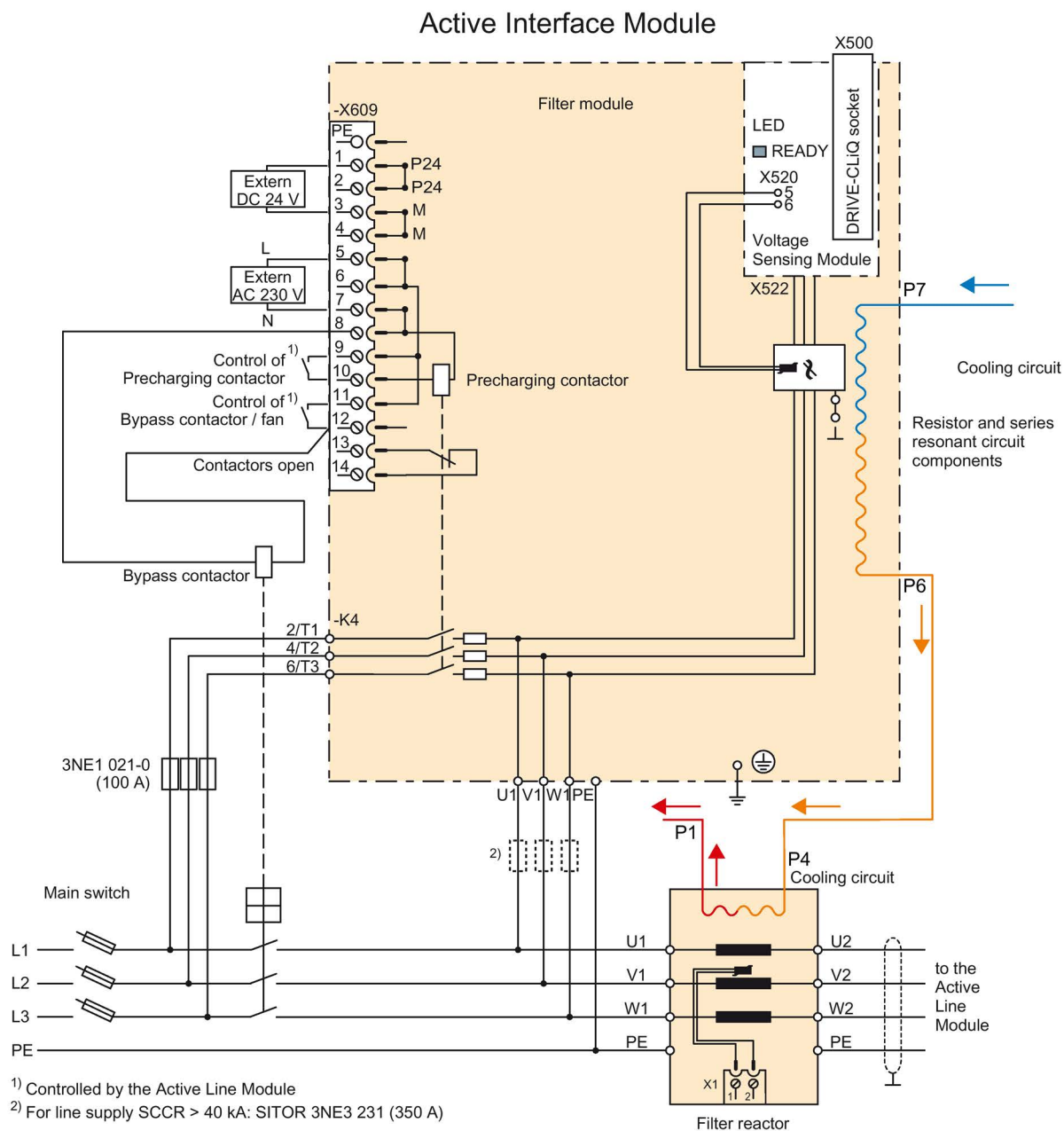
Figure 4-15 Connection example of liquid-cooled Active Interface Module, frame size JIL, valid for article numbers 6SL3305-7TE38-4AA5, 6SL3305-7TG37-4AA5, 6SL3305-7TG41-0AA5 and 6SL3305-7TG41-3AA5
