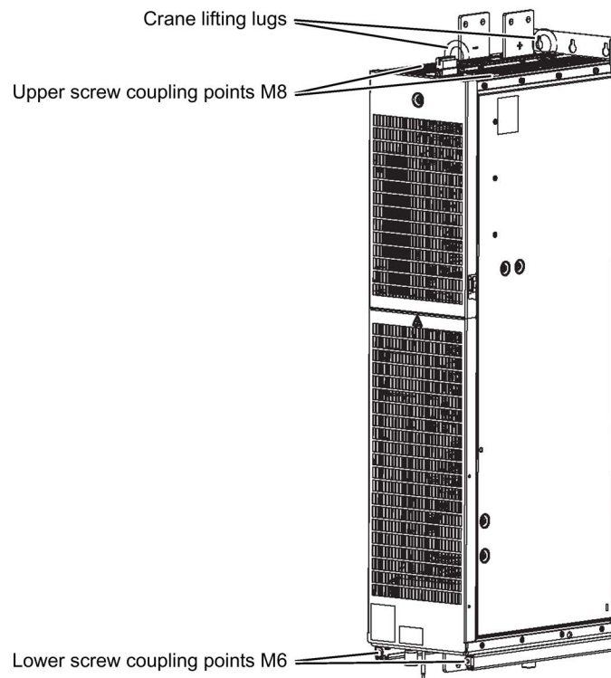
Figure 7-11 Crane lifting lugs / screw coupling points for mechanical support
