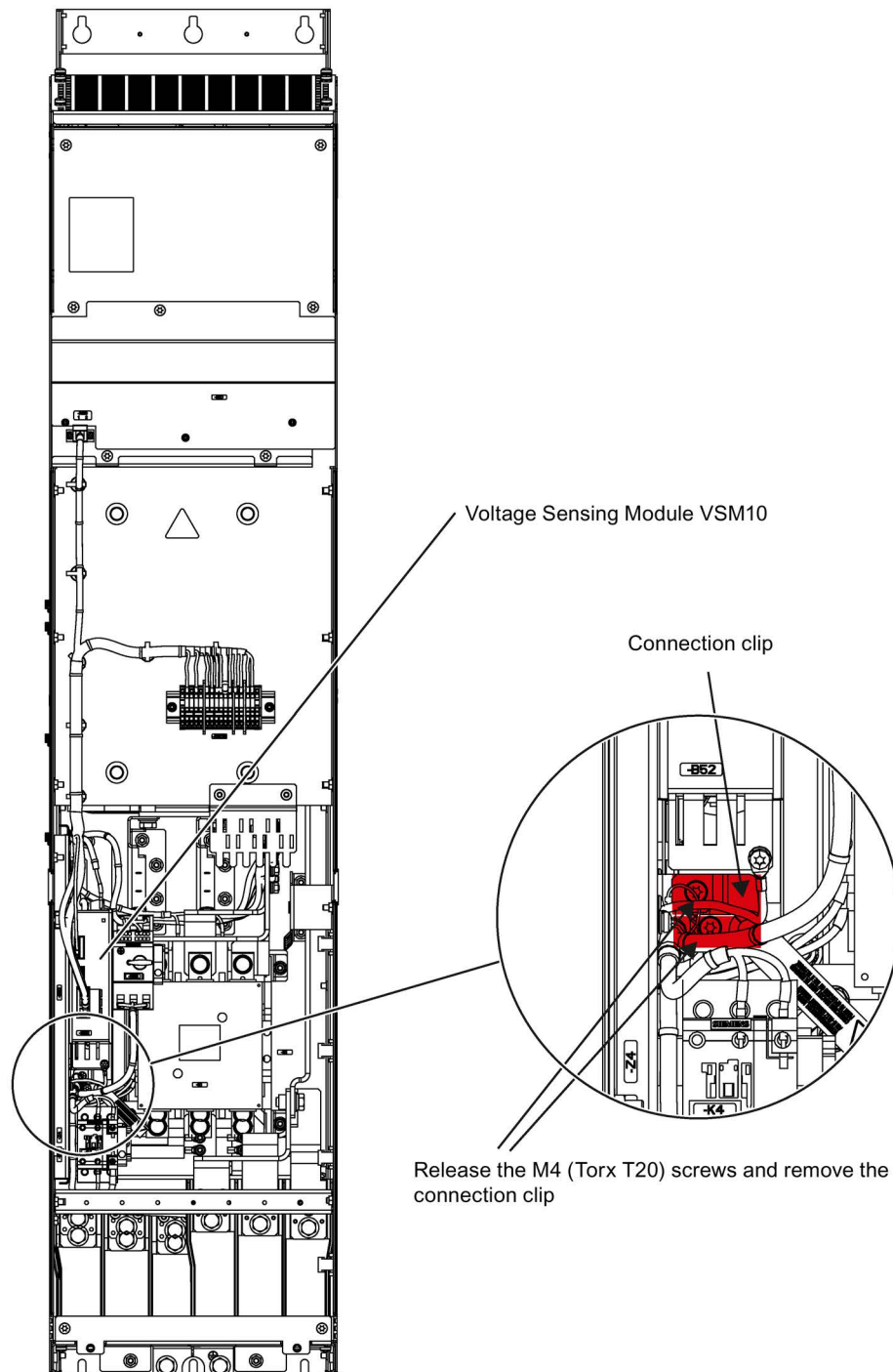
Figure 4-11 Removing the connection clip of the basic interference suppression module to ground for frame size G1
