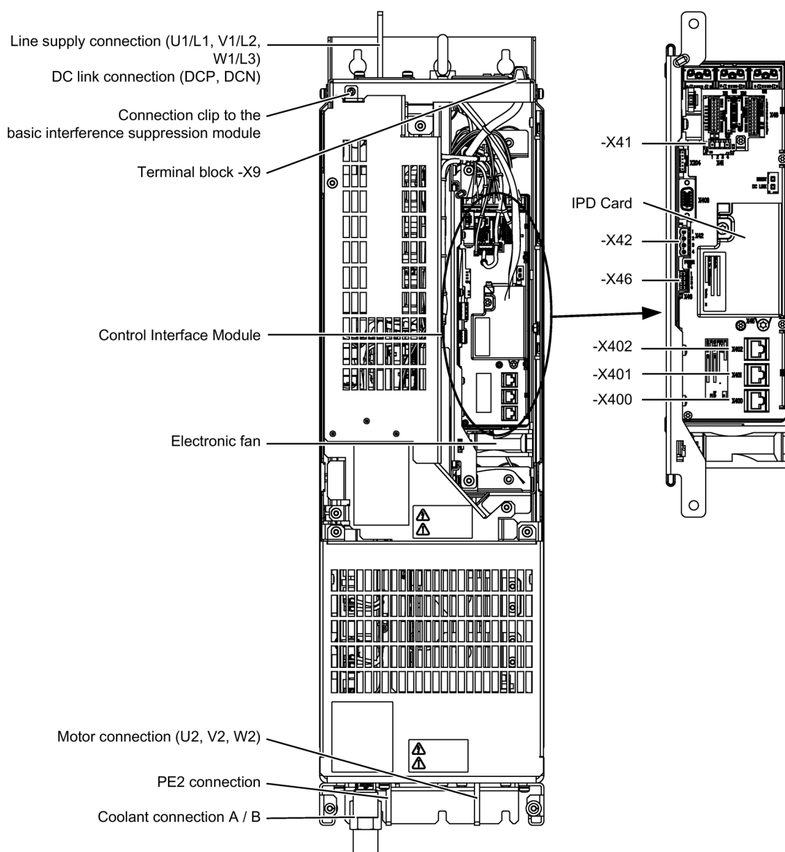
Figure 5-2 Power Module, frame size GL
