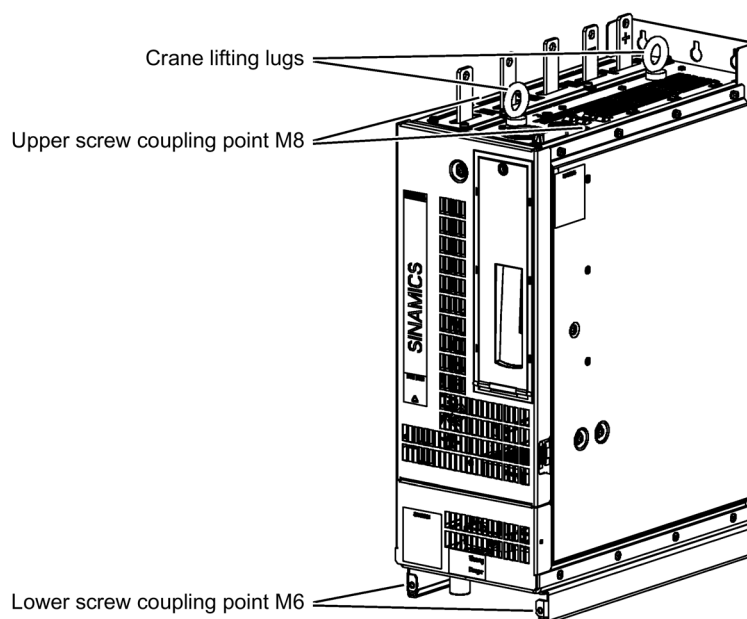
Figure 5-6 Crane lifting lugs / screw coupling points for mechanical support
