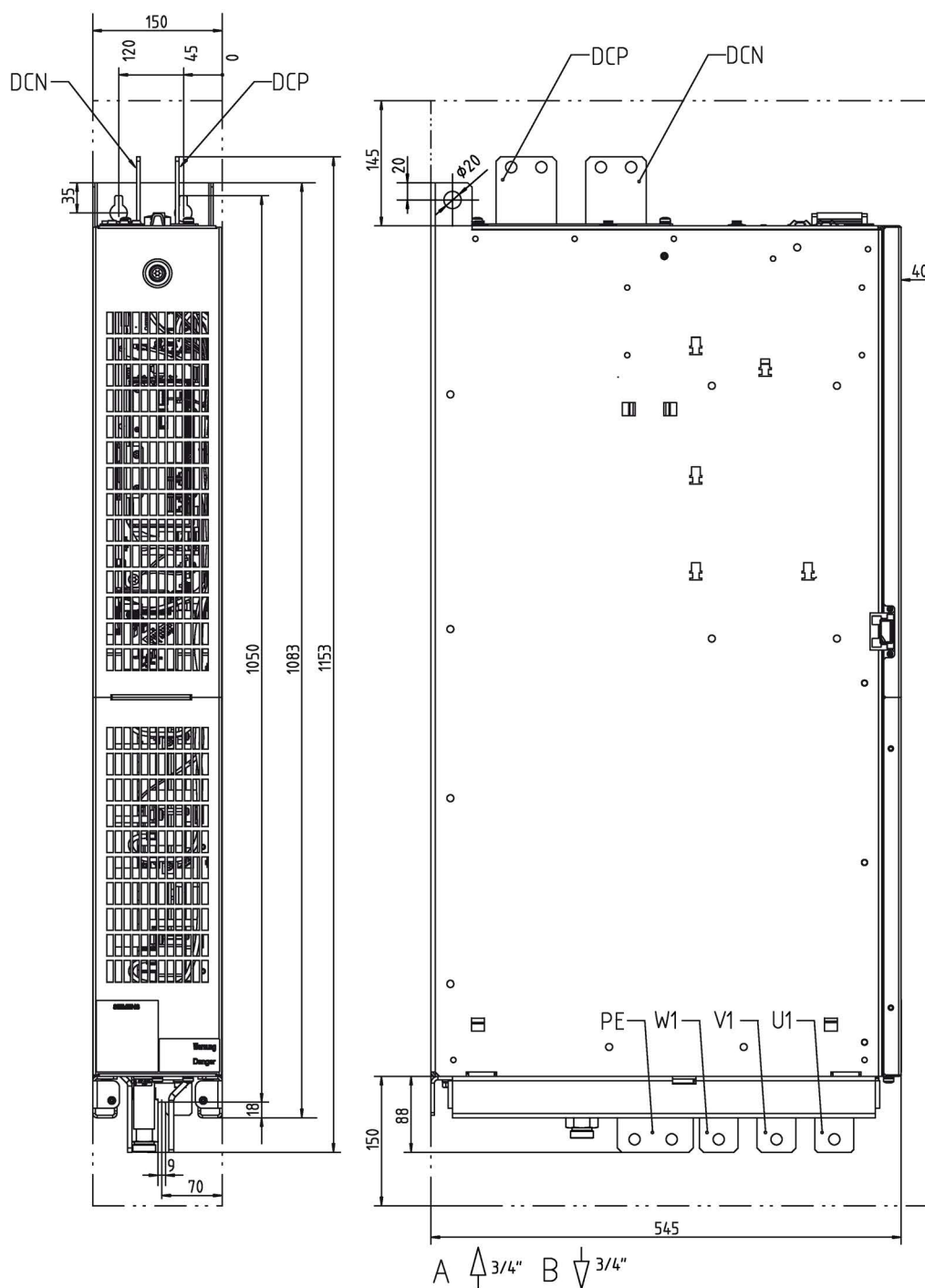
Figure 6-16 Dimension drawing Active Line Module, frame size GXL Front view, side view
