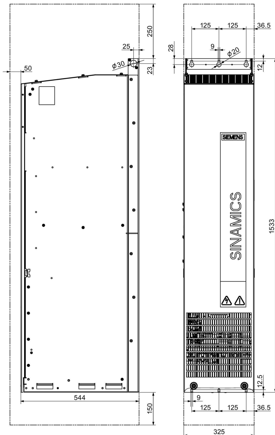
Figure 4-8 Dimension drawing for Active Interface Module, frame size G1 Side view, front view
