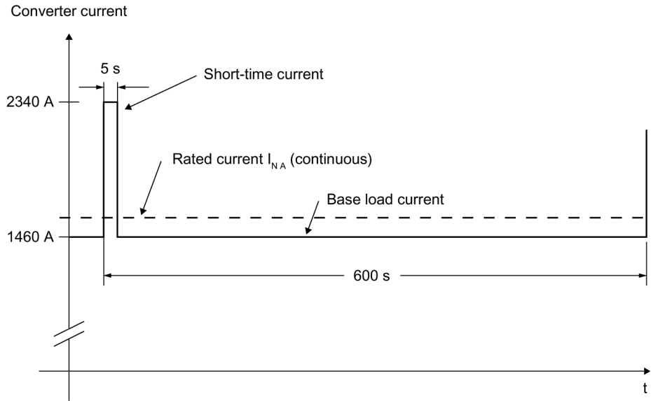
Figure 7-15 High overload for Motor Module 6SL3325-1TG41-6AP3
