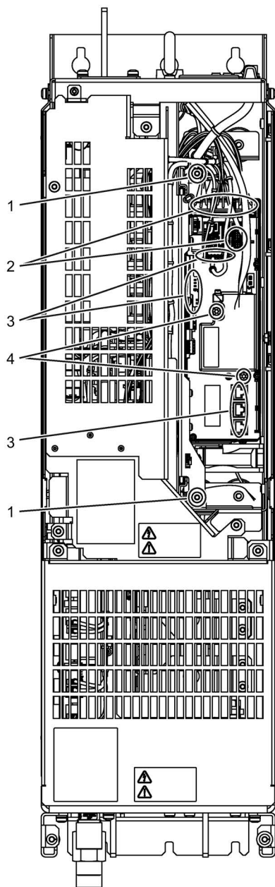
Figure 11-14 Replacing the electronic fan, Power Module, frame size GL
