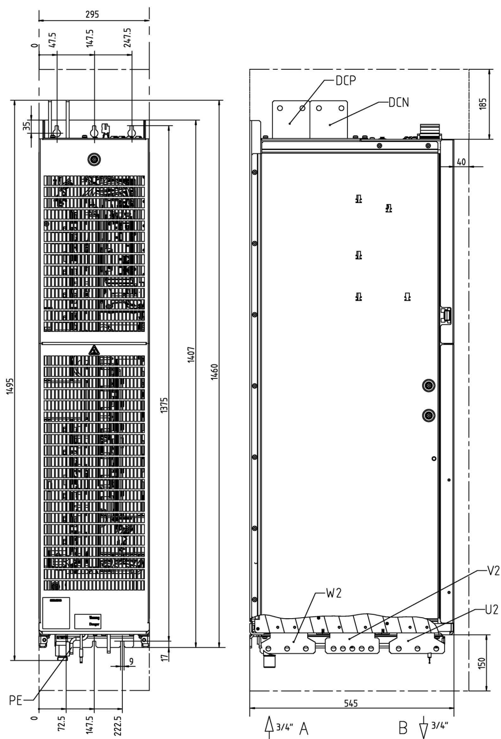
Figure 7-10 Dimension drawing Motor Module, frame size JXL, article numbers 6SL3325-1TE41-4AS3, 6SL3325-1TG41-6AA3. Front view, side view
