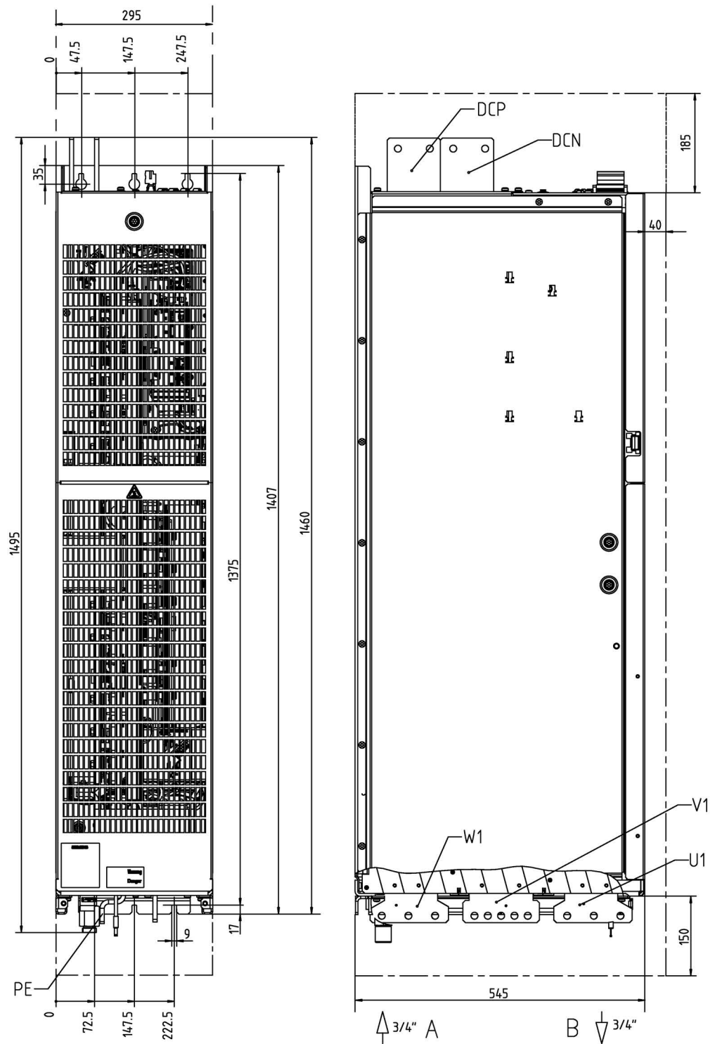
Figure 6-19 Dimension drawing Active Line Module, frame size JXL, article number 6SL3335-7TG41-6AA3. Front view, side view
