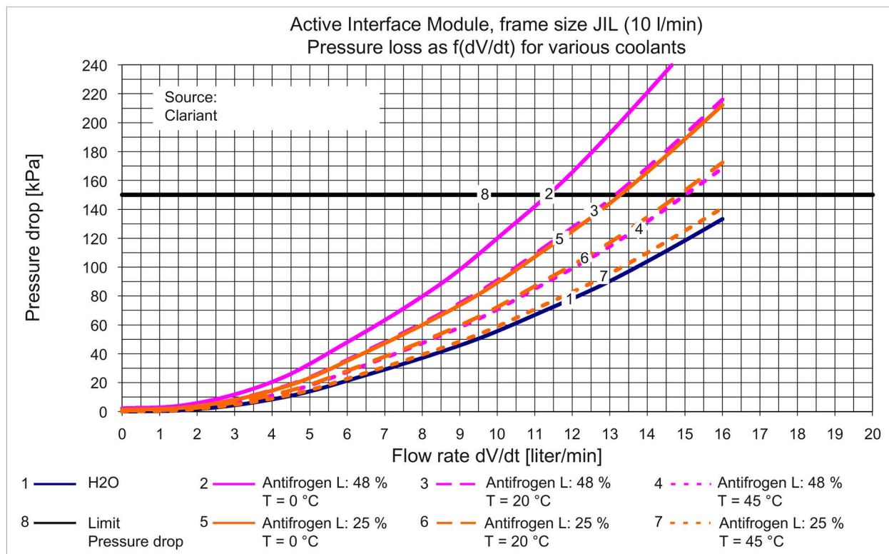
Figure 10-19 Pressure drop as a function of volumetric flow for Active Interface Module, frame size JIL, 10 l/min
