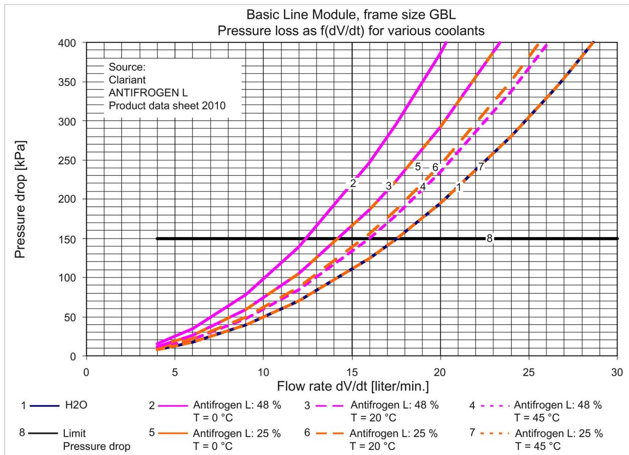
Figure 10-14 Pressure drop as a function of volumetric flow for Basic Line Module, frame size GBL
