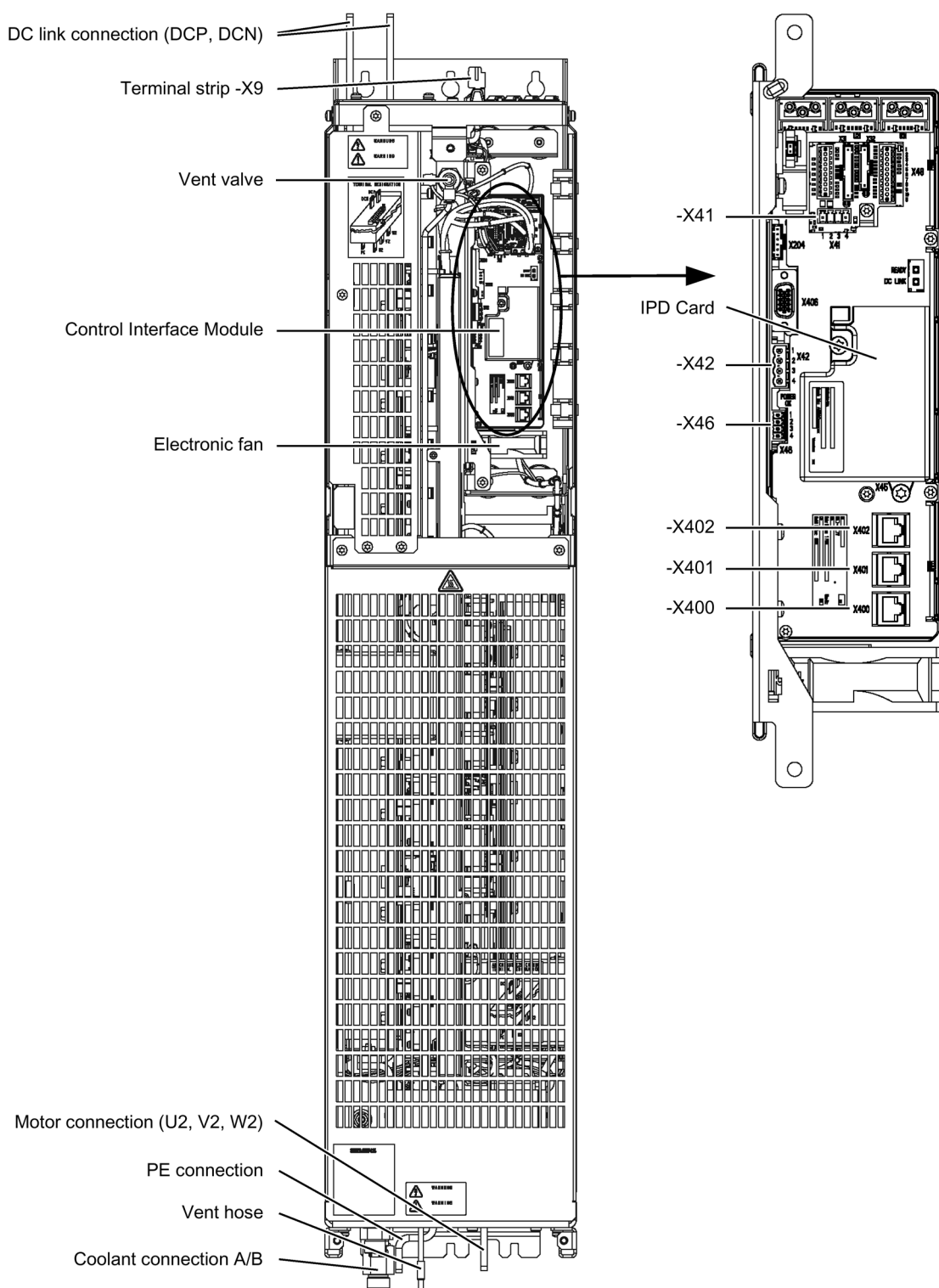
Figure 7-4 Motor Module, frame size JXL
