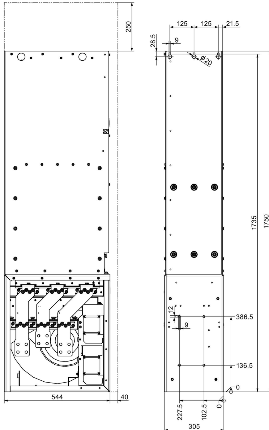
Figure 4-9 Dimension drawing for Active Interface Module, frame size HI Side view, rear view
