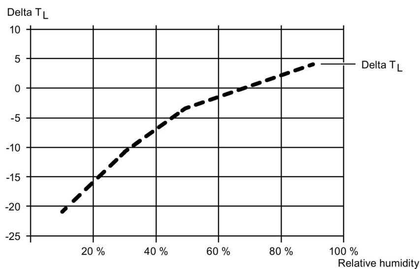
Figure 10-23 Curve to determine the temperature \Delta T_L
