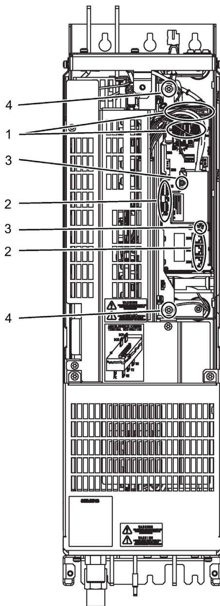
Figure 11-17 Replacing the electronic fan, Active Line Module, and Motor Module, frame size HXL
