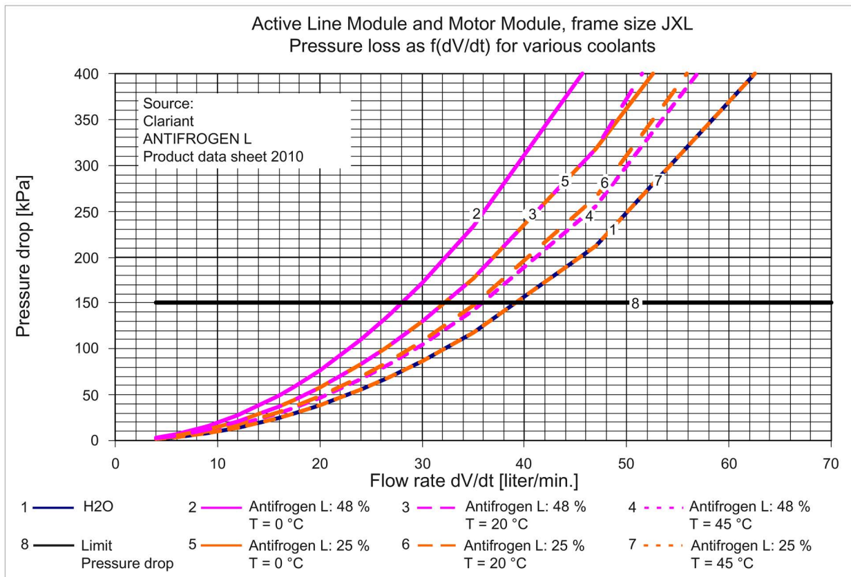
Figure 10-18 Pressure drop as a function of volumetric flow for Active Line Module and Motor Module, frame size JXL
