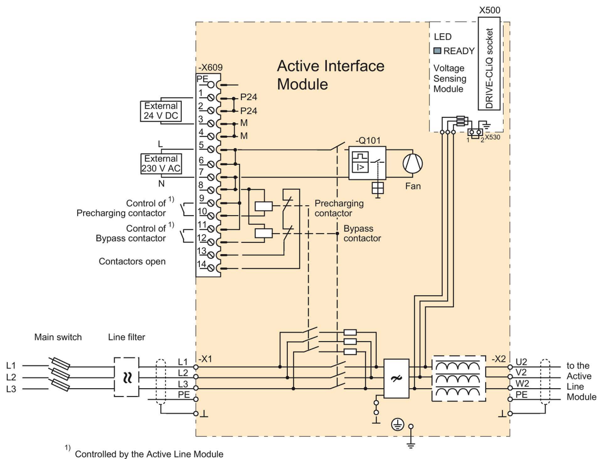
Figure 4-5 Connection example Active Interface Module, frame size GI
