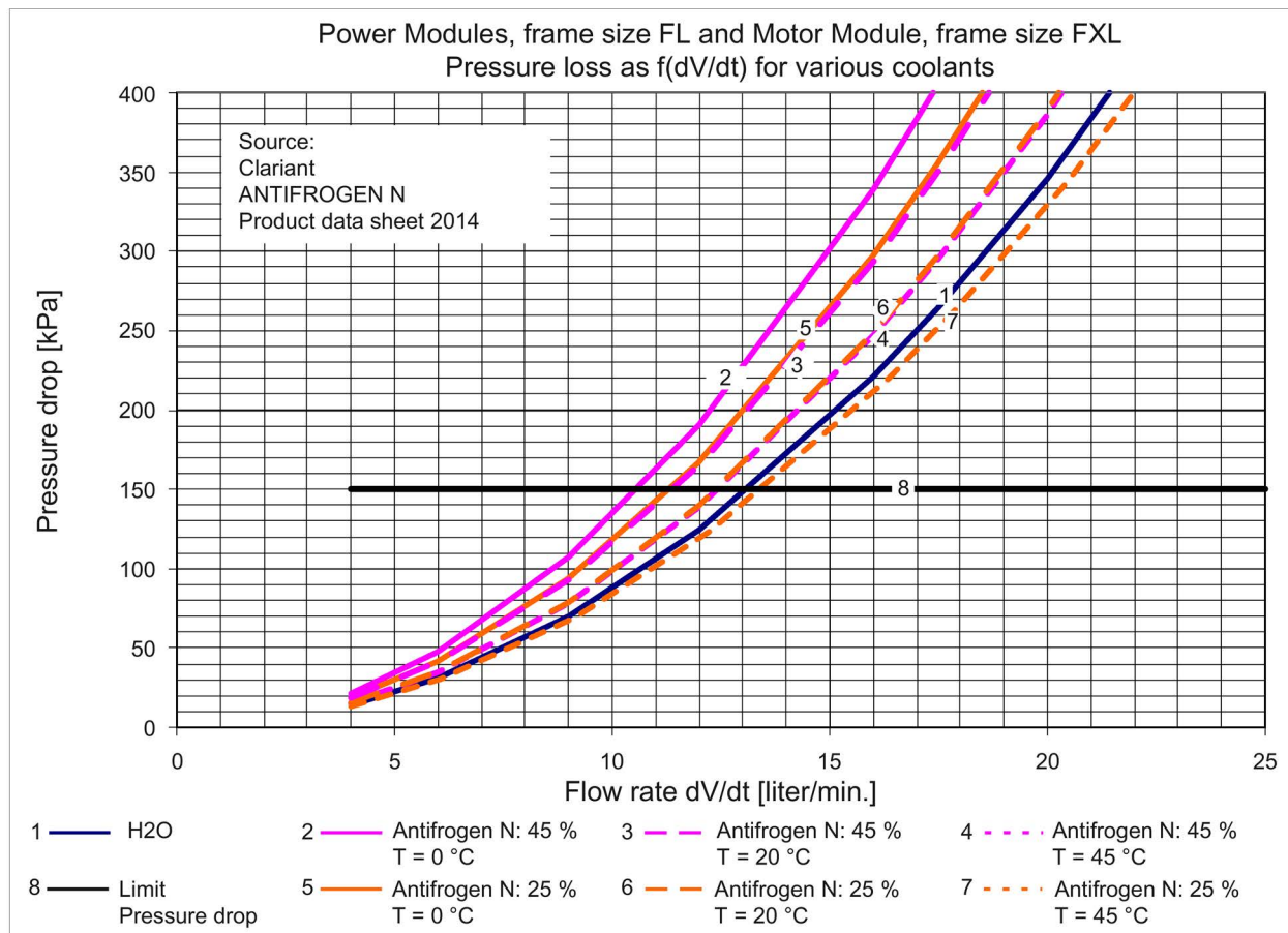
Figure 10-7 Pressure drop as a function of volumetric flow for Power Module frame size FL, and Motor Module frame size FXL
