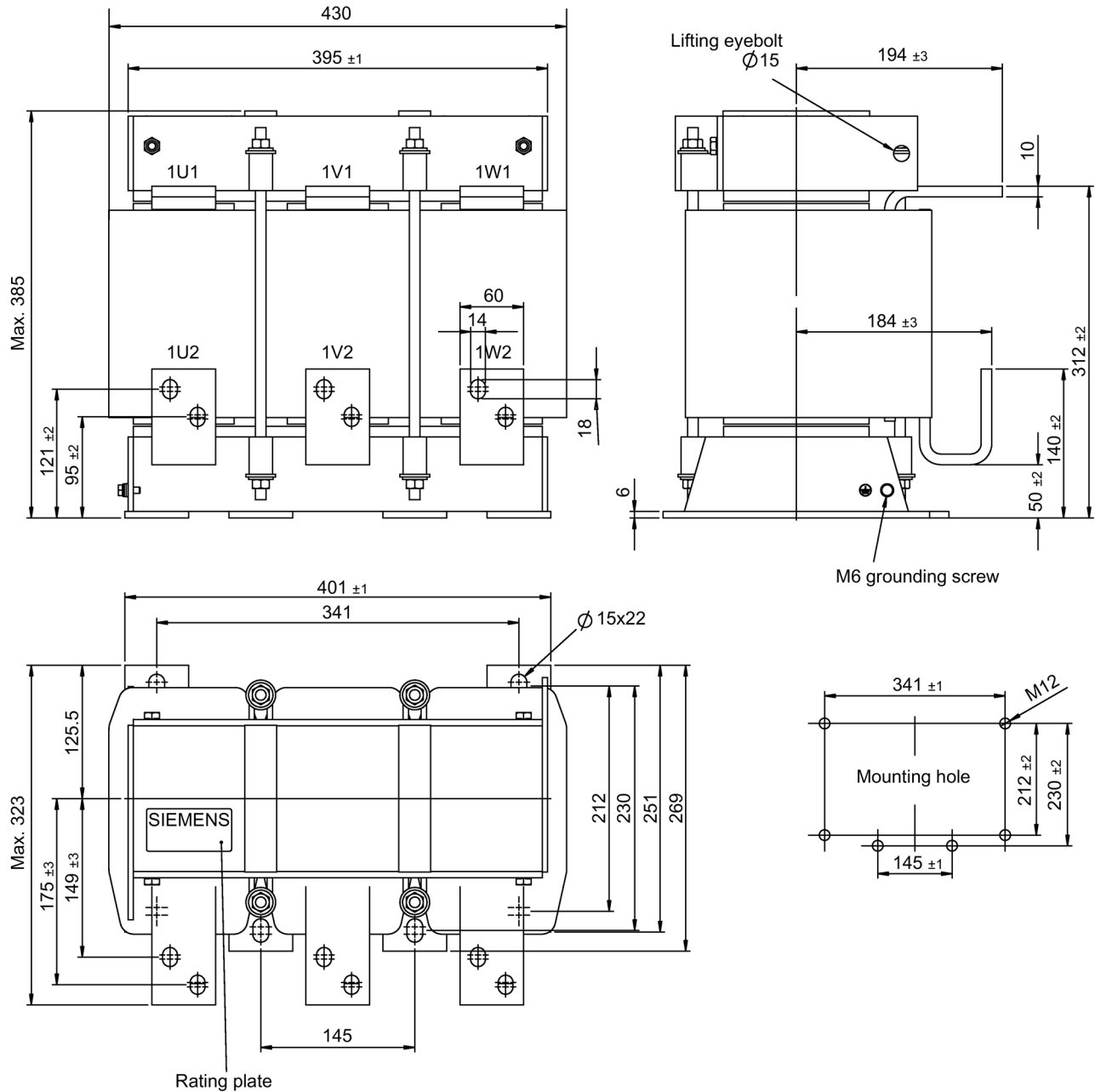
Figure 8-23 Dimension drawing for dV/dt filter compact plus voltage peak limiter, type 4 dV/dt reactor
