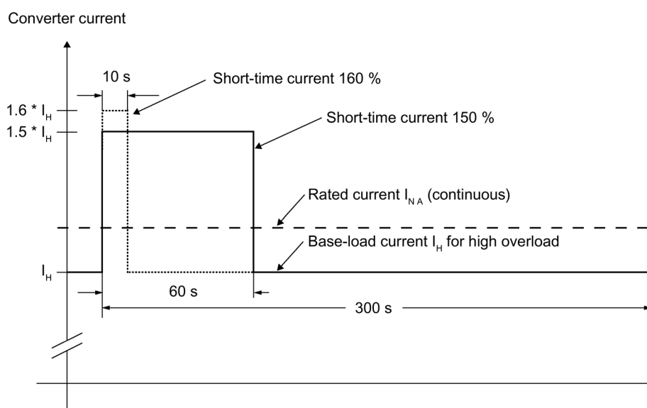
Figure 5-10 High overload
