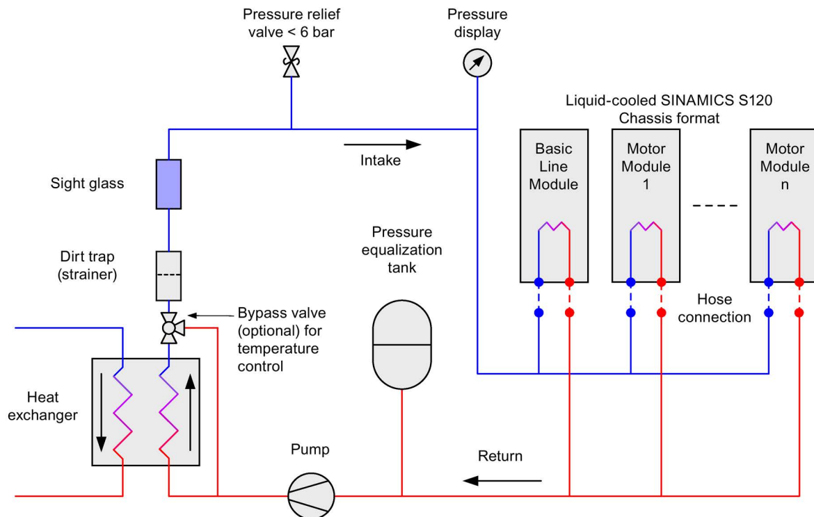
Figure 10-1 Recommendation for closed circuit
