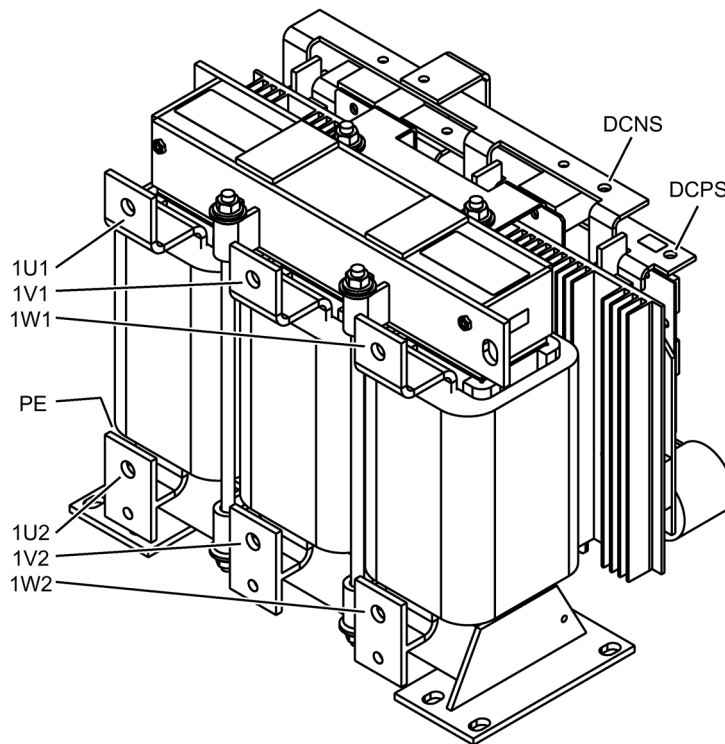
Figure 8-15 Interface overview for dv/dt filter compact plus Voltage Peak Limiter, Type 3
