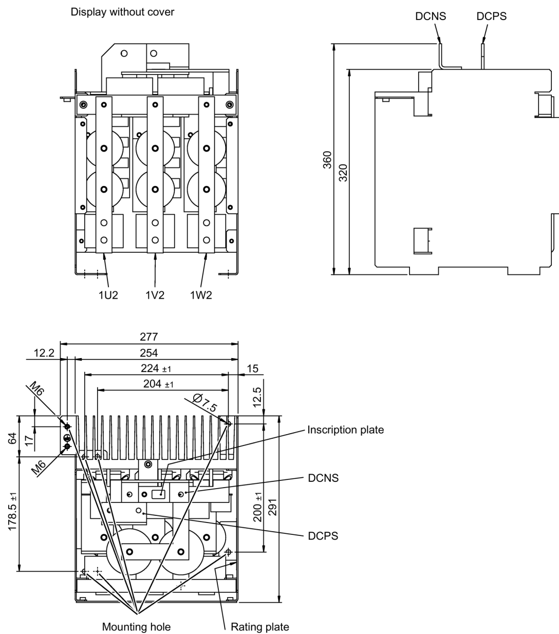
Figure 8-24 Dimension drawing for dv/dt filter compact plus voltage peak limiter, type 4 Voltage peak limiter
