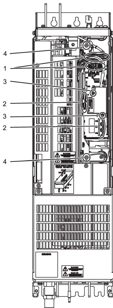
Figure 11-6 Replacing the Control Interface Module, Active Line Module and Motor Module, frame size HXL
