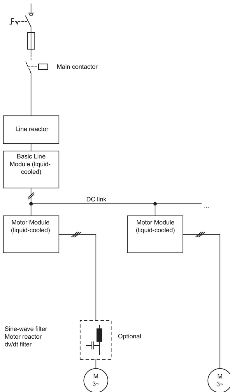
Figure 3-8 Basic structure of a drive system with liquid-cooled SINAMICS S120 and unregulated infeed
