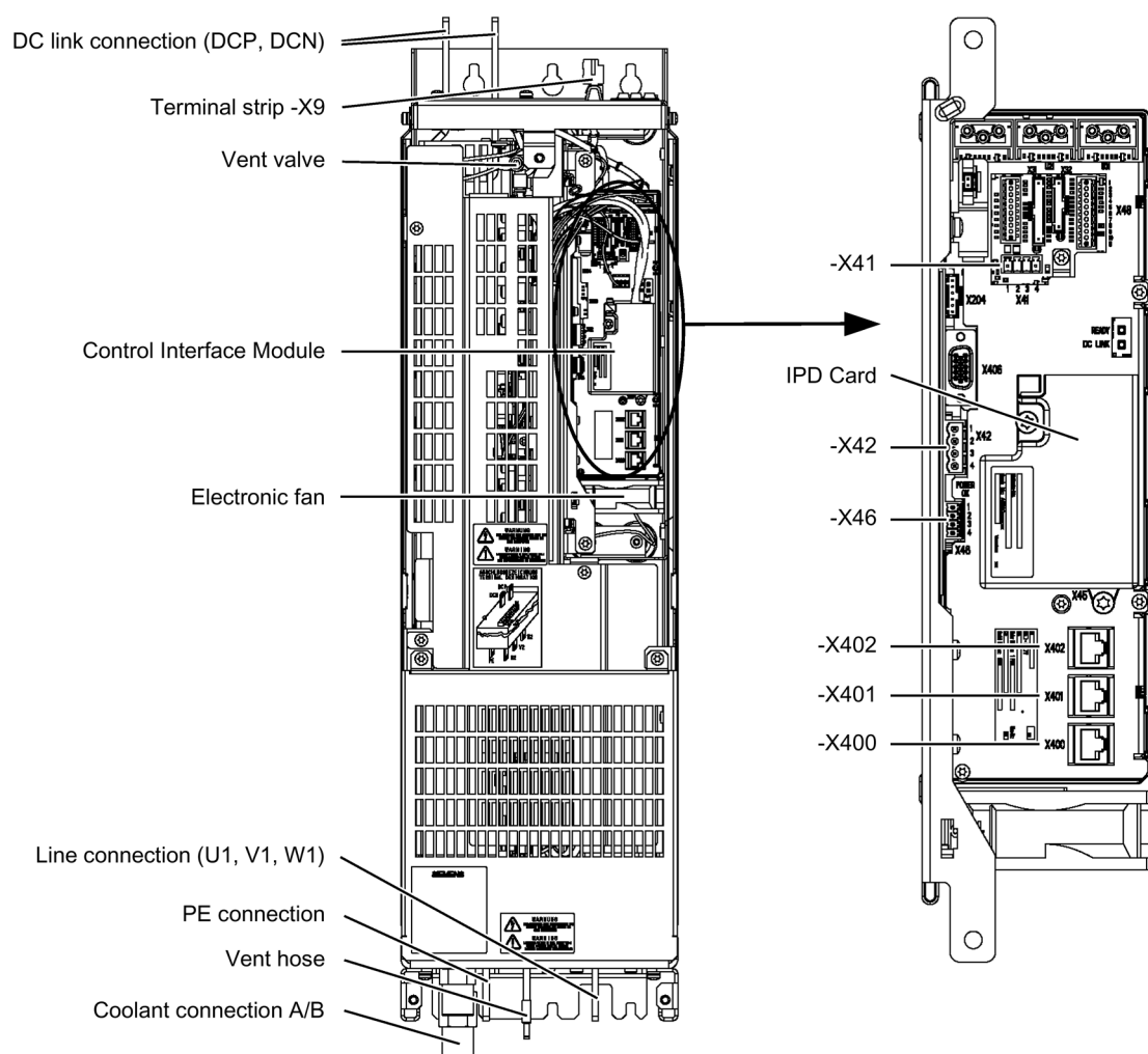
Figure 6-13 Active Line Module, frame size HXL
