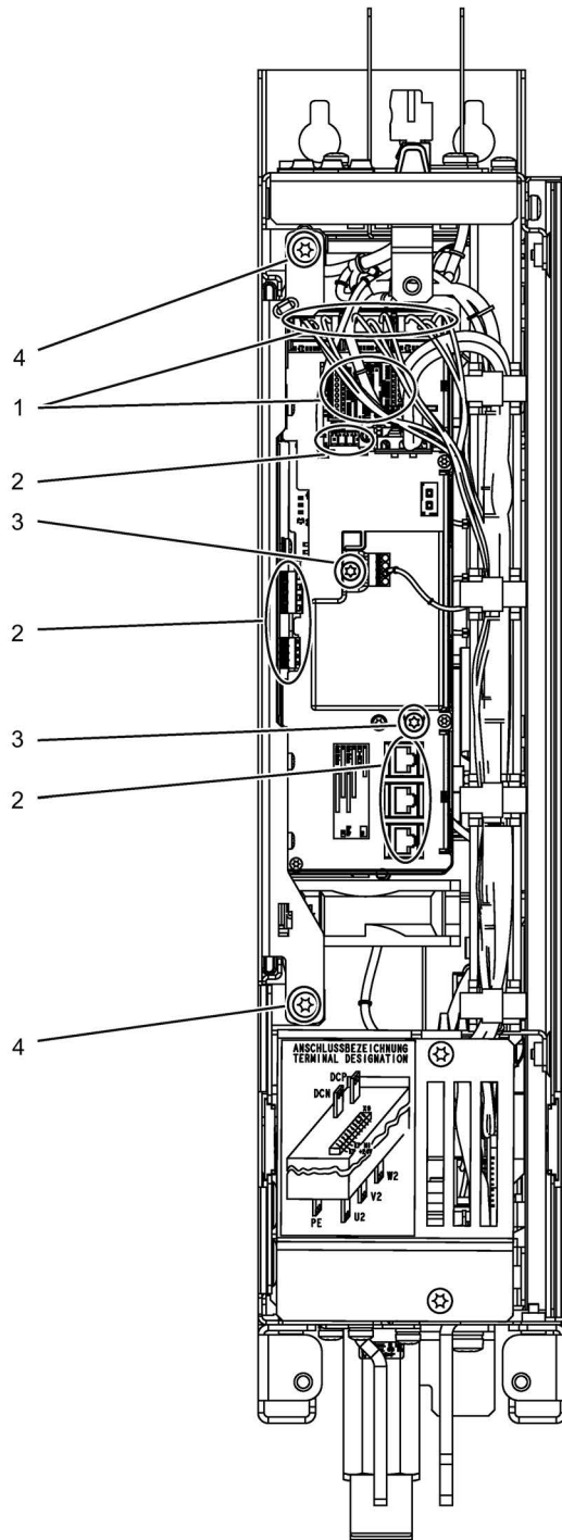
Figure 11-15 Replacing the electronic fan, Motor Module, frame size FXL
