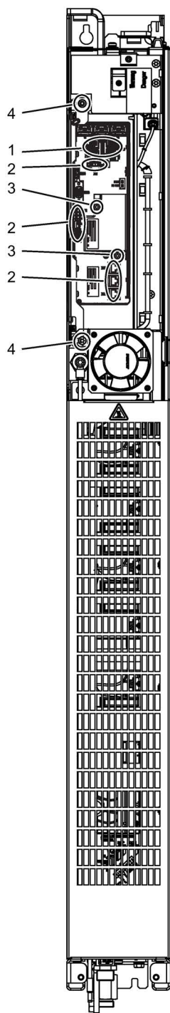
Figure 11-12 Replacing the Control Interface Module, Basic Line Module, frame size GBL
