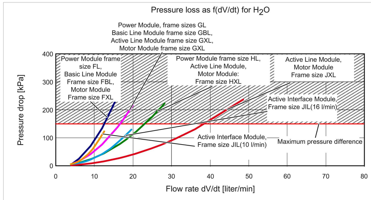
Figure 10-4 Pressure drop as a function of volumetric flow
