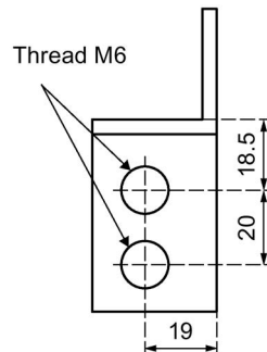
Figure 9-2 Bolting points for the mounting rails (dimensions in mm)
