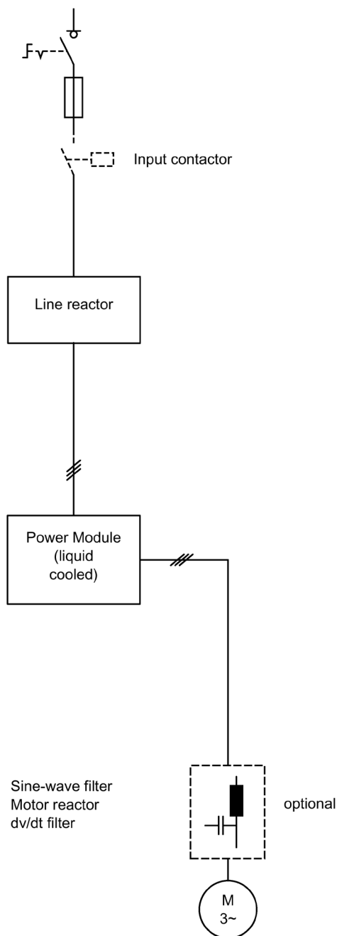
Figure 3-6 Principle structure of a drive system with liquid-cooled SINAMICS S120 Power Modules
