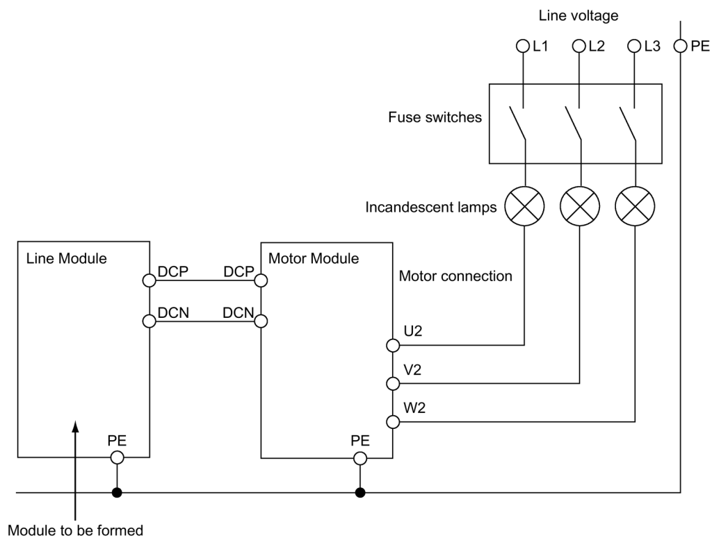
Figure 11-25 Forming circuit for Line Modules
