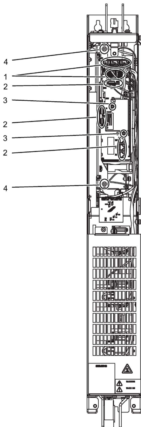
Figure 11-16 Replacing the electronic fan, Active Line Module, and Motor Module, frame size GXL
