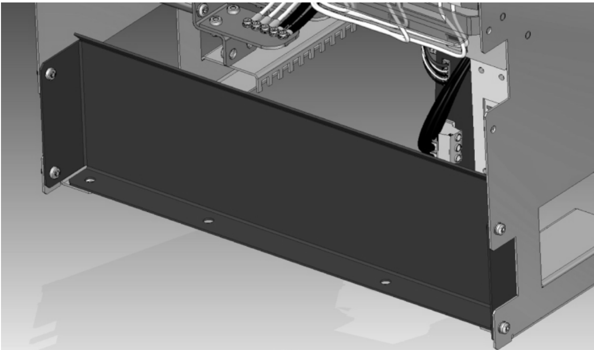
Figure 4-20 Transport plate on the underside of the filter module
