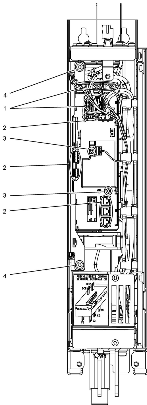
Figure 11-4 Replacing the Control Interface Module, Motor Module, frame size FXL
