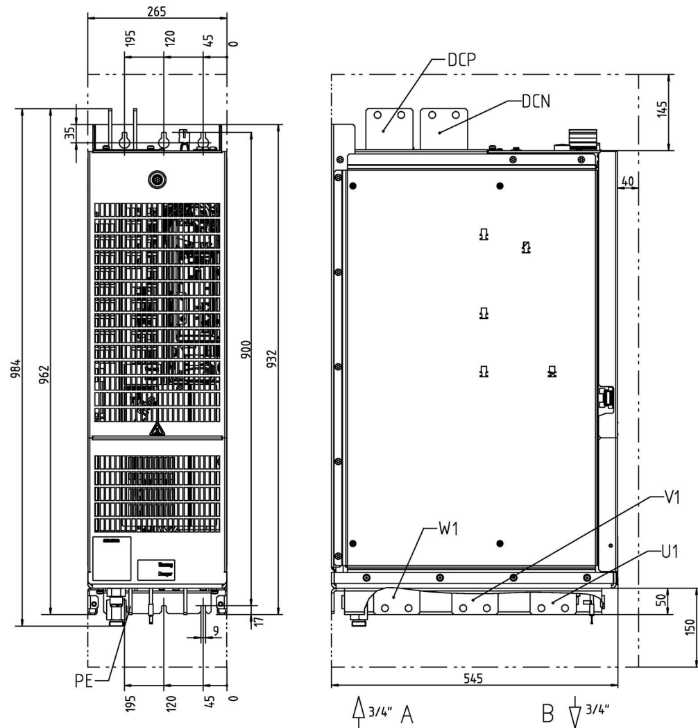
Figure 6-17 Dimension drawing Active Line Module, frame size HXL Front view, side view
