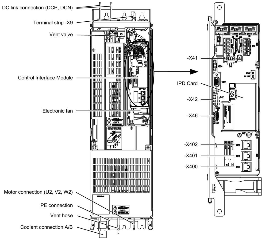
Figure 7-3 Motor Module, frame size HXL
