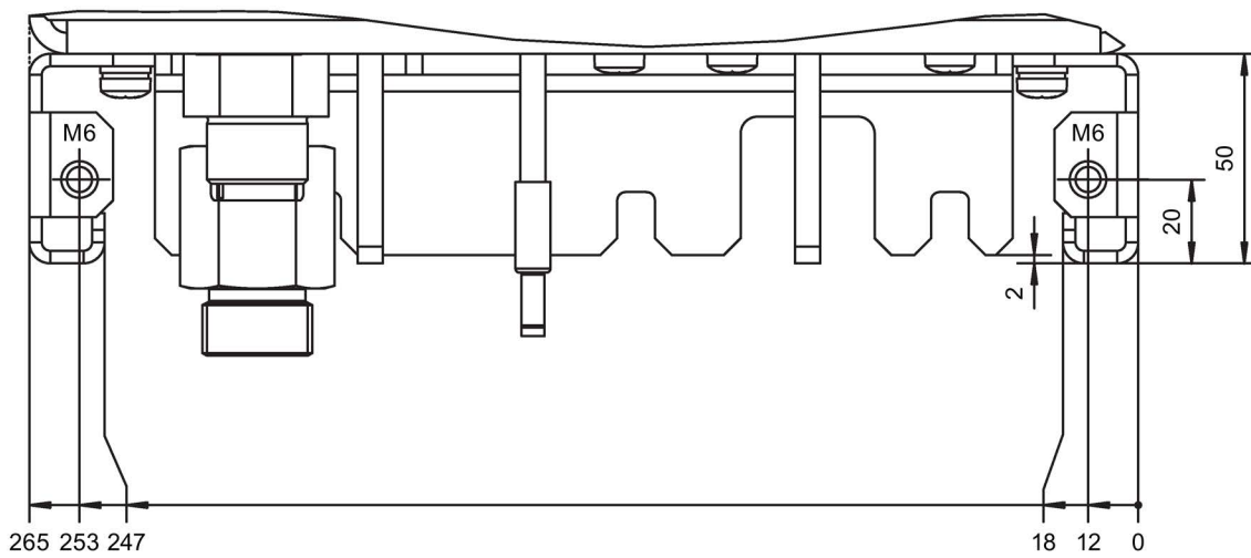
Figure 9-7 Rail profile, Active Line Module and Motor Module, frame size HXL (dimension data in mm)
