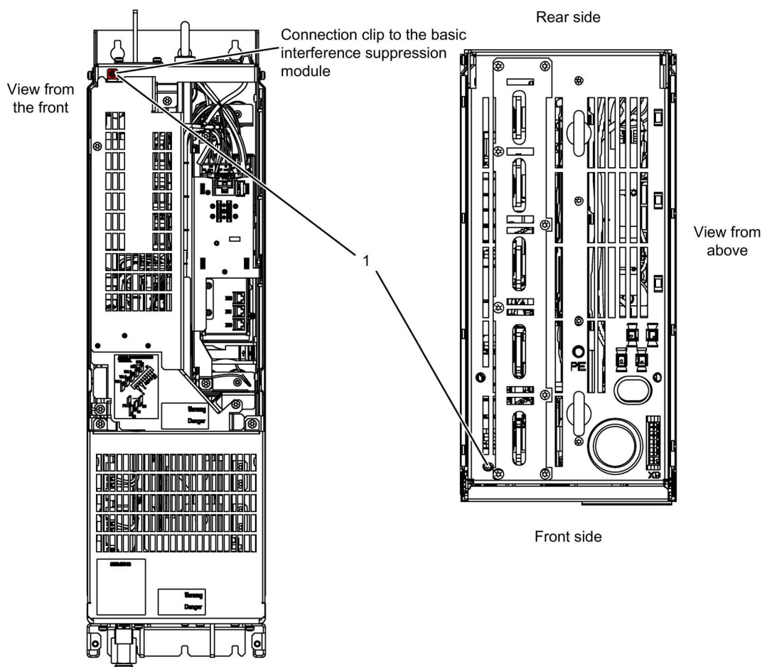
Figure 5-8 Removing the connection clip of the basic interference suppression module to ground
