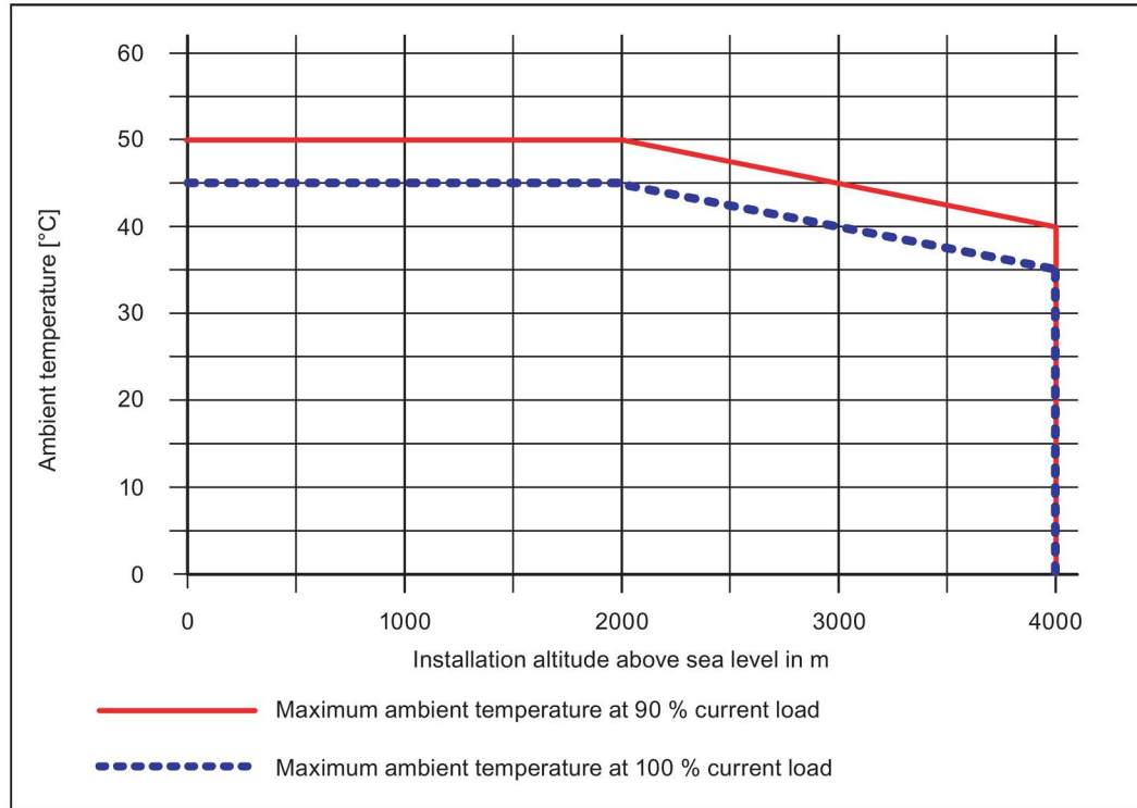
Figure 3-5 Maximum ambient temperature as a function of installation altitude
