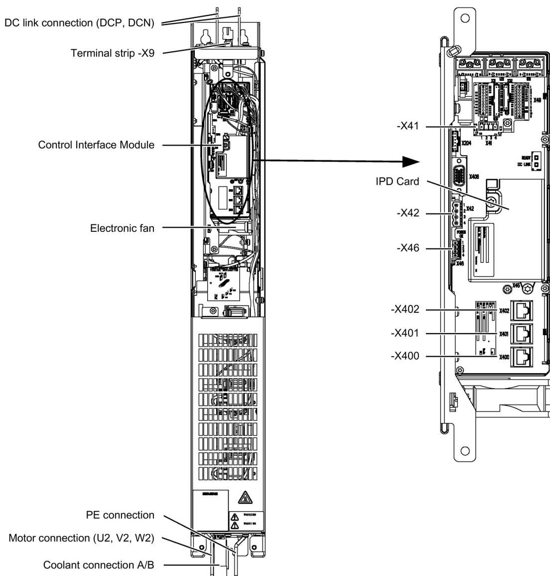
Figure 7-2 Motor Module, frame size GXL
