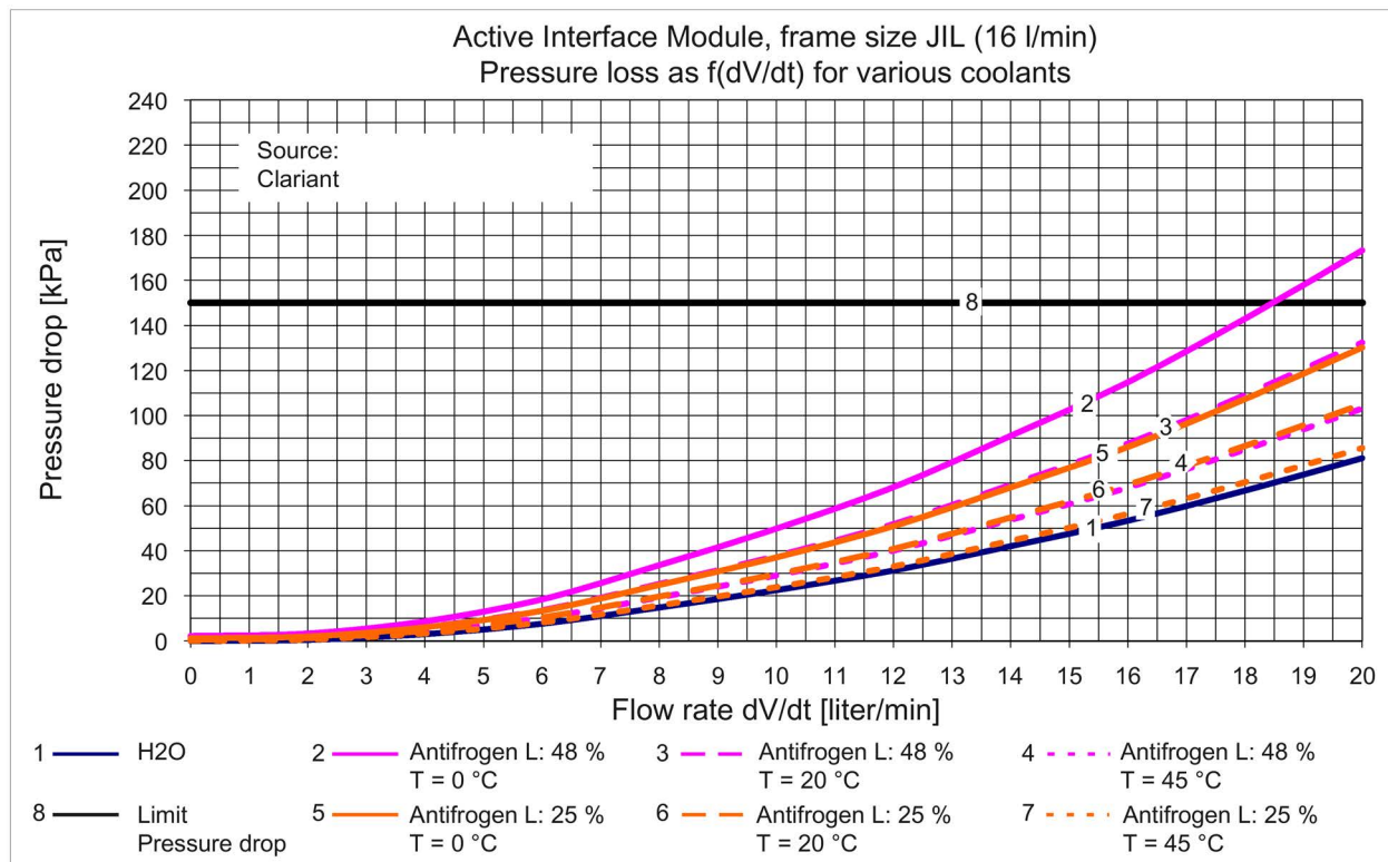
Figure 10-20 Pressure drop as a function of volumetric flow for Active Interface Module, frame size JIL, 16 l/min
