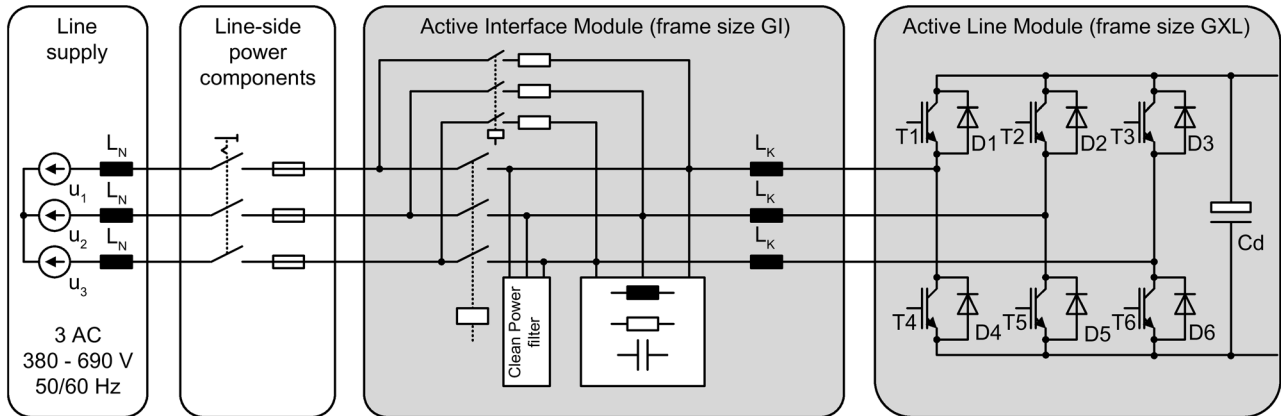
Figure 6-10 Overview of Active Infeeds, frame size GXL
