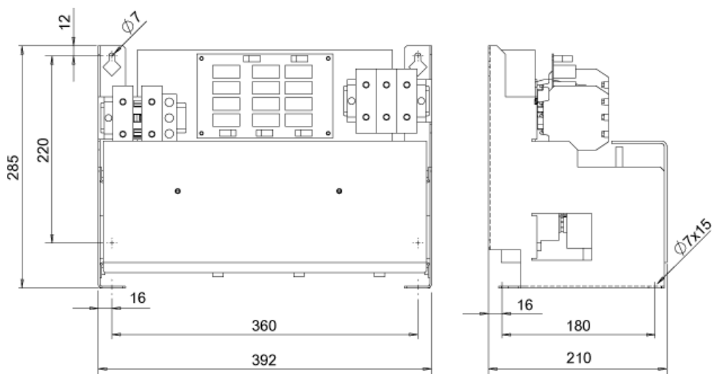
Figure 8-11 Dimension drawing of the voltage peak limiter, type 2
