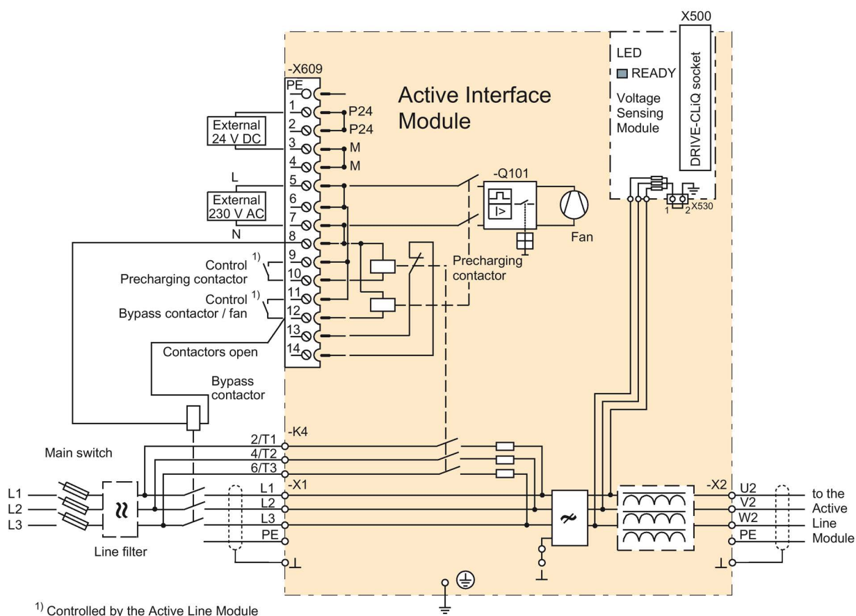
Figure 4-6 Connection example Active Interface Module, frame size HI
