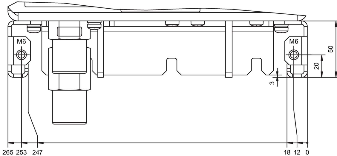
Figure 9-3 Rail profile, Power Modules, frame sizes FL, GL (dimensions in mm)
