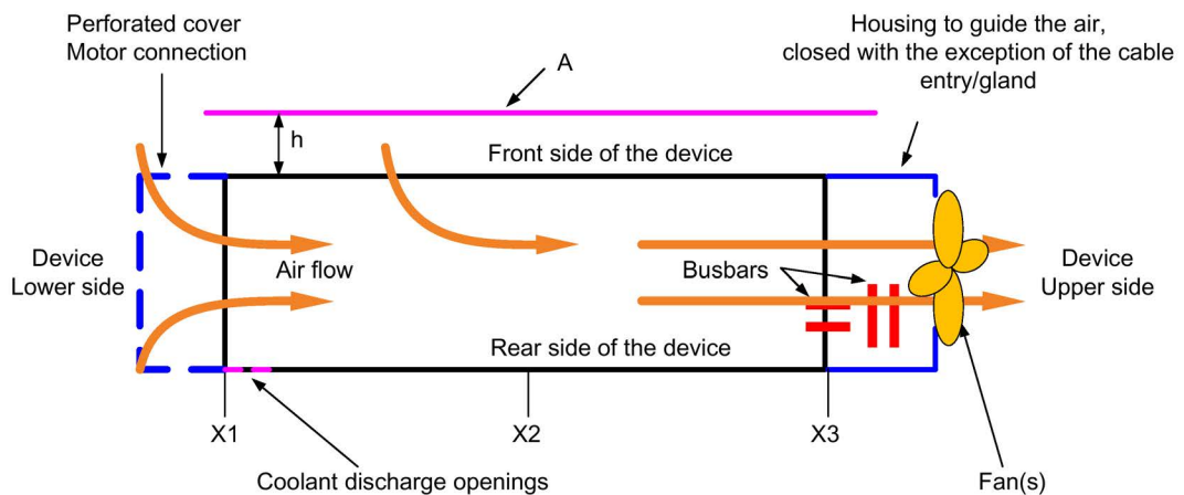
Figure 9-9 Basic layout for horizontal installation position (side view)
