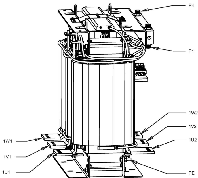
Figure 4-13 Interface overview filter reactor, size JIL, valid for article numbers 6SL3005-ODE38-4AA0, 6SL3005-ODG37-4AA0 and 6SL3005-ODG41-3AA0
