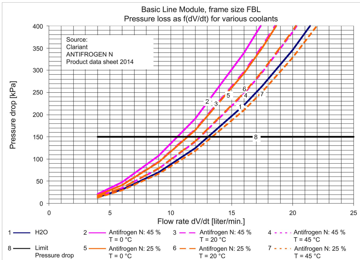
Figure 10-5 Pressure drop as a function of volumetric flow for Basic Line Module, frame size FBL
