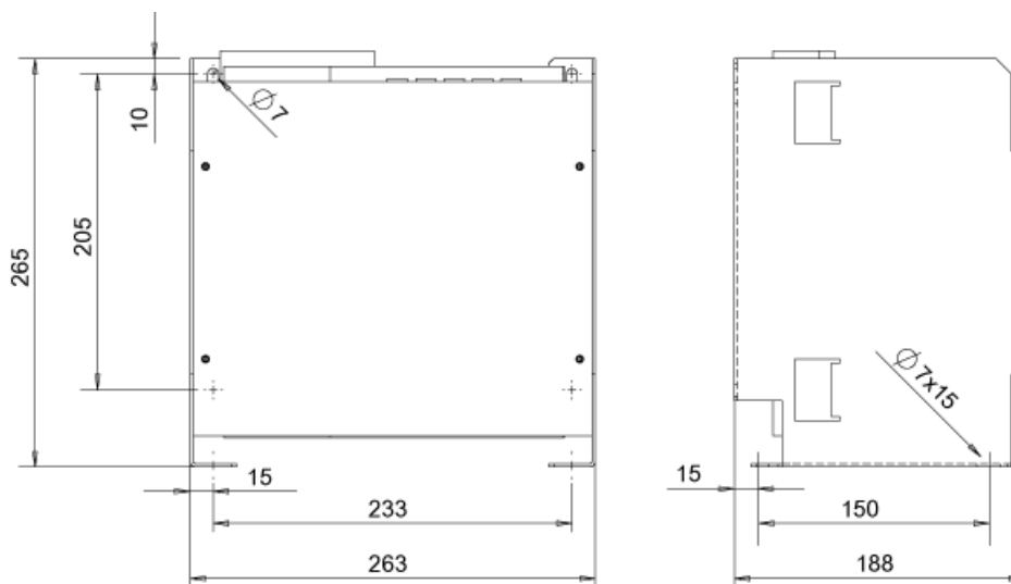
Figure 8-10 Dimension drawing of the voltage peak limiter, type 1
