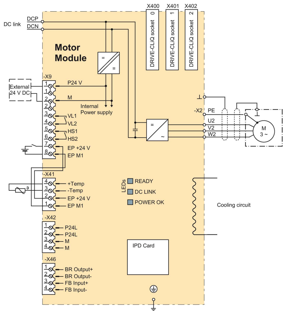
Figure 7-5 Connection example Motor Module
