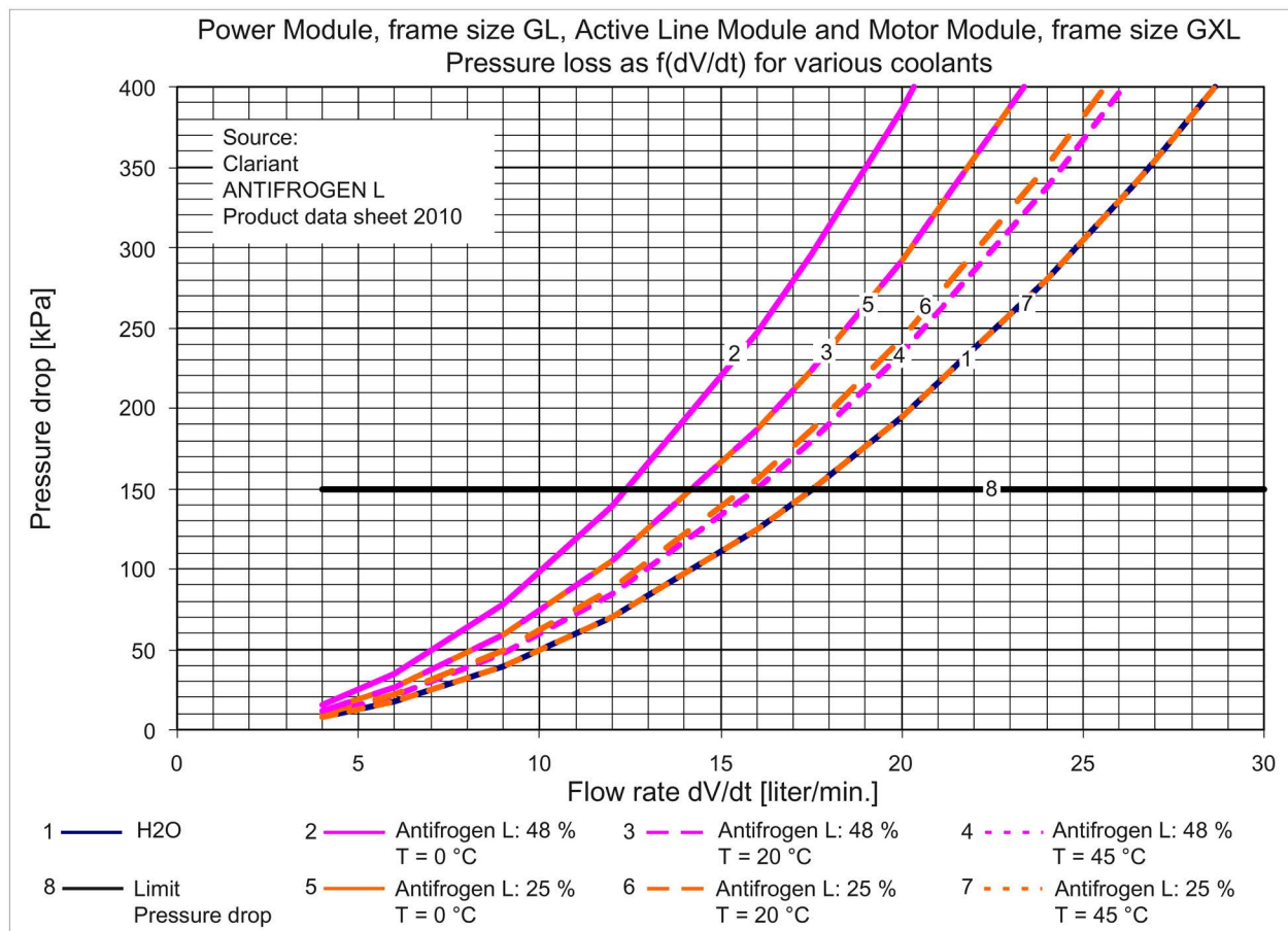
Figure 10-16 Pressure drop as a function of volumetric flow for Power Module frame size GL, Active Line Module and Motor Module frame size GXL
