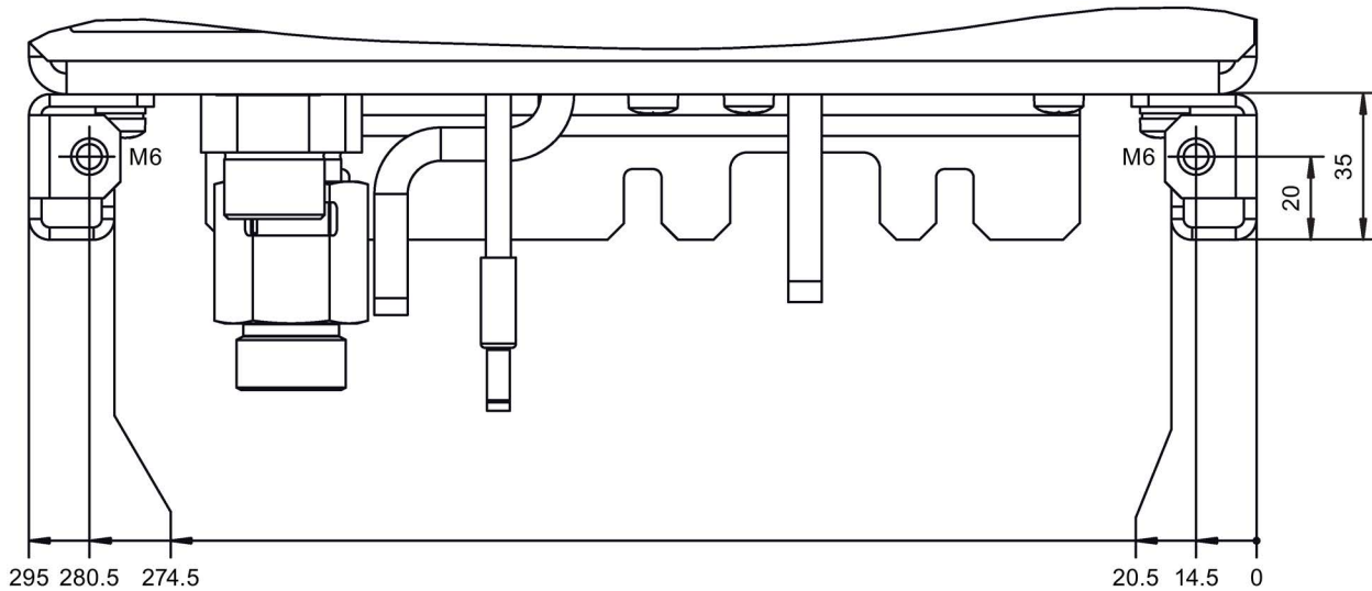
Figure 9-8 Rail profile, Active Line Module and Motor Module, frame size JXL, (dimensions in mm)
