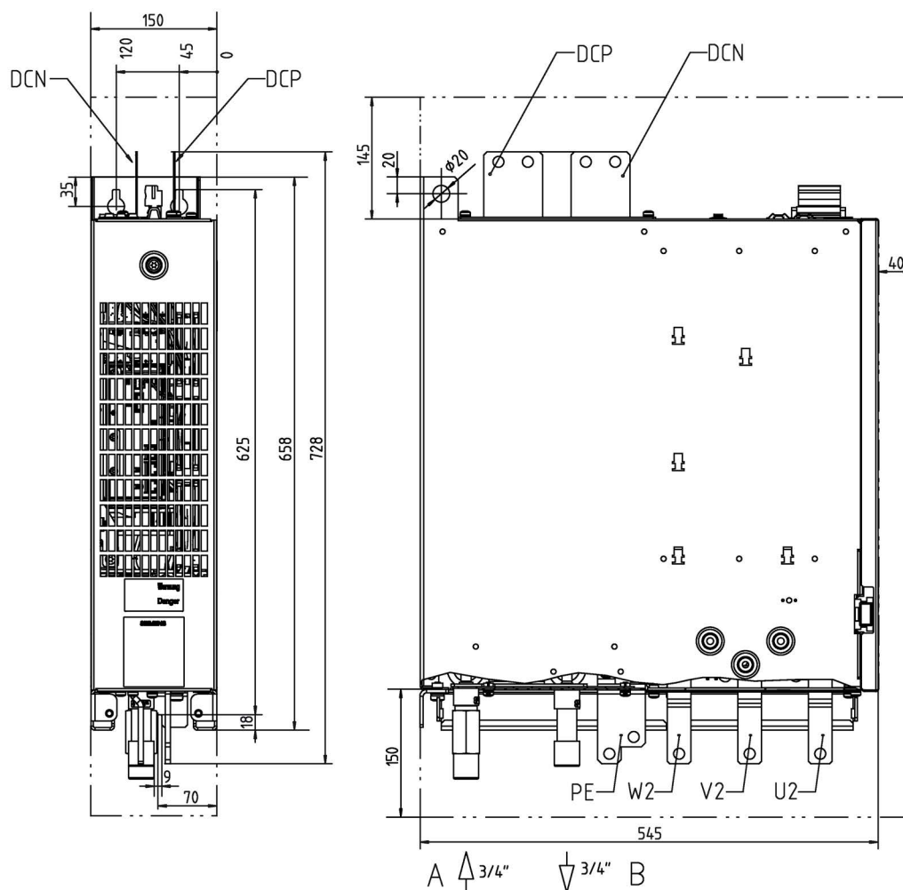
Figure 7-6 Dimension drawing Motor Module, frame size FXL. Front view, side view
