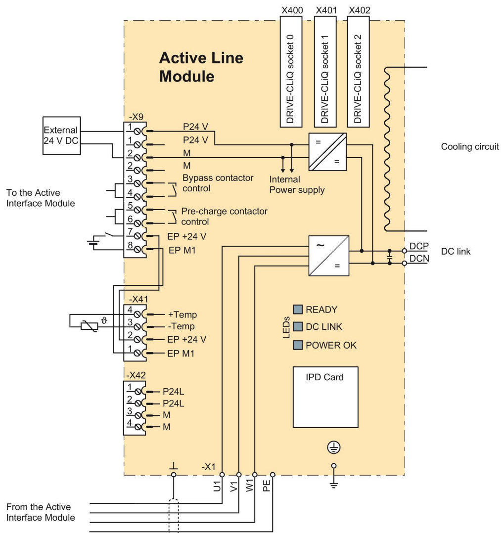
Figure 6-15 Example connection of Active Line Module
