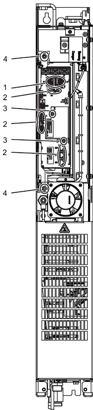
Figure 11-19 Replacing the electronic fan, Basic Line Module, frame size FBL
