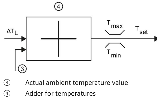
Figure 10-25 Formation of the setpoint depending on the ambient temperature
