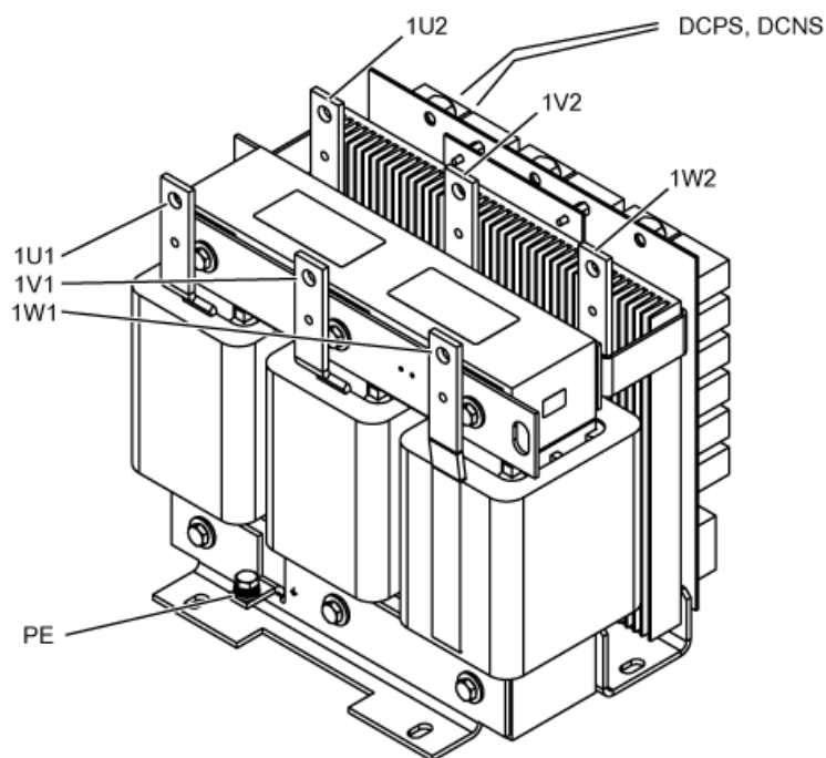
Figure 8-14 Interface overview for dv/dt filter compact plus Voltage Peak Limiter, Type 2
