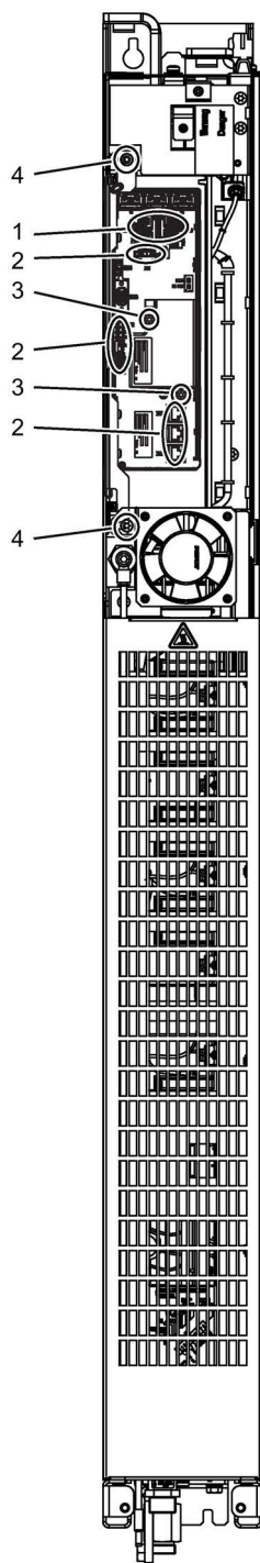
Figure 11-20 Replacing the electronic fan, Basic Line Module, frame size GBL
