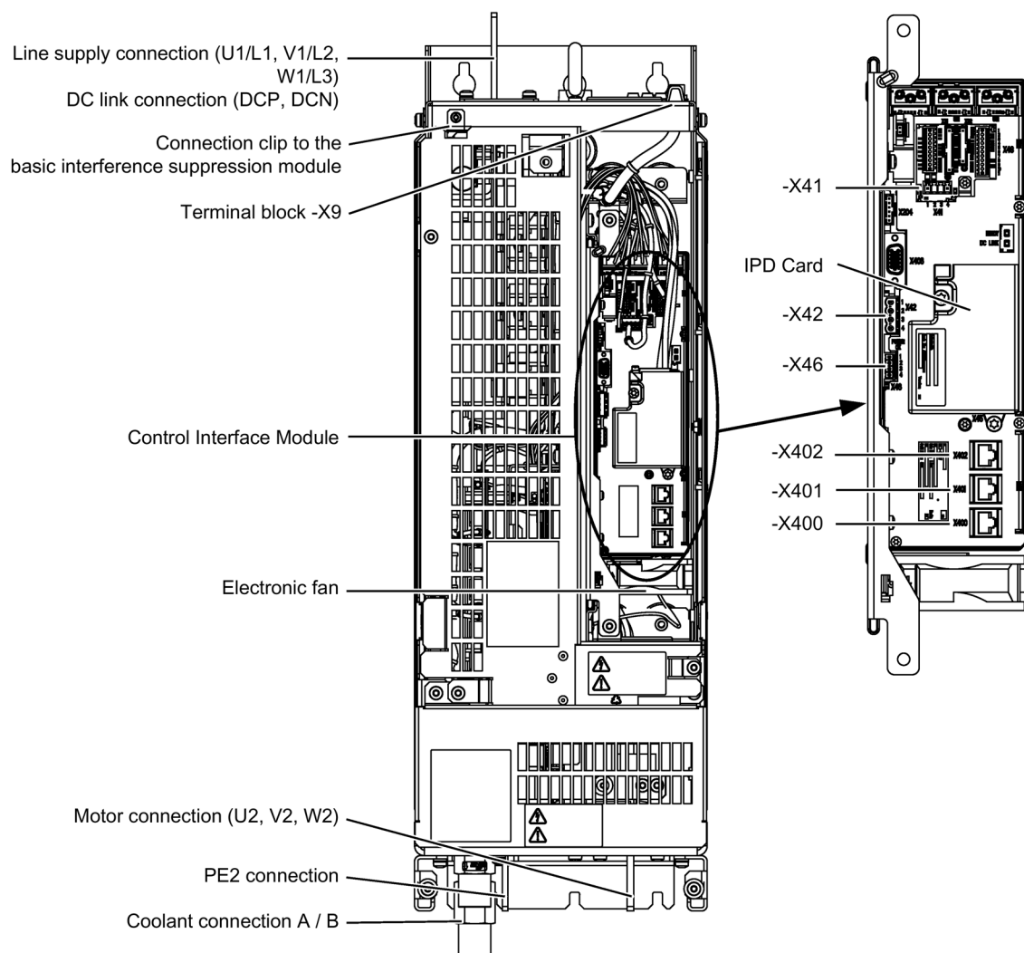
Figure 5-1 Power Module, frame size FL
