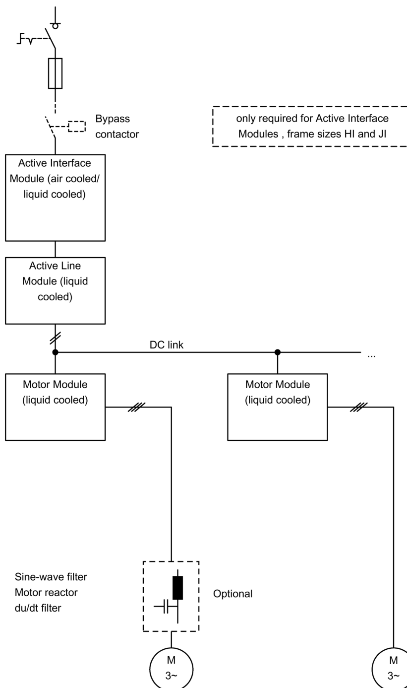
Figure 3-7 Basic structure of a drive system with liquid-cooled SINAMICS S120 and regulated infeed
