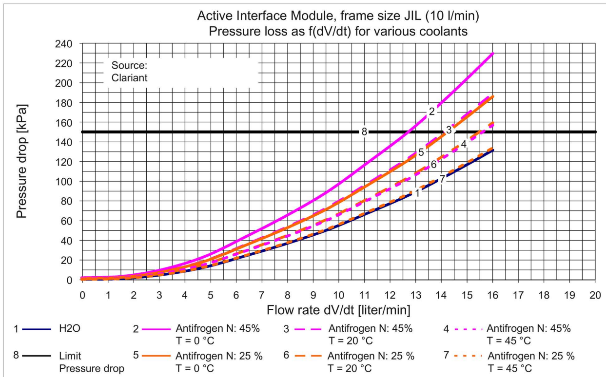
Figure 10-11 Pressure drop as a function of the flow rate for Active Interface Modules, frame size JIL, 10 l/min
