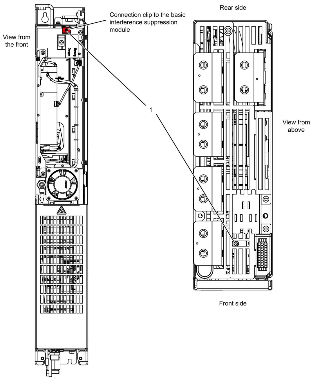
Figure 6-8 Removing the connection clip of the basic interference suppression module to ground
