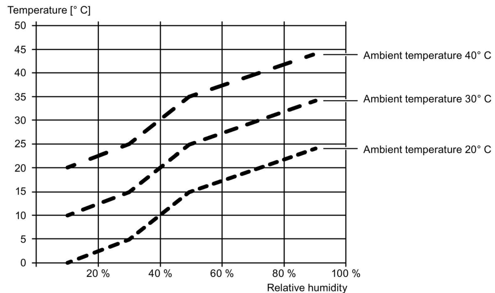
Figure 10-22 Examples of the minimum coolant temperature setpoint depending on the humidity for ambient temperatures of 20, 30 and 40 °C (dew point plus 2 °C)
