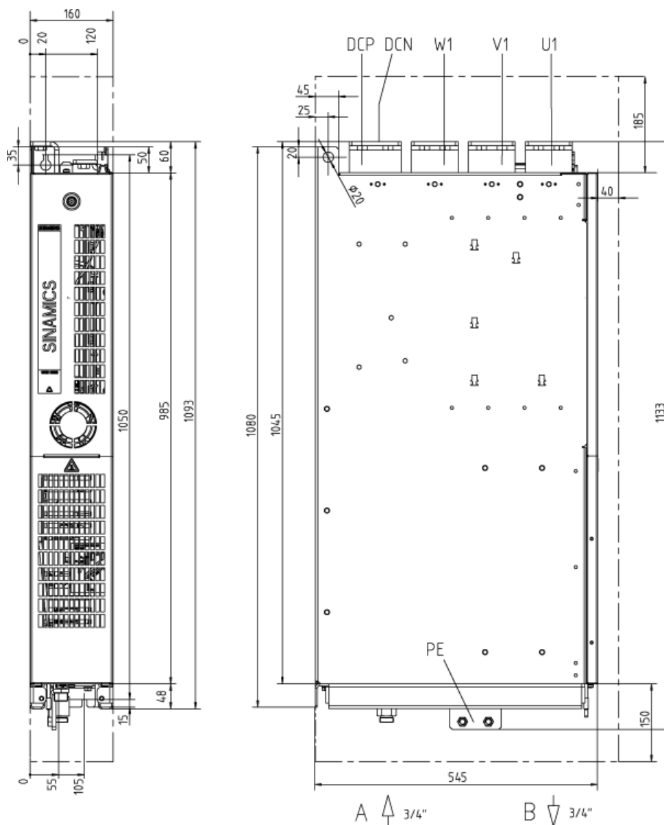
Figure 6-4 Dimension drawing, Basic Line Module, frame size GBL. Front view, side view
