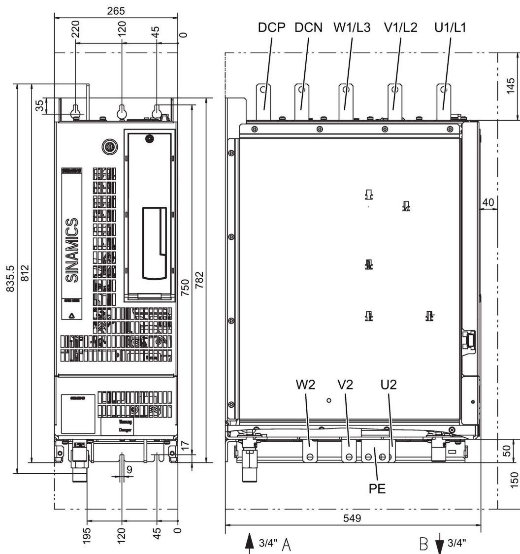
Figure 5-4 Dimension drawing Power Module, frame size FL. Front view, side view
