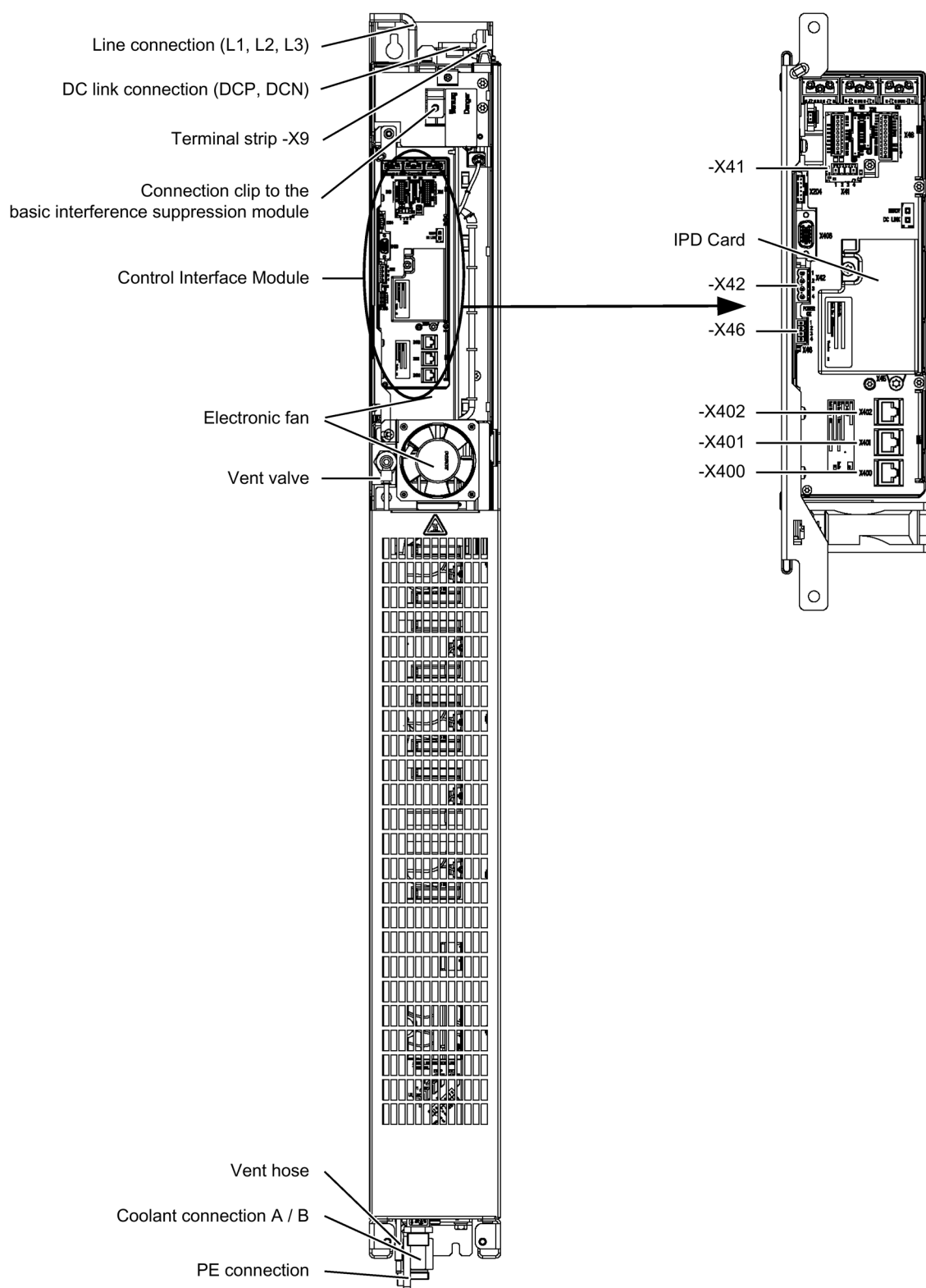
Figure 6-2 Basic Line Module, frame size GBL
