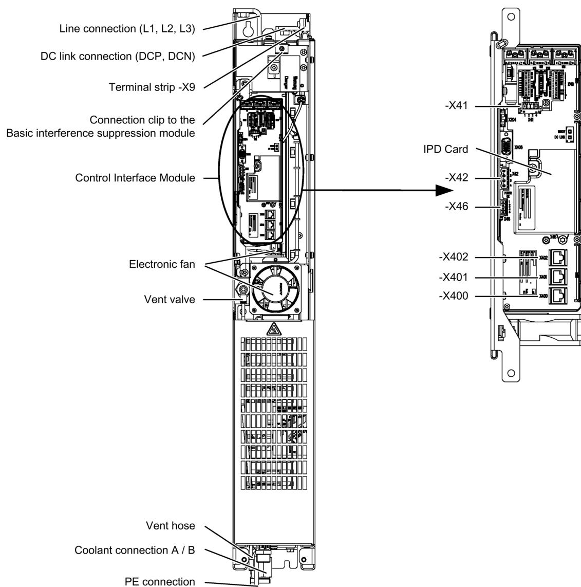
Figure 6-1 Basic Line Module, frame size FBL
