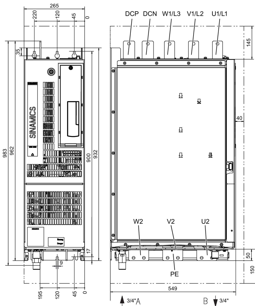
Figure 5-5 Dimension drawing Power Module, frame size GL. Front view, side view
