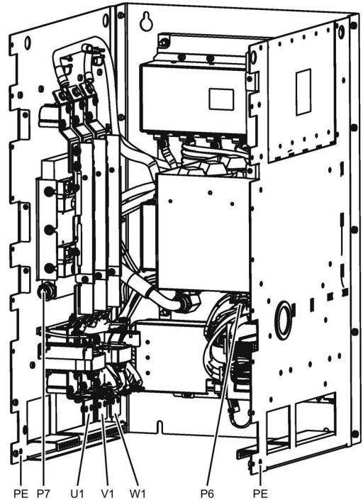
Interface overview filter module, size JIL, valid for function release FS = 03
