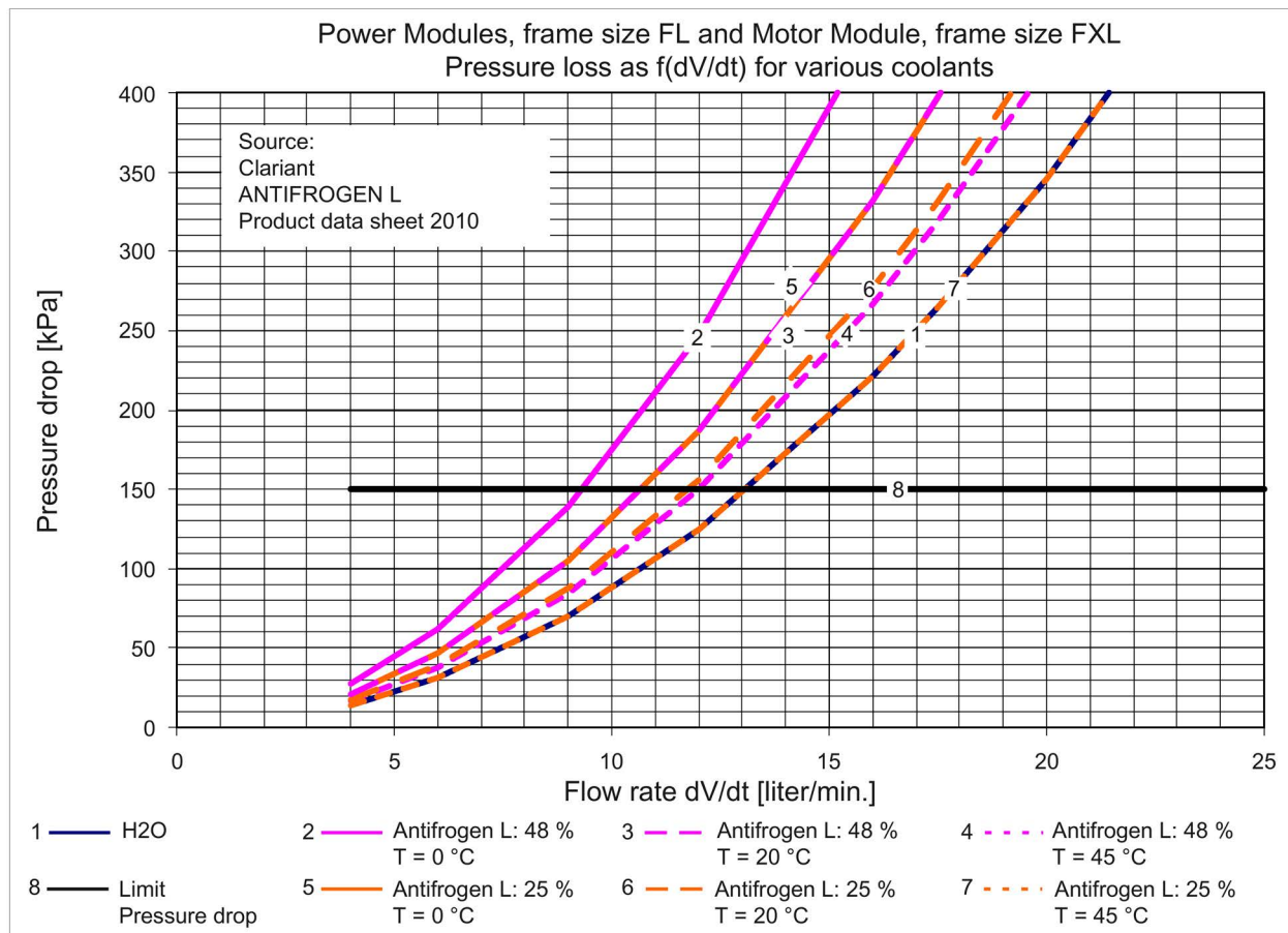
Figure 10-15 Pressure drop as a function of volumetric flow for Power Module frame size FL, and Motor Module frame size FXL
