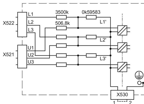
Figure 4-17 Internal circuit of the VSM10 Voltage Sensing Module
