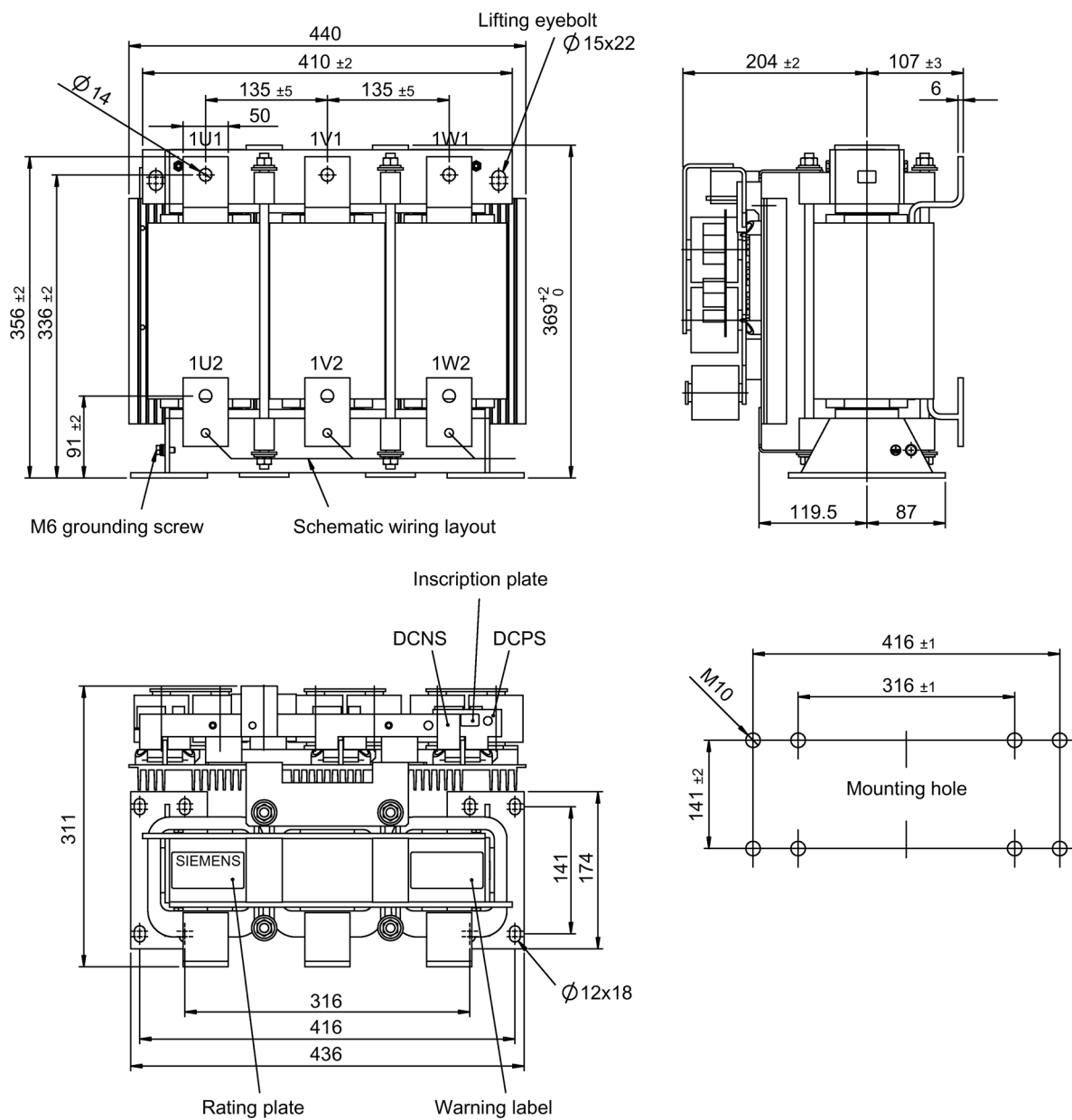
Figure 8-22 Dimension drawing for dv/dt filter compact plus voltage peak limiter, type 3
