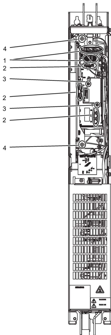
Figure 11-5 Replacing the Control Interface Module, Active Line Module and Motor Module, frame size GXL
