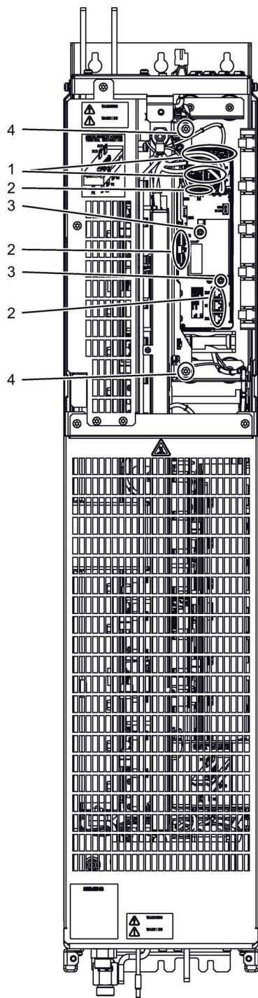
Figure 11-18 Replacing the electronic fan, Active Line Module, and Motor Module, frame size JXL
