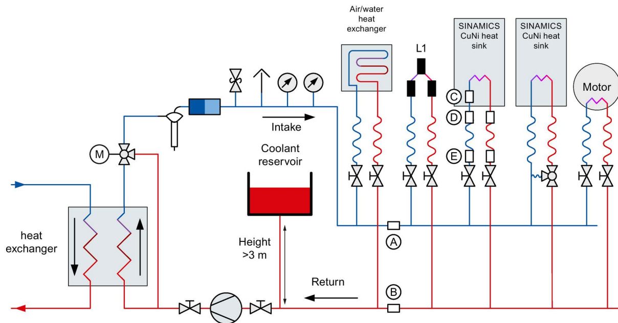
Figure 10-3 Arrangement of pressure compensator, component pressure drops
