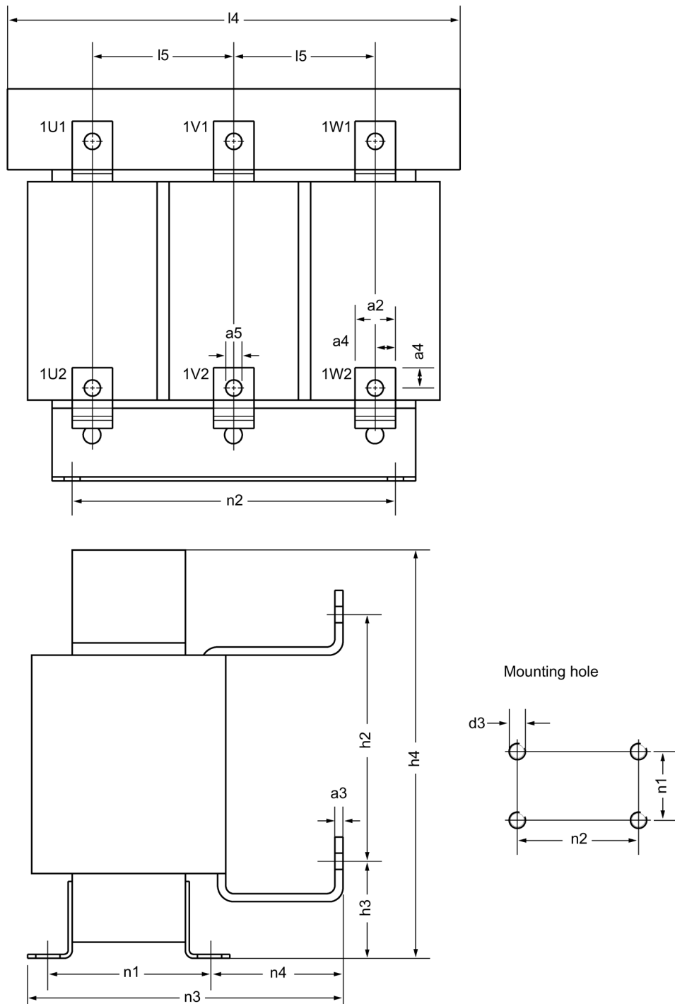
Figure 4-1 Dimension drawing of line reactor for Power Modules
