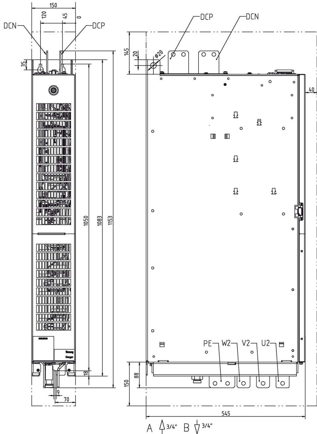
Figure 7-7 Dimension drawing Motor Module, frame size GXL. Front view, side view
