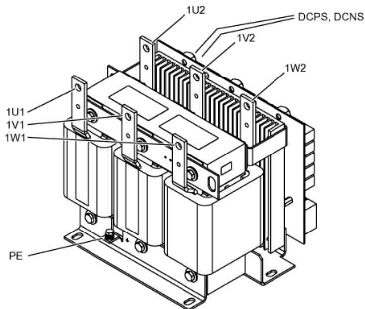
Figure 8-13 Interface overview for dv/dt filter compact plus Voltage Peak Limiter, Type 1
