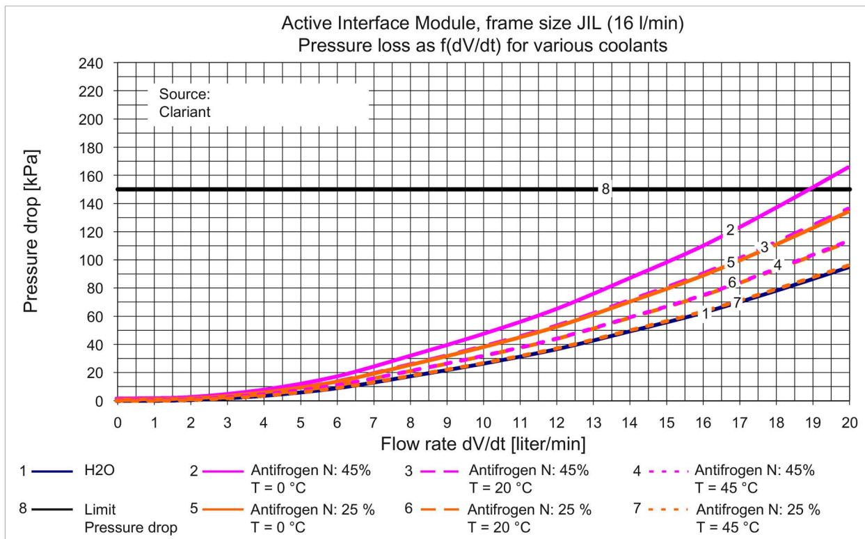
Figure 10-12 Pressure drop as a function of the flow rate for Active Interface Modules, frame size JIL, 16 l/min
