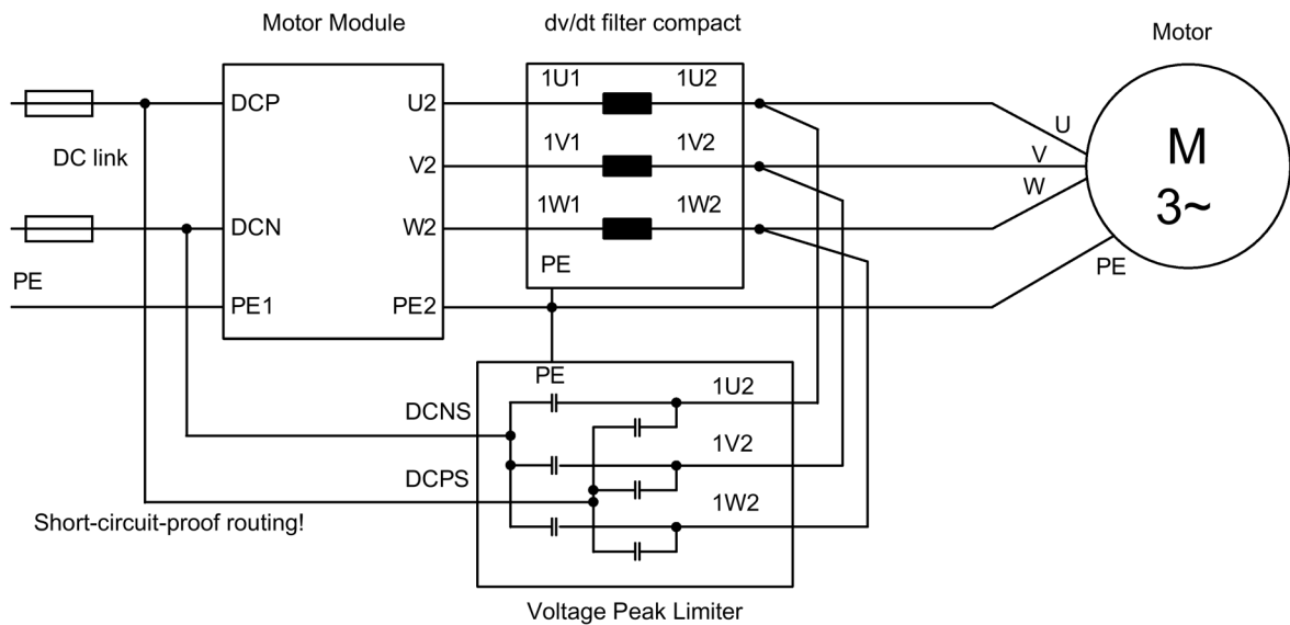
Figure 8-19 Connecting the dv/dt filter compact plus Voltage Peak Limiter - separate components
