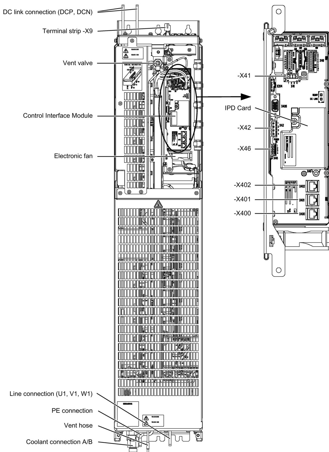
Figure 6-14 Active Line Module, frame size JXL
