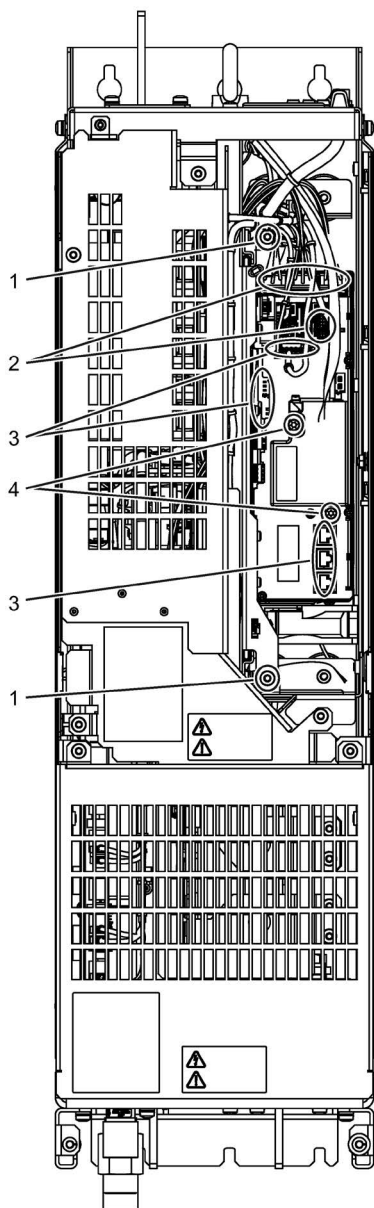
Figure 11-3 Replacing the Control Interface Module, Power Module, frame size GL
