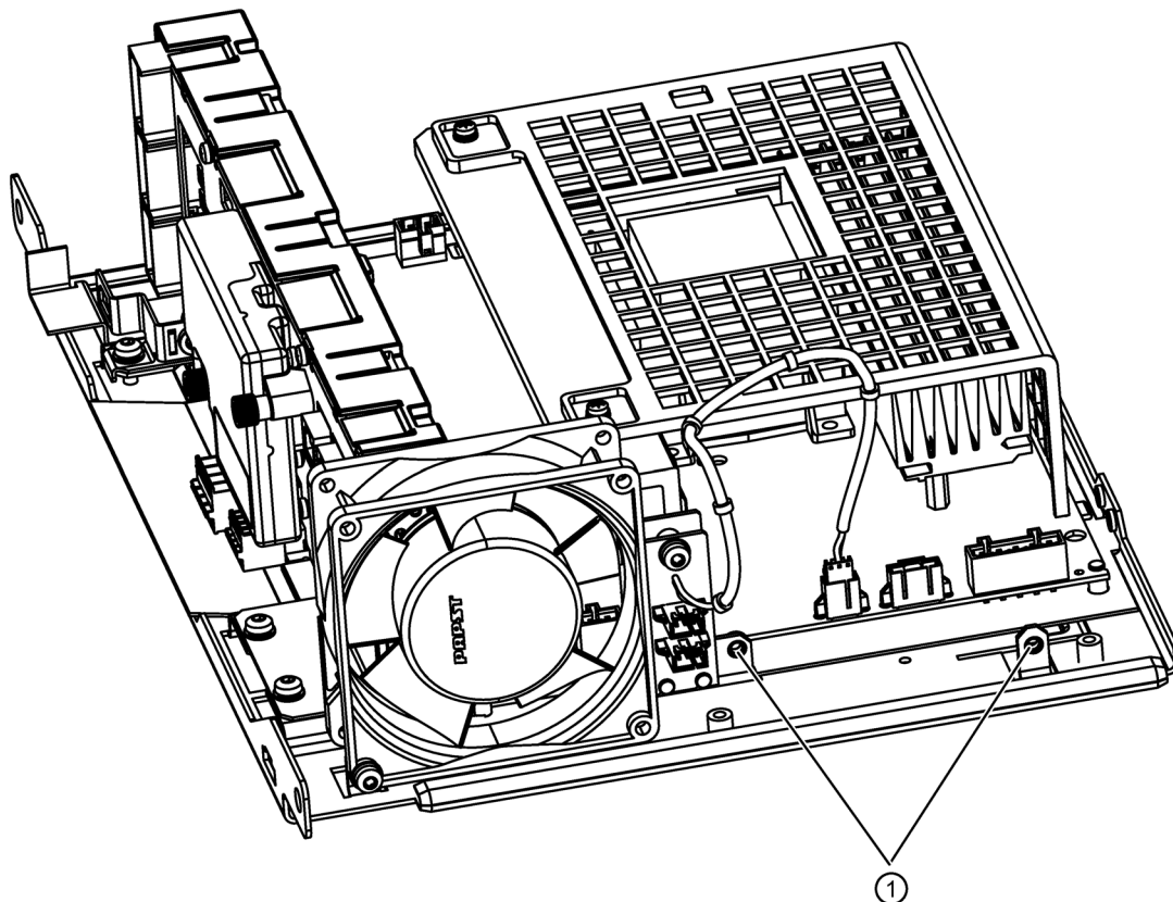
Figure 11-9 Replacement part, Control Interface Module with an electronics fan
