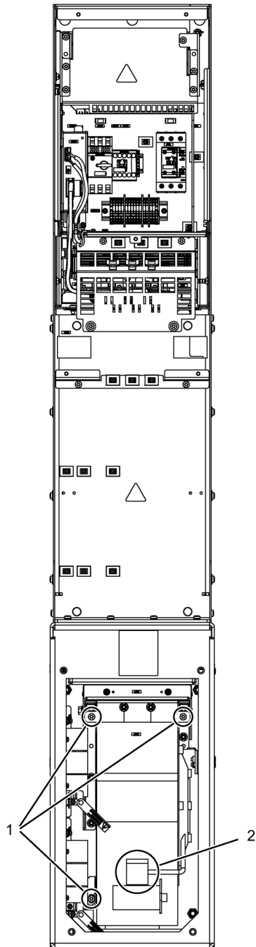
Figure 11-23 Replacing the fan, Active Interface Module, frame size HI
