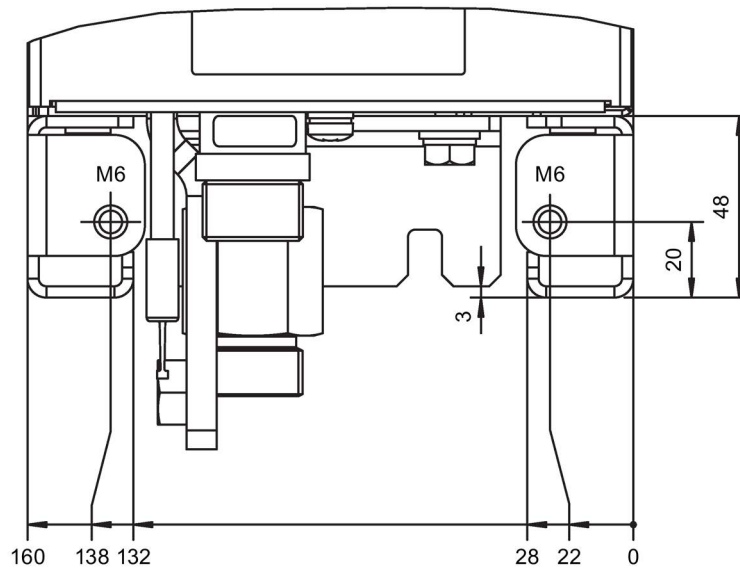
Figure 9-4 Rail profile, Basic Line Module, frame sizes FBL, GBL (dimensions in mm)
