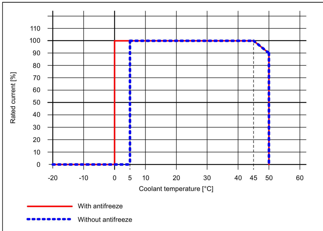
Figure 3-3 Maximum output current as a function of coolant temperature
