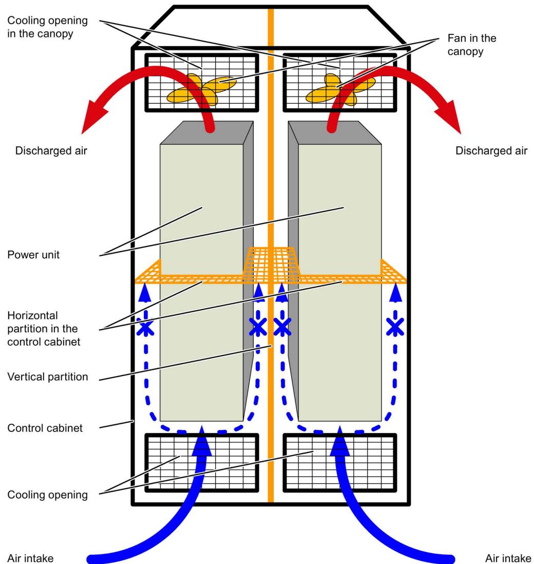
Figure 9-1 Example showing a partition in the control cabinet
