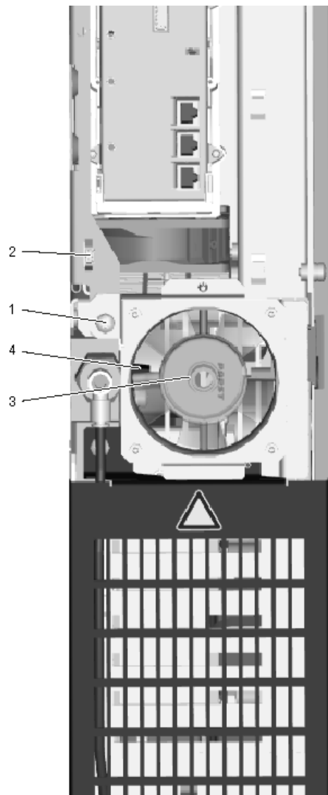
Figure 10-27 Removing the electronics fan to actuate the vent valve
