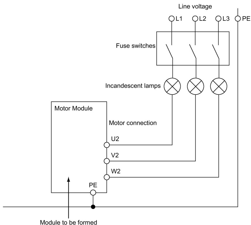
Figure 11-26 Forming circuit for Motor Modules
