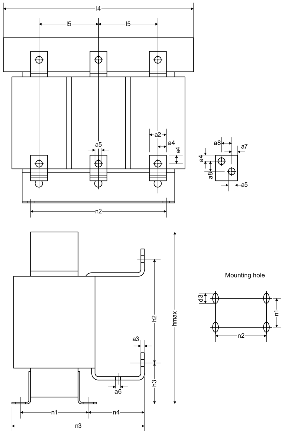
Figure 8-9 Dimension drawing, dv/dt reactor
