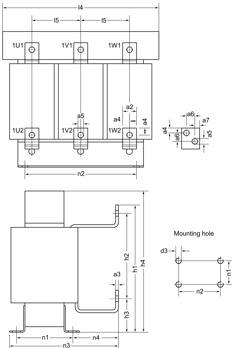
Figure 4-2 Dimension drawing of line reactors for Basic Line Modules
