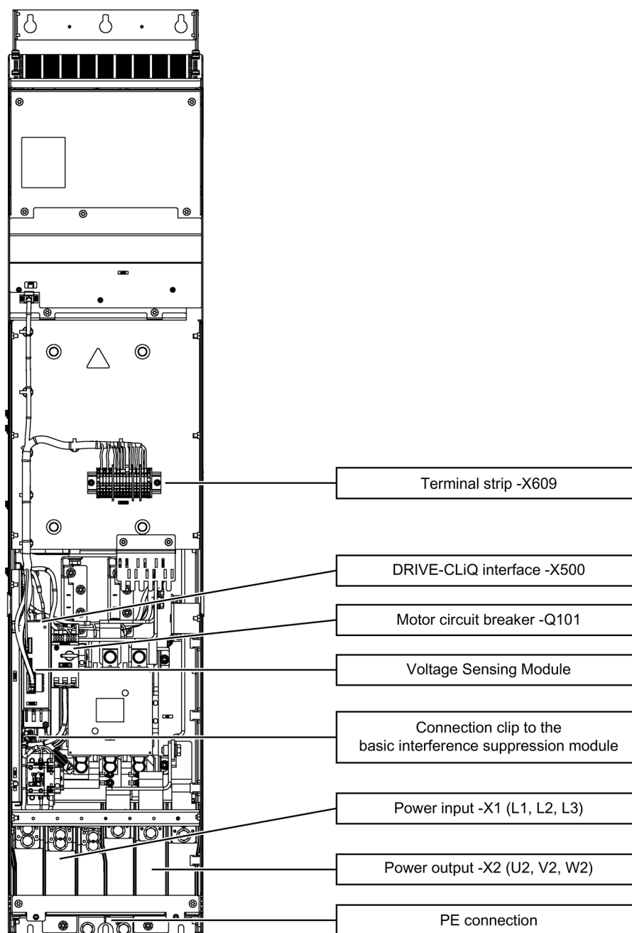
Figure 4-3 Interface overview in the Active Interface Module, frame size G1
