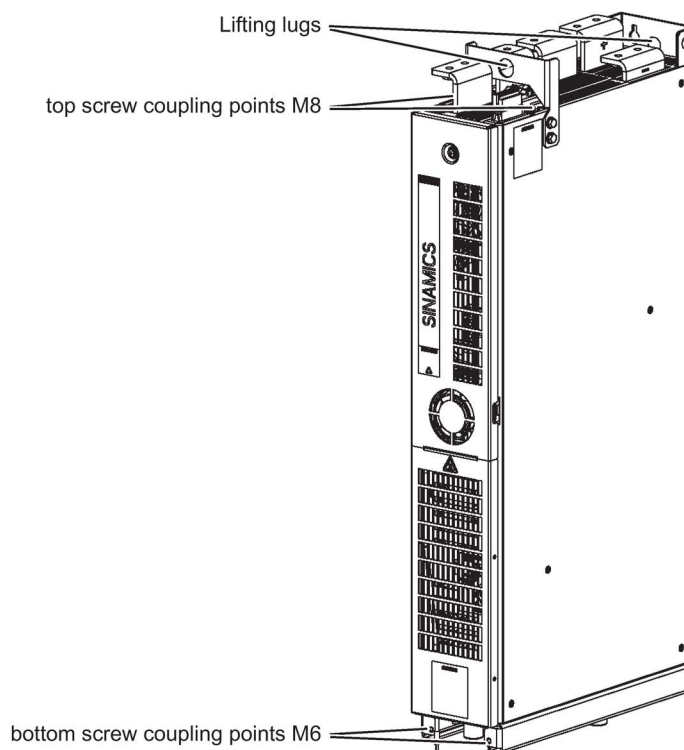
Figure 6-6 Lifting lugs / screw coupling points for mechanical support
