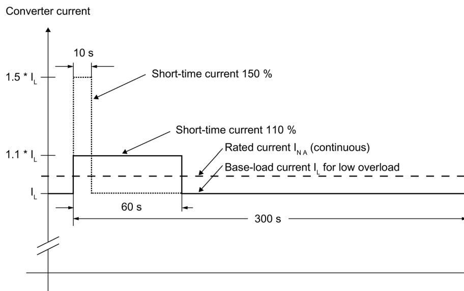
Figure 5-9 Low overload
