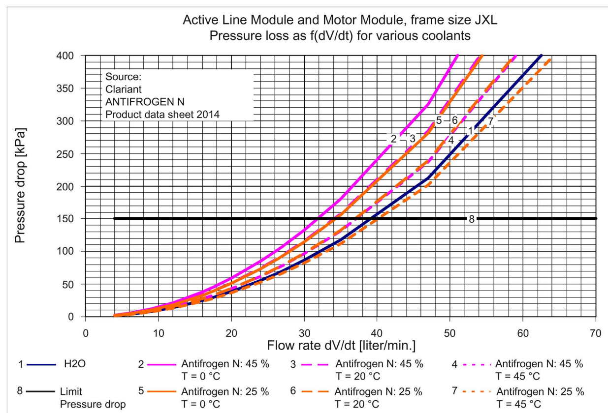
Figure 10-10 Pressure drop as a function of volumetric flow for Active Line Module and Motor Module, frame size JXL
