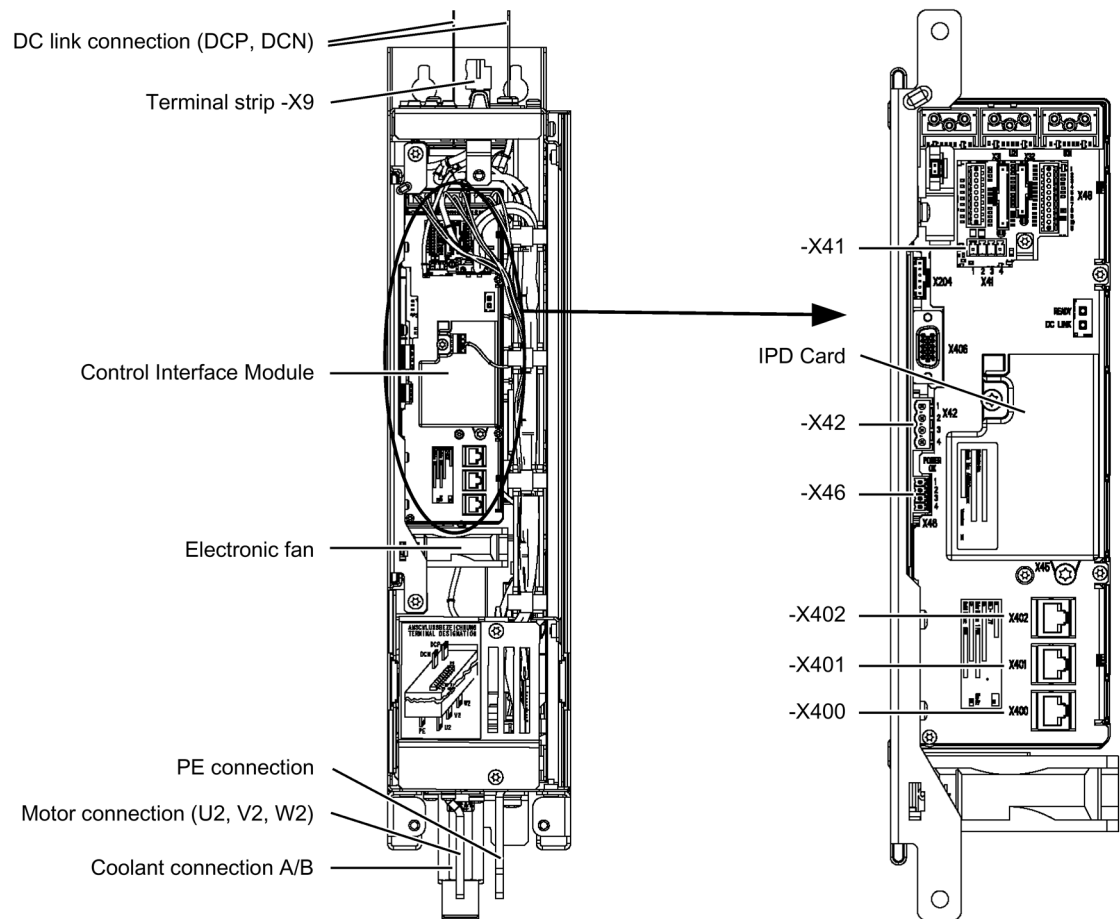
Figure 7-1 Motor Module, frame size FXL
