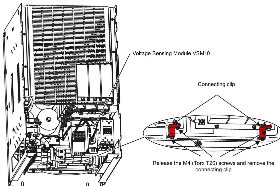
Figure 4-27 Removing the connection clip of the basic interference suppression module to ground
