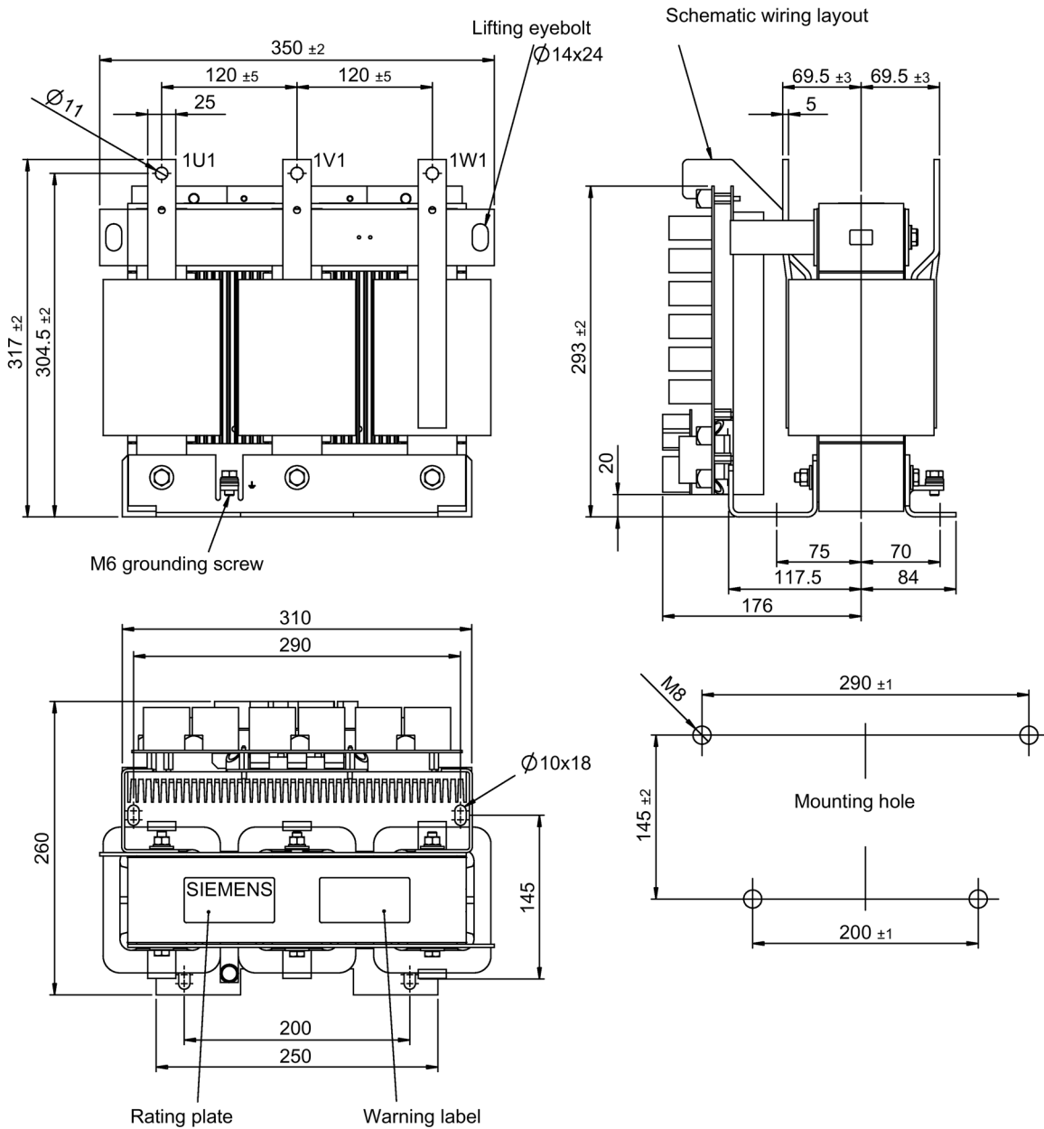
Figure 8-21 Dimension drawing for dV/dt filter compact plus voltage peak limiter, type 2
