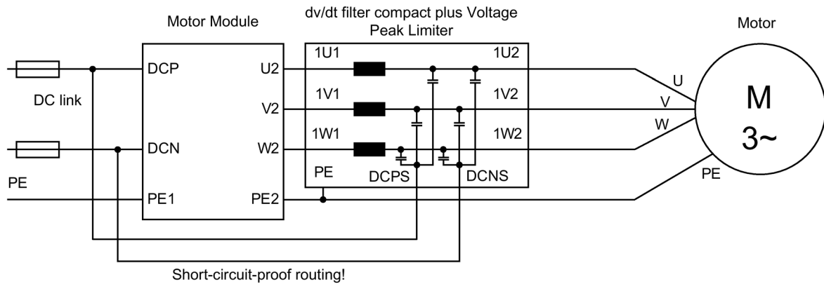
Figure 8-18 Connecting the dv/dt filter compact plus Voltage Peak Limiter - complete unit
