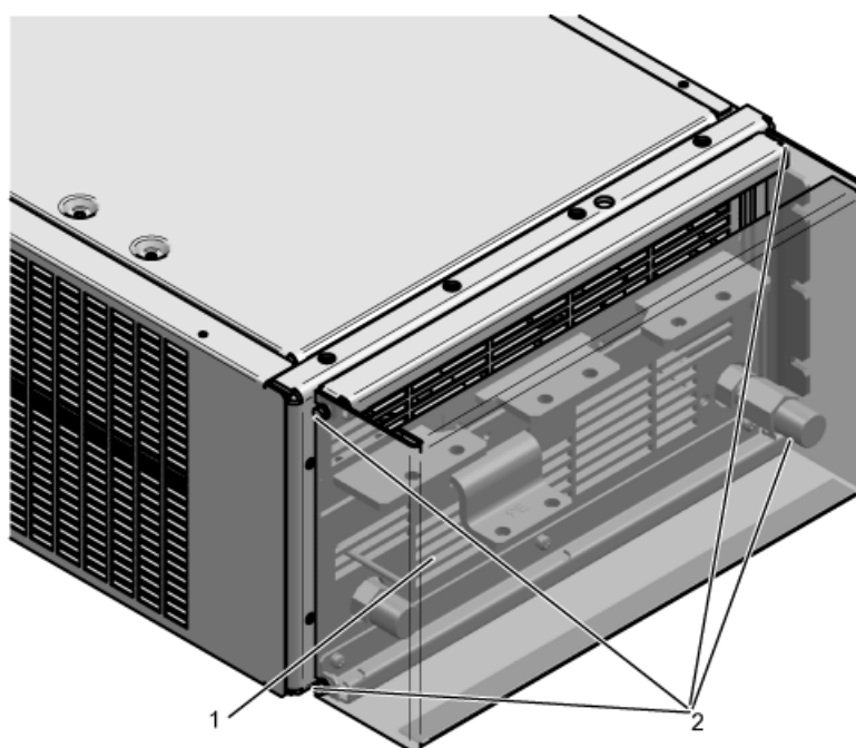
Figure 6-21 Protection guard
