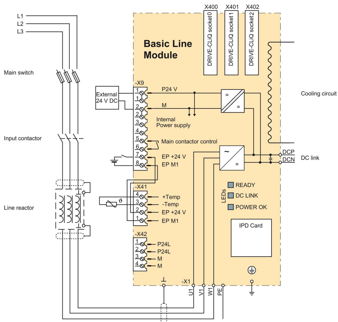
Figure 6-3 Connection example for Basic Line Modules
