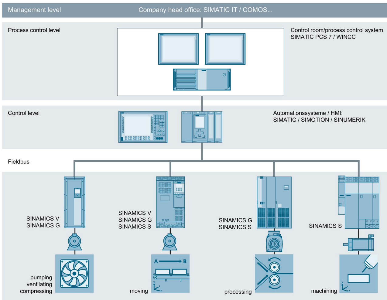
Figure 3-2 SINAMICS in the automation environment
