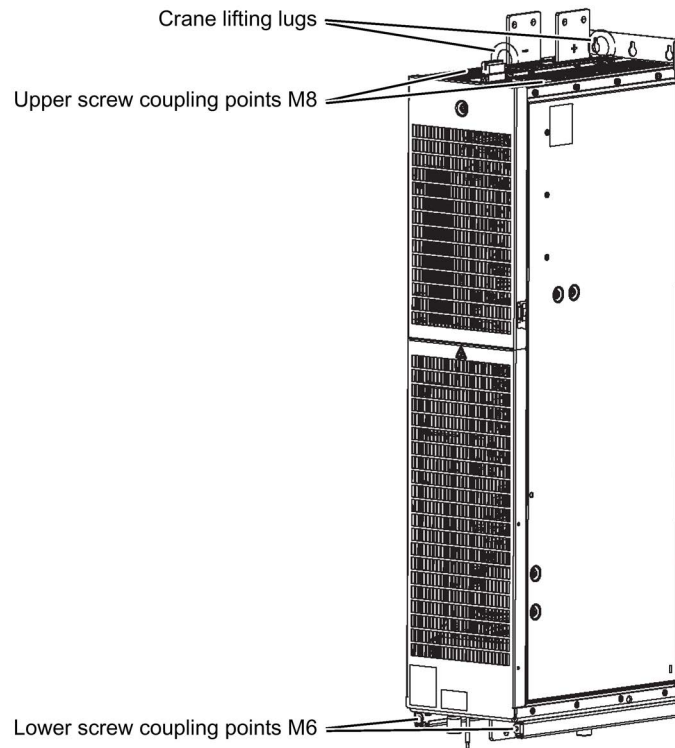
Figure 6-20 Crane lifting lugs / screw coupling points for mechanical support
