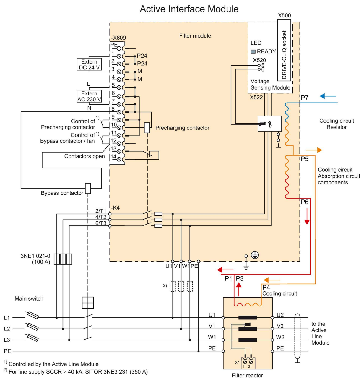
Figure 4-16 Connection example of liquid-cooled Active Interface Module, frame size J1L, valid for article numbers 6SL3305-7TE41-4AA5 and 6SL3305-7TG41-6AA5
