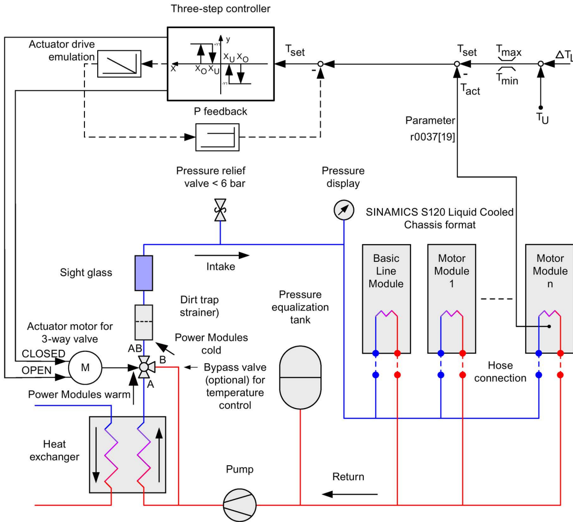
Figure 10-21 Principle of a flow control with 3-way valve as protection against condensation
