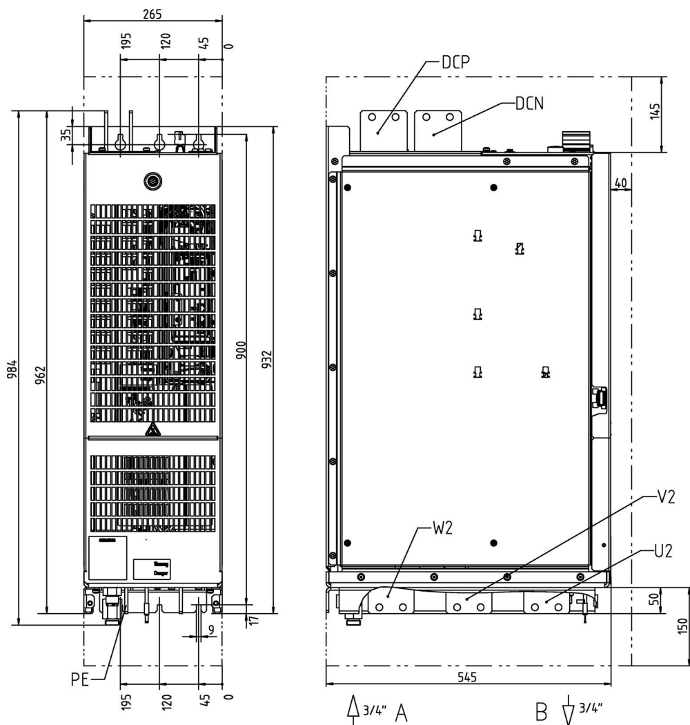
Figure 7-8 Dimension drawing Motor Module, frame size HXL. Front view, side view
