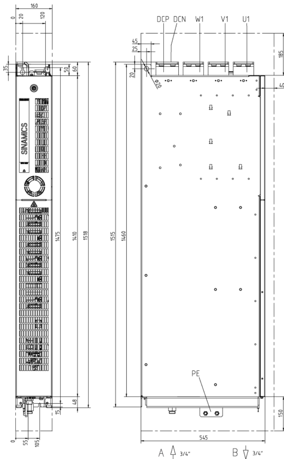
Figure 6-5 Dimension drawing, Basic Line Module, frame size GBL. Front view, side view
