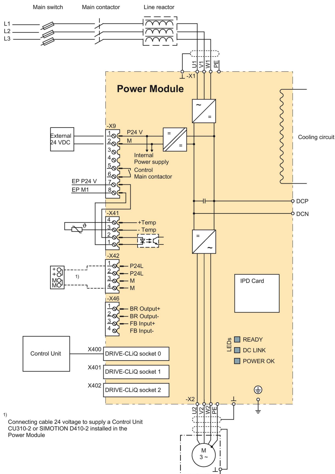
Figure 5-3 Connection example for Power module
