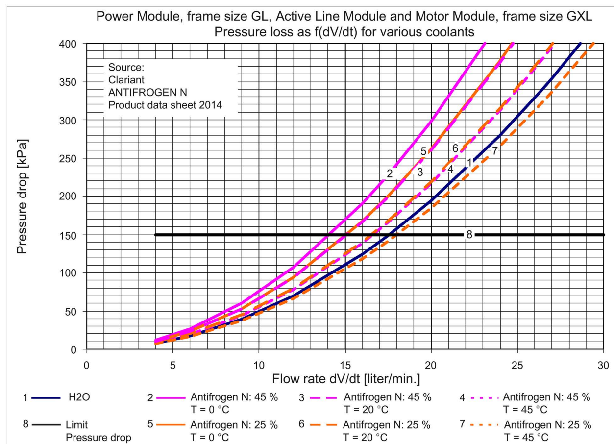
Figure 10-8 Pressure drop as a function of volumetric flow for Power Module frame size GL, Active Line Module and Motor Module frame size GXL
