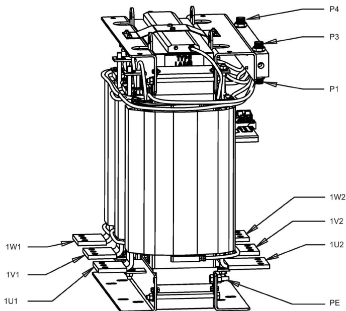
Figure 4-14 Interface overview filter reactor, frame size JIL, valid for article numbers 6SL3005-ODE41-4AA0 and 6SL3005-ODG41-6AA0
