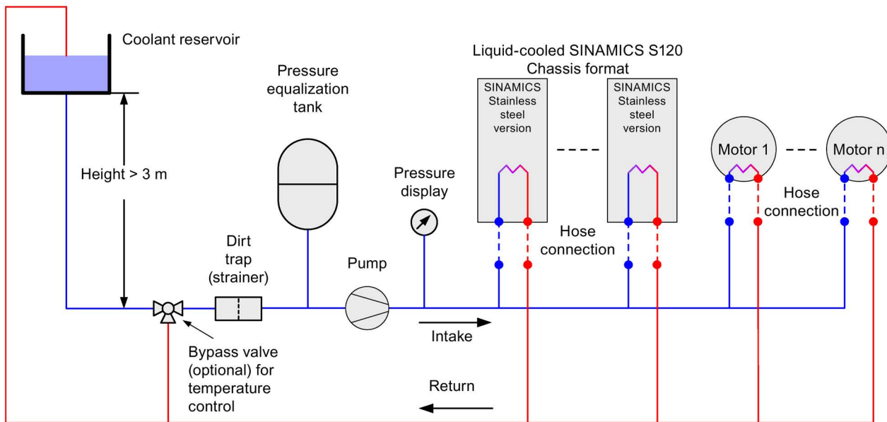
Figure 10-2 Recommendation for open circuit
