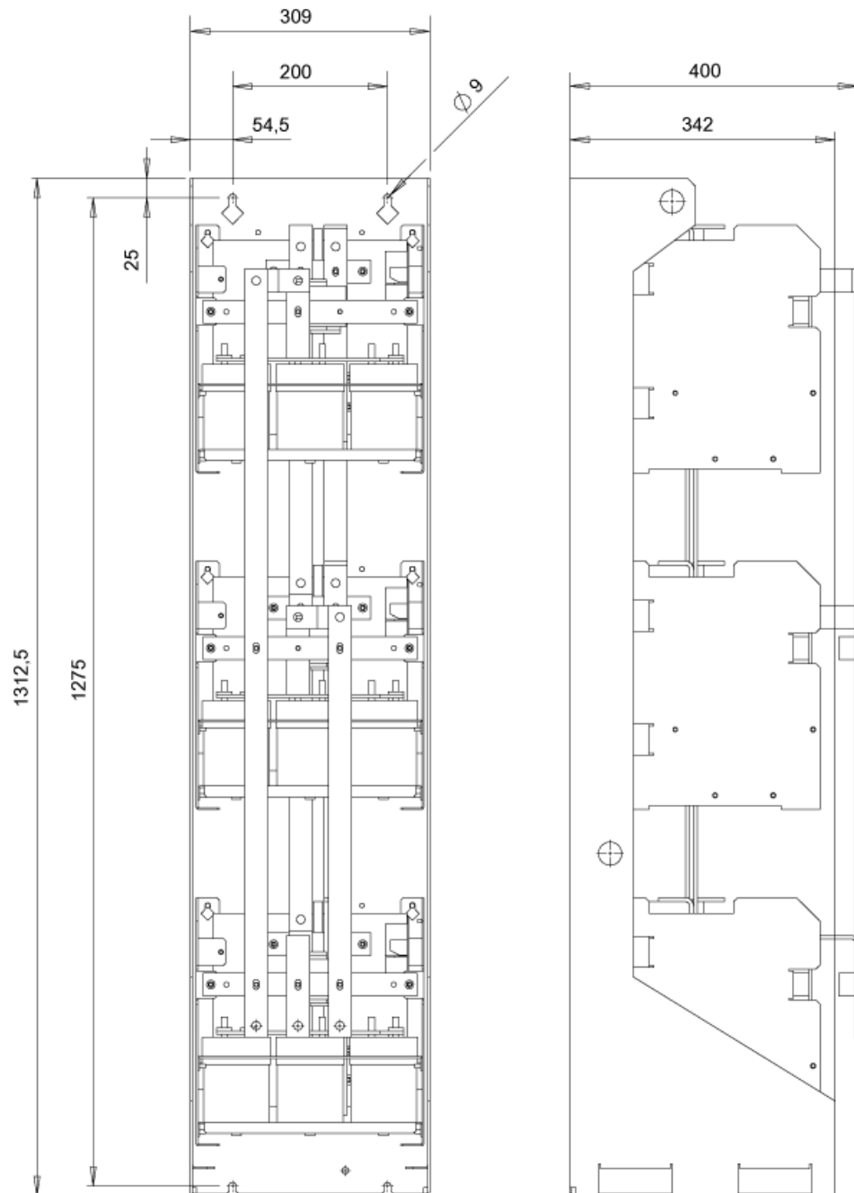
Figure 8-12 Dimension drawing of the voltage peak limiter, type 3
