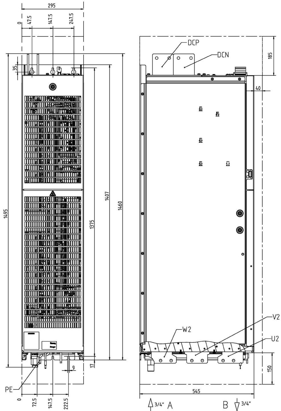
Figure 7-9 Dimension drawing Motor Module, frame size JXL, article numbers 6SL3325-1TE41-0AA3, 6SL3325-1TE41-4AA3, 6SL3325-1TG38-1AA3, 6SL3325-1TG41-0AA3, 6SL3325-1TG41-2AA3, 6SL3325-1TG41-3AA3. Front view, side view
