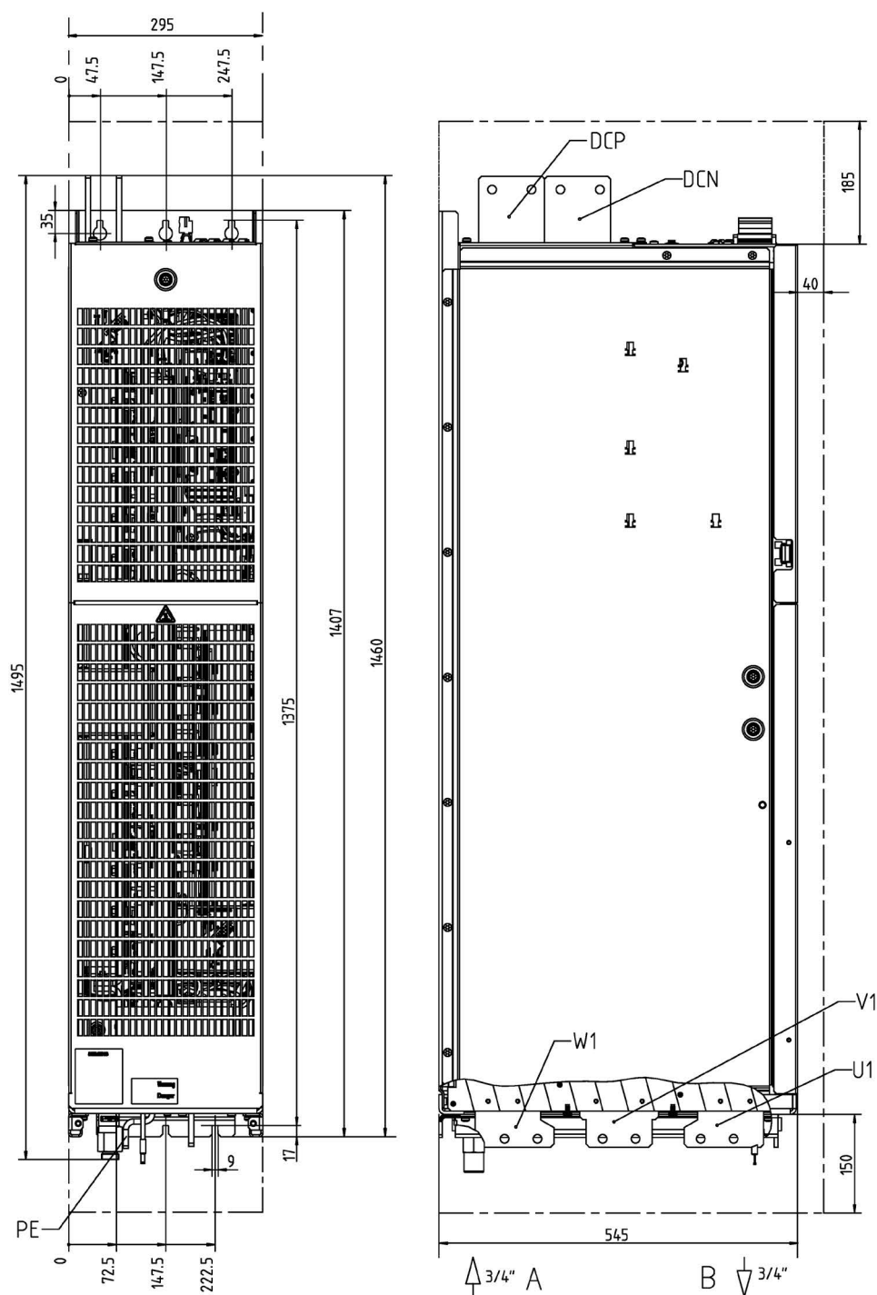
Figure 6-18 Dimension drawing Active Line Module, frame size JXL, article numbers 6SL3335-7TE41-0AA3, 6SL3335-7TE41-4AA3, 6SL3335-7TG41-0AA3, 6SL3335-7TG41-3AA3. Front view, side view
