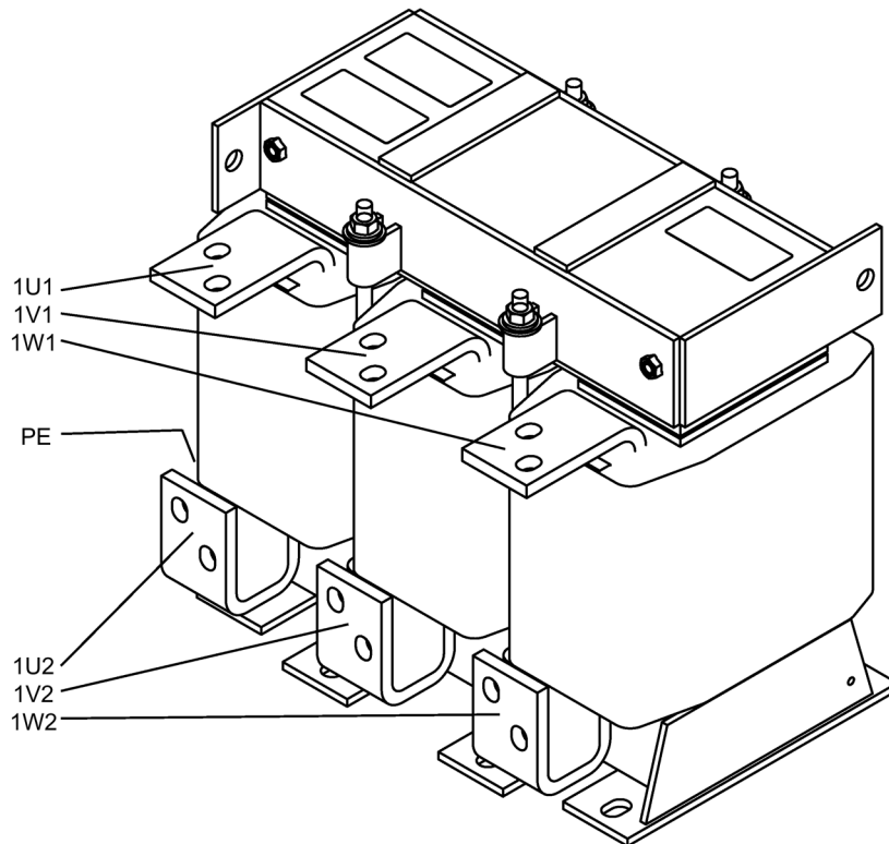
Figure 8-16 Interface overview for dv/dt filter compact plus Voltage Peak Limiter, Type 4 dv/dt reactor
