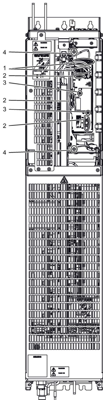
Figure 11-7 Replacing the Control Interface Module, Active Line Module and Motor Module, frame size JXL
