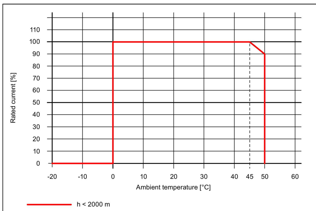
Figure 3-4 Maximum current as a function of ambient temperature
