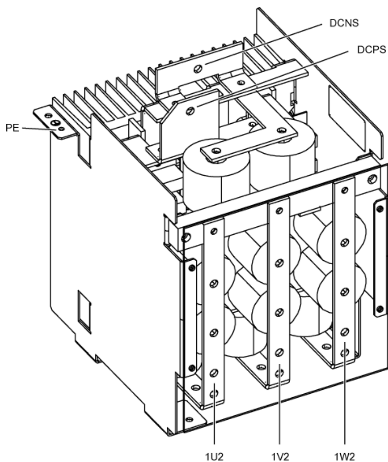
Figure 8-17 Interface overview for dv/dt filter compact plus Voltage Peak Limiter, Type 4 Voltage Peak Limiter
