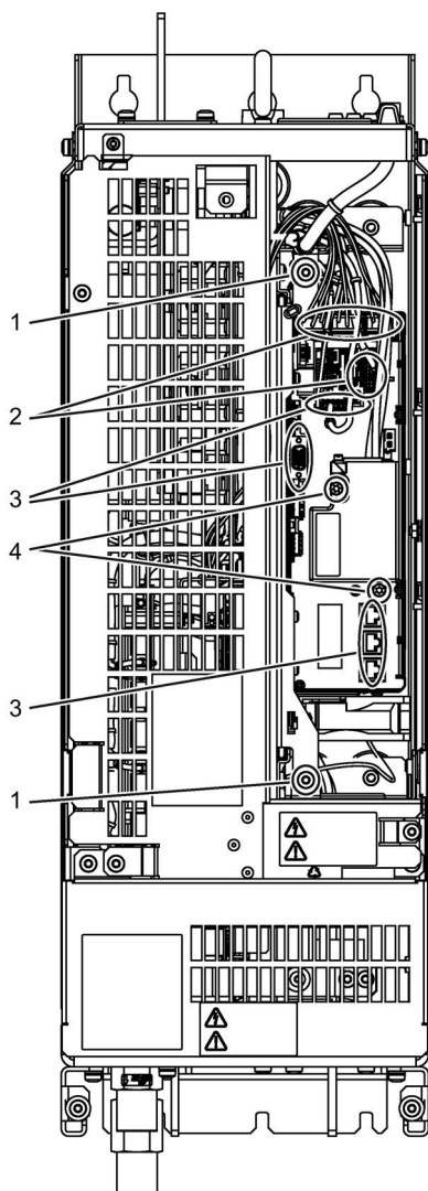
Figure 11-13 Replacing the electronic fan, Power Module, frame size FL
