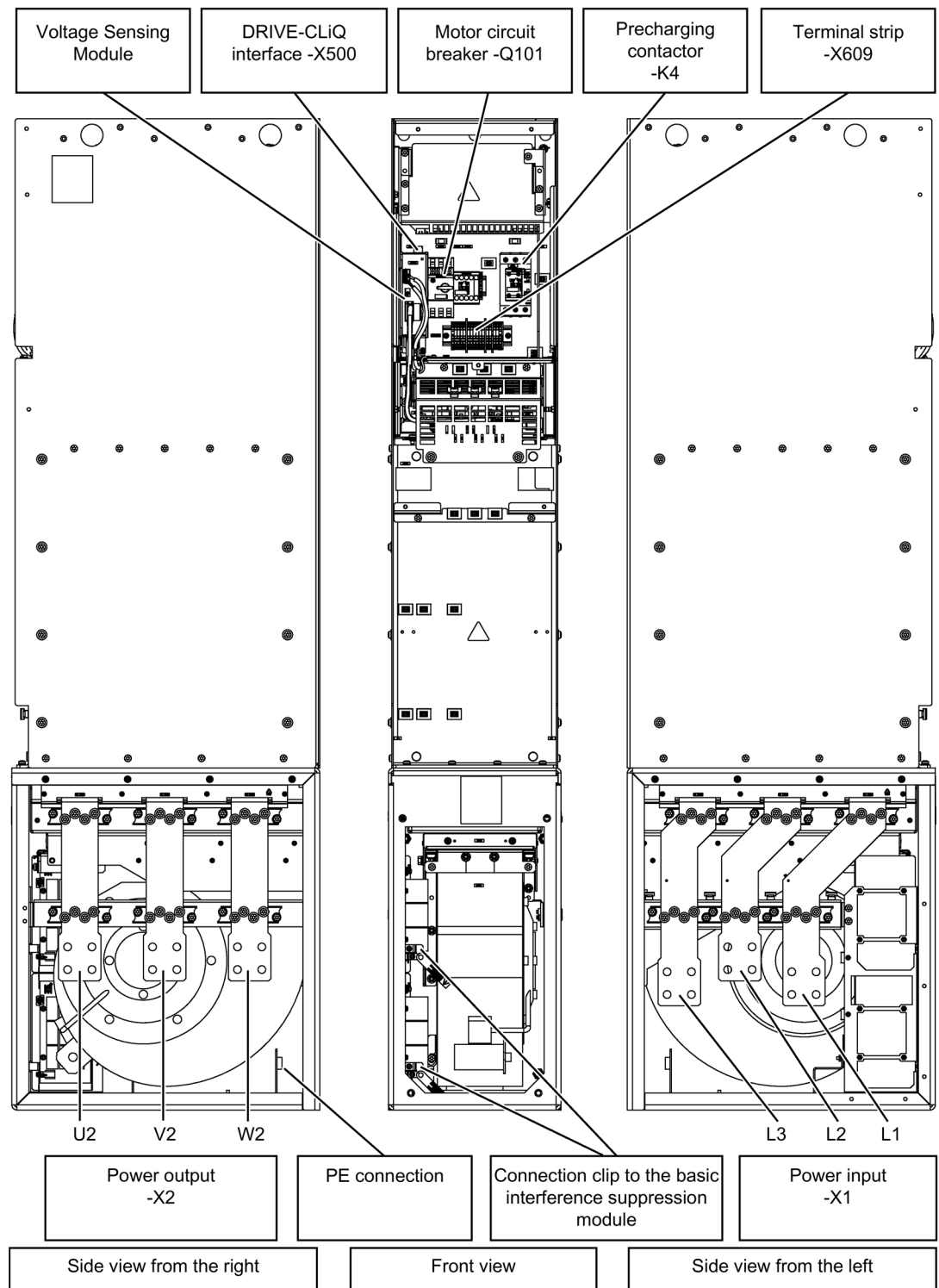
Figure 4-4 Interface overview in the Active Interface Module, frame size HI
