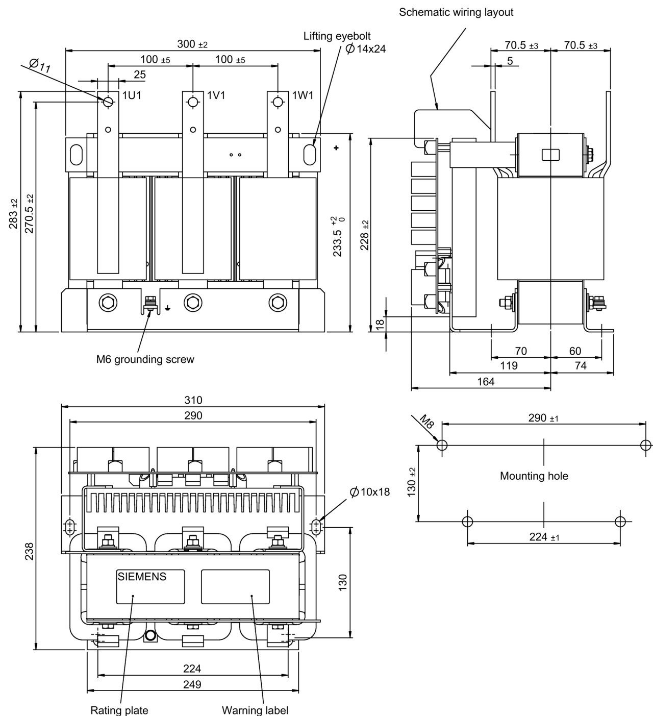
Figure 8-20 Dimension drawing for dv/dt filter compact plus voltage peak limiter, type 1
