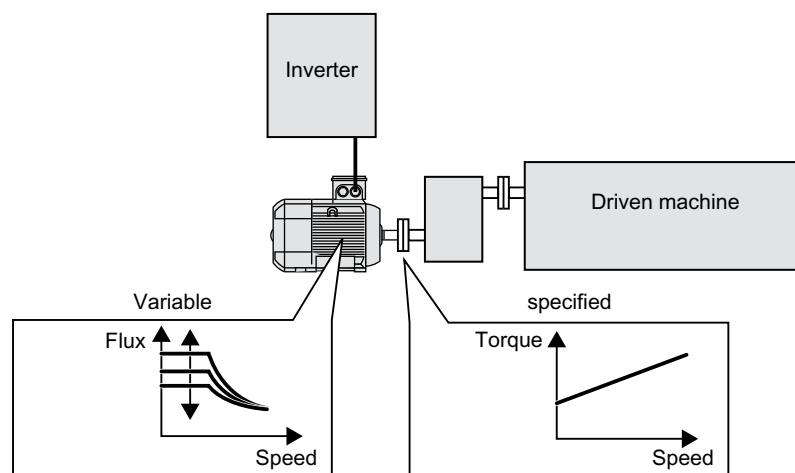
Figure 8-188 Efficiency optimization by changing the motor flux
