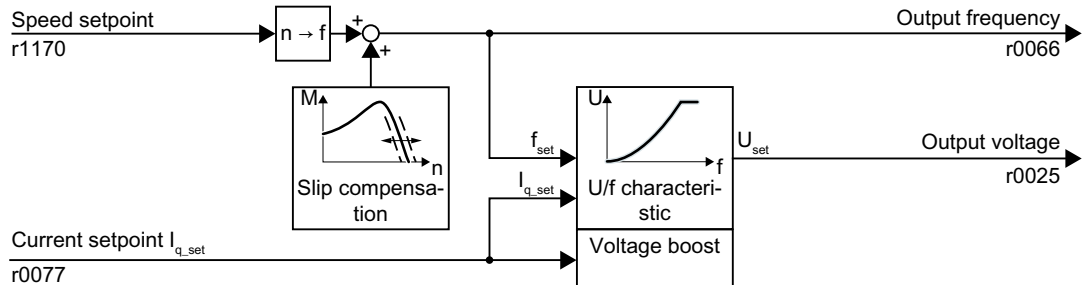
Figure 8-103 Default setting of the V/f control after selecting Standard Drive Control
