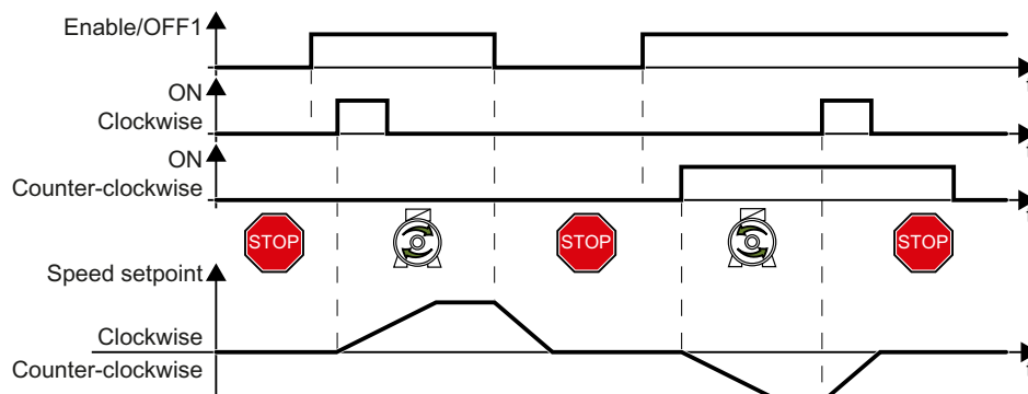
Figure 8-53 Three-wire control, enable/clockwise/counter-clockwise rotation
