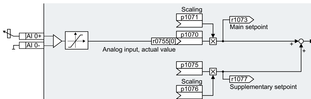
Figure 8-66 Example: Analog input 0 as setpoint source
