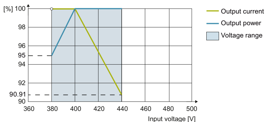
Figure 12-1 Current and voltage derating as a function of the input voltage
