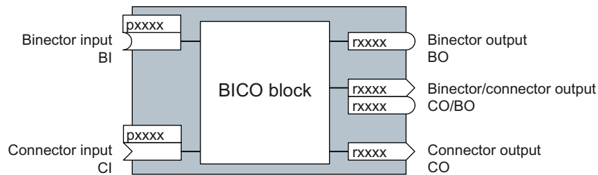
Figure 8-208 Symbols for binector and connector inputs and outputs
