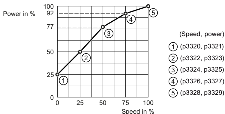
Figure 8-200 Factory setting of the flow characteristic
