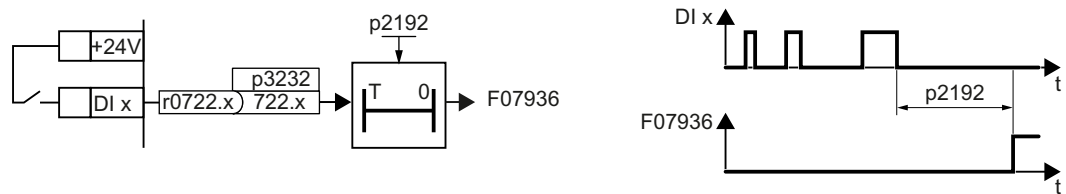
Figure 8-176 Function plan and time response of the speed monitoring
