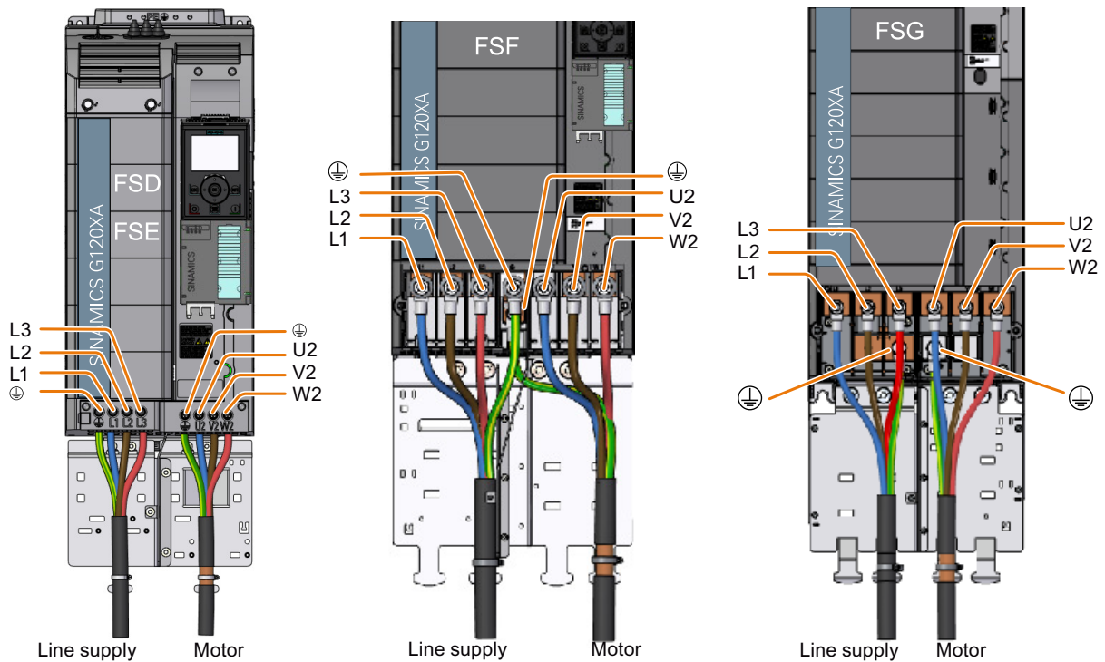
Figure 4-13 Connections for the line supply and motor
