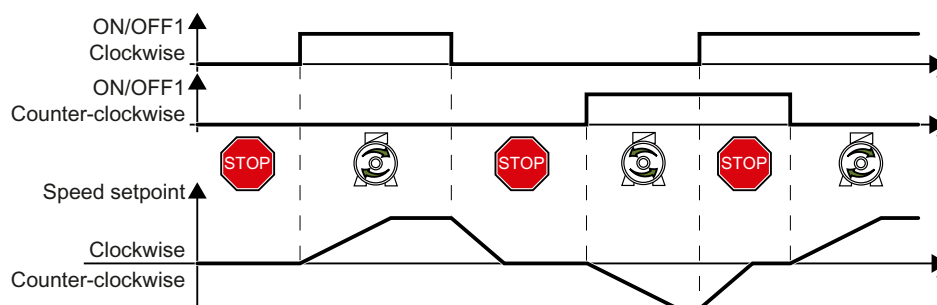
Figure 8-52 Two-wire control, clockwise/counter-clockwise rotation
