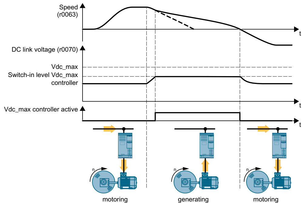
Figure 8-168 Simplified representation of the V_{dc\_max} control
