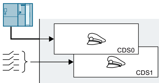
Figure 8-34 Converter control either via fieldbus or via terminal strip
