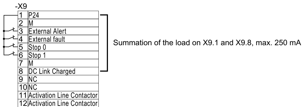
Figure 4-20 Connecting internal 24 V power supply
