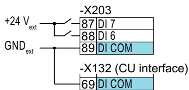
Figure 2-2 Connecting P-switching contacts
