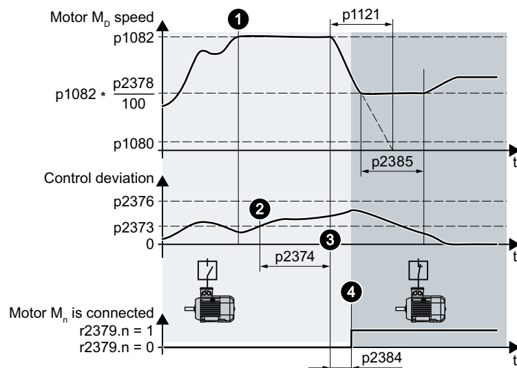
Figure 8-94 Activate uncontrolled motors M_1 \dots M_2
