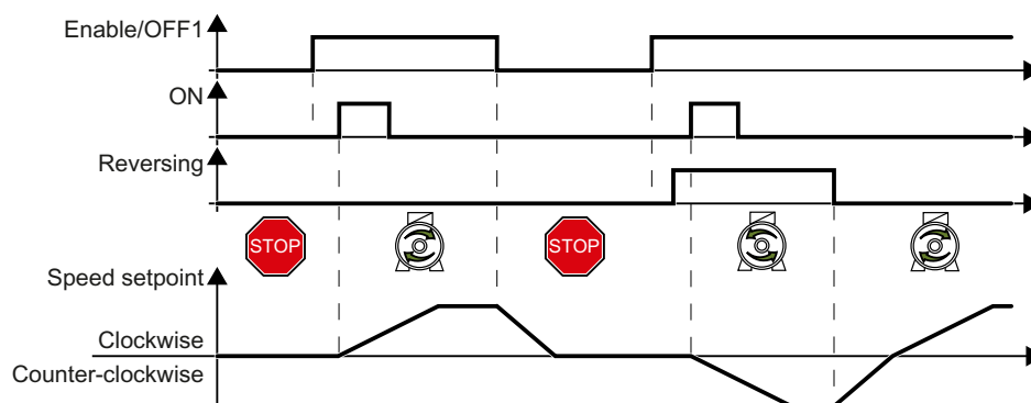
Figure 8-54 Three-wire control, enable/ON/reverse
