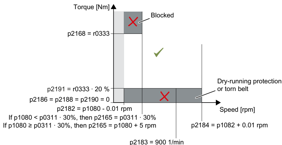
Figure 8-175 Default settings for fans and compressors
