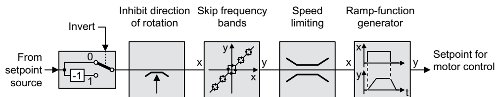
Figure 8-78 Setpoint processing in the converter
