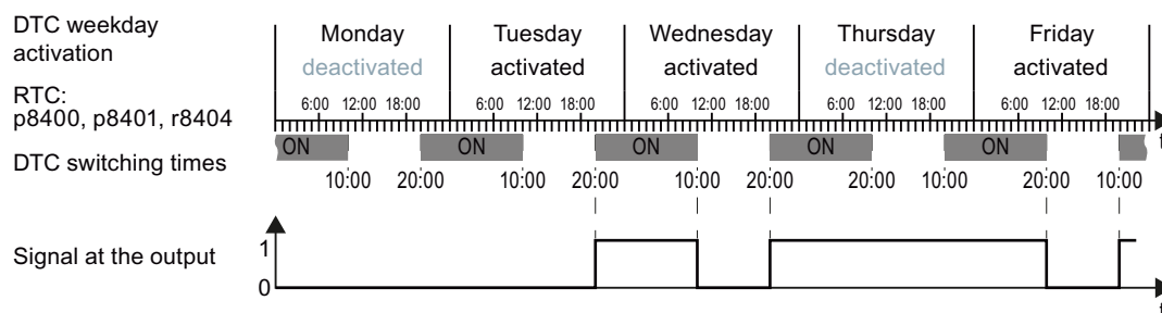
Figure 8-96 Example of the response of the time switch.
