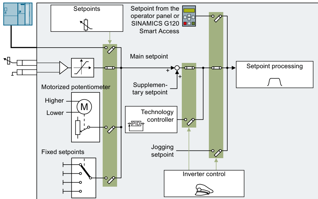
Figure 8-65 Setpoint sources for the converter
