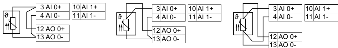
Figure 8-165 Two-wire connection, three-wire connection and four-wire connection
