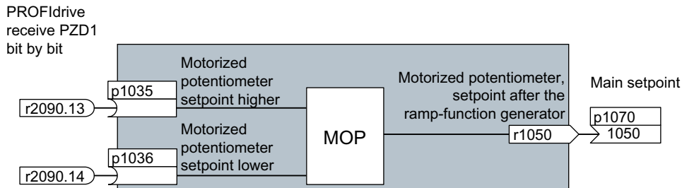
Figure 8-207 Example: Signal interconnection of two blocks for digital input 0
