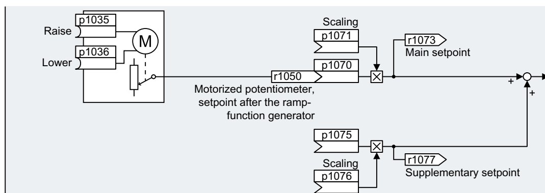
Figure 8-68 Motorized potentiometer as setpoint source
