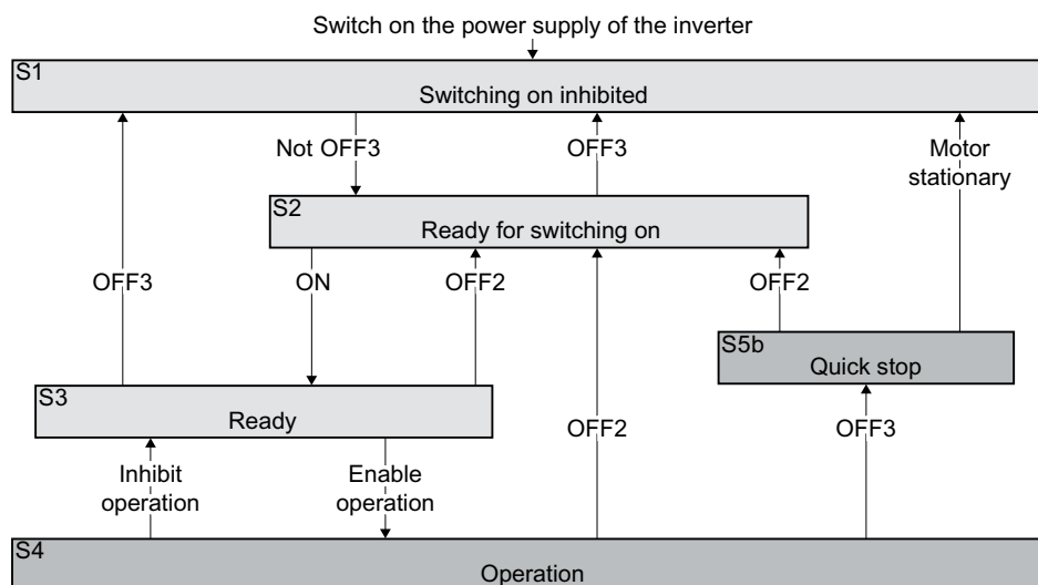
Figure 8-3 Sequence control of the converter when the motor is switched on and off
