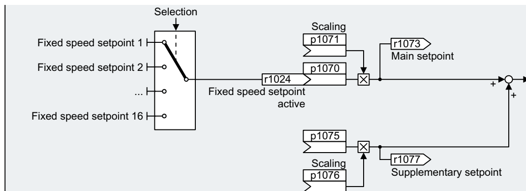
Figure 8-70 Fixed speed setpoint as setpoint source
