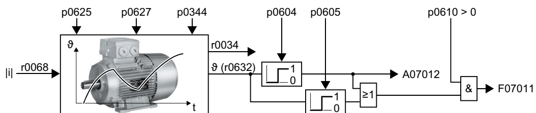
Figure 8-166 Thermal motor model 2 for induction motors
