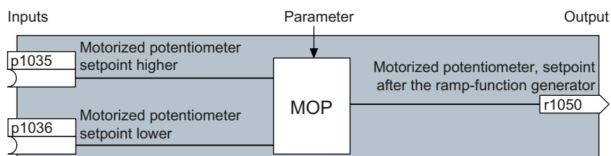
Figure 8-206 Example of a block: Motorized potentiometer (MOP)
