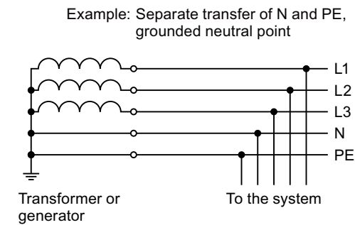
Figure 4-5 TN system
