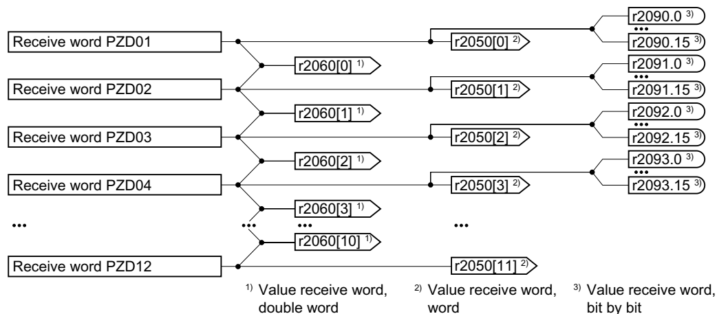
Figure 8-17 Interconnection of the receive data
