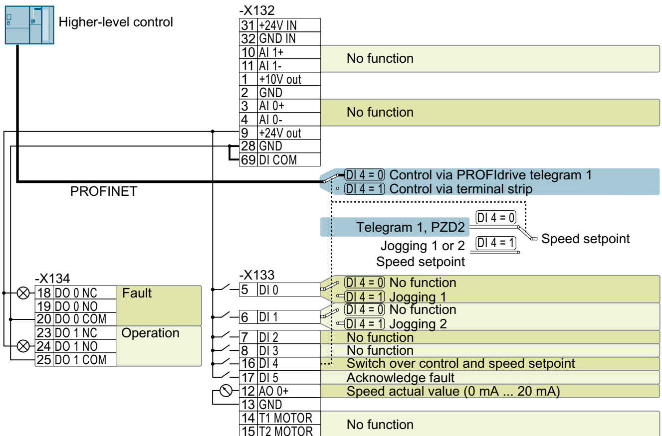
Figure 4-18 Factory setting for converters with PROFINET interfaces
