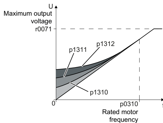
Figure 8-102 The resulting voltage boost using a linear characteristic as example
