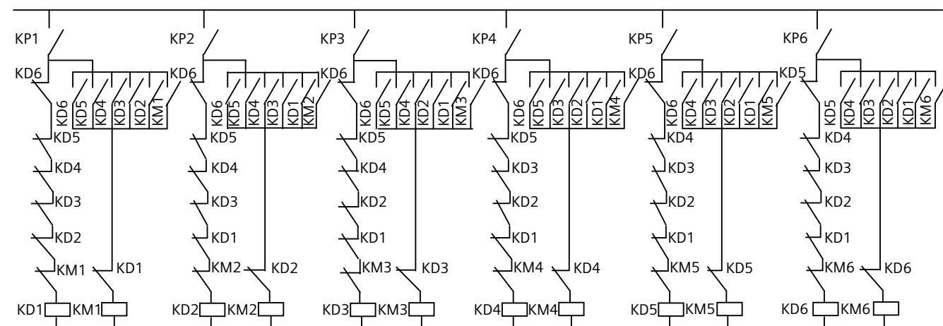
Figure 8-58 External relay control circuit
