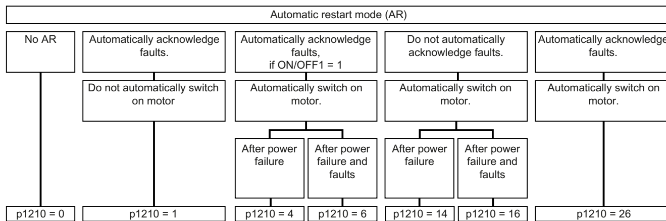
Figure 8-184 Automatic restart modes
