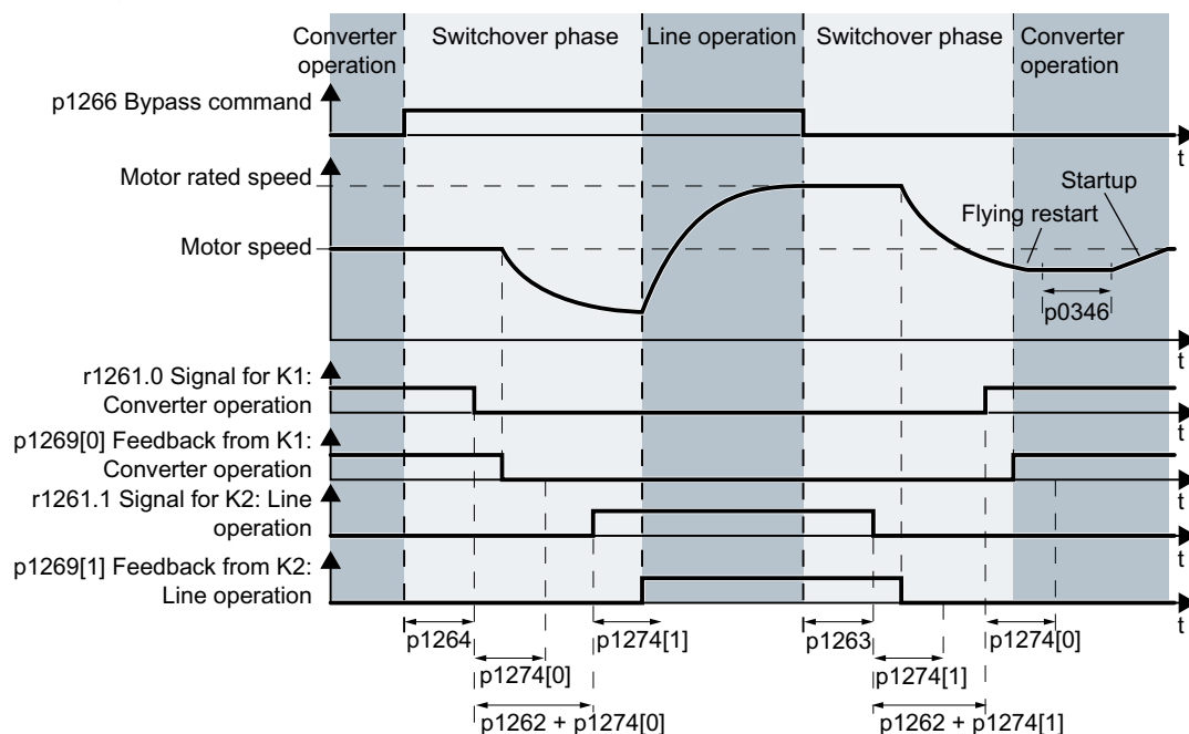
Figure 8-194 Changeover when activating via a control signal ( p1267.0 = 1 )
