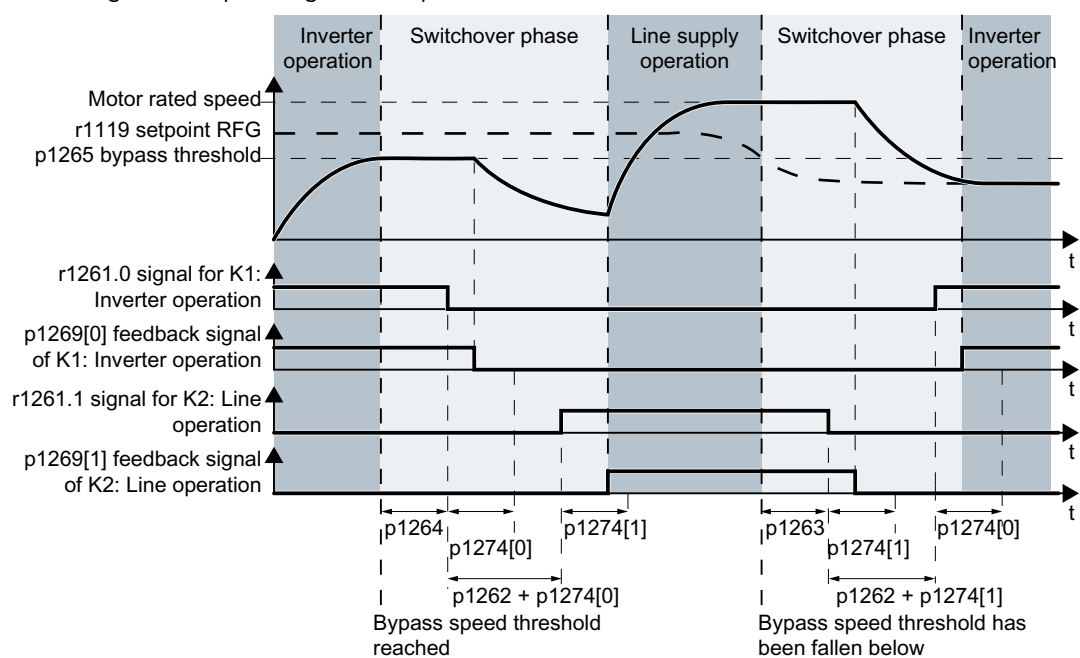
Figure 8-195 Changeover depending on the speed ( p1267.1 = 1 )
