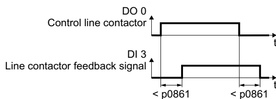
Figure 8-197 Line contactor control via DO 2 with feedback signal via DI 3
