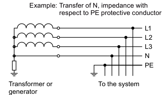
Figure 4-7 IT system
