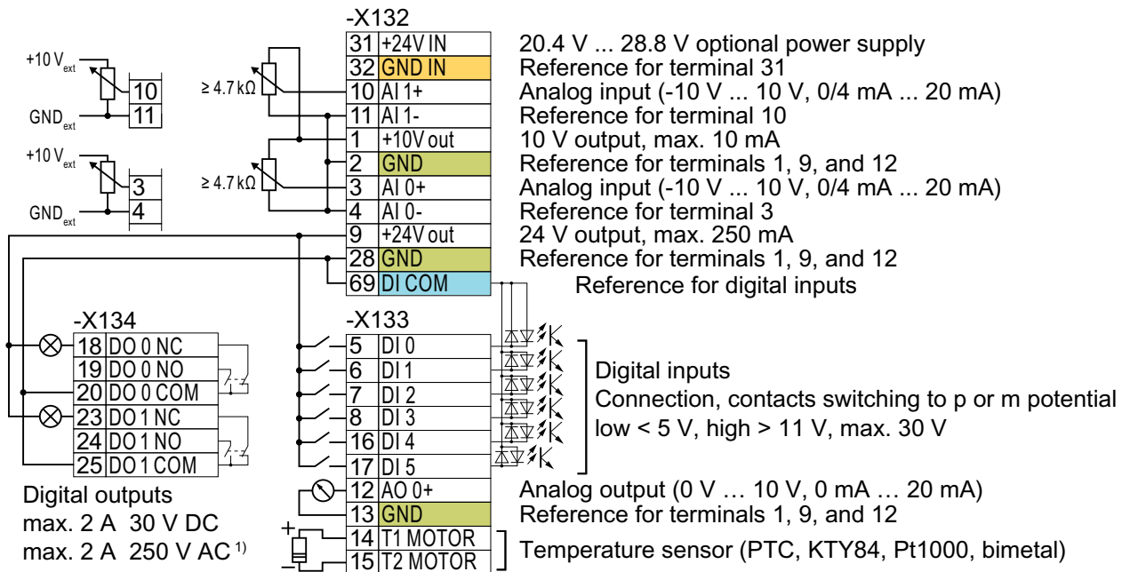
Figure 4-15 Wiring the digital inputs with p-switching contacts and an internal 24 V power supply (terminal 9)
