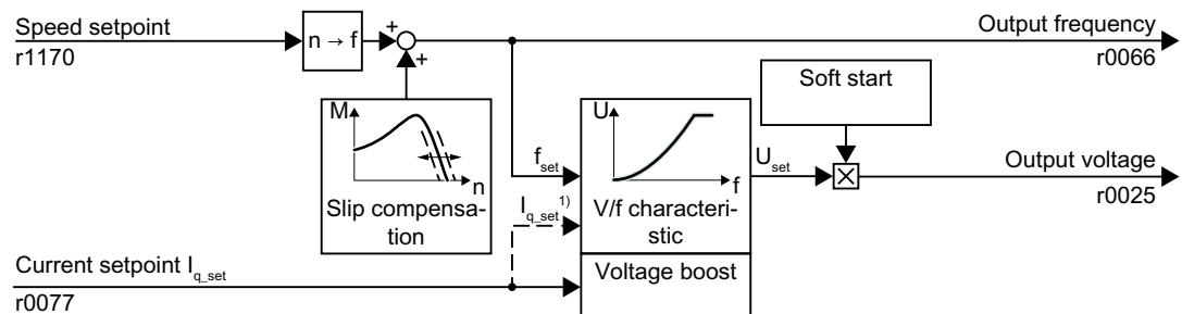
Figure 8-100 Simplified function diagram of the V/f control
