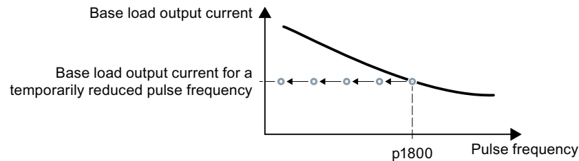
Figure 8-164 Derating characteristic and base load output current for overload
