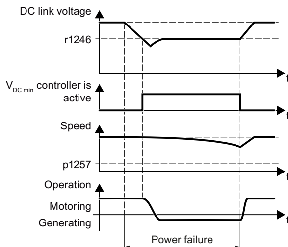
Figure 8-186 Principle mode of operation of kinetic buffering
