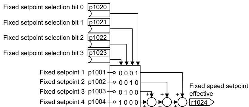
Figure 8-71 Direct selection of the fixed speed setpoint
