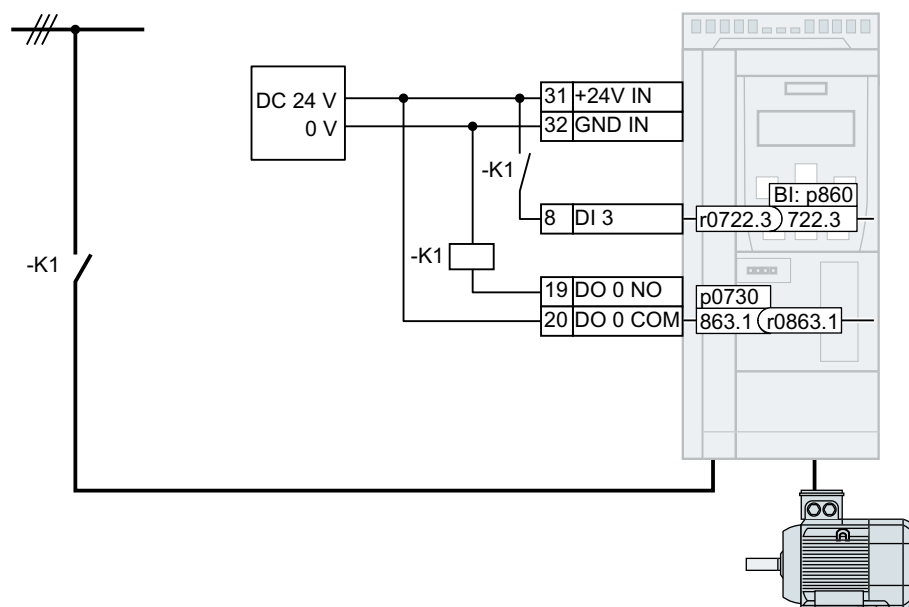
Figure 8-196 Line contactor control via DO 0 with feedback signal via DI 3
