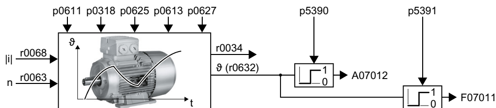
Figure 8-167 Thermal motor model 1 for reluctance motors
