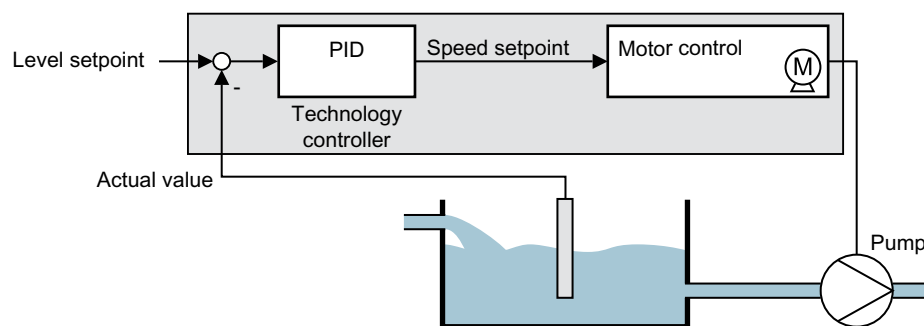
Figure 8-83 Example: Technology controller as a level controller
