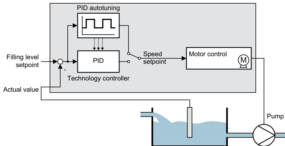
Figure 8-85 Autotuning using closed-loop level control as example
