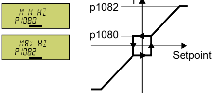
Figure 5-11 Minimum and maximum motor frequency
