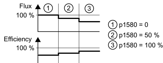
Figure 8-192 Qualitative result of efficiency optimization, method 1
