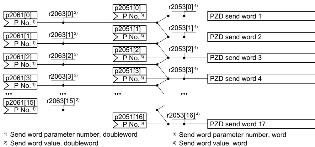
Figure 8-16 Interconnection of the send data
