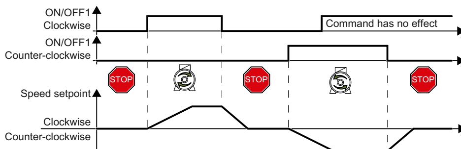
Figure 8-51 Two-wire control, clockwise/counter-clockwise rotation 1
