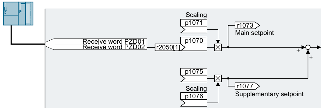
Figure 8-67 Fieldbus as setpoint source
