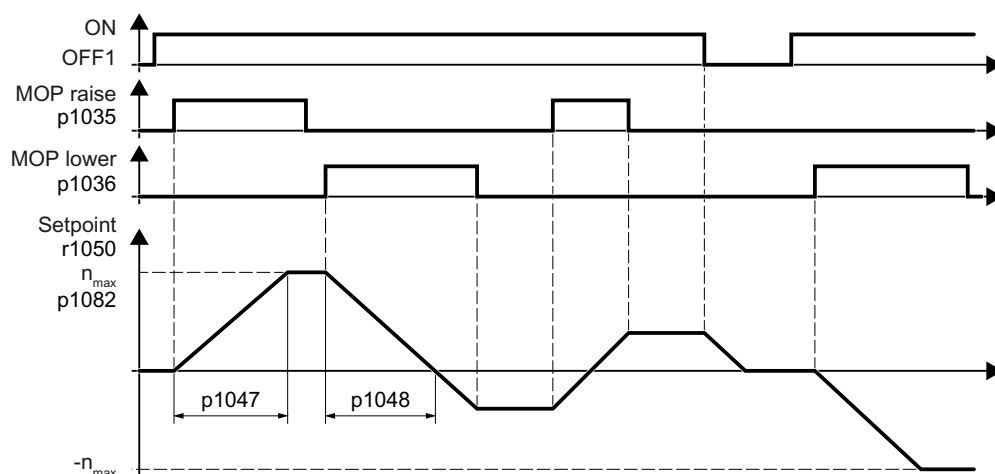
Figure 8-69 Function chart of the motorized potentiometer
