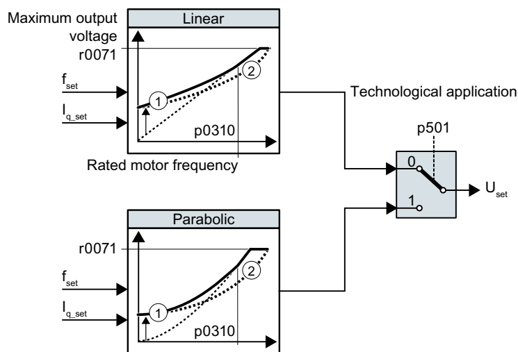
Figure 8-104 Characteristics after selecting Standard Drive Control
