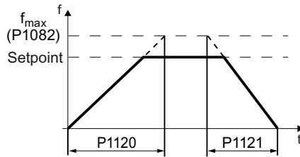
Figure 5-8 Ramp-up and ramp-down time of the motor
