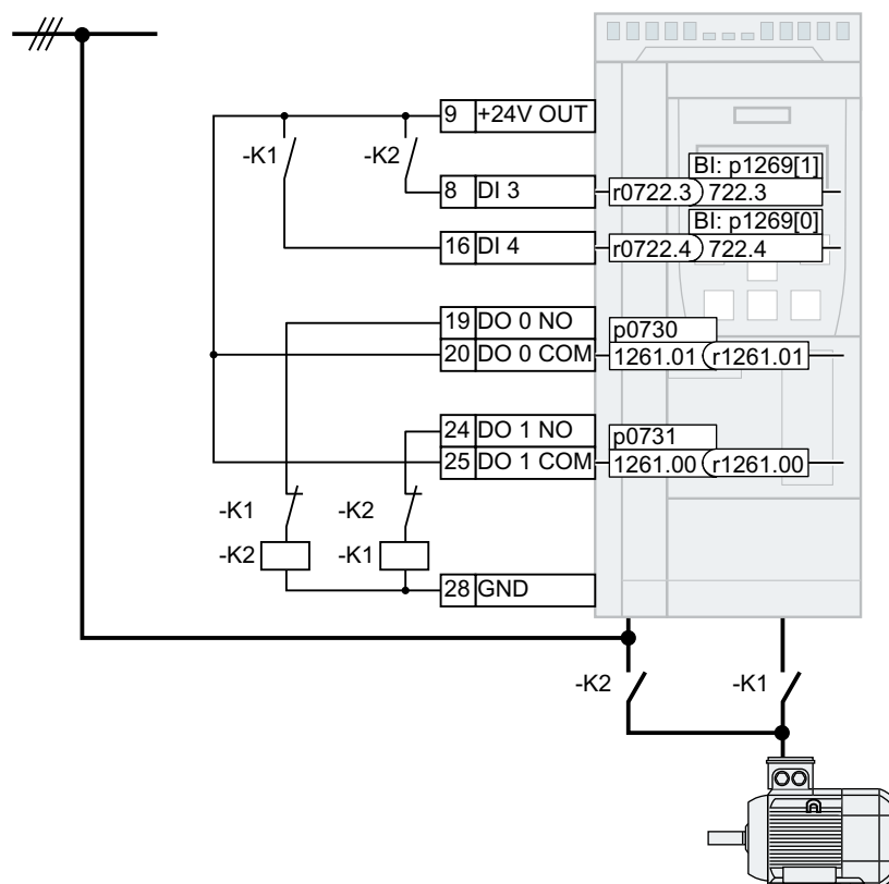
Figure 8-193 Bypass control via converter
