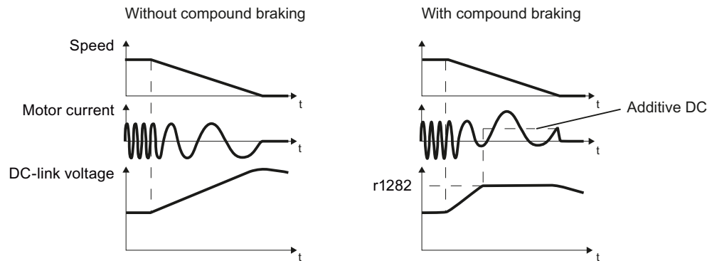
Figure 8-161 Motor brakes with and without active compound braking
