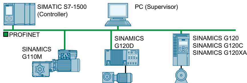
Figure 4-21 The converter in PROFINET IO operation (examples)
