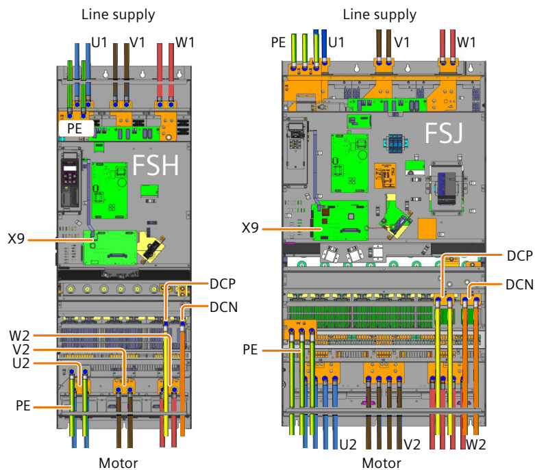
Figure 4-14 Connections for the line supply and motor
