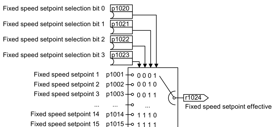
Figure 8-72 Binary selection of the fixed speed setpoint
