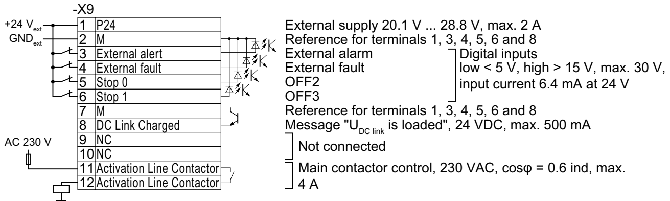
Figure 4-19 Connecting external 24 V power supply
