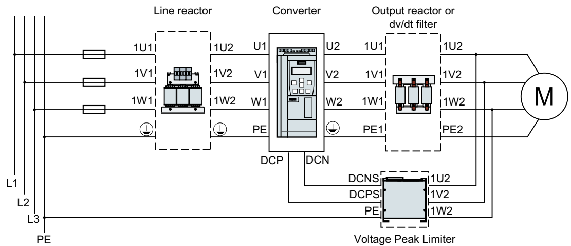
Figure 4-10 Connecting converters FSH/FSJ and their optional components
