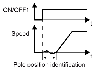
Figure 8-163 Pole position identification after switching on the motor
