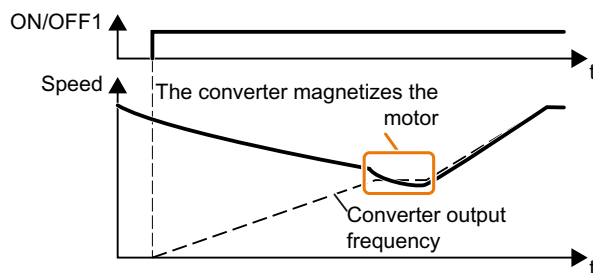
Figure 8-183 Principle of operation of the "flying restart" function
