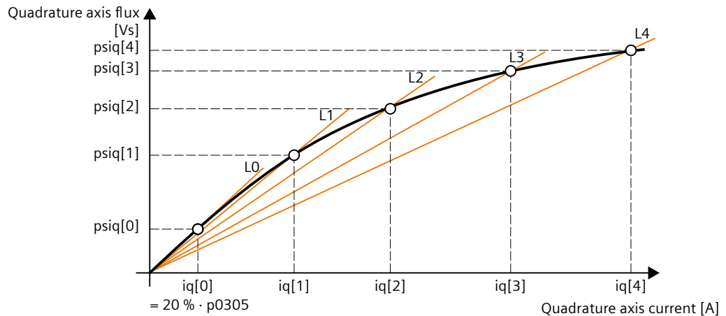
Figure 8-99 Saturation characteristic of the permanent magnet synchronous motor
