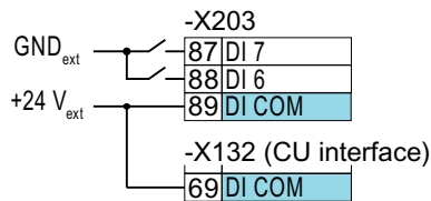
Figure 2-3 Connecting M-switching contacts
