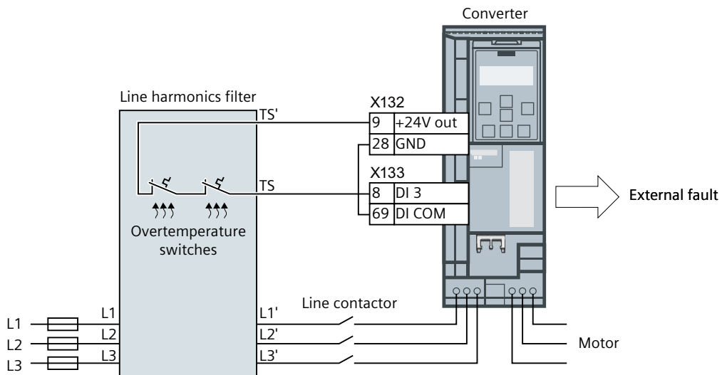
Figure 2-1 Protection of the line harmonic filter
