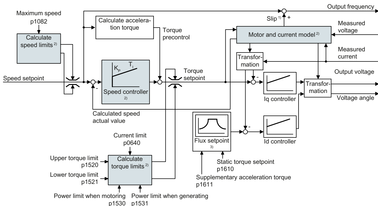
Figure 8-116 Simplified function diagram for sensorless vector control with speed controller
