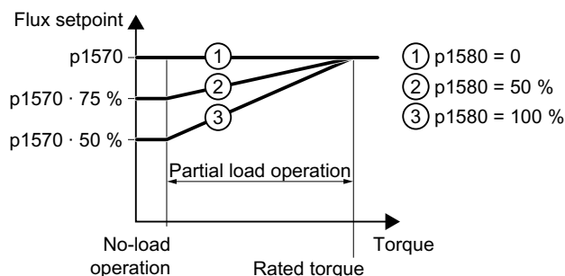
Figure 8-191 Reduce the flux setpoint in the partial load range of the motor
