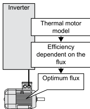
Figure 8-189 Determining the optimum flux from the motor thermal model
