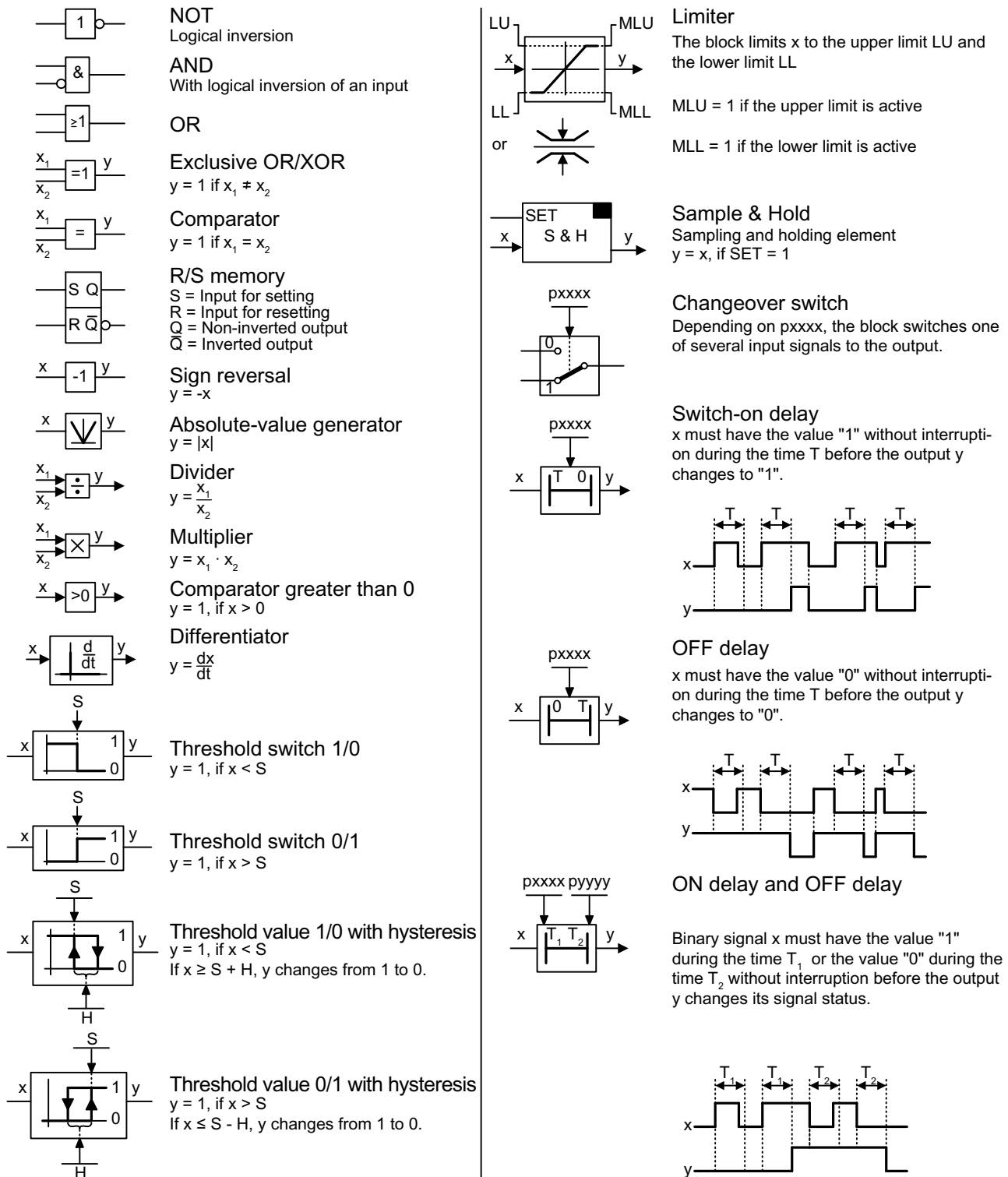
Figure 8-204 Binary and analog blocks
