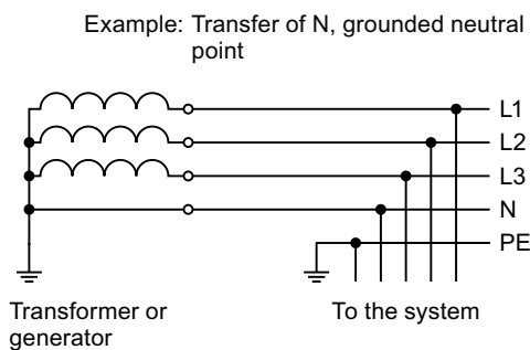
Figure 4-6 TT system
