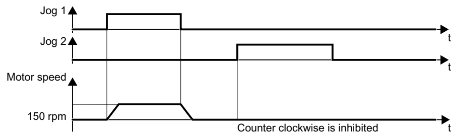
Figure 5-5 Logging the motor in the factory setting
