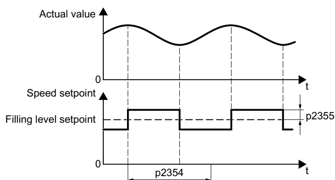
Figure 8-86 Example for speed setpoint and actual process value for autotuning
