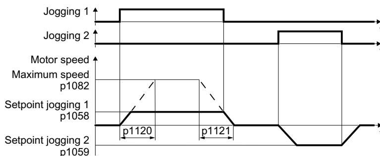
Figure 8-33 Behavior of the motor when "jogging"
