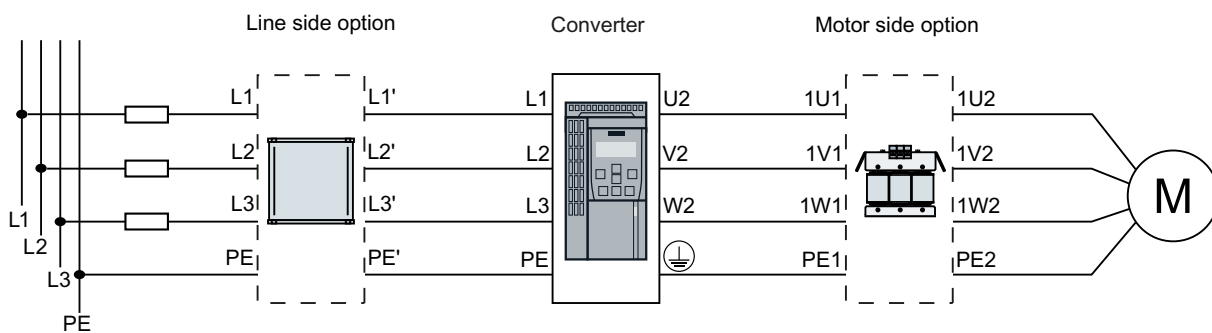
Figure 4-9 Connecting converters FSA...FSG and their optional components
