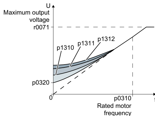
Figure 8-105 The resulting voltage boost using a linear characteristic as example
