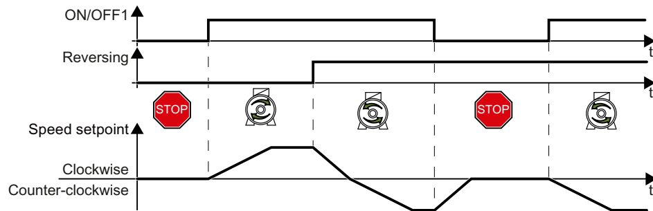
Figure 8-50 Two-wire control, ON/reverse
