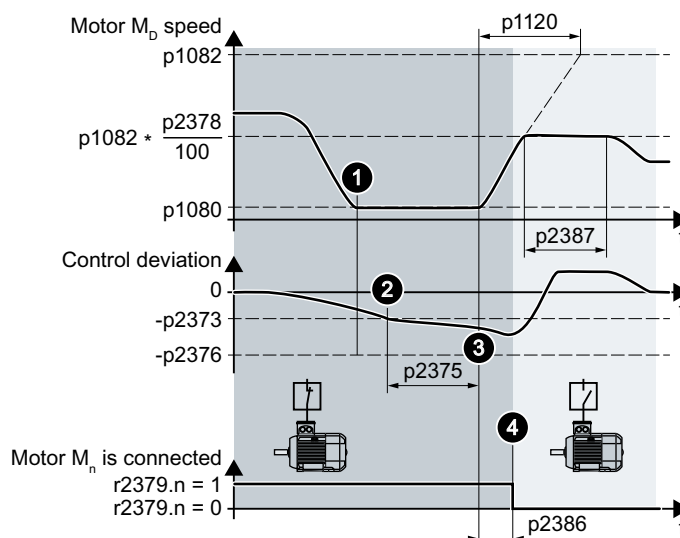
Figure 8-95 Deactivate uncontrolled motors M_1 \dots M_2
