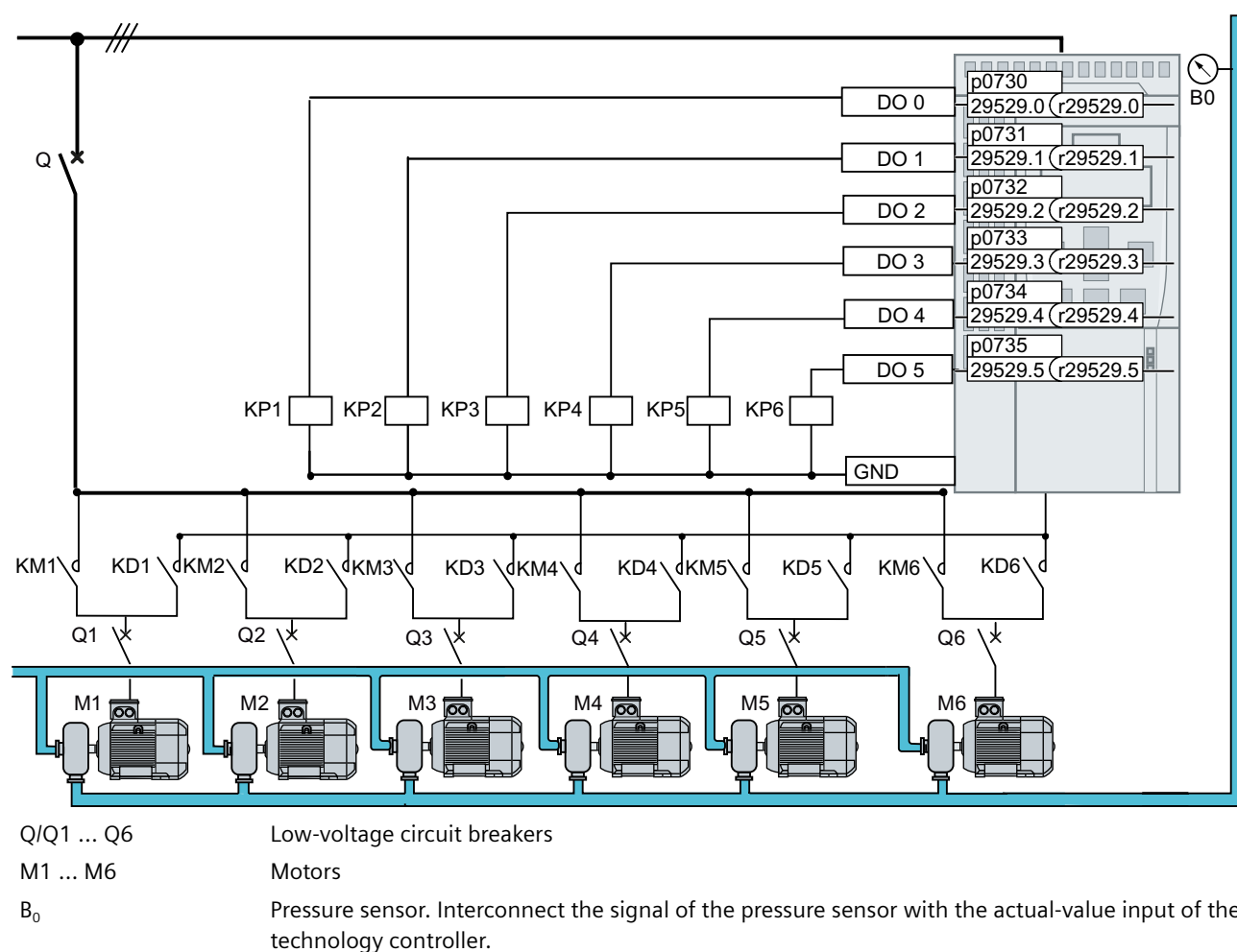
Figure 8-57 Mains circuit
