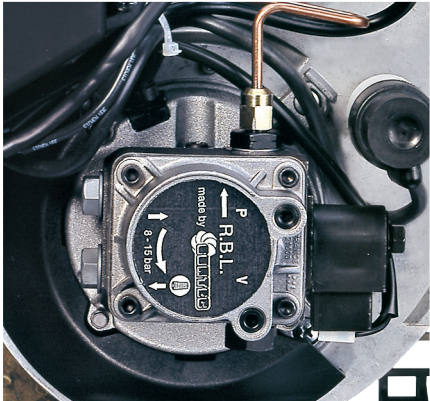
Fuel pump
