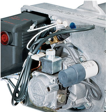
Pre-heater
