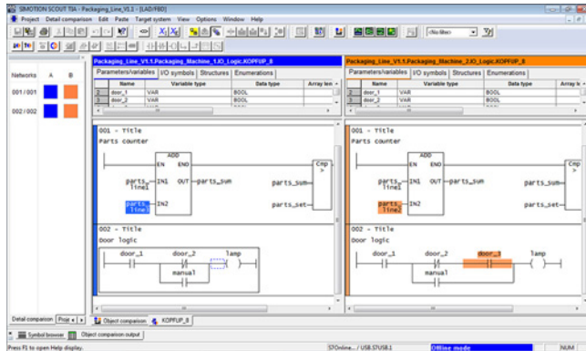
Detail comparison with ladder logic (LAD)
