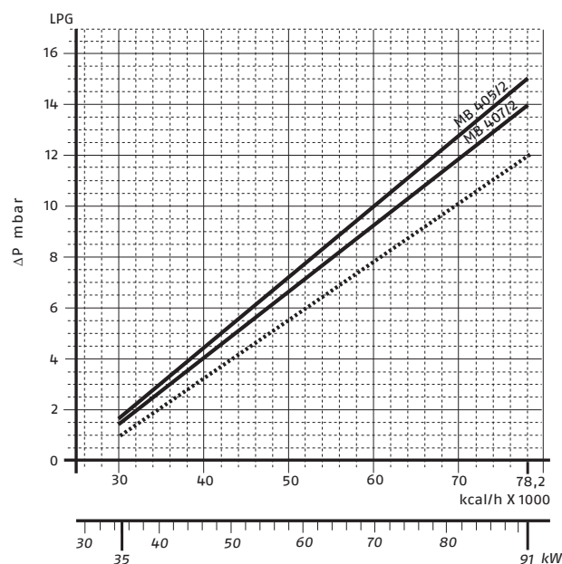
BS2D (LPG)
