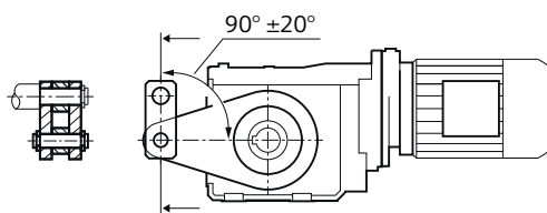
Figure 6-16 Toggle lever design
