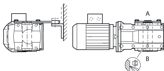
Figure 12-33 Mounting positions for bevel gearbox BAD shaft-mounted design, sizes 19 - 29
