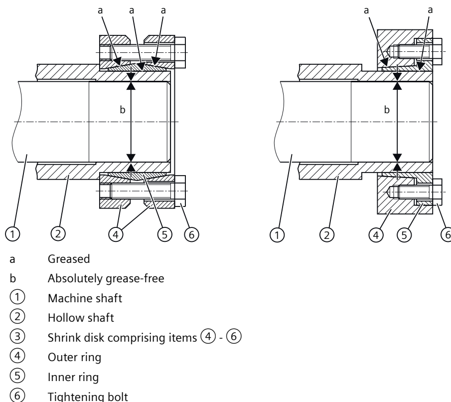
Figure 6-9 Mounting the shrink disk
