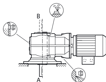
Figure 12-36 Mounting positions for bevel gearbox K.F flange-mounted design and KAZ with housing flange, sizes 39 - 189
