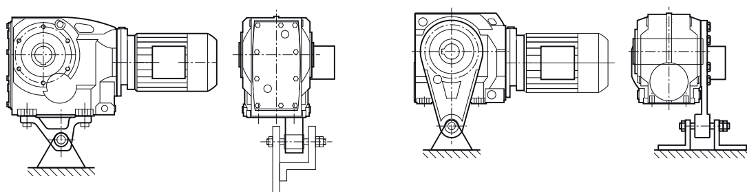
Figure 6-13 Mounting suggestion for torque arm on foot and flange
