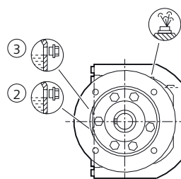
Figure 12-21 Mounting positions for helical gearbox DF/ZF flange-mounted design and DZ/ZZ with housing flange, size 39
