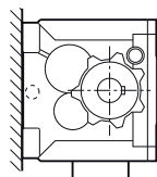
Figure 12-16 Mounting positions for helical gearbox D/Z foot-mounted design, sizes 19 - 29
