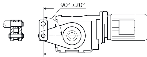
Figure 6-14 Toggle lever design
