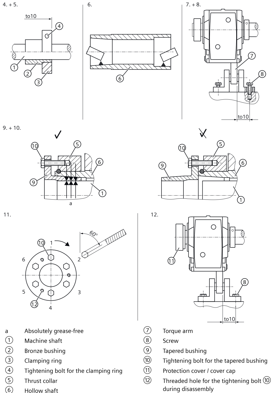
Figure 6-10 Installing SIMOLOC
