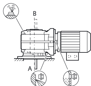
Figure 12-43 Mounting positions for helical worm gearbox CF flange-mounted design and CAZ housing flange, sizes 39 - 89
