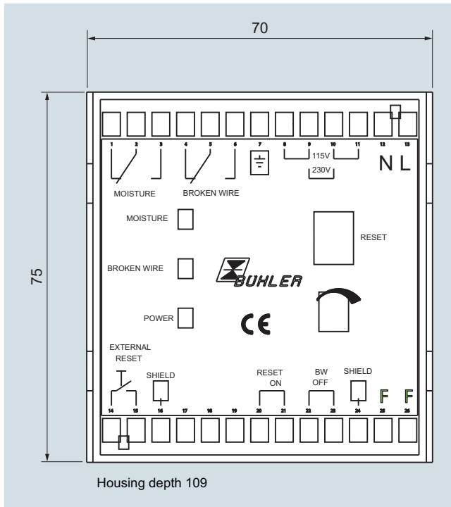
Wiring module for non-hazardous applications
