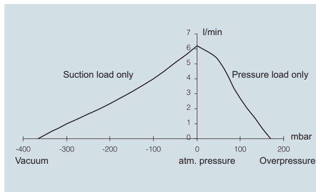
Diaphragm pump, capacity
