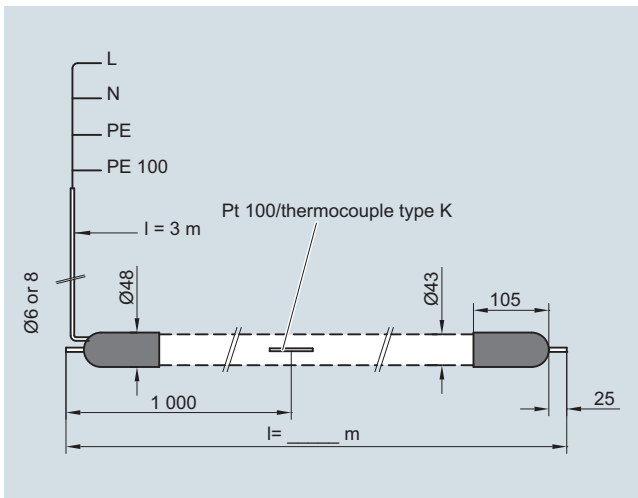
Temperature-controlled, heated sample gas line for operating temperatures up to max. 200 °C, non-replaceable Teflon core
