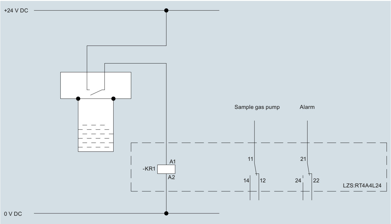
Example wiring with sample gas pump
