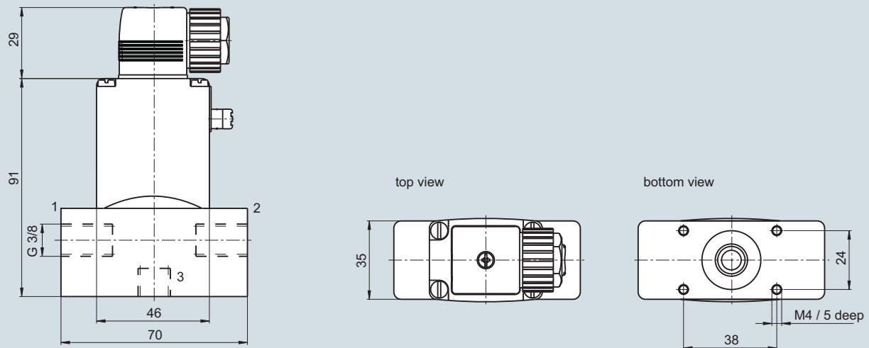
3/2-way solenoid valve 24/230V made of PVDF, with appliance socket
