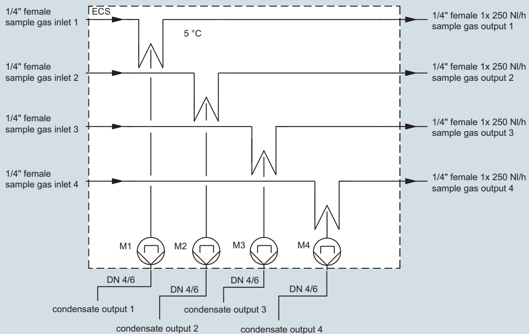
Design with 4 gas paths
