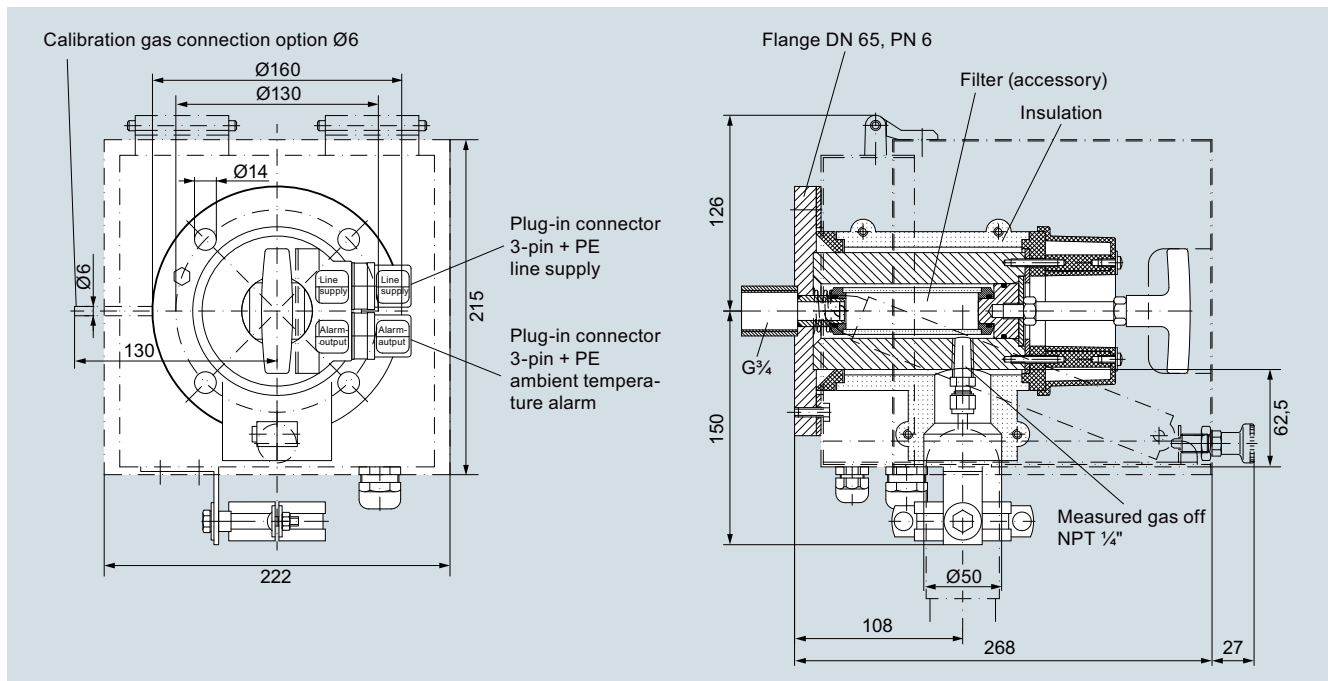
Gas sampling probe with external, electrically heated filter, with self-regulating heating elements (weatherproof cover indicated by dash-dotted line)
