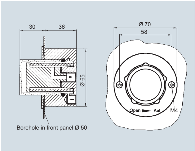
Front mounting filter
