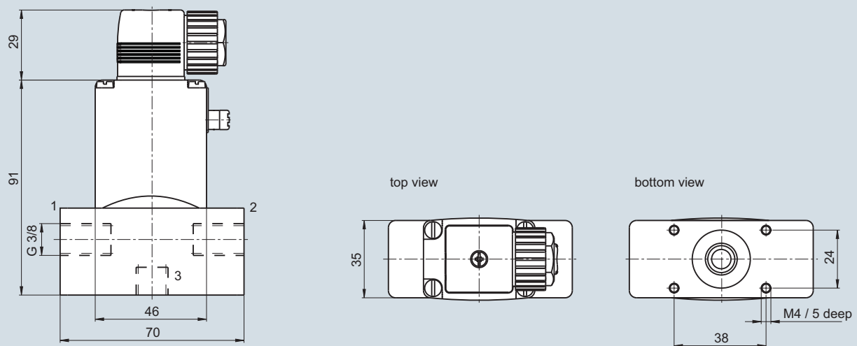
2/2-way solenoid valve 24/230 V made of PVDF, with appliance socket
