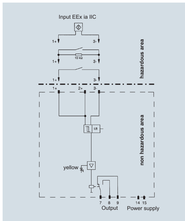
Isolated switch amplifier, schematic diagram (1 channel)
