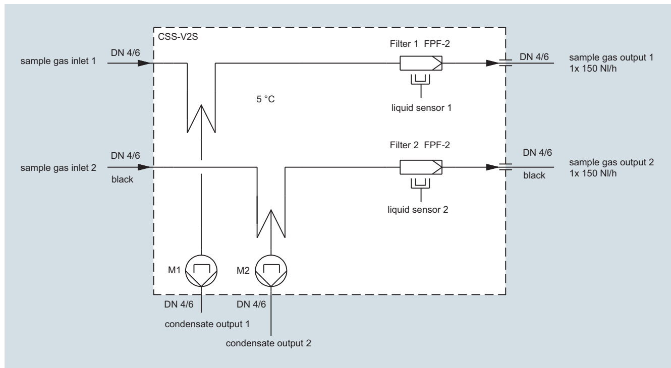
Design with 2 gas paths; version 2
