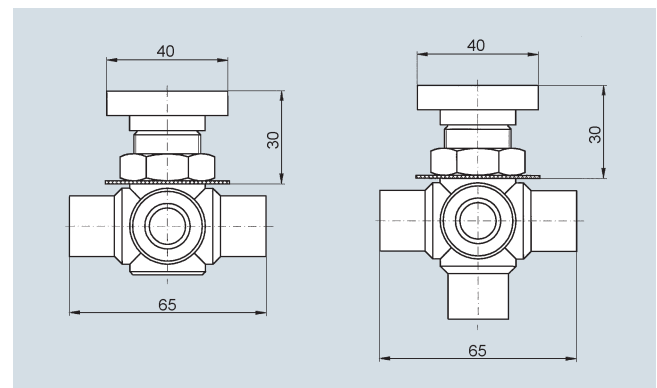
3-way and 5-way ball valves
