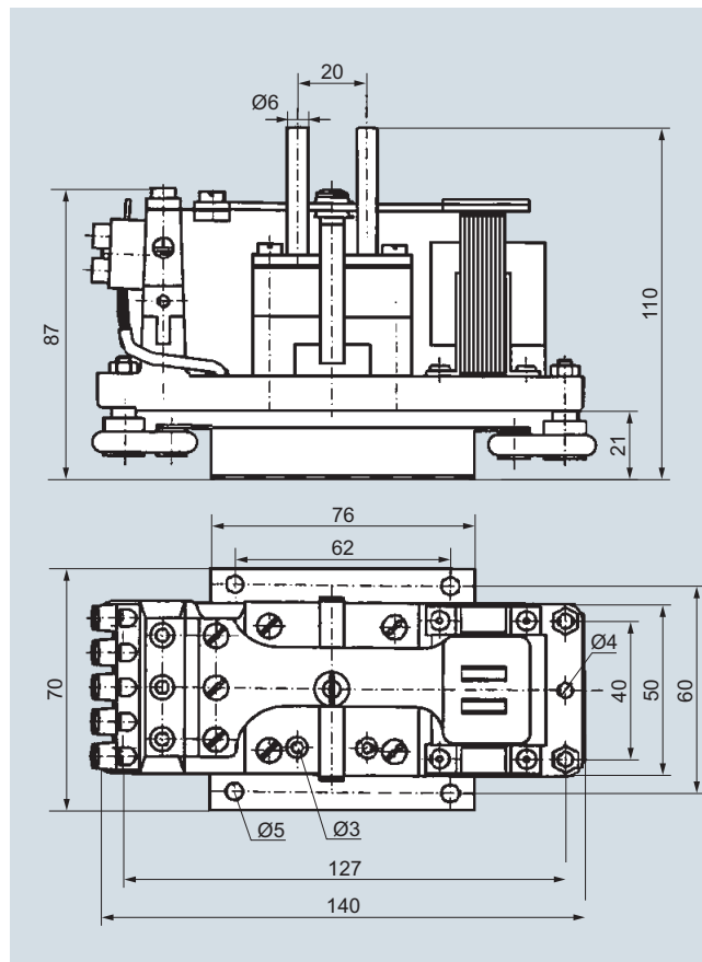
Diaphragm pump with metal-free gas ducts and pump suspension
