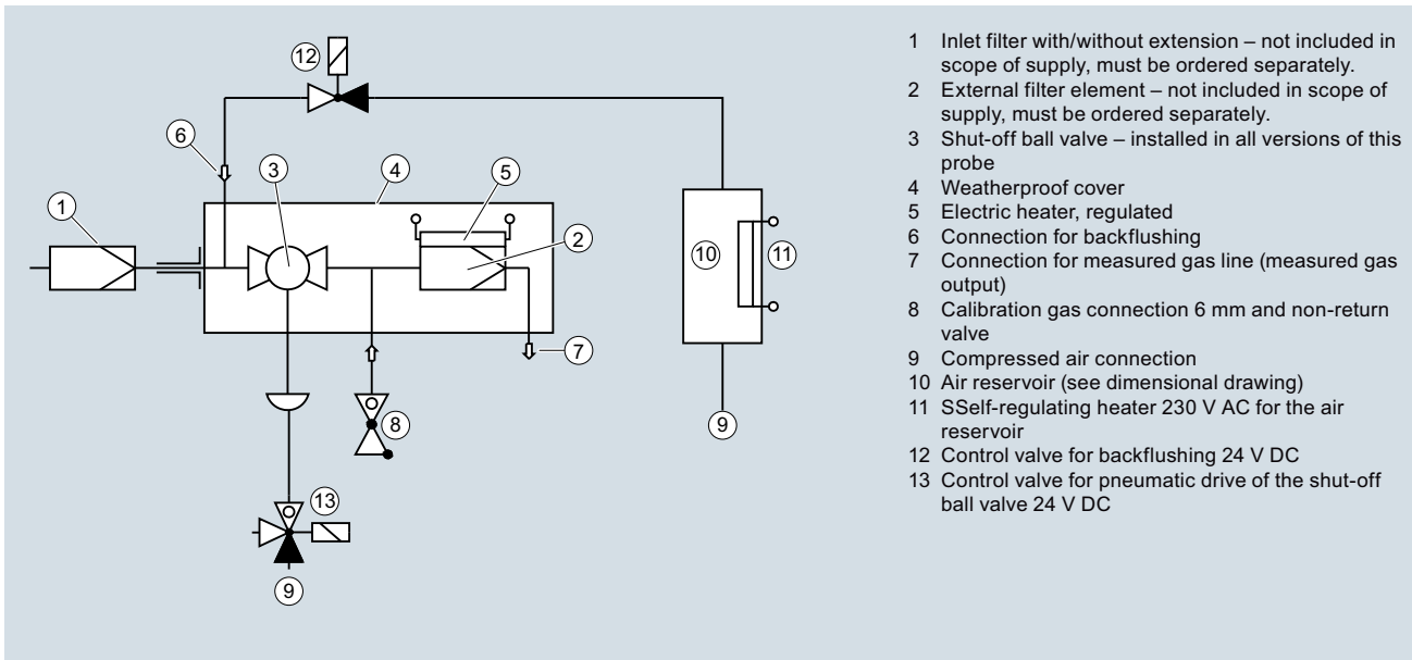
Diagram of the probe 7MB1943-2FA07
