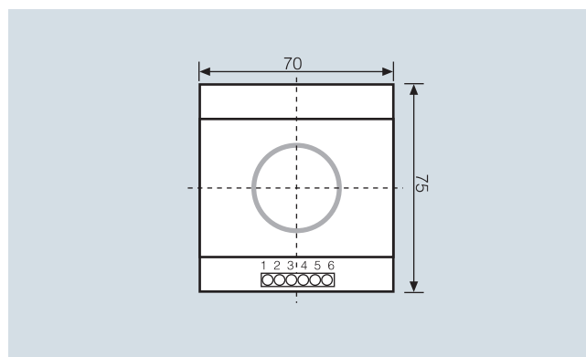
Pump controller
