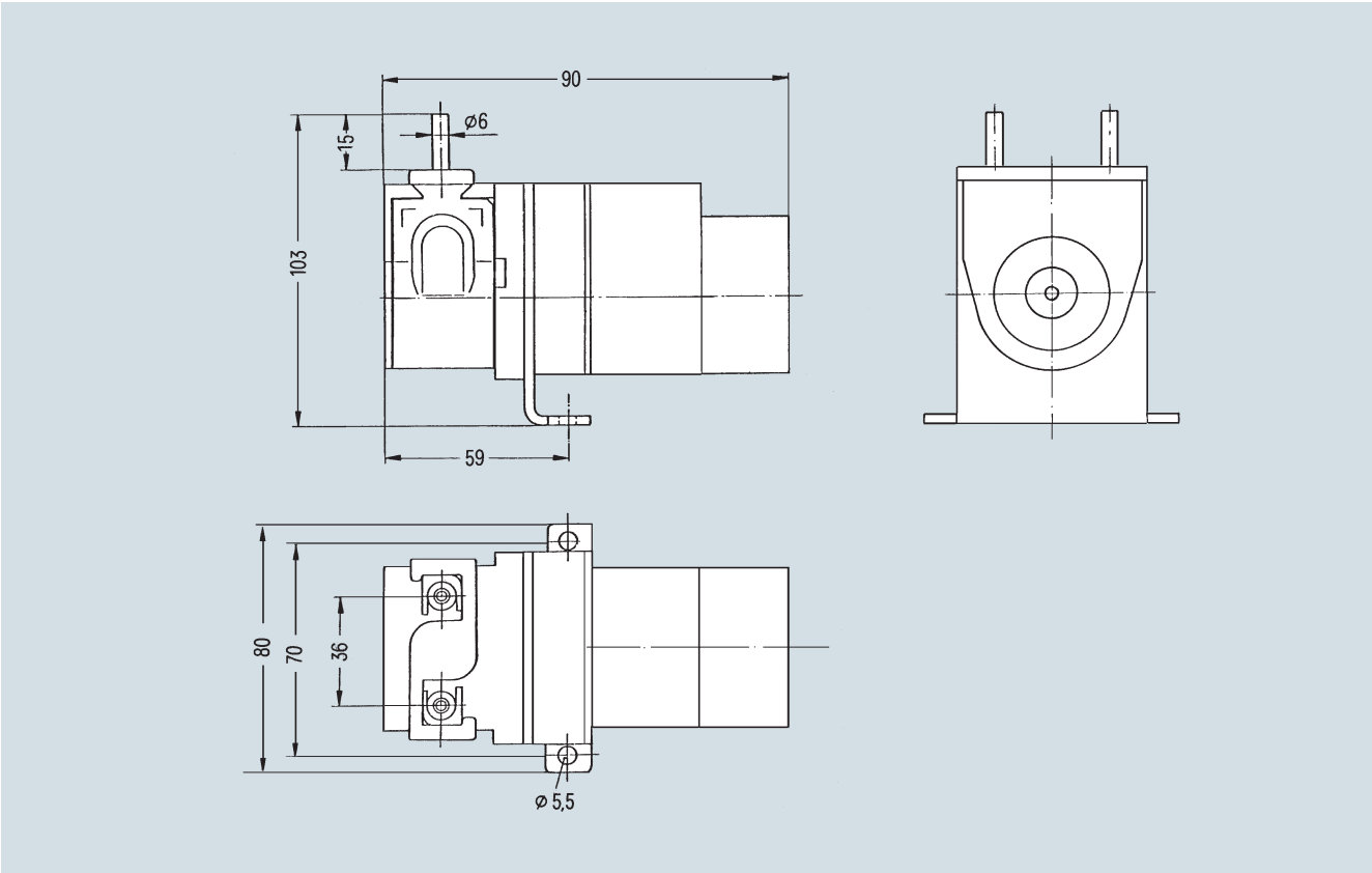
Hose pump
