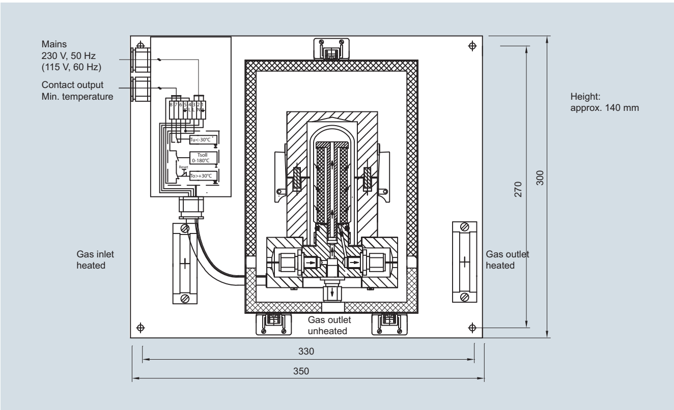
Temperature-controlled, heated sample gas filter for operating temperatures up to max. 180 °C, gas inlet on left (for FIDAMAT total hydrocarbon analyzer)
