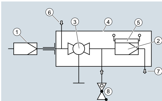
Diagram of the probe 7MB1943-2FA03
