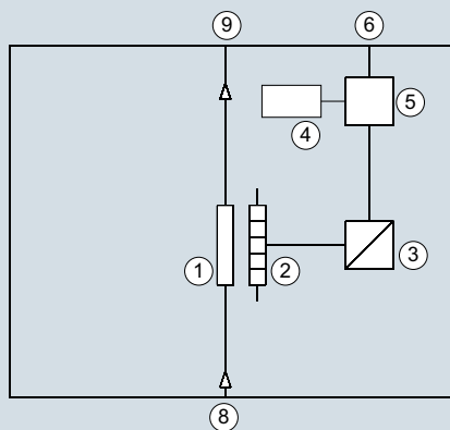
Converter without solenoid valves
