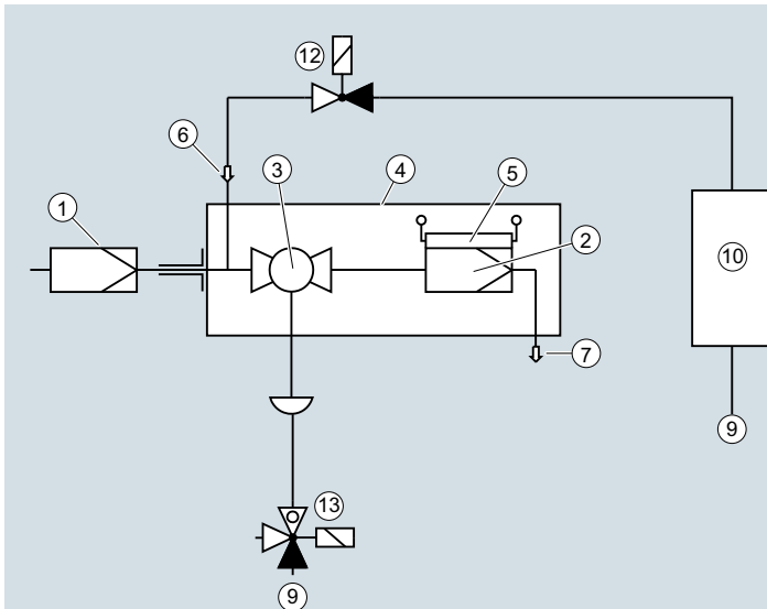
Diagram of the probe 7MB1943-2FA04
