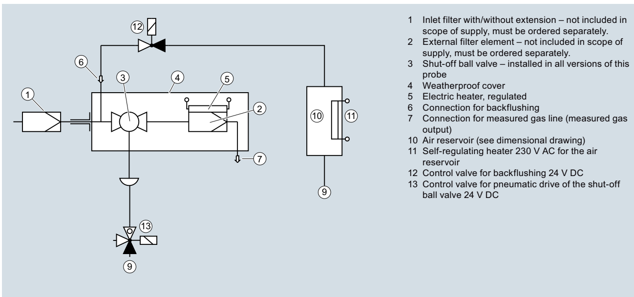
Diagram of the probe 7MB1943-2FA06
