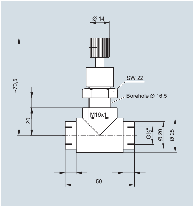
Needle valve made of PVDF
