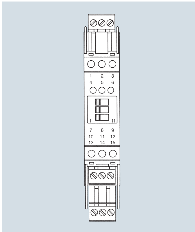
Isolated switch amplifier, front view
