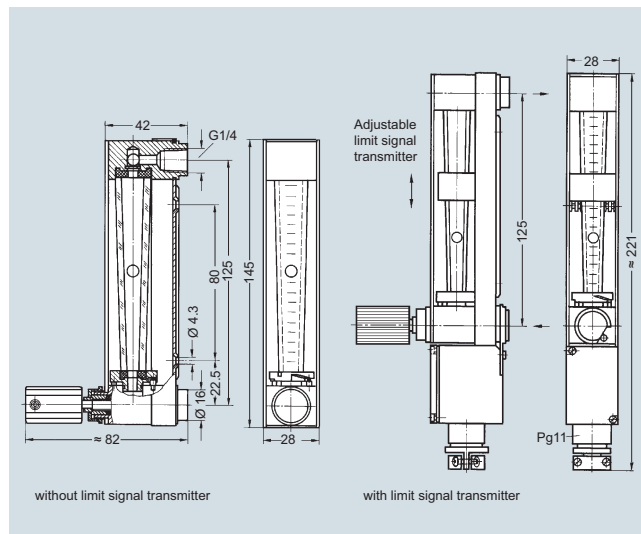
Flowmeter DK 800
