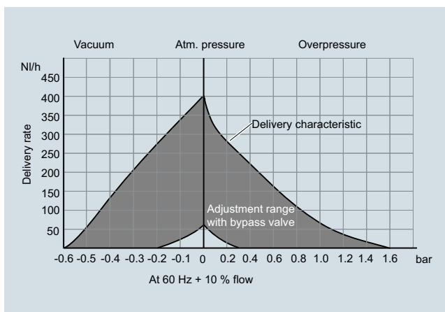
Corrosion-resistant bellows pump, capacity
